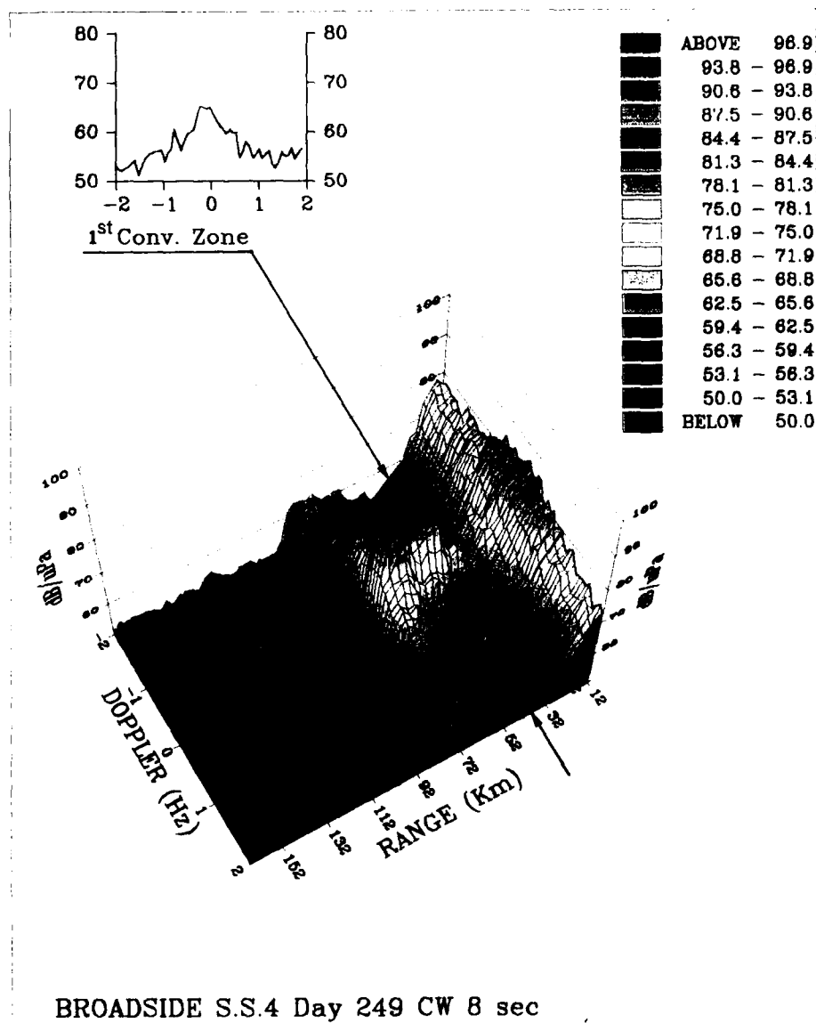
Fig. 24. Spectral time history of received intensities: 8 s, 370 Hz CW transmission, broadside beam; sea-state 4.
