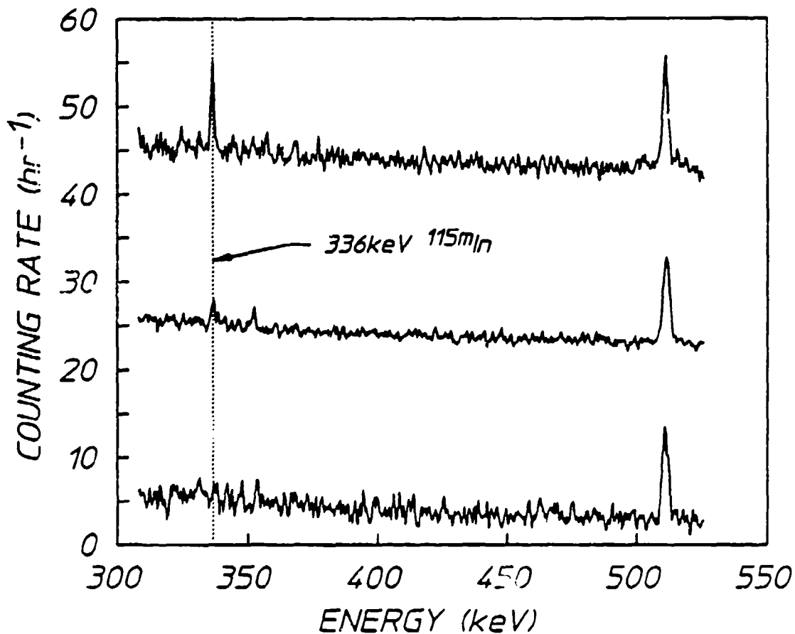
Figure 2: Three sequential spectra from an intrinsic Ge detector begun at times 6.5, 9.2, and 19.0 hours after the irradiation with a flash of bremsstrahlung with a 1.3 MeV end point. Data have been offset by 40, 20, and 0 counts/h, respectively. The 336.2 keV peak is seen to decay with the appropriate half-life of 4.49 hours for ^{115m}\text{In} . The other structure is the annihilation peak at 511 keV.
