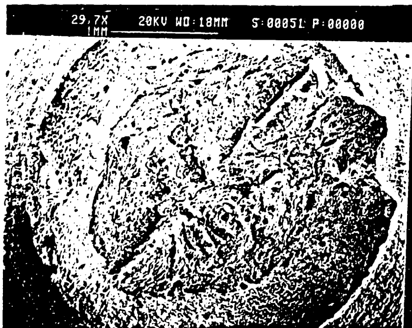
Figure 27(b.) Sample 51 (-30°C) Fracture Surface, Low Magnification
