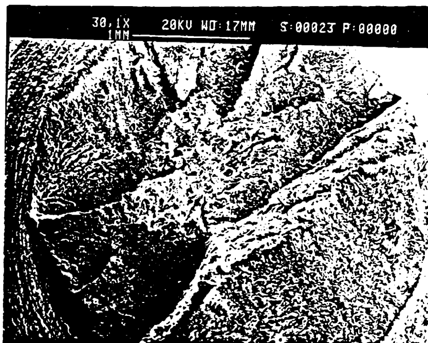
Figure 27(e.) Sample 23 (-101°C) Fracture Surface, Low Magnification
