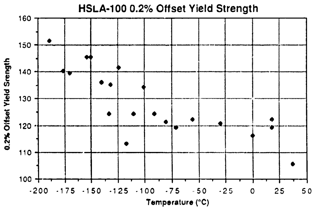
Figure 21 0.2 Percent Offset Yield Strength
