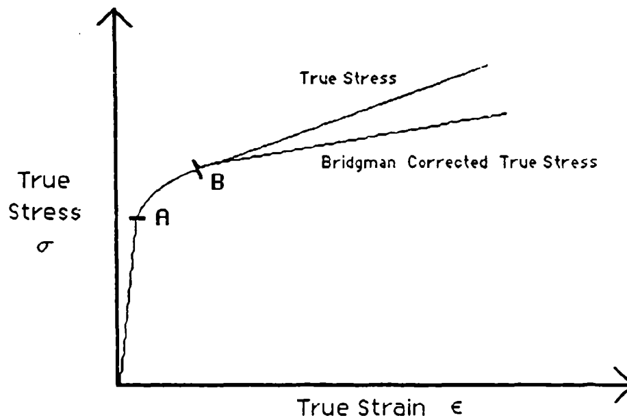
Figure 2. Typical True Stress-True Strain Curve
