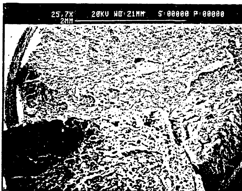
Figure 27(h.) Sample 47 (-150°C) Fracture Surface, Low Magnification
