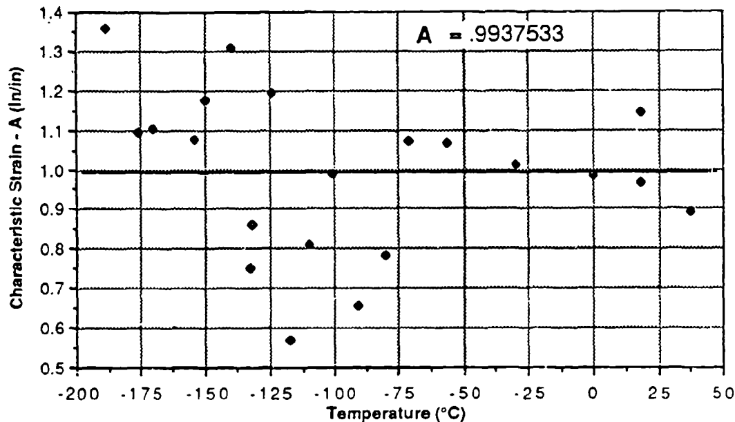
Figure 15 Characteristic Strain as a Function of Temperature
