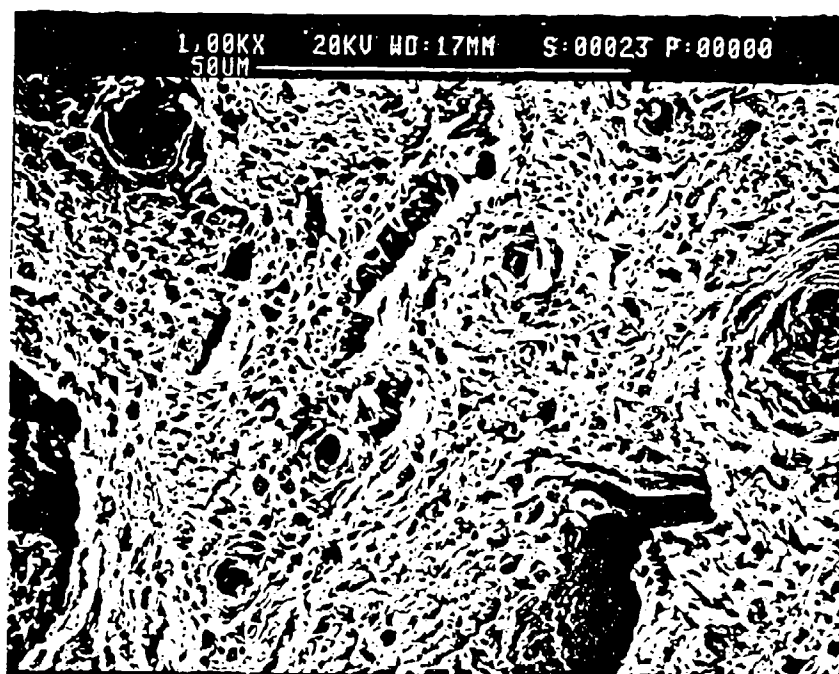
Figure 27(f.) Sample 23 (-101°C) Fracture Surface, High Magnification
