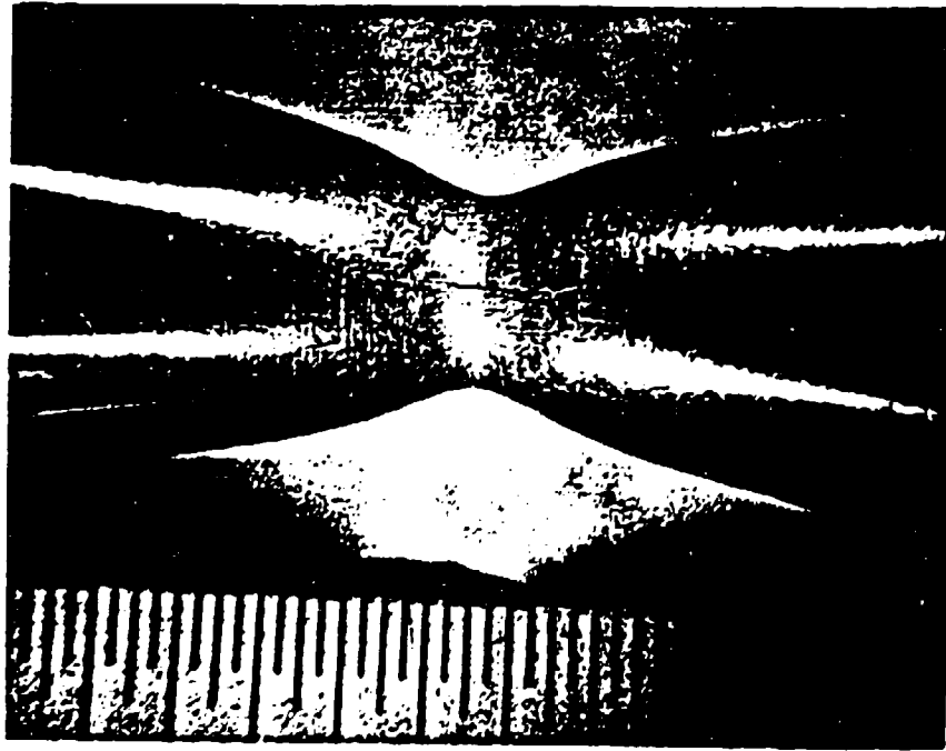
Figure 24 HSLA-100 Sample 19 (-117°C) Vertical Split 1 Ruler Division \approx 1/64 inch
