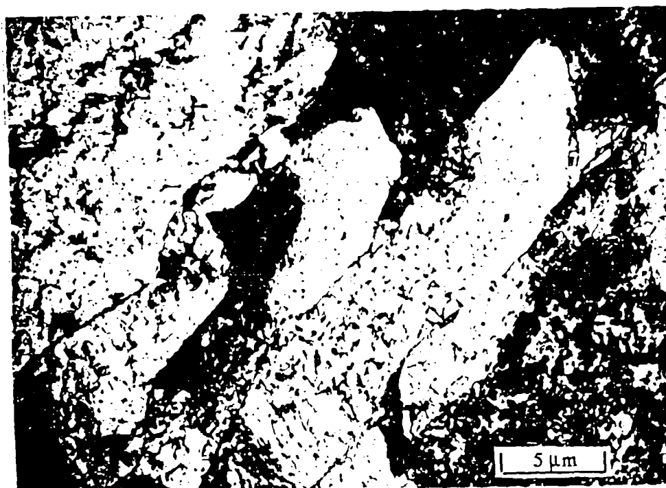
Figure 5 TEM Micrograph of Aged HSLA-100
