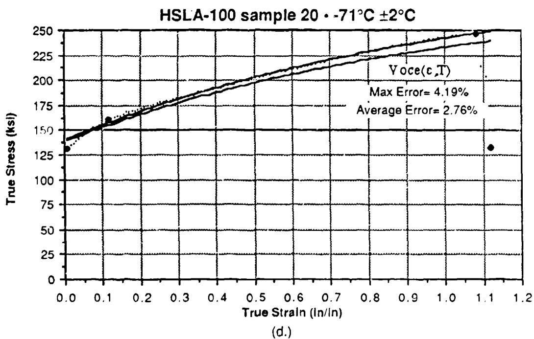
Figure 18 Final Voce( \epsilon, T ) Comparison Plots
