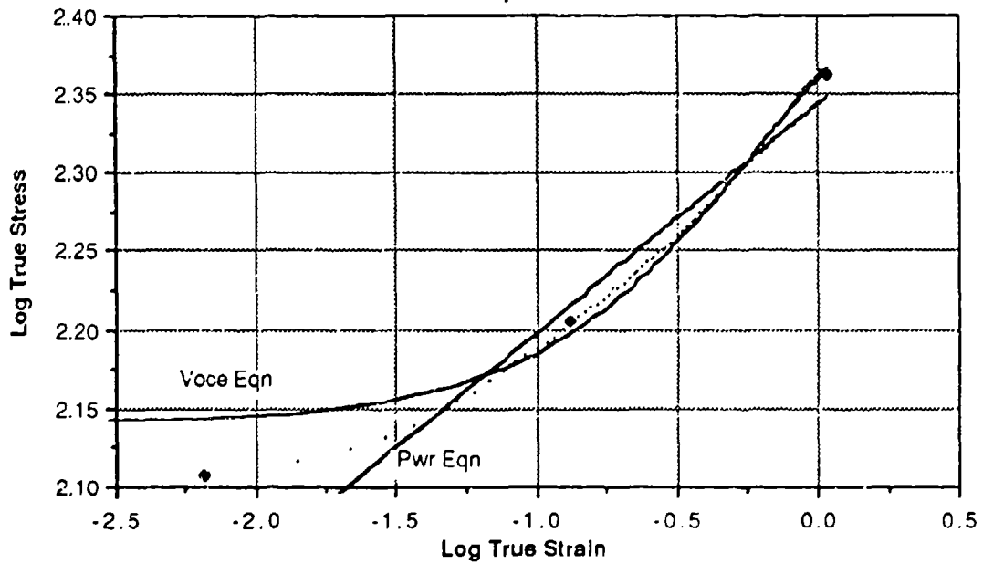
Figure 13 Comparison of the Voce and Power Equations
