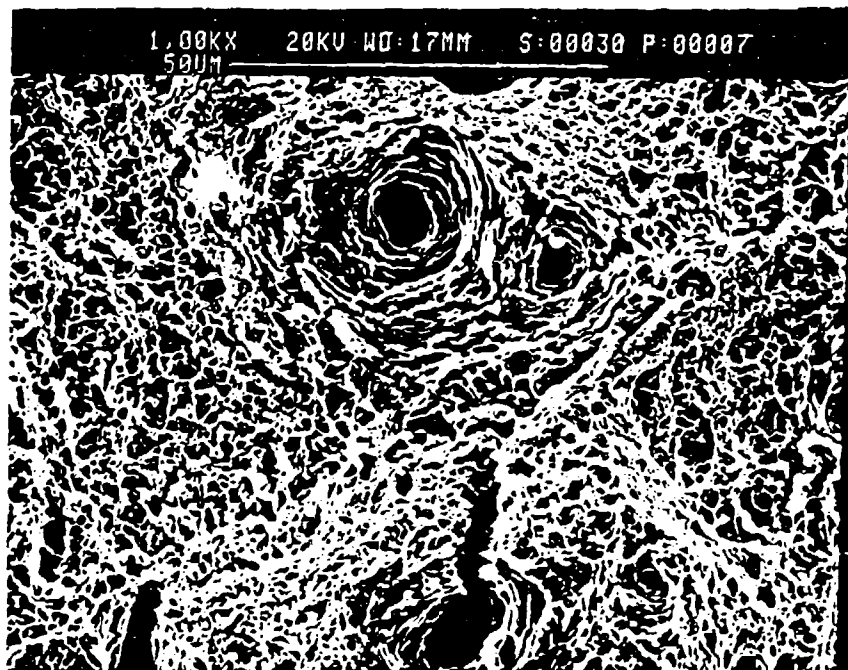
Figure 27(c.) Sample 30 (6°C) Fracture Surface, High Magnification
