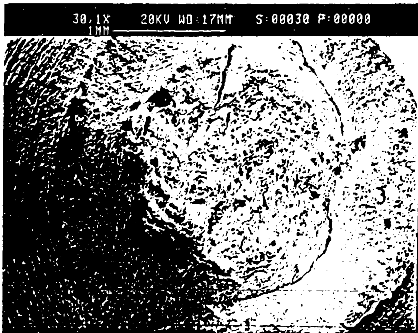
Figure 27(a.) Sample 30 (0°C) Fracture Surface, Low Magnification
