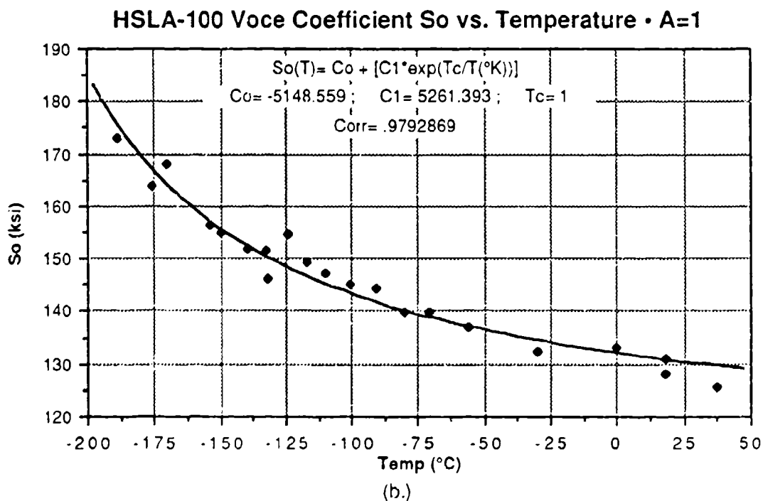
Figure 17 Voce Stress Coefficients as a Function of Temperature (2)
