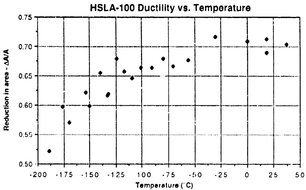
Figure 22 Ductility of HSLA-100
