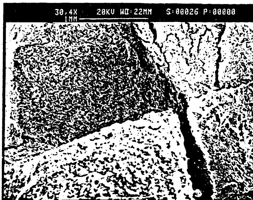
Figure 27(g.) Sample 26 (-140°C) Fracture Surface, Low Magnification
