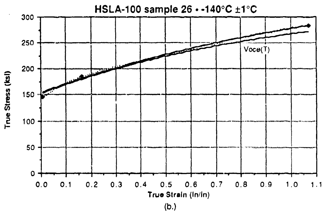
Figure 16 Voce(T, \epsilon ) - Plots of Two Tests
