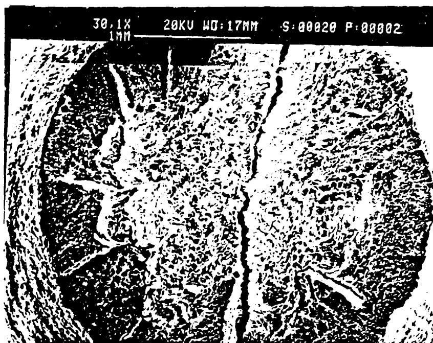
Figure 27(d.) Sample 20 (-71°C) Fracture Surface, Low Magnification
