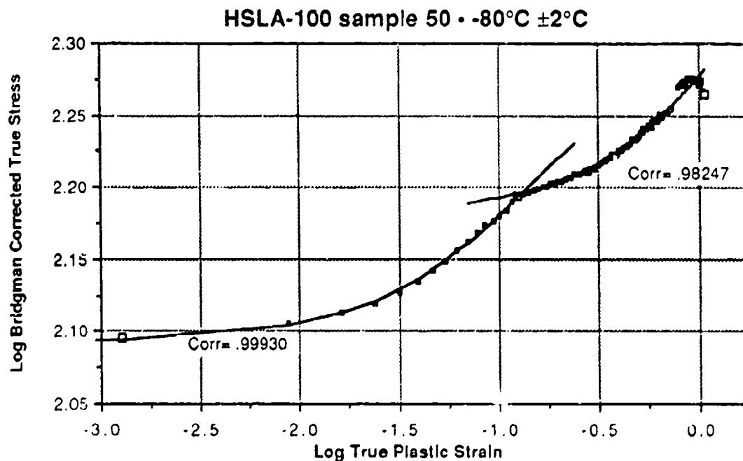
Figure 29 Two Curve Fit for the Bridgman Corrected True Stress / True Plastic Strain
