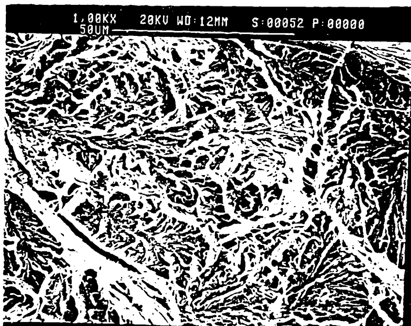
Figure 27(i.) Sample 52 (-170°C) Fracture Surface, High Magnification
