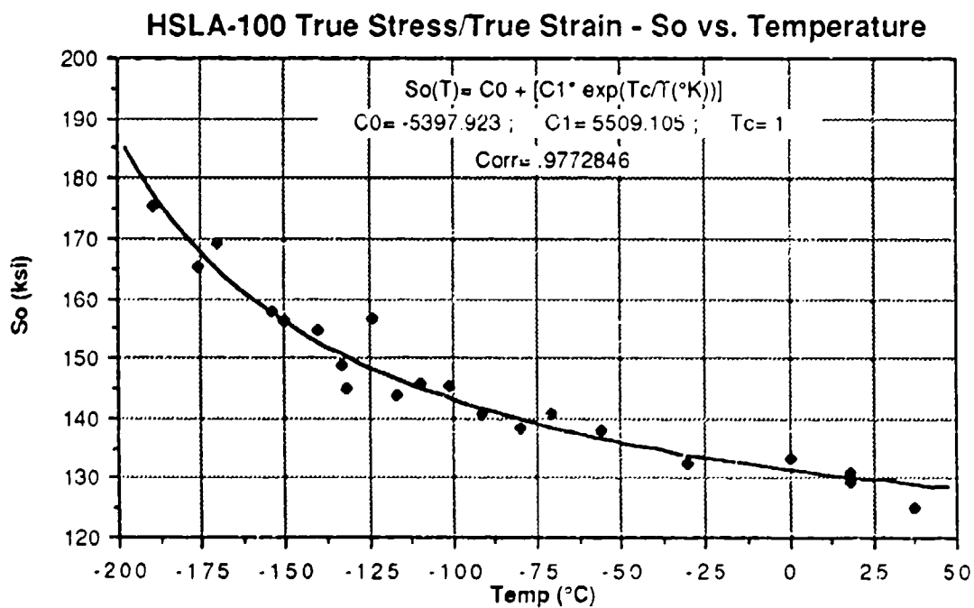
Figure 14 Voce Stress Coefficients as a Function of Temperature (1)
