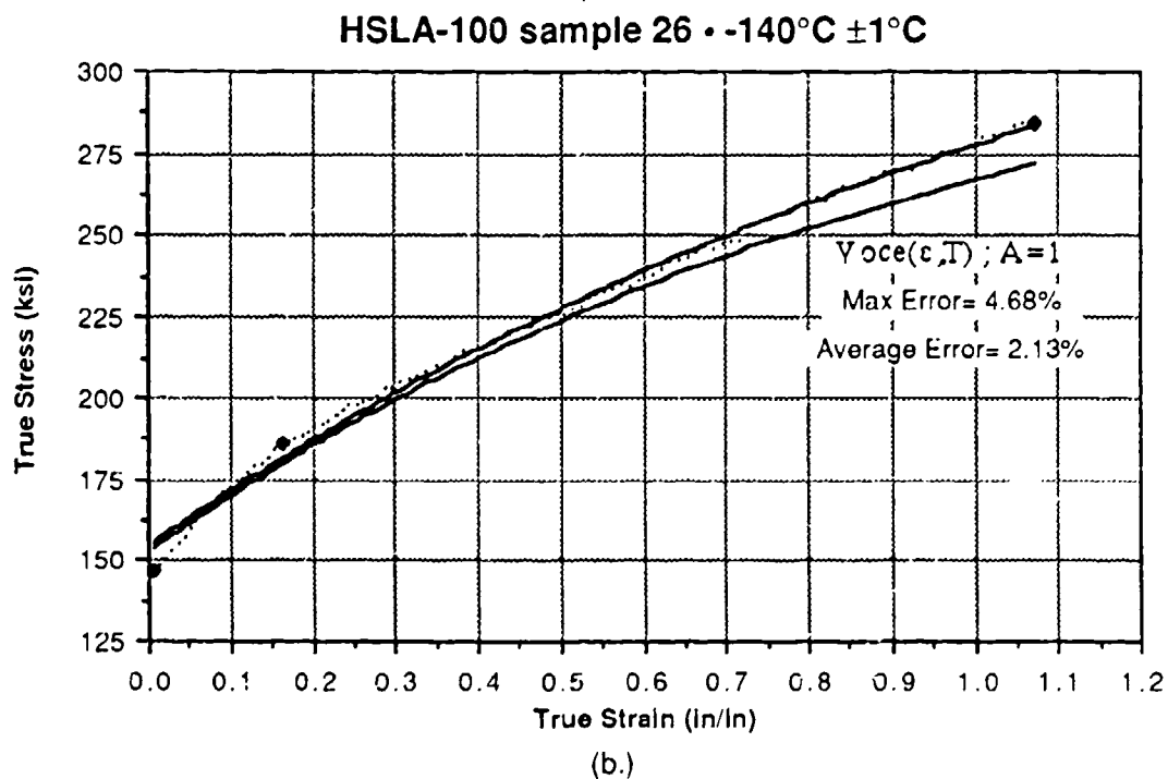
Figure 18 Final Voce( \epsilon, T ) Comparison Plots
