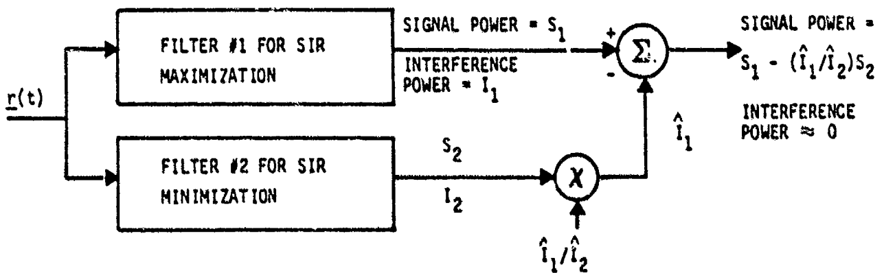
Figure 7-6. An interference canceller using filters for SIR maximization and minimization.
