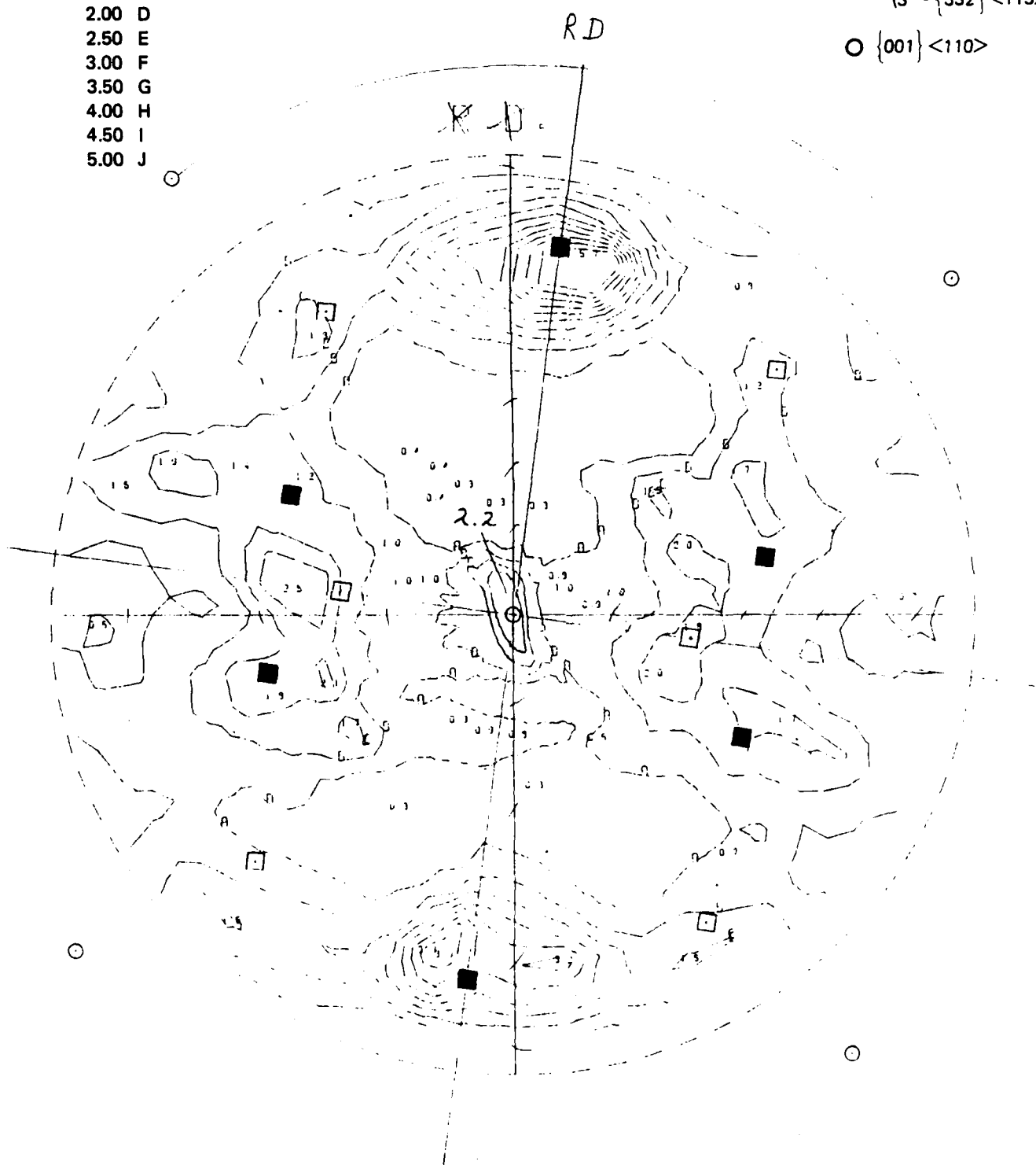
Figure 2b. The (200) pole figure showing texture of the 2-inch-thick plate at the midthickness (1/2 T) section. Dotted circle 80° from center of projection.
