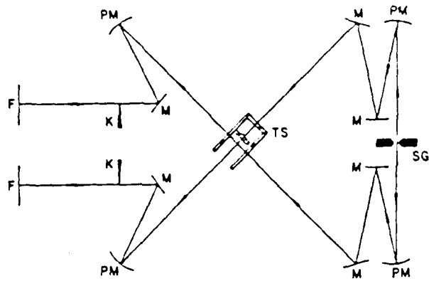
Fig. 3. Two direction schlieren system. SG is the spark gap, M are plane mirrors, PM are parabolic mirrors, TS is the test section, K are knife edges and F are photographic plates.
