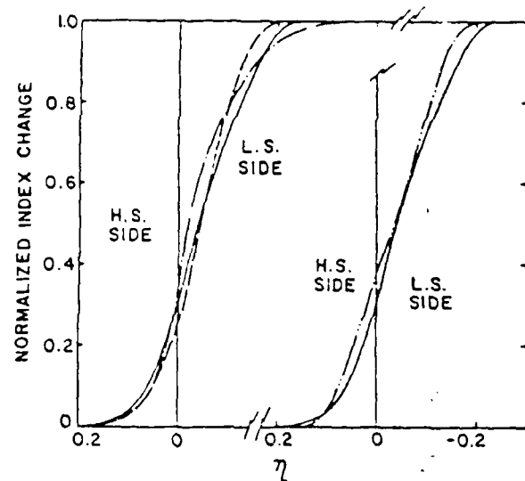
Fig. 6. Nondimensional index profiles. Left hand graph shows our data for various Mach numbers: M=0.1 (solid line), M=0.3 (dash-dot line) and M=0.6 (dashed line). Right hand graph compares our M=0.1 data (solid line) with data from Fiedler 5 (dash-double dot line).
