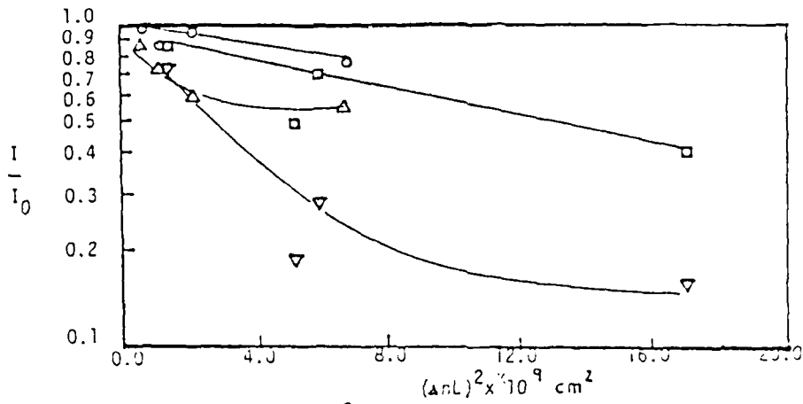
FIGURE 9 Strehl Ratio vs (\Delta n L)^2 . \circ -0.5 cm beam, 1.0 cm downstream, \square -0.5 cm beam, 2.0 cm ds, \Delta -1.0 cm beam, 1.0 cm ds, \nabla -1.0 cm beam, 2.0 cm ds.
