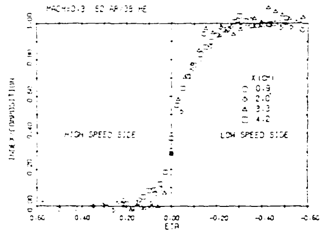
Fig. 5. Nondimensional index profiles of M=0.32 , \lambda_p=1.07 jet. x is the distance downstream of the nozzle exit.
