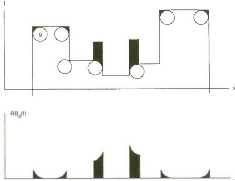
Figure 3.8. Rolling ball transform (1-D).
