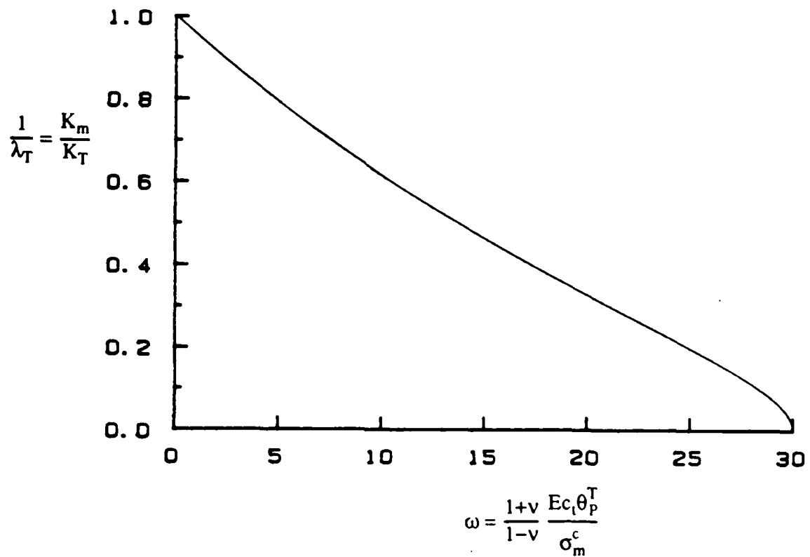
Fig. 4 Transformation toughening: reciprocal of toughening ratio versus toughening parameter, up to "lock-up".
