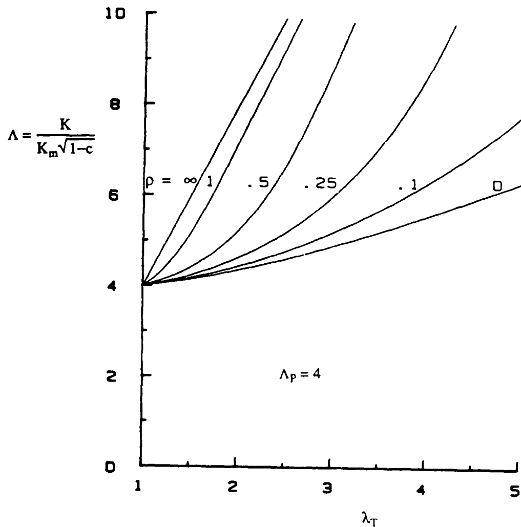
Fig. 10 Modified toughening ratio for various values of coupling parameter \rho = (1+\nu)cS/\sigma_m^c ; \Lambda_p = 4 .
