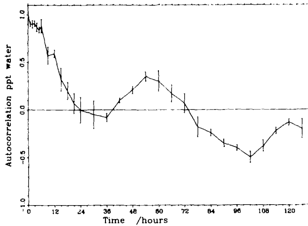
Fig. 12: The autocorrelation function for precipitable water ( w ) measured from ships in the summer/autumn of 1978 during the JASIN experiment. [After Taylor, 1983.]
