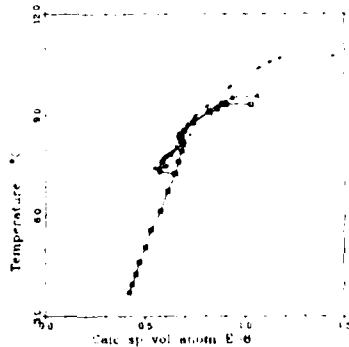
Fig. 7: The dependence of calculated specific volume anomaly on temperature. The data are those used for Figs. 3 and 4. The mean profile ( \square ) extends from the surface to P = 1500 dbar. The seasonal profiles, from the surface to P = 250 dbar, are denoted as follows: spring (May-Jul), \Delta ; summer (Aug-Oct), + ; autumn (Nov-Jan), \times ; winter (Feb-Apr), \diamond . The symbols show the positions of the standard depth levels used by Levitus: 0, 10, 20, 30, 40, 50, 75, 100, 125, 150, 200, 250, 300, 400, 500, 600, 700, 800, 900, 1000, 1100, 1200, 1300, 1400, and 1500 m.
