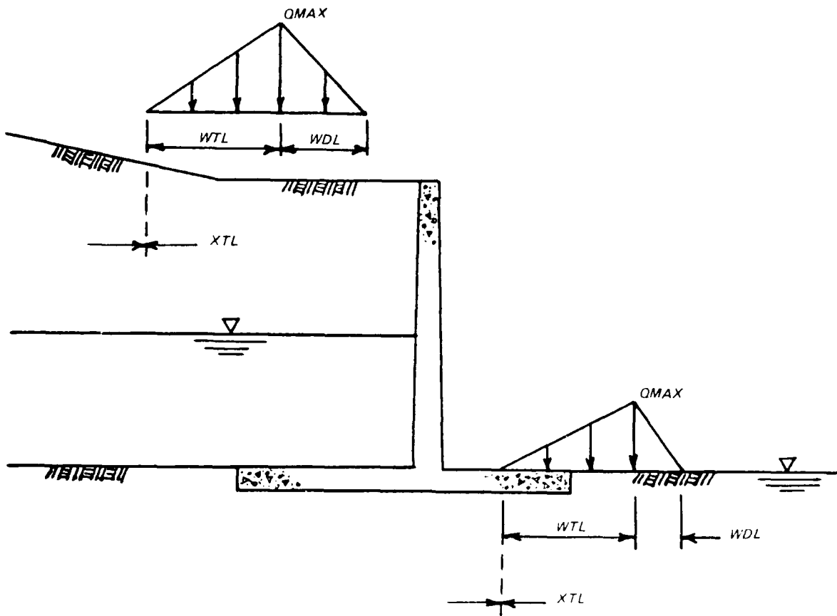
Figure 32. Triangular loads
