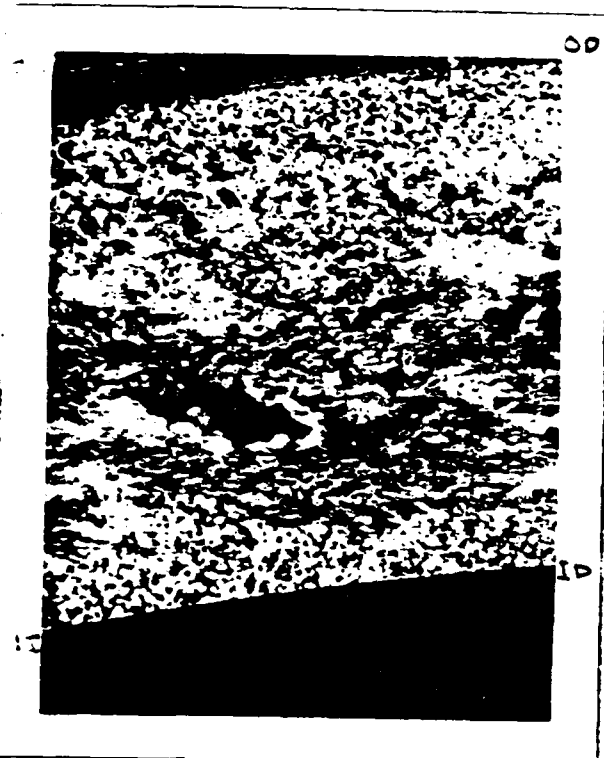
Rib No. 84-77 Damaged at 24000 rpm(1.6 million DN) (25X Magnification)
