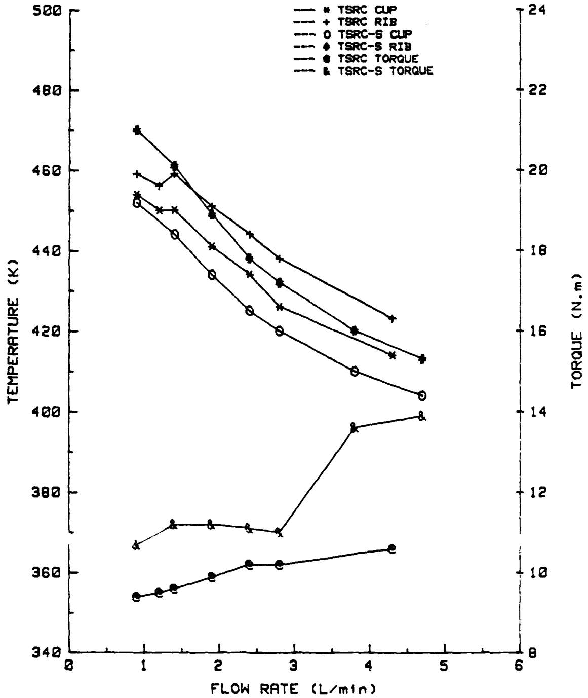
Figure 17 - TEMPERATURE and TORQUE vs FLOW RATE at 24000 RPM CBS1000M 75% and CBS 600 RIBBED CUP
