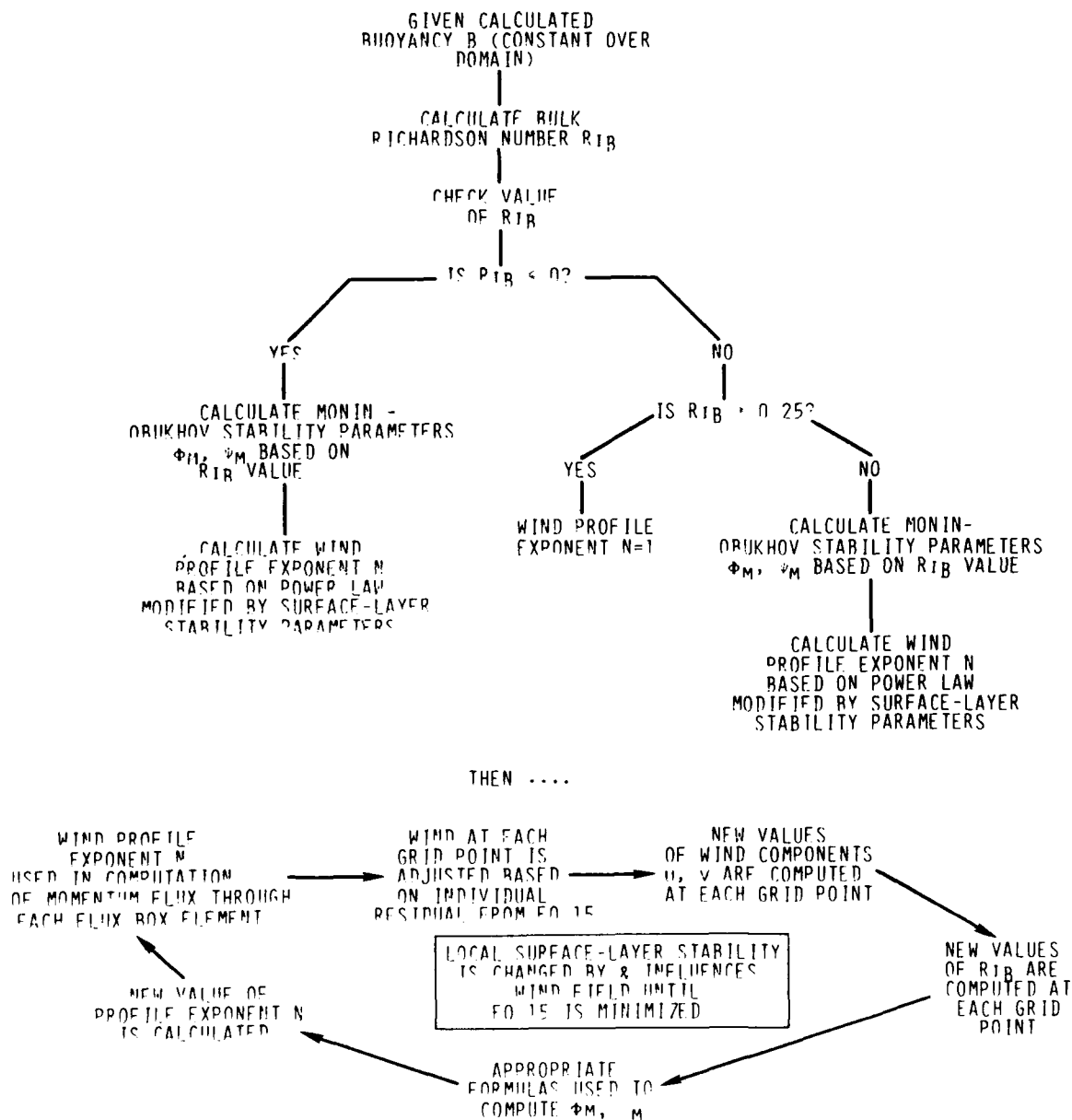
Figure 6. Flowchart Describing Calculation of Wind Profile Exponent n Based on Values of Buoyancy and Windspeed. Top flowchart shows calculation at individual grid point. Bottom flowchart shows how exponent calculation leads to changes in momentum flux, and changes in flux feedback to alter subsequent computations of n .
