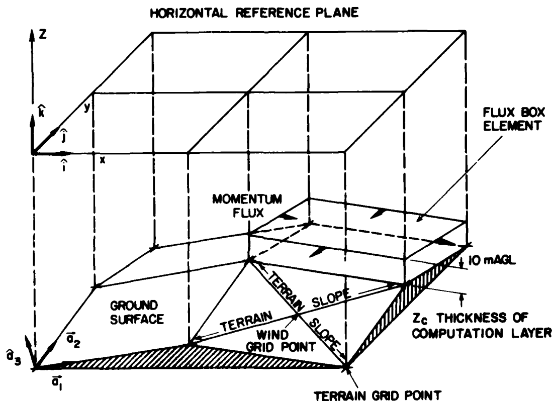
Figure 2. Diagram Showing Grid Structure and Geometry of Model Domain, With Structure of Individual Flux Box. Notice that the staggered grid system allows terrain slopes centered on the wind grid points to be integrated into model calculations, through the terrain-following coordinate axes a_1 and a_2 (after Ball and Johnson 8 )
