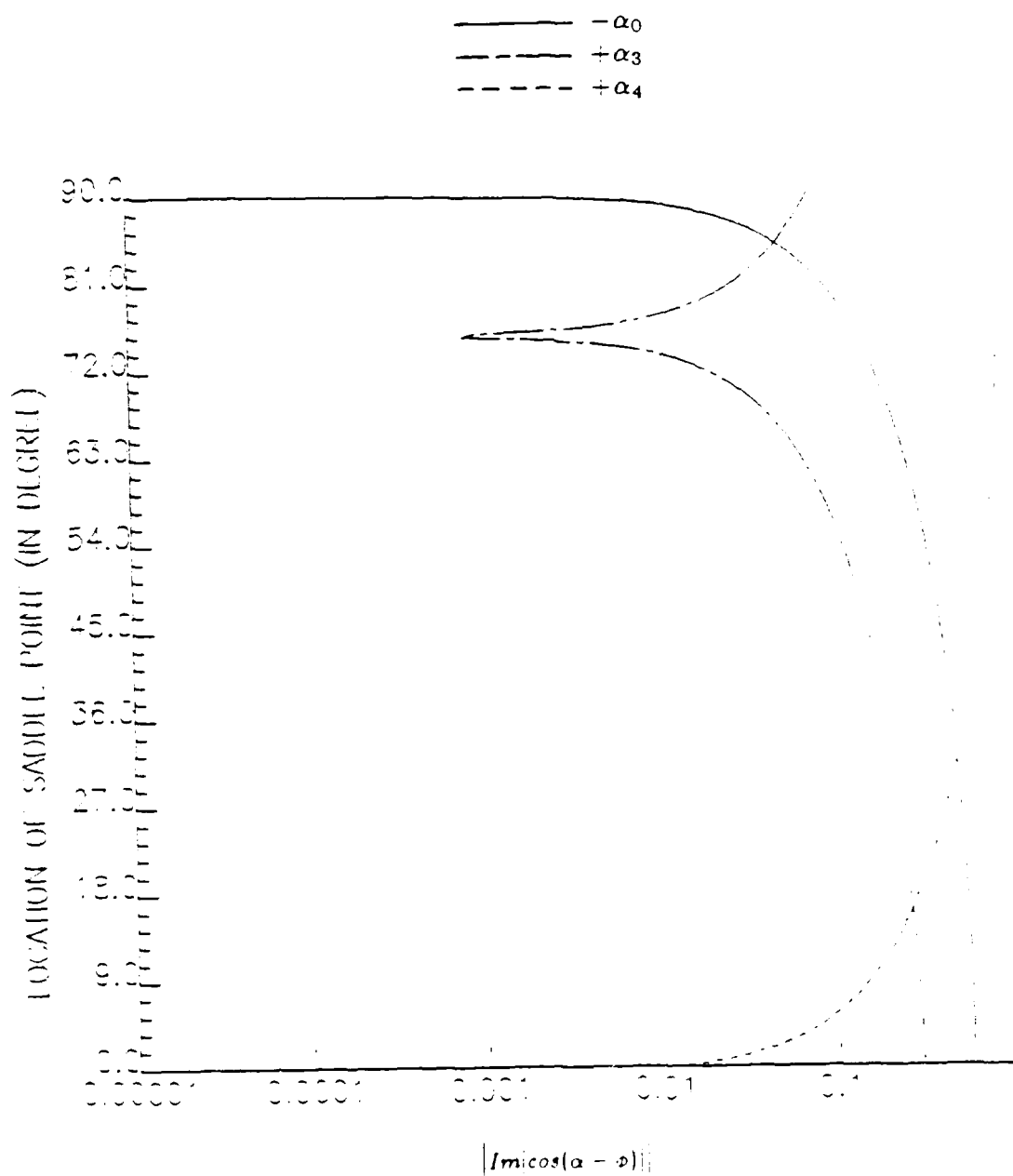
Figure 10 Absolute values of Im[\cos(\alpha - \phi)] , \Omega = 1.0 .
