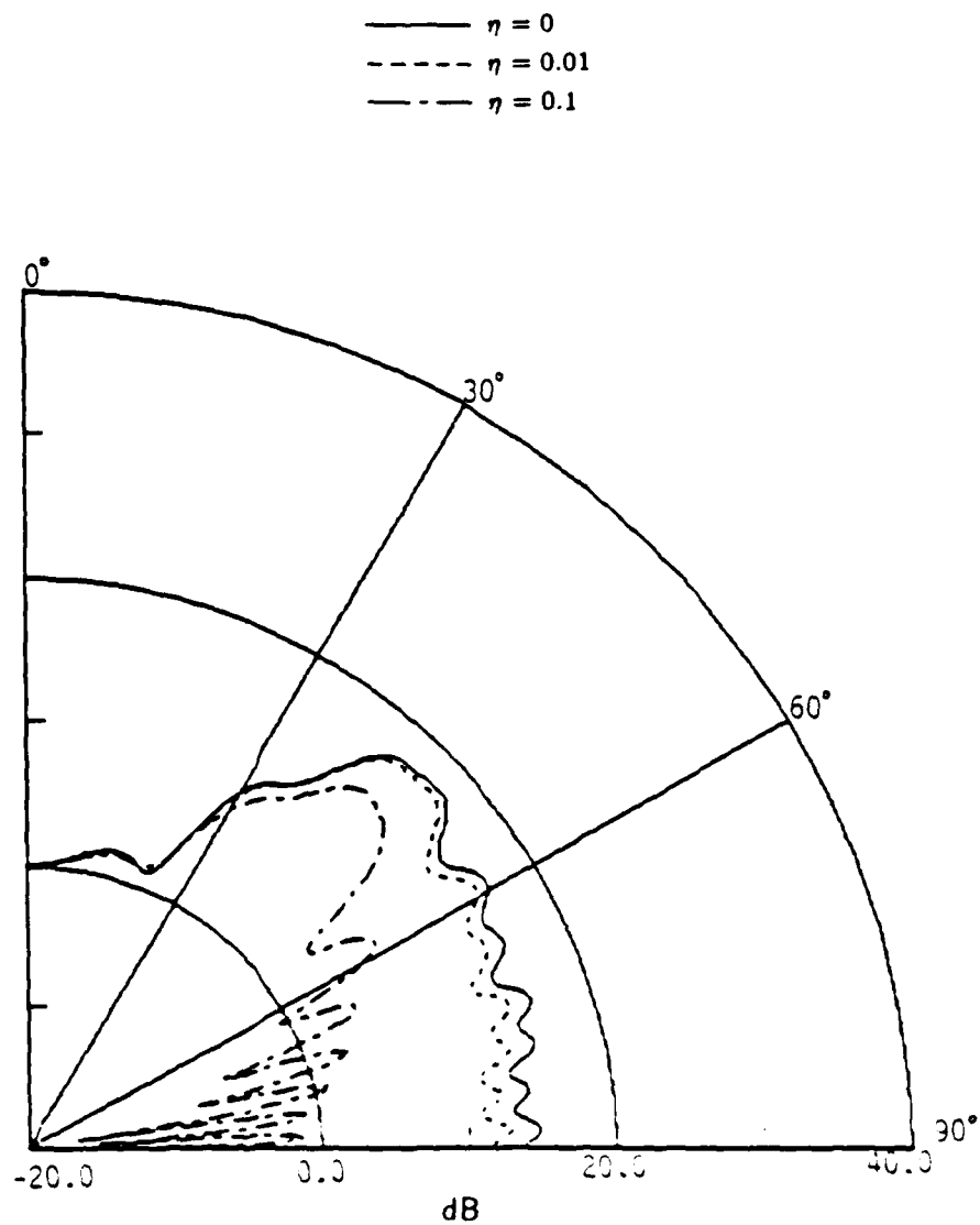
Figure 42 Normalized directivity function for a line-excited plate with structural damping. k_0 r = 10^2 . \Omega = 10.0 .
