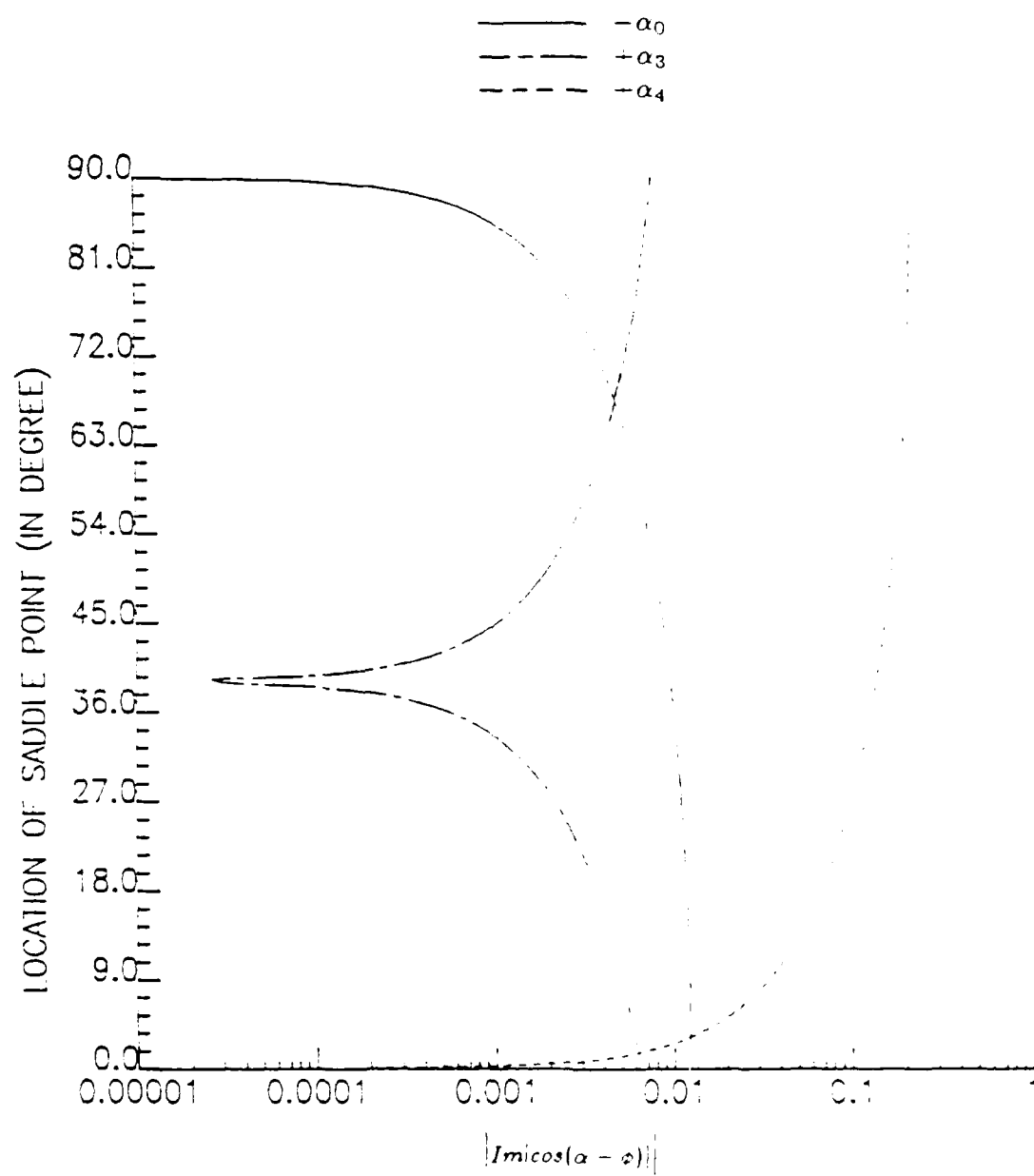
Figure 11 Absolute values of Im[\cos(\alpha - \phi)] , \Omega = 5.0 .
