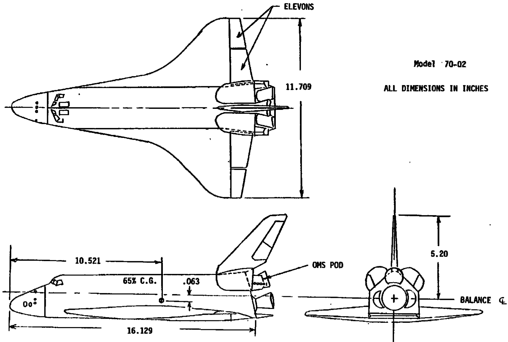
Figure 2. Shuttle Orbiter 1.25% Scale Model
