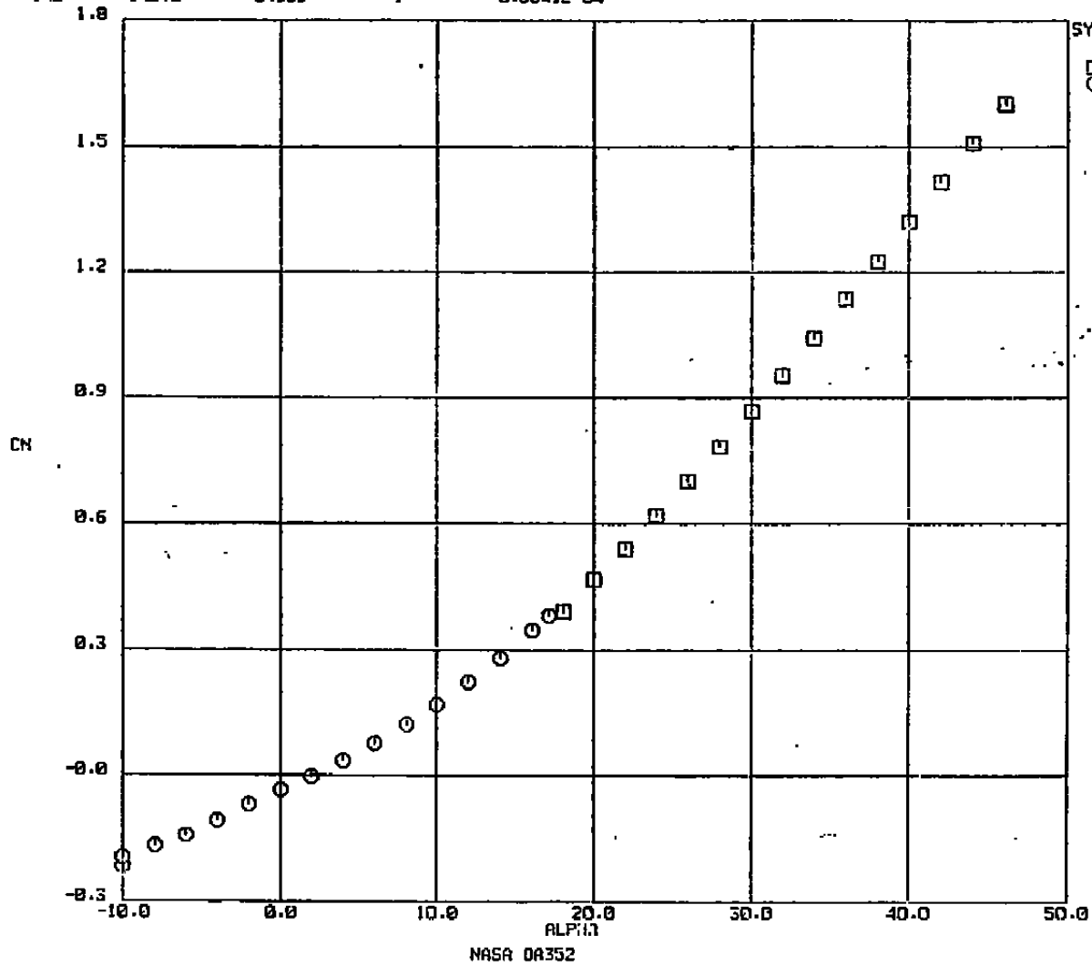
Sample 3. Plotted Force and Moment Data
