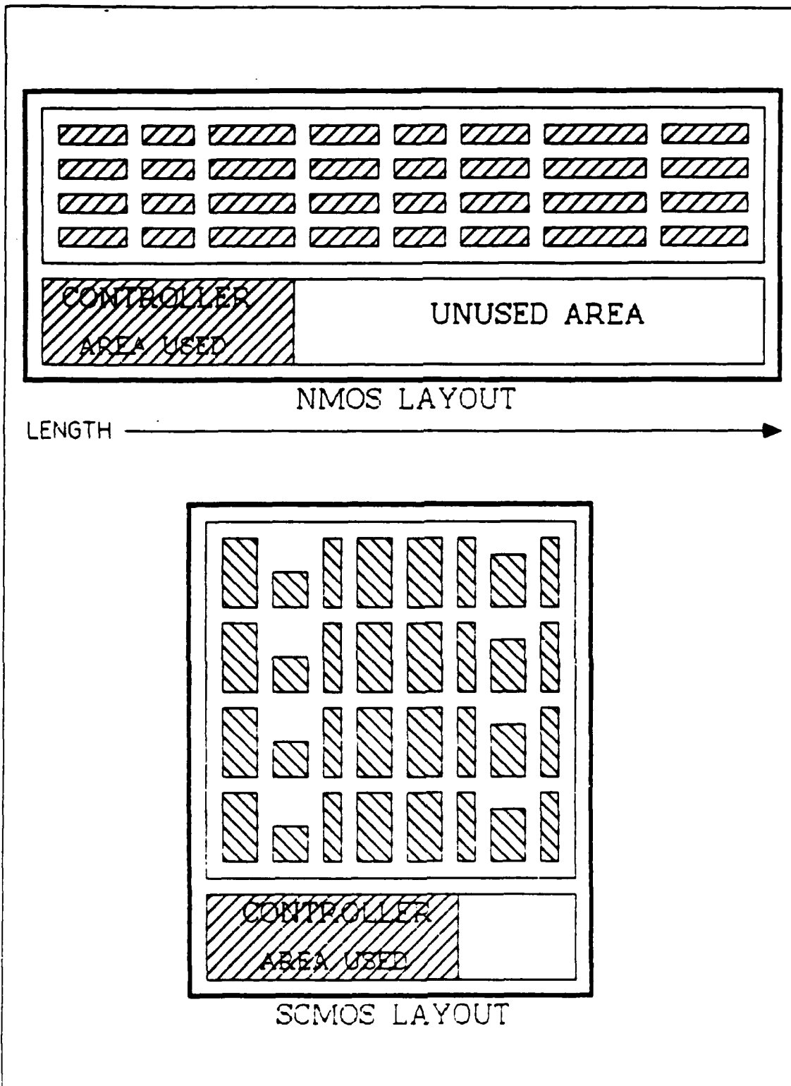
Figure 2.5 Data-path Dimensions.
