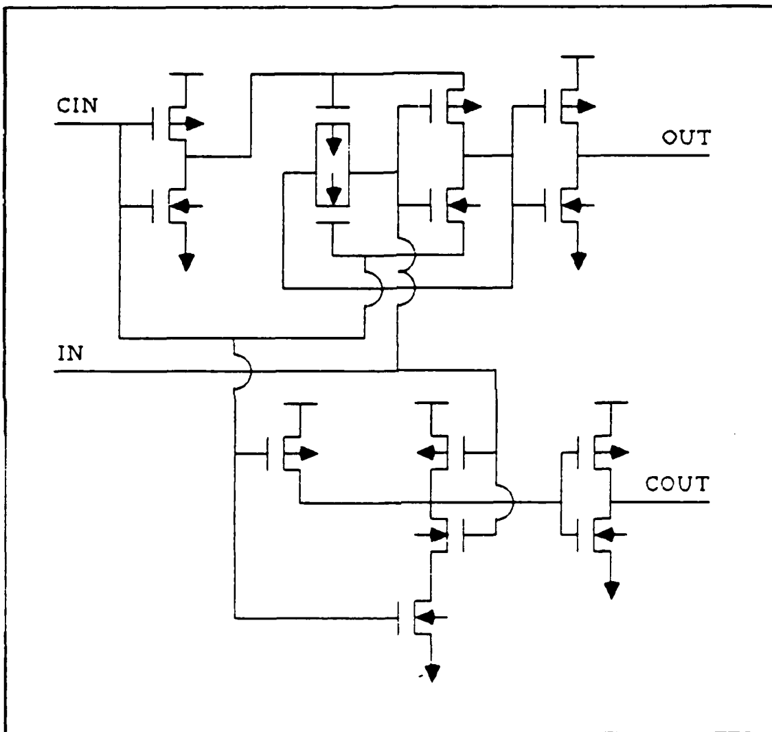
Figure 2.4 Transistor Schematic (Incrementor).
