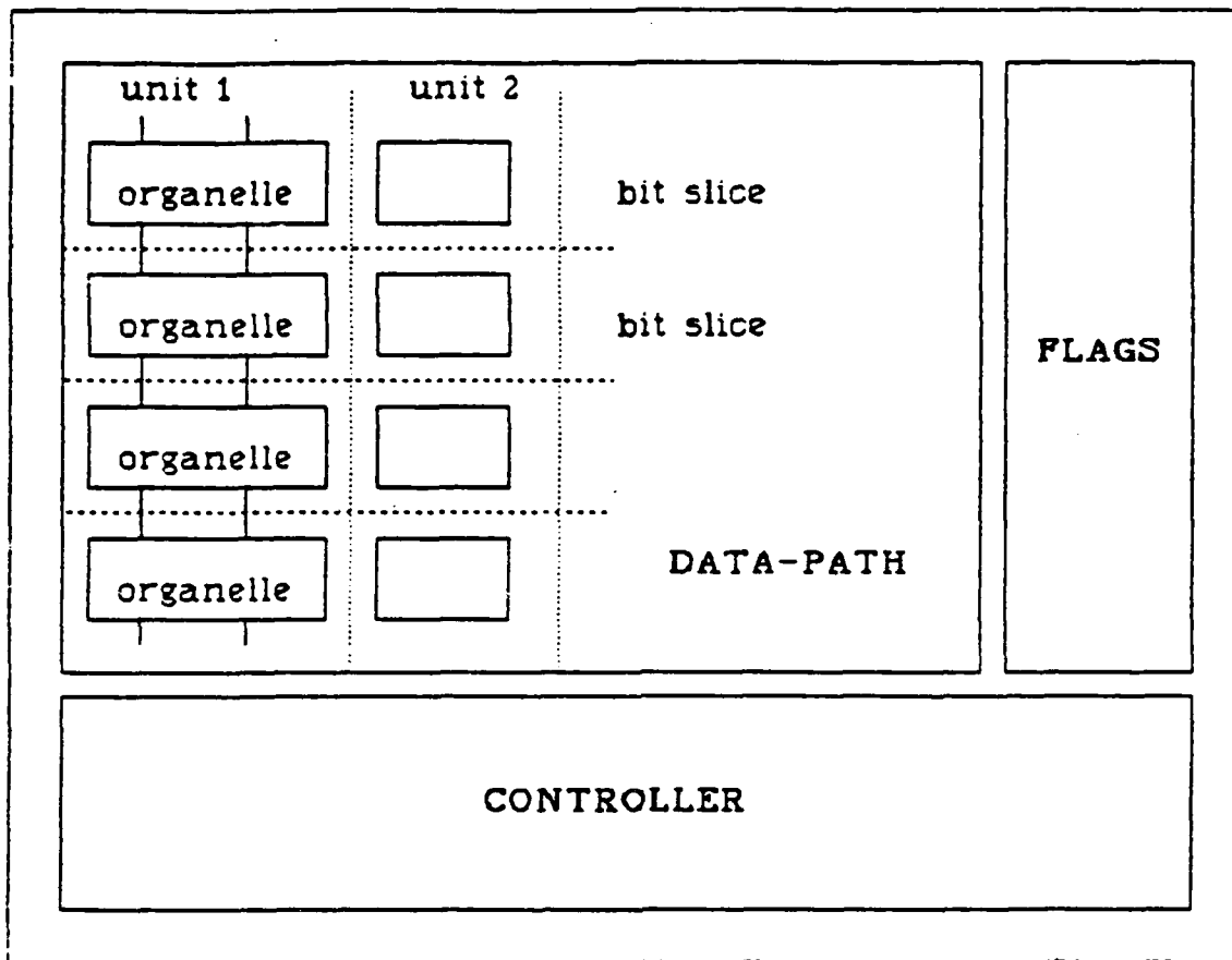
Figure 2.1 MacPitts Internal Layout.
