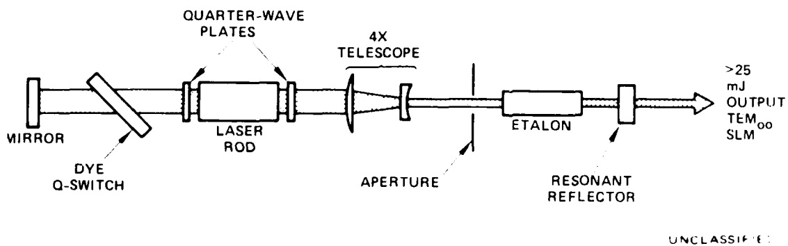
Figure 40. Single-longitudinal, single-transverse mode oscillator.
