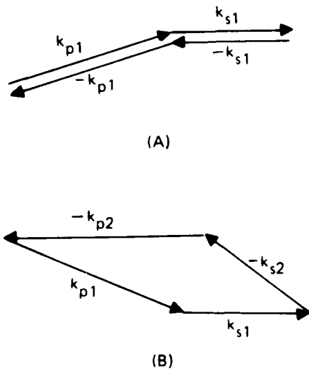
Figure 4. Four-wave mixing with multi-transverse mode pump and Stokes waves.
