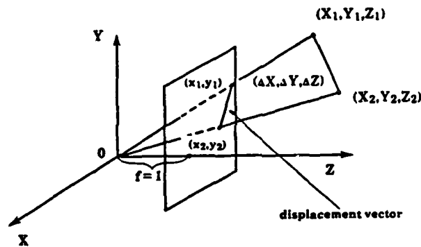
Figure 5.7: Motion of a point
