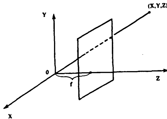
Figure 5.1: Perspective projection
