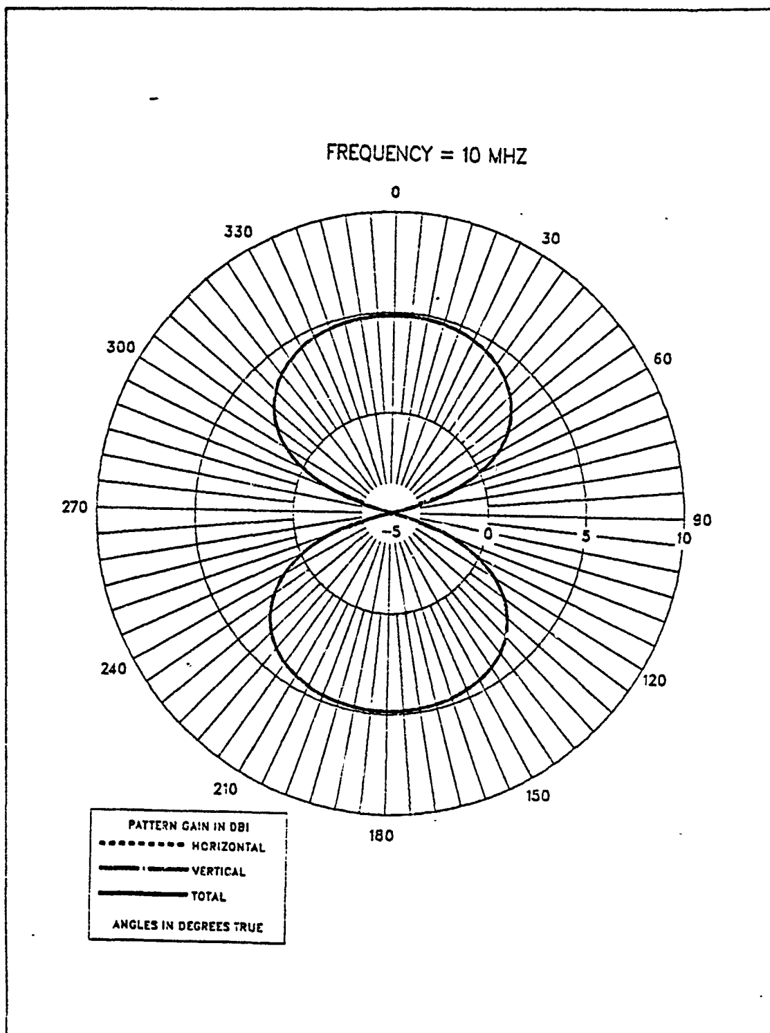
Figure 2.25 E-Field Azimuth Pattern at 10 MHz for TF-TLA.
