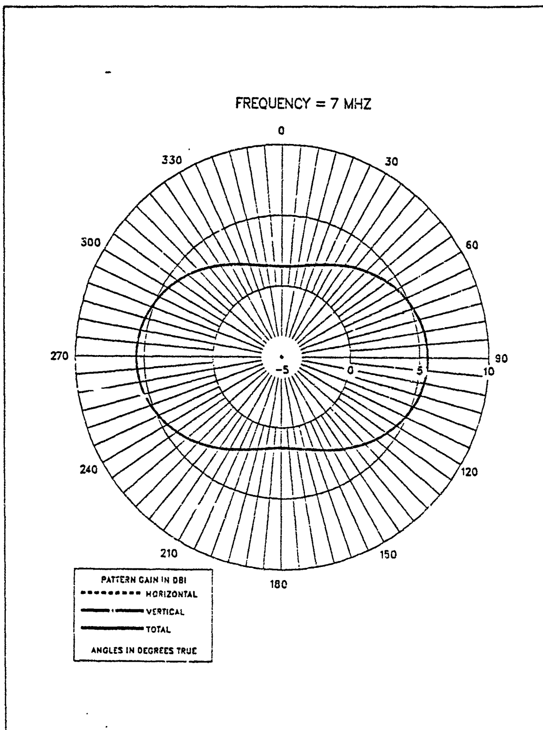
Figure 2.17 E-Field Azimuth Pattern at 7 MHz for EF-TLA.
