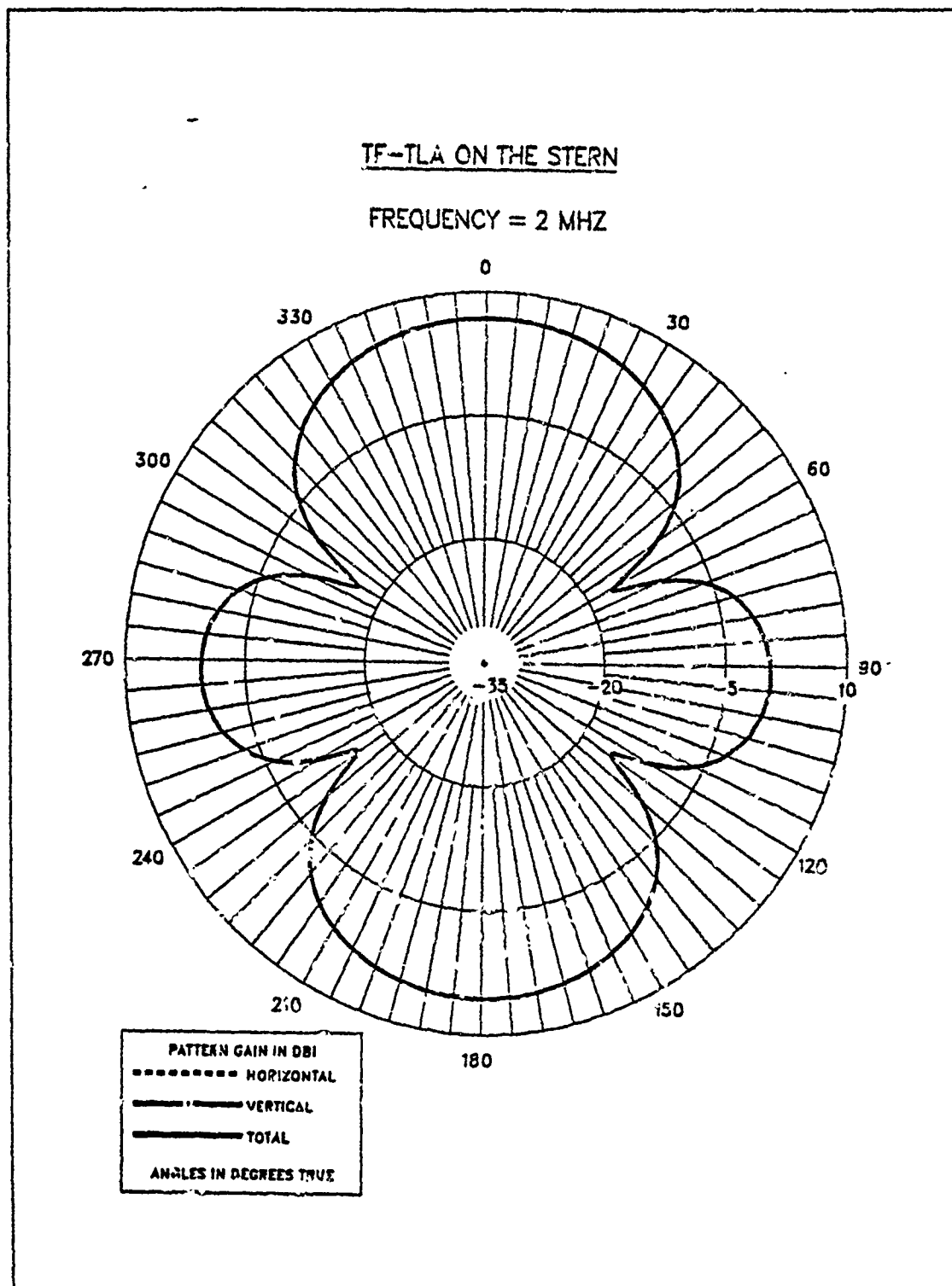
Figure E.19 E-Field Azimuth Pattern at 2.0 MHz for TF-TLA on the Stern.
