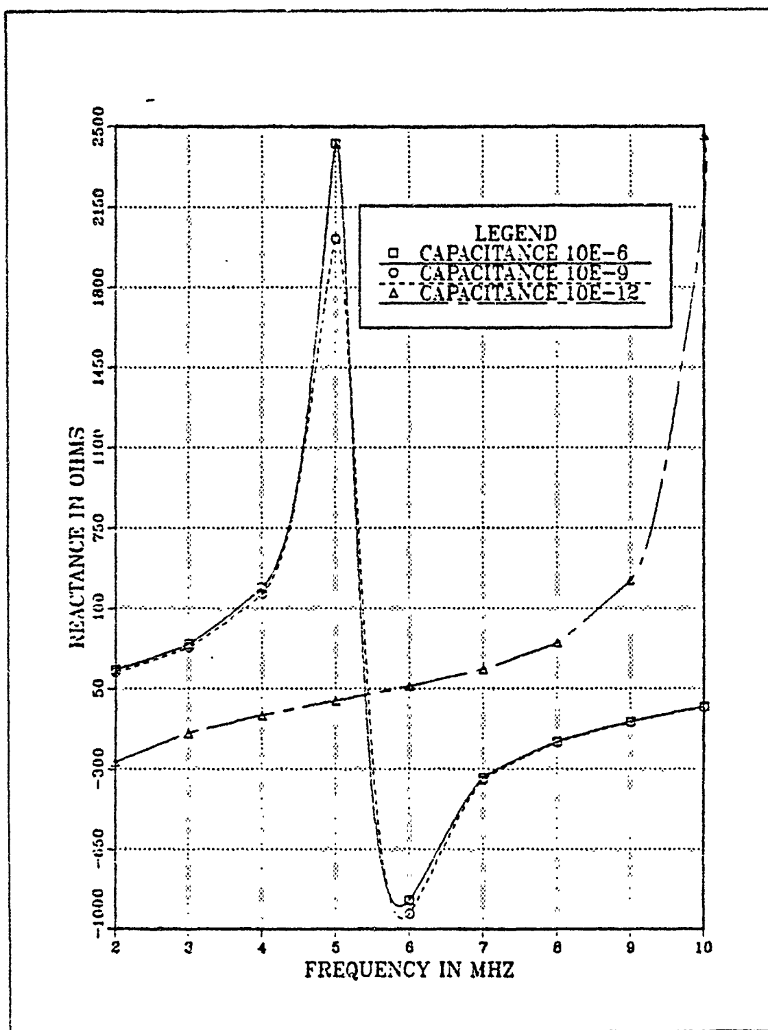
Figure 2.9 Reactance vs Frequency for EF-TLA with Three Different Capacitive Loads.
