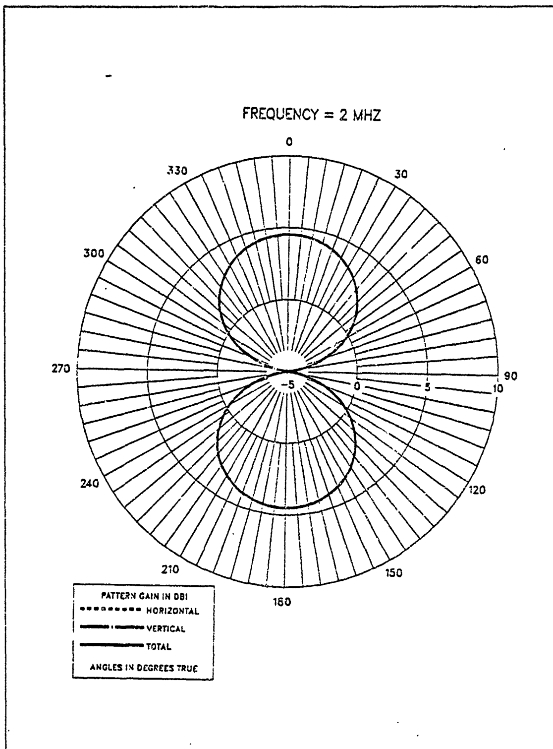
Figure 2.13 E-Field Azimuth Pattern at 2 MHz for EF-TLA.
