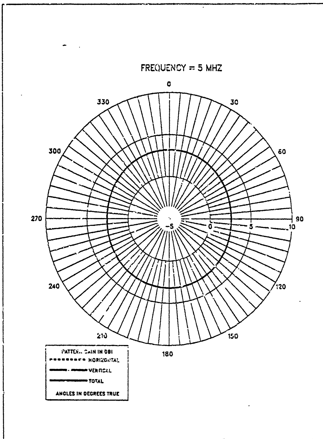
Figure D.3 E-Field Azimuth Pattern at 5 MHz for CEF-TLA.
