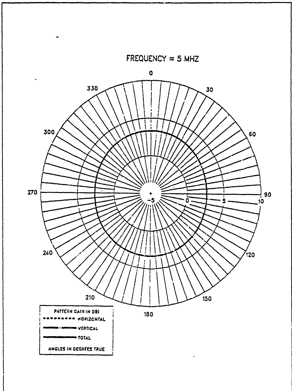
Figure 2.15 E-Field Azimuth Pattern at 5 MHz for EF-TLA.
