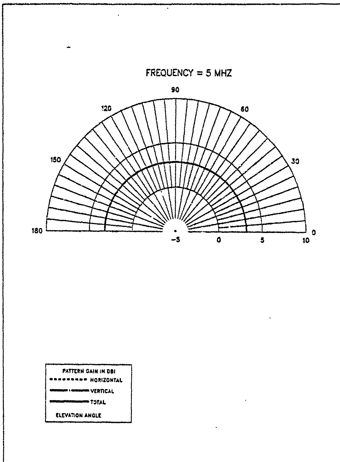
Figure D.4 E-Field Elevation Pattern at 5 MHz for CEF-7LA.
