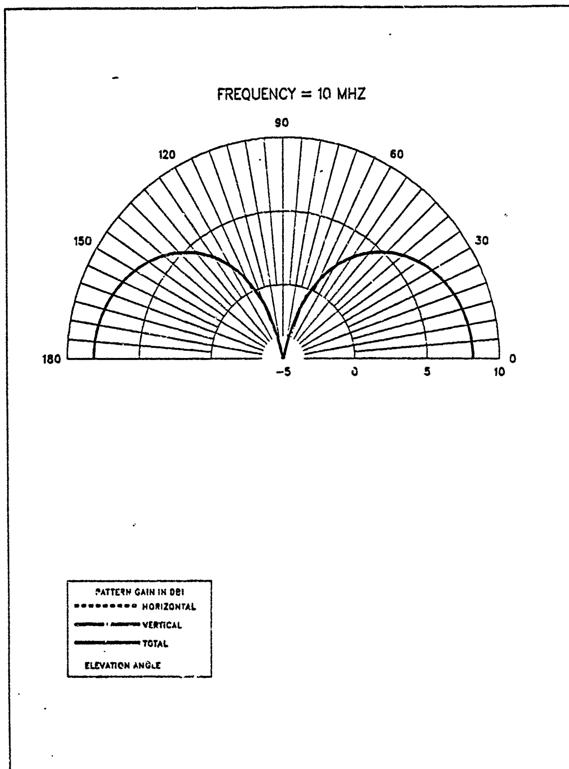
Figure D.8 E-Field Elevation Pattern at 10 MHz for CEF-TLA.
