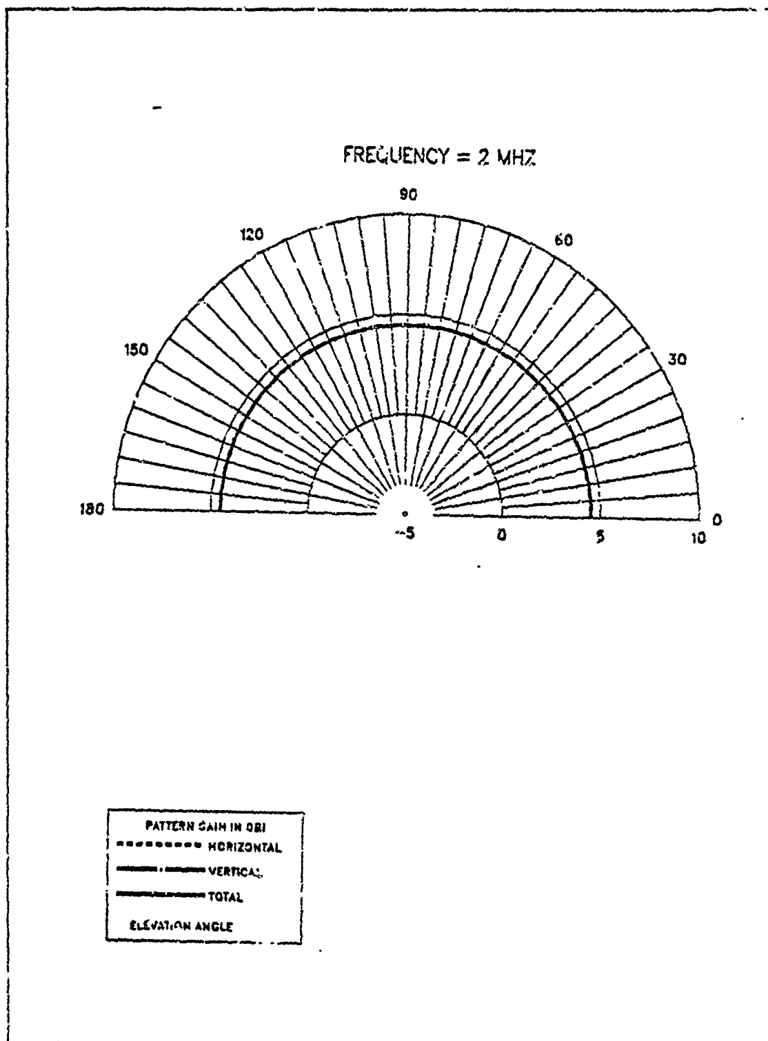
Figure D.2 E-Field Elevation Pattern at 2 MHz for CEF-1 LA.
