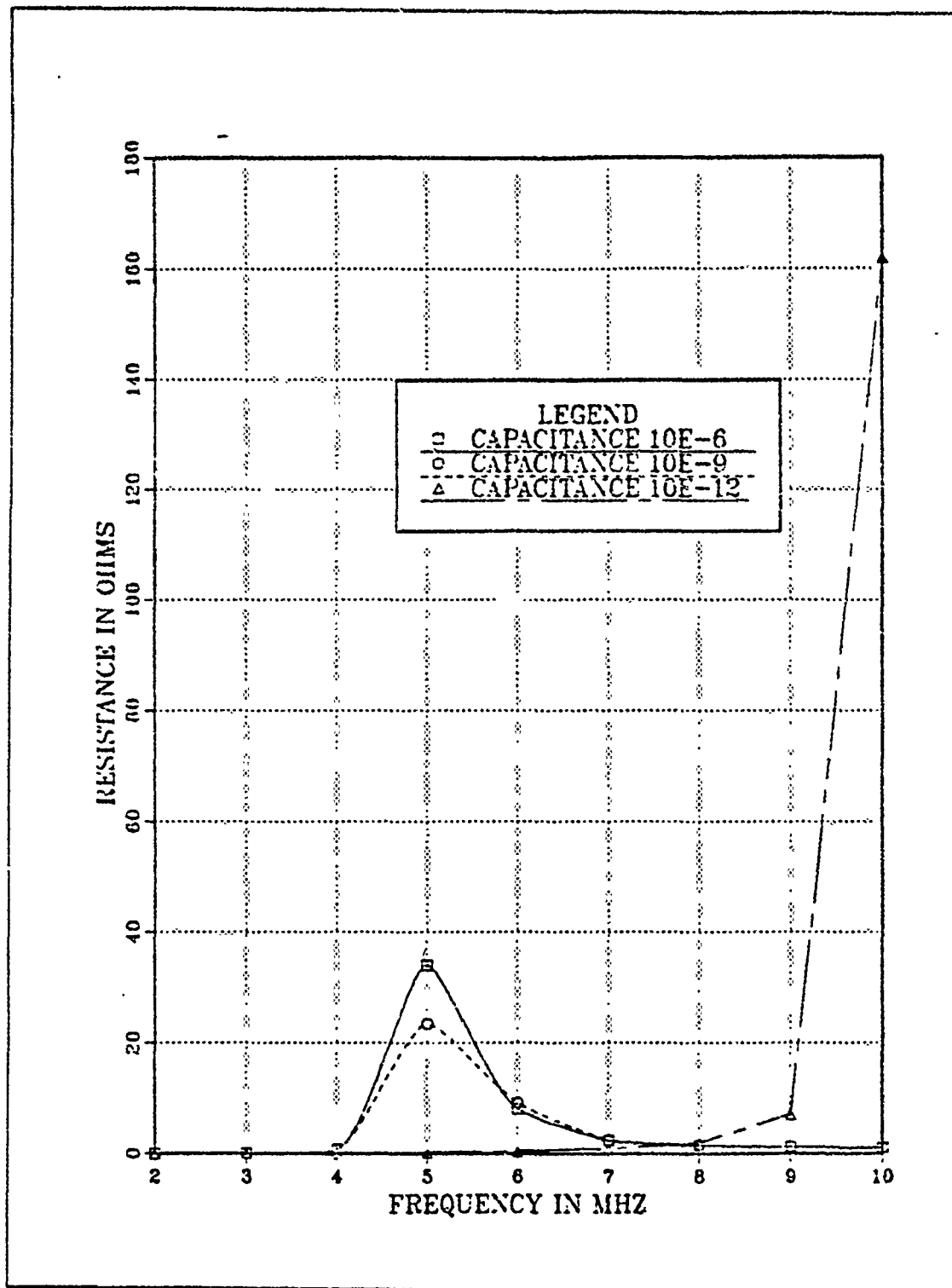
Figure 2.8 Resistance vs Frequency for EF-TLA with Three Different Capacitive Loads.
