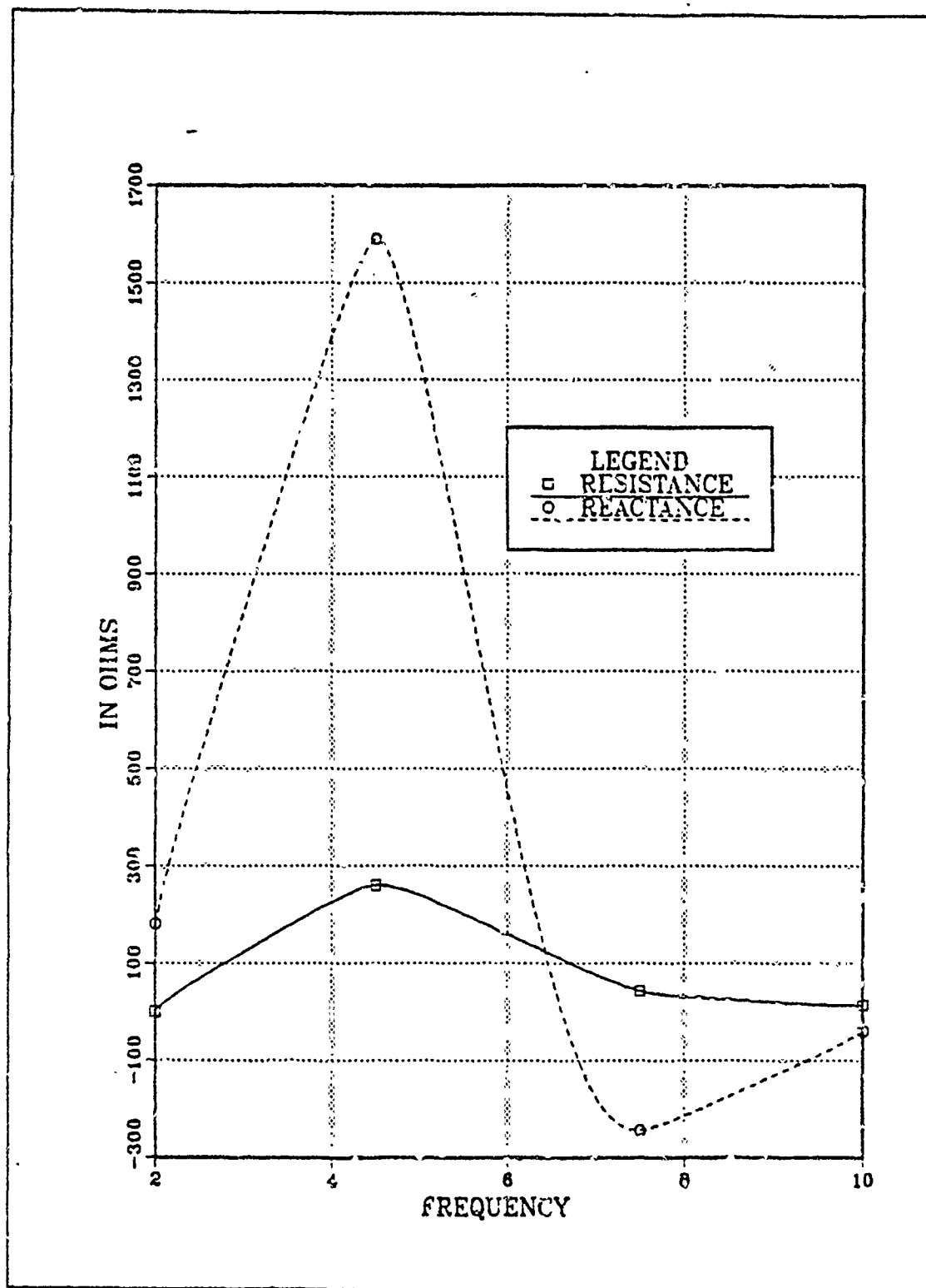
Figure 3.7 Input Impedance vs Frequency for EF-TLA on the Stern.
