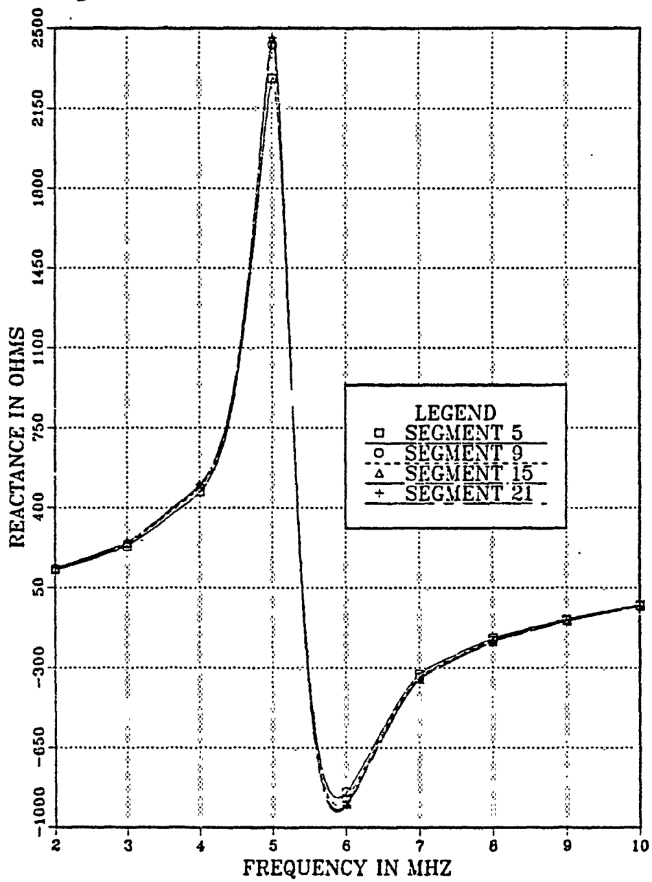
Figure 2.5 Reactance vs Frequency for EF-TLA with Four Different Segmentations.
