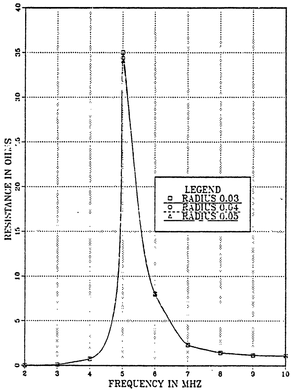
Figure 2.2 Resistance vs Frequency for a 9 Segment EF-TLA with Three Different Wire Radii.
