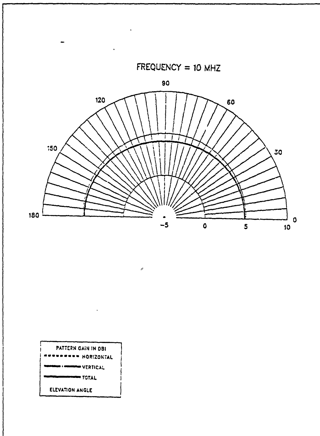
Figure 2.26 E-Field Elevation Pattern at 10 MHz for TF-TLA.
