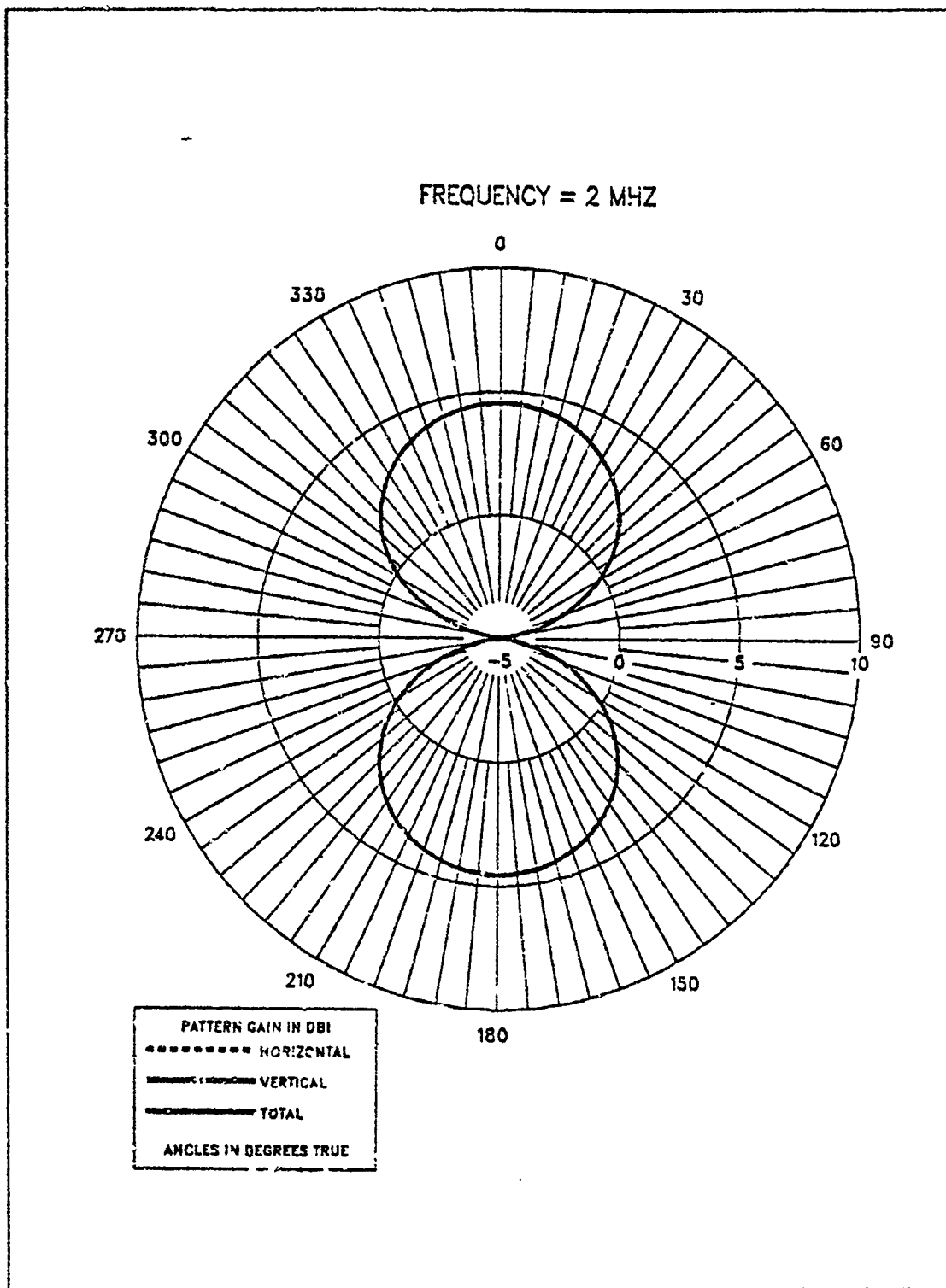
Figure D.1 E-Field Azimuth Pattern at 2 MHz for CEF-TLA.
