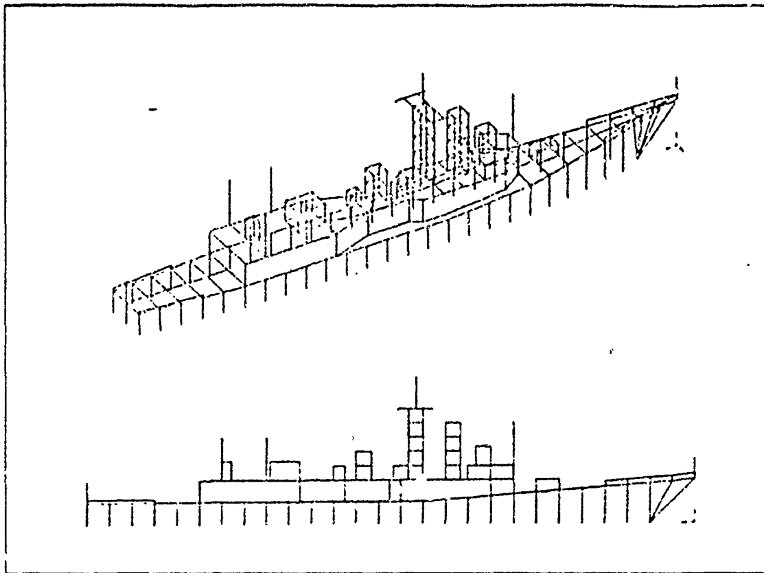
Figure 3.4 Wire Grid Model of an FFG-45 Frigate with Antenna on the Stern.
