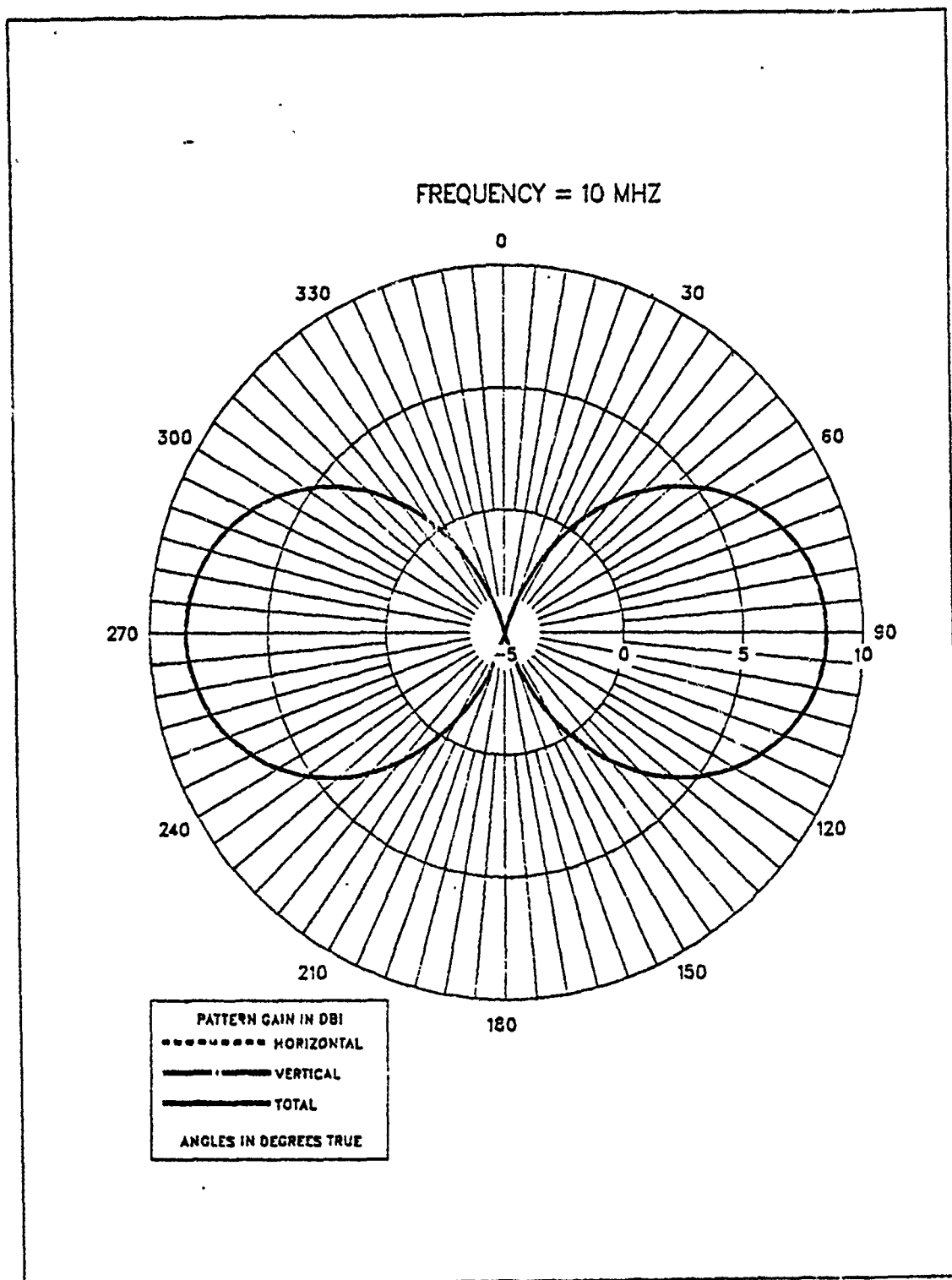
Figure D.7 E-Field Azimuth Pattern at 10 MHz for CEF-1LA.
