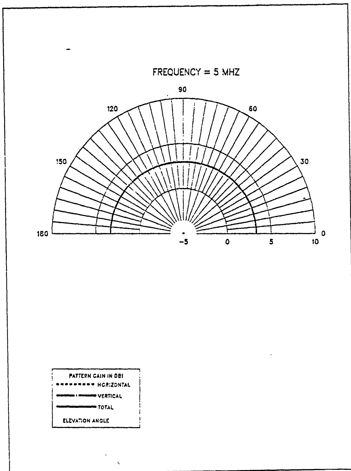
Figure 2.16 E-Field Elevation Pattern at 5 MHz for EF-TLA.
