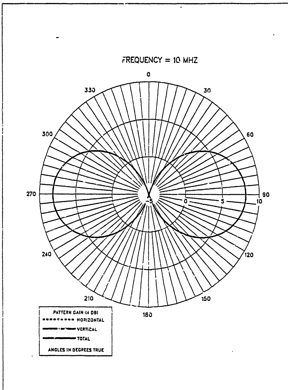
Figure 2.19 E-Field Azimuth Pattern at 10 MHz for EF-TLA.
