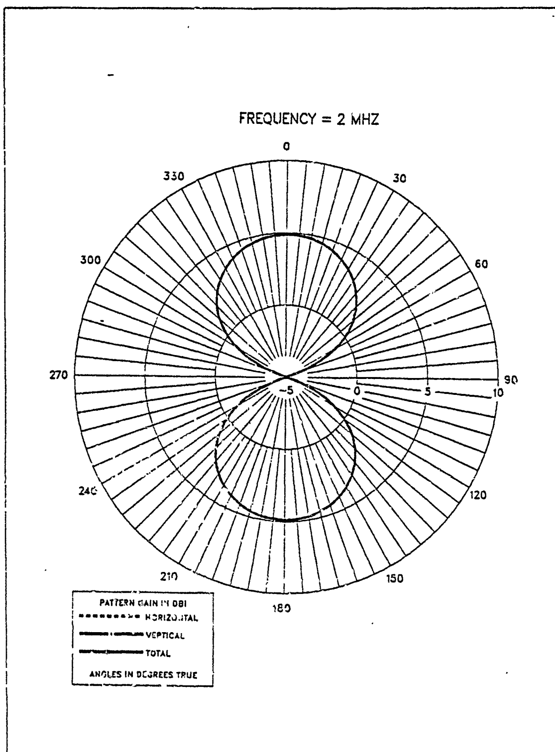
Figure 2.21 E-Field Azimuth Pattern at 2 MHz for TF-1LA.
