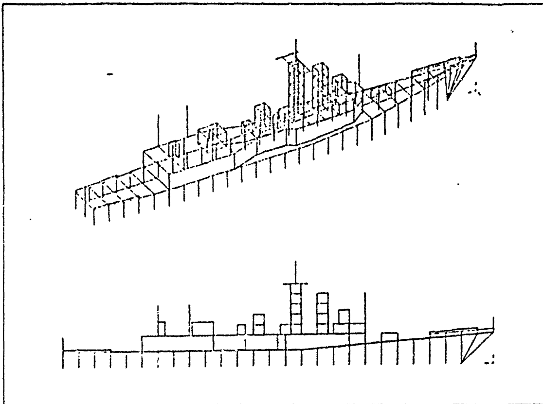
Figure 3.5 Wire Grid Model of an FFG-45 Frigate with Antenna on the Bow and the Stern.
