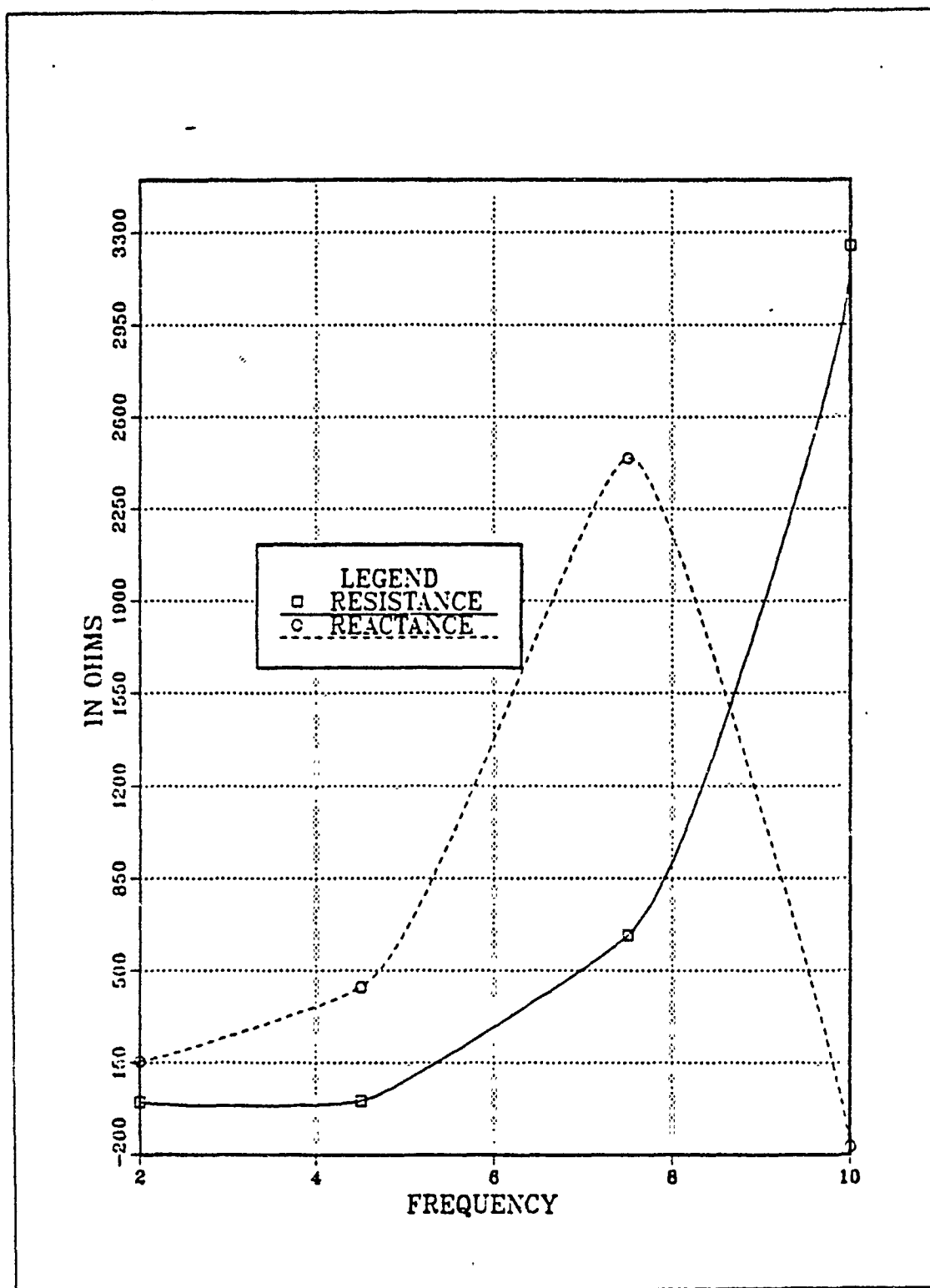
Figure 3.10 Input Impedance vs Frequency for TF-TLA on the Stern.
