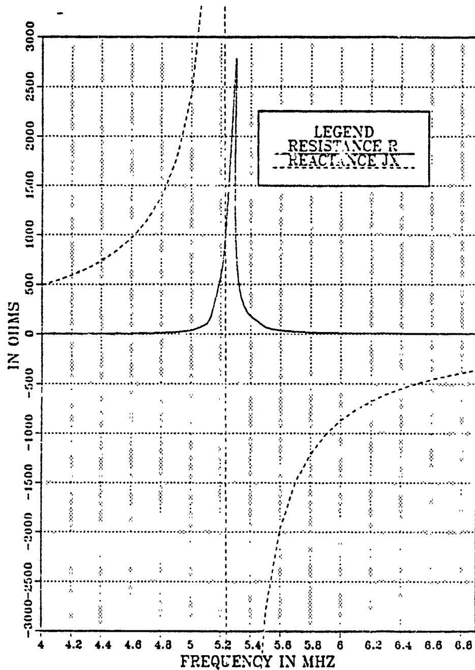
Figure 2.12 Impedance Plot of EF-TLA from 4.0 - 6.9 MHz with 9 Segments and a 0.05 Meter Radius.
