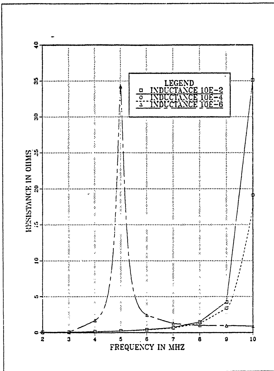
Figure 2.10 Resistance vs Frequency for EF-TLA with Three Different Inductive Loads.
