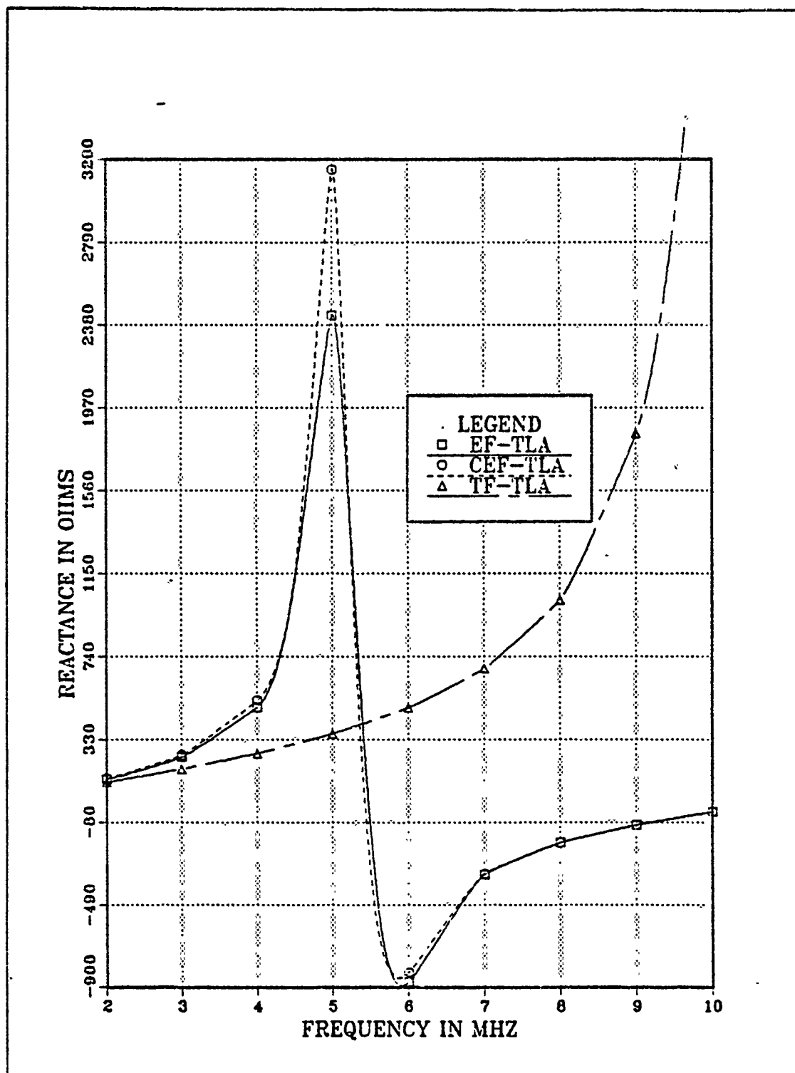
Figure 2.7 Reactance vs Frequency for TLA with Three Different Feed Points.
