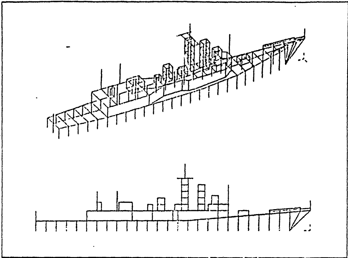
Figure 3.3 Wire Grid Model of an FFG-45 Frigate with Antenna on the Bow.
