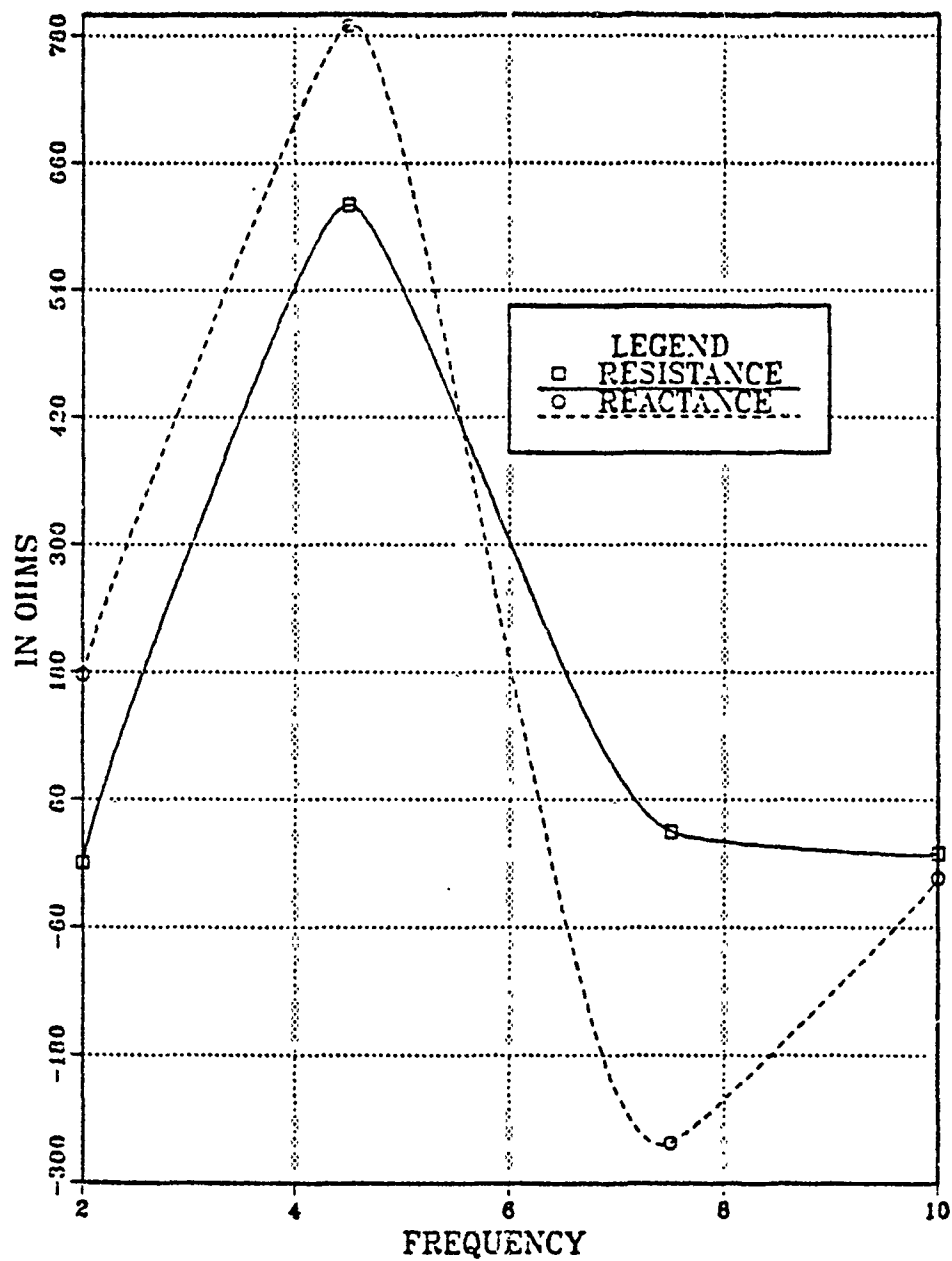
Figure 3.6 Input Impedance vs Frequency for EF-TLA on the Bow.
