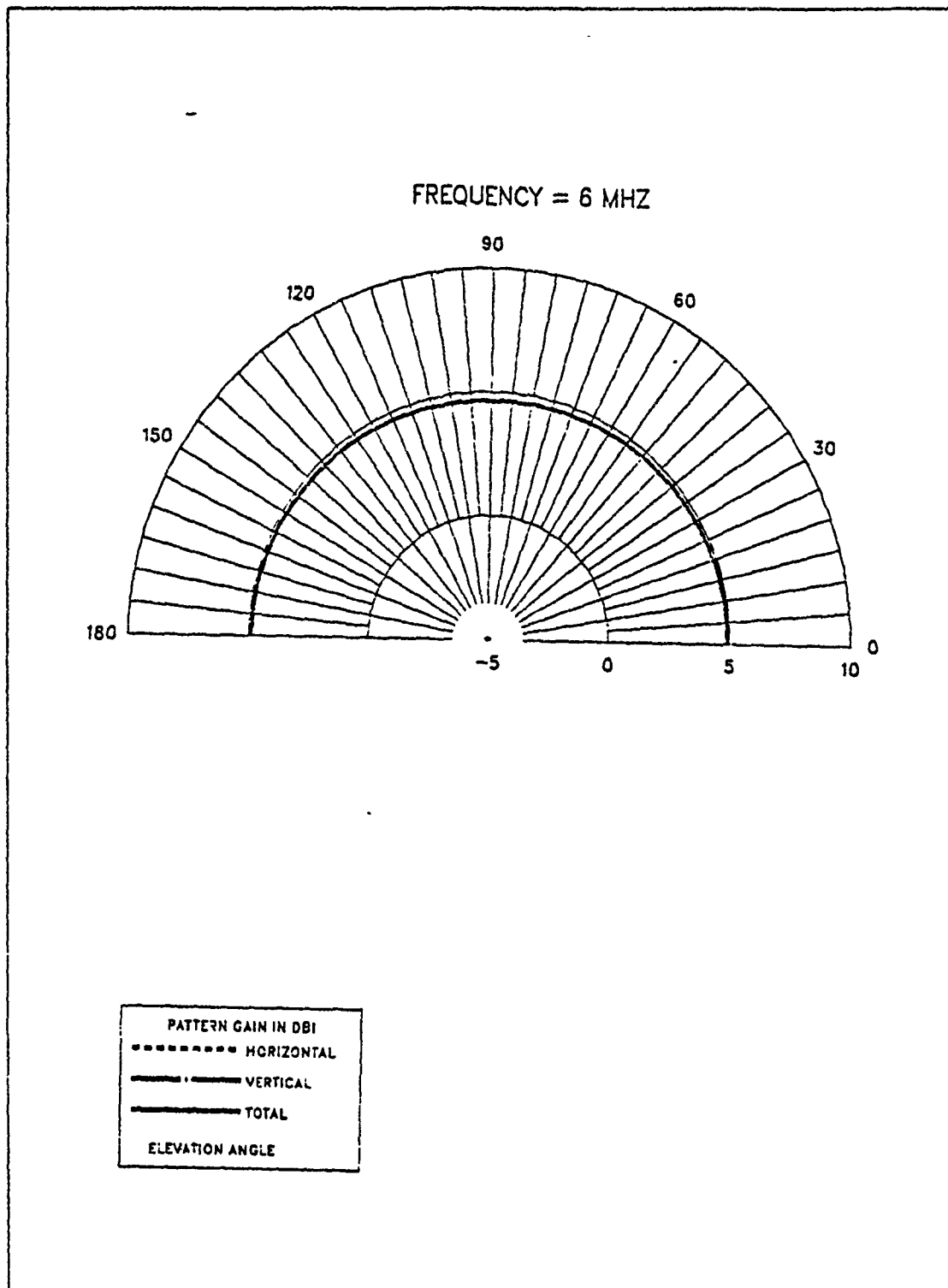
Figure 2.24 E-Field Elevation Pattern at 6 MHz for TF-TLA.
