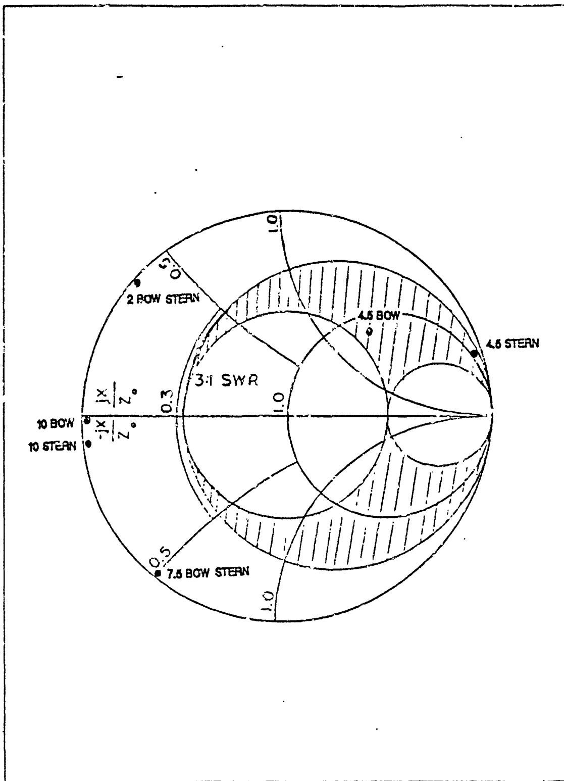
Figure 3.14 Smith Chart Showing 3:1 VSWR Impedance Plot of EF-TLA : Z_0 = 500 \text{ Ohm}
