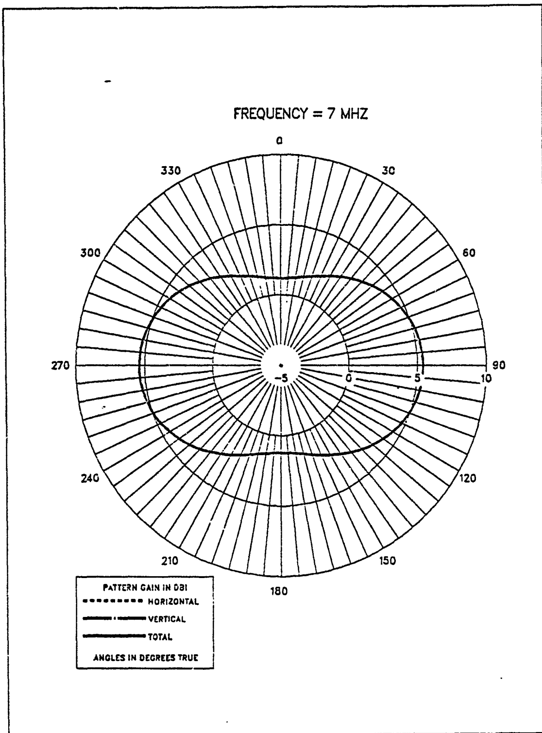
Figure D.5 E-Field Azimuth Pattern at 7 MHz for CEF-TLA.
