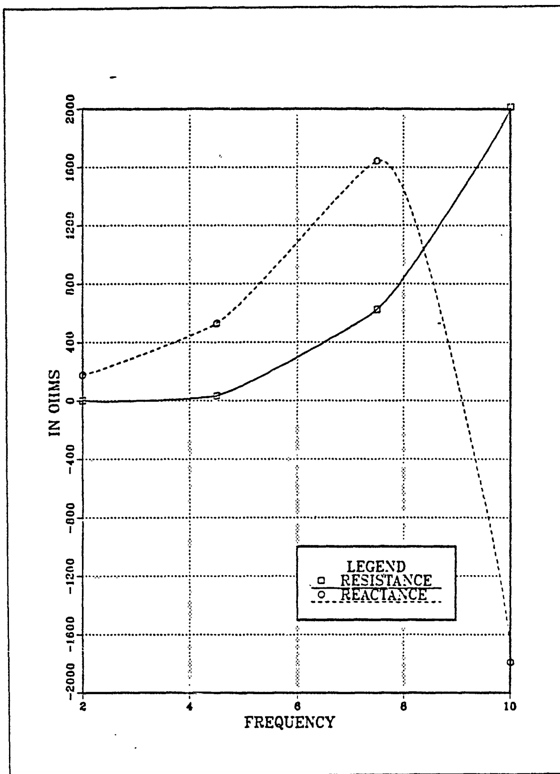
Figure 3.9 Input Impedance vs Frequency for TF-TLA on the Bow.
