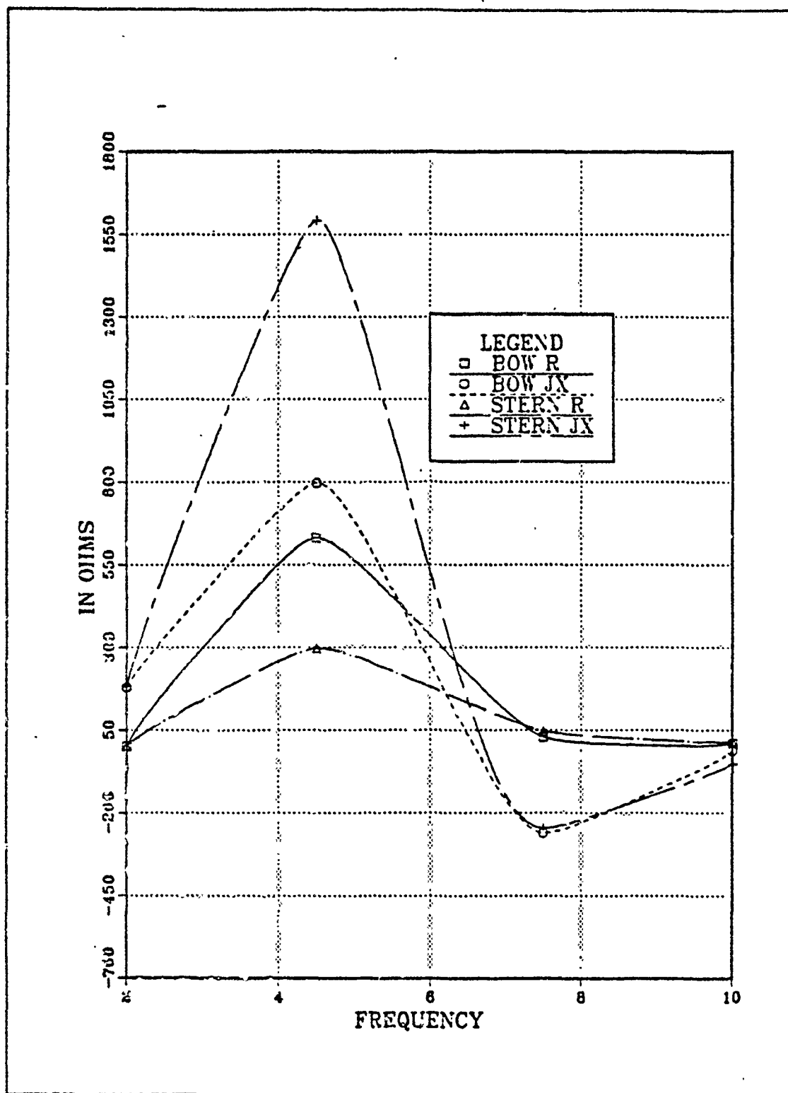
Figure 3.8 Input Impedance vs Frequency for EF-TLA on the Bow and the Stern.
