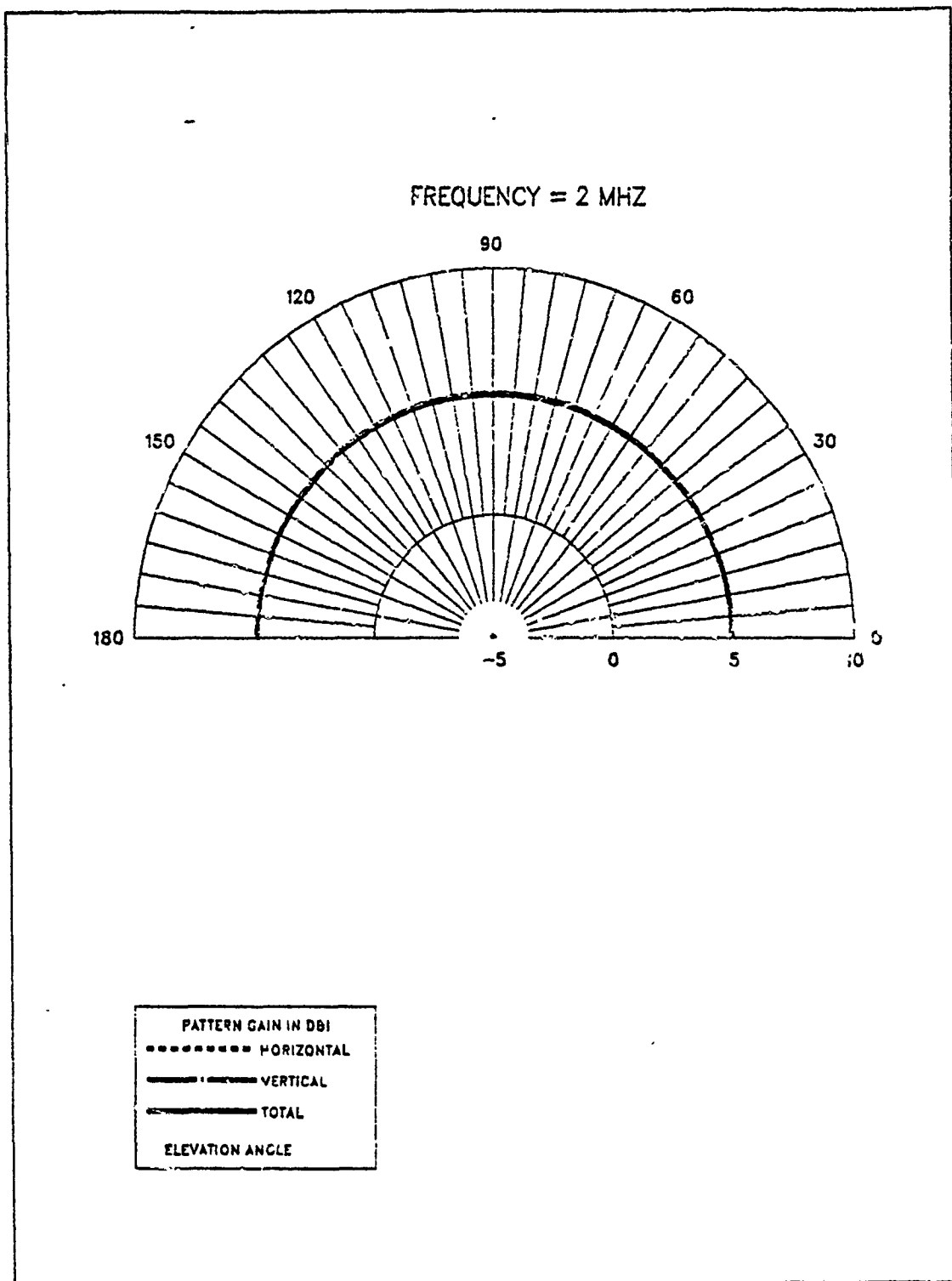
Figure 2.22 E-Field Elevation Pattern at 2 MHz for TF-TLA.
