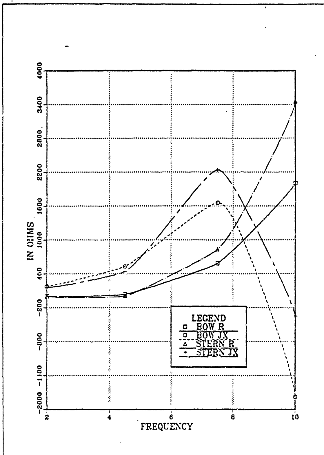
Figure 3.11 Input Impedance vs Frequency for TF-TLA on the Bow and the Stern.
