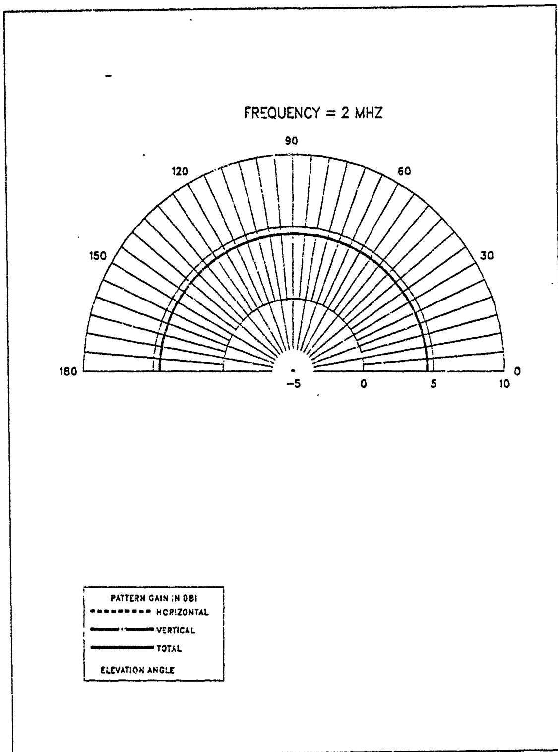
Figure 2.14 E-Field Elevation Pattern at 2 MHz for EF-TLA.
