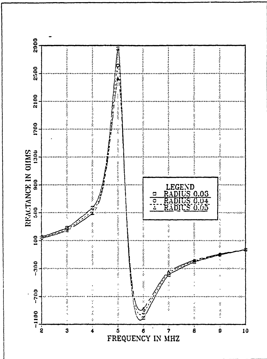
Figure 2.3 Reactance vs Frequency for a 9 Segment EF-TLA with Three Different Wire Radii.
