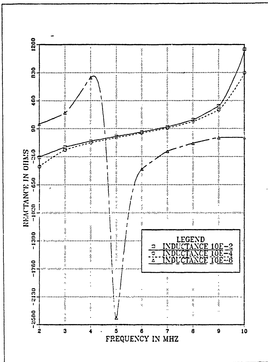
Figure 2.11 Reactance vs Frequency for EF-TLA with Three Different Inductive Loads.
