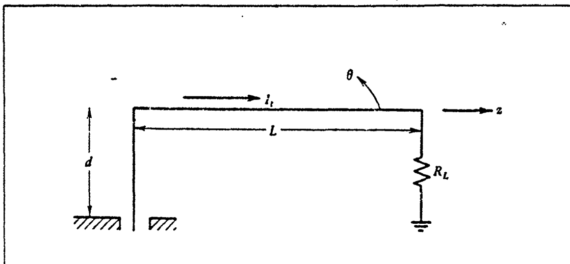
Figure 1.1 Transmission Line Antenna.
