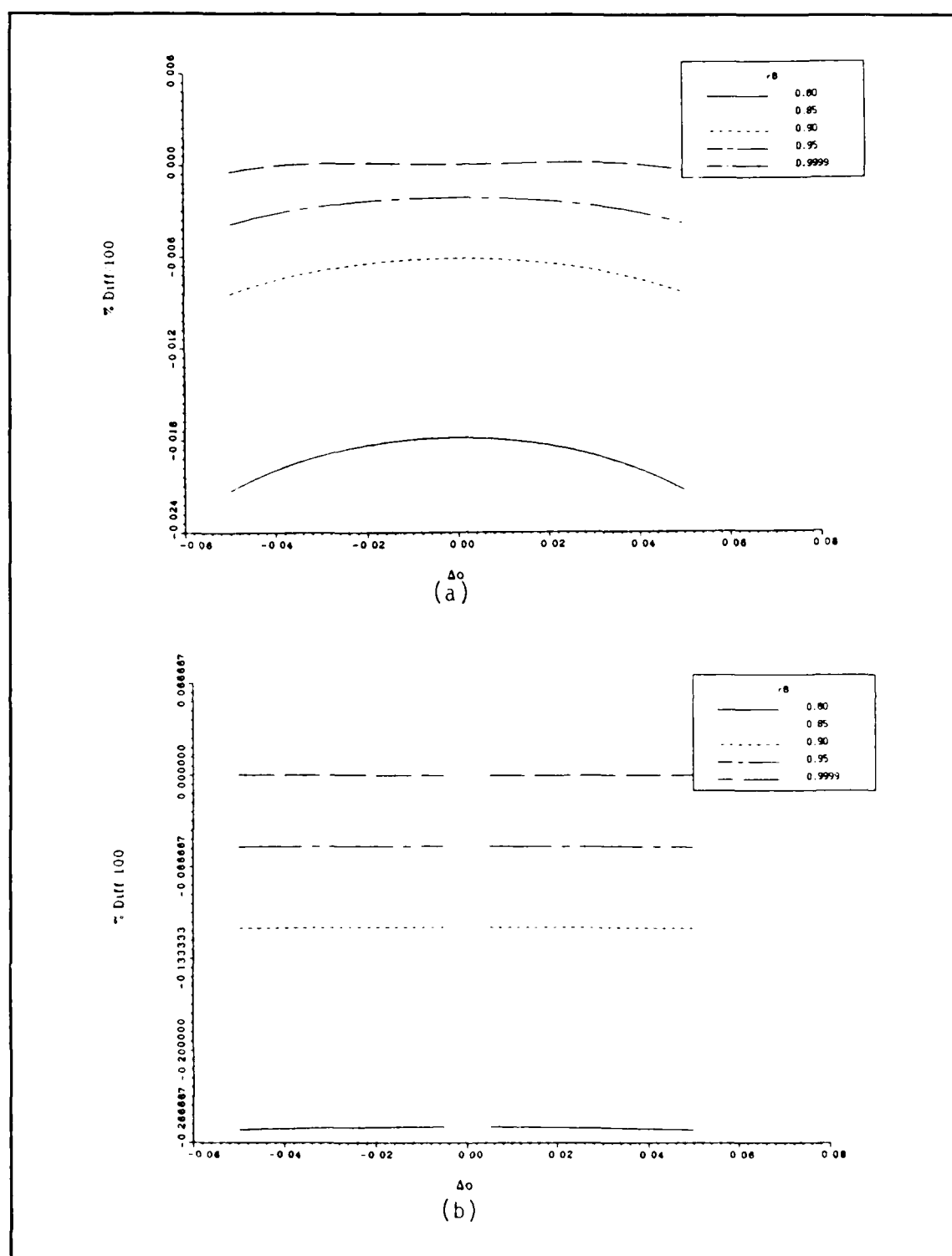
Figure 7.20. Percentage differences in the observables, TWL and Chow models. The laser parameters are from data set 27. (a) I_R(0) and I_n , (b) I_L , and (c) G_2 .
