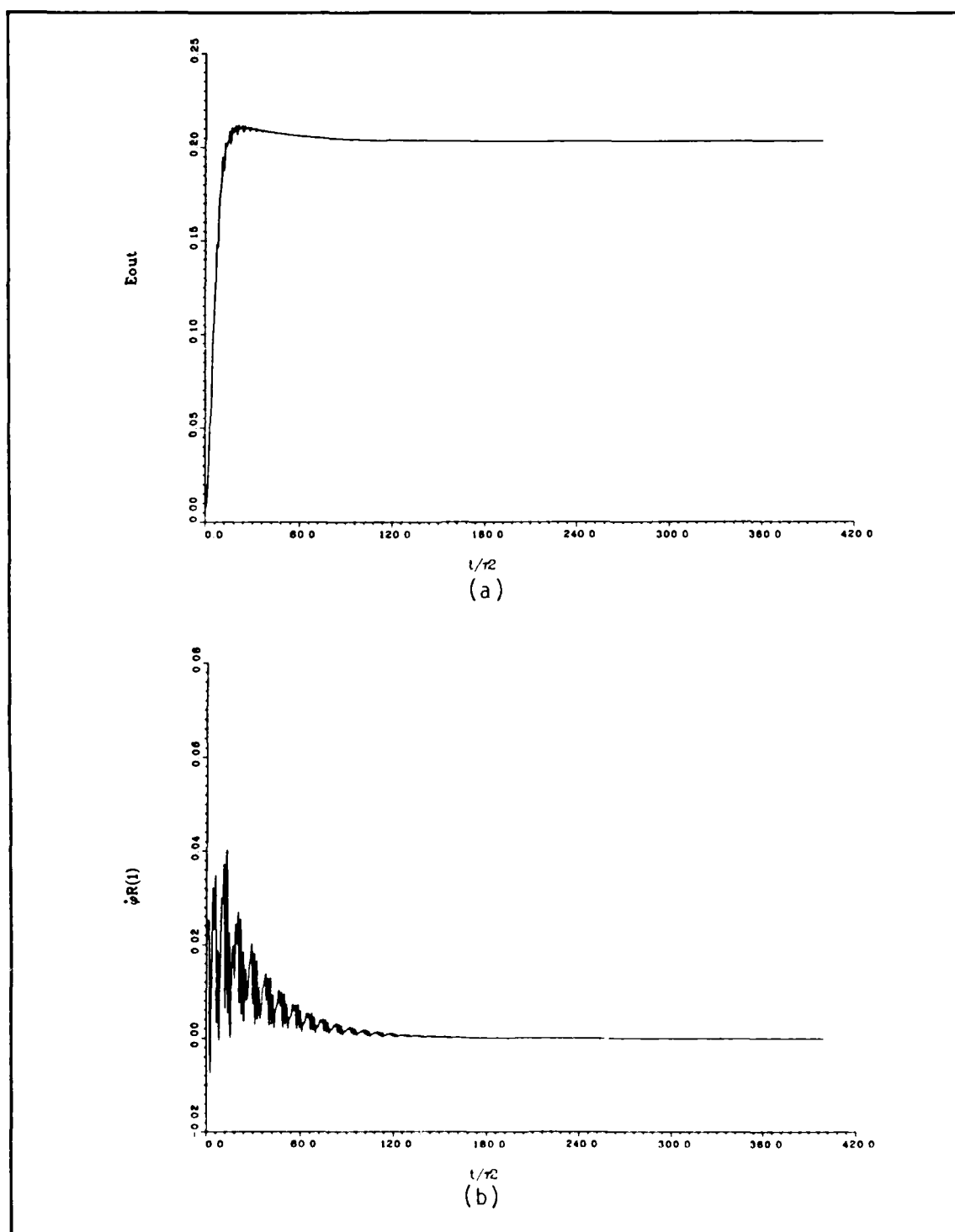
Figure 7.9. Injected laser output field with the injected signal strength above the locking threshold. I_{IN} = 3.61 \times 10^{-4} . All other parameters are taken from Figure 7.7. (a) \hat{E}_{out} vs \hat{t} . (b) \hat{\phi}_R(1) vs \hat{t} .
