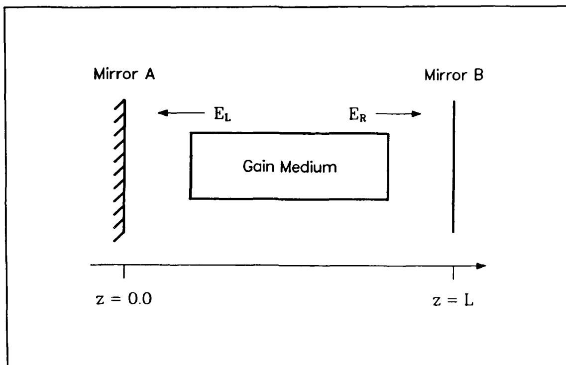
Figure 3.1. The Fabry-Perot laser.
