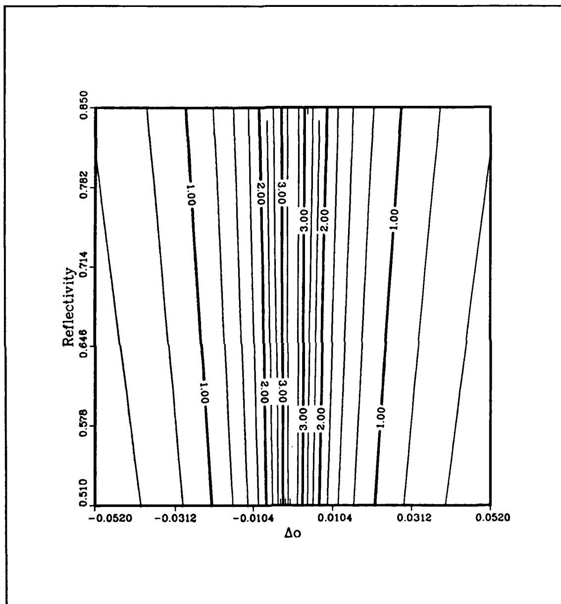
Figure C.58. \log_{10} G_2 contours at the MG2 point (data set 27). The data is from as large a rectangular region in the (\Delta\delta, r_D) plane as possible.
