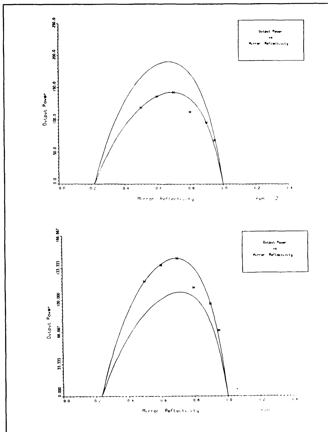
Figure 7.16. XeF laser data. Theoretical curves for both models are plotted. (a) Data fit to the TWL model. (b) Data fit to the simple saturable gain model.
