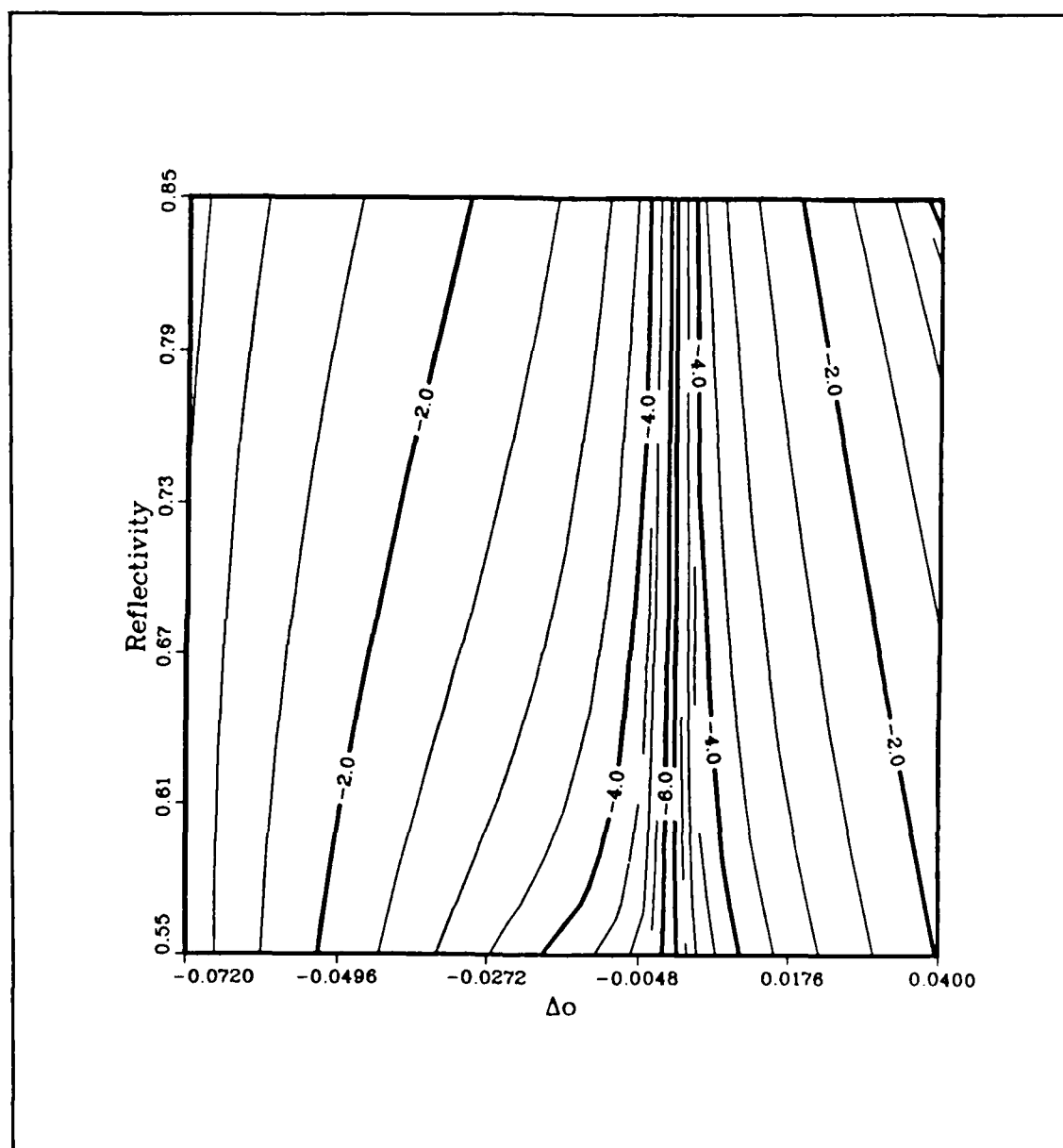
Figure C.25. \log_{10} I_I contours at the MG2 point (data set 36). The data is from as large a rectangular region in the (\Delta\hat{o}, r_B) plane as possible.
