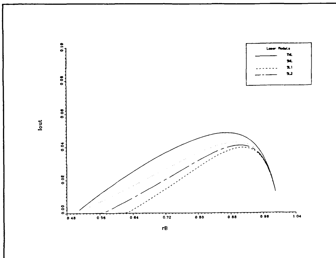
Figure 7.12. I_{out} vs r_B for the TWL, SWL, SL1, and SL2 models. All parameters are from data set 27.
