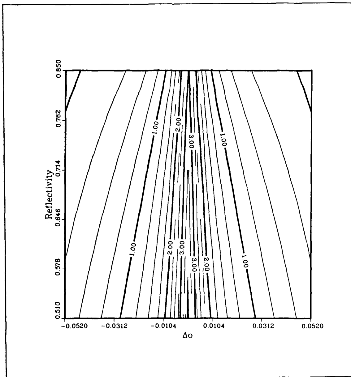
Figure C.41. \log_{10} G_1 contours at the MG2 point (data set 27). The data is from as large a rectangular region in the (\Delta\hat{o}, r_D) plane as possible.
