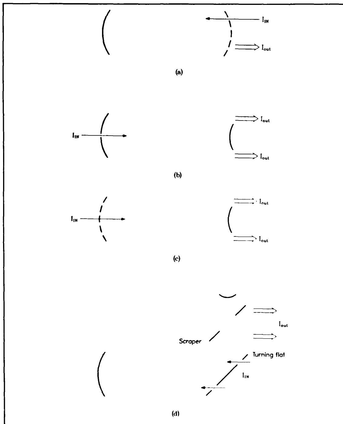
Figure 1.2. Various methods of injection locking. The dotted lines indicate partially transmissive mirrors. I_{IN} is the injected field; I_{out} is the output field from the slave laser. Adapted from (38).
