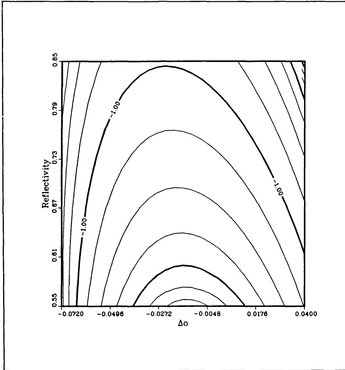
Figure C.8. \log_{10} I_R(0) contours at the MG2 point (data set 36). The data is from as large a rectangular region in the (\Delta\hat{o}, r_D) plane as possible.
