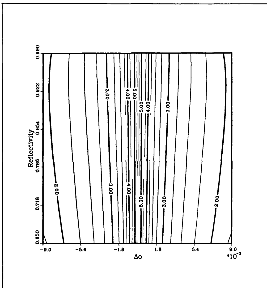
Figure C.52. \log_{10} G_2 contours at the MII point (data set 27).
