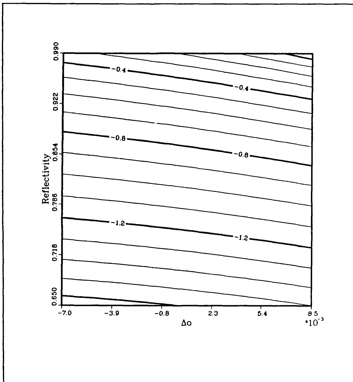
Figure C.6. \log_{10} I_R(0) contours at the MG2 point (data set 36). The data is from the region in the (\Delta\delta, r_B) plane where the cubic curves retain the s-shape.
