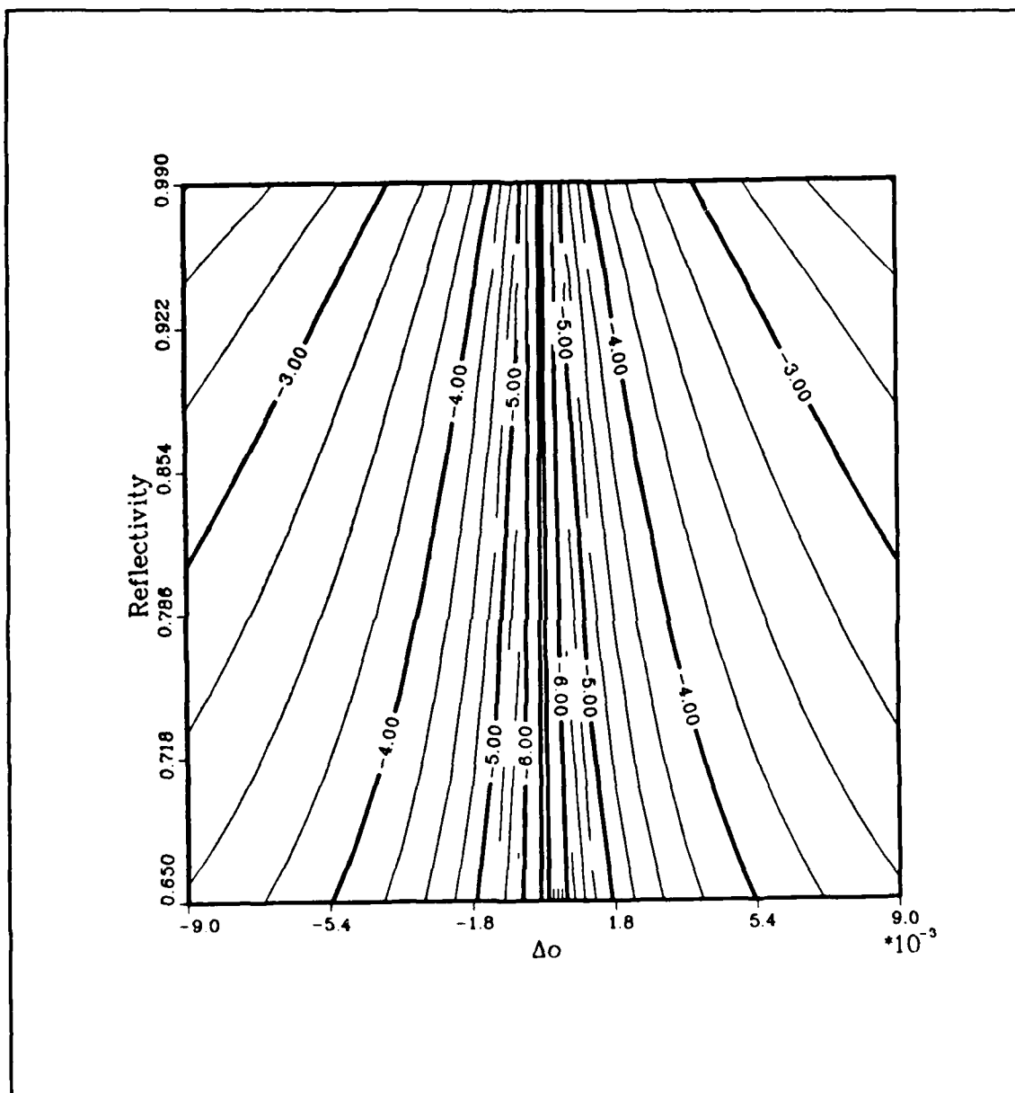
Figure C.22. \log_{10} I_I contours at the MG2 point (data set 27). The data is from the region in the (\Delta\delta, \tau_B) plane where the cubic curves retain the s-shape.
