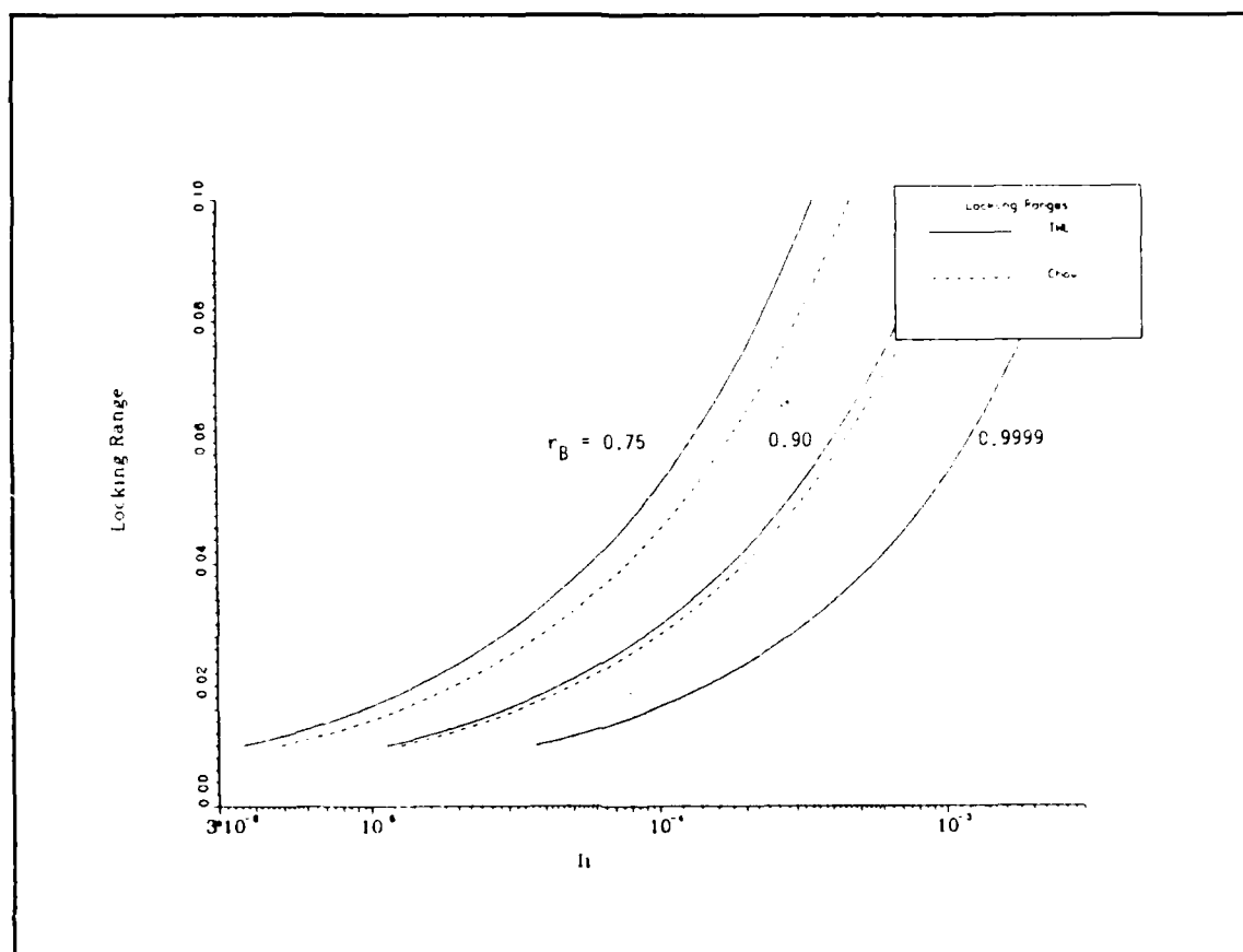
Figure 7.22. Full locking range comparisons between the TWL and Chow models. The laser parameters are from data set 27.
