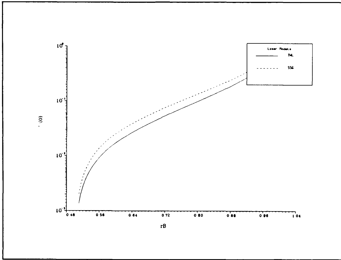
Figure 7.10. I_R(0) vs r_B for the simple saturable gain (SSG) model and the TWL model. All parameters are taken from data set 27.
