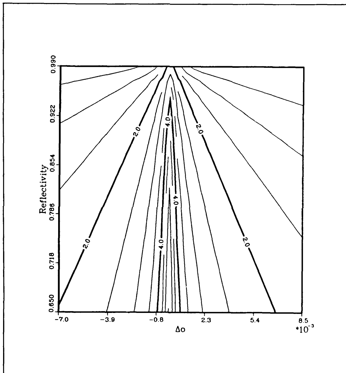
Figure C.38. \log_{10} G_1 contours at the MG1 point (data set 36).
