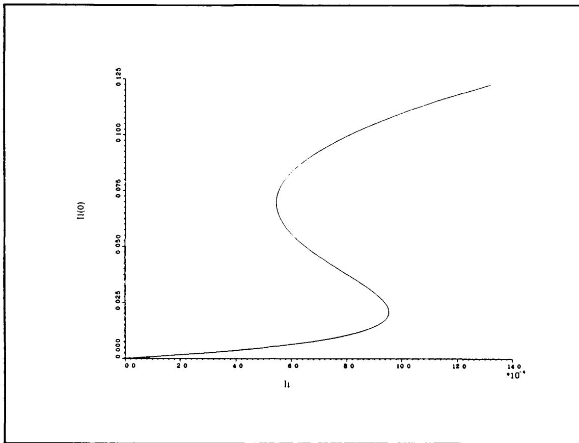
Figure 8.1. A sample cubic curve. M = 1.33 , \Delta\delta = 0.008 . All other parameters are taken from data set 15.
