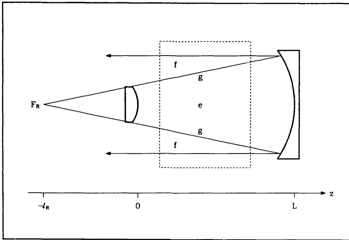
Figure 5.2. The fields in the PBCUR laser.
