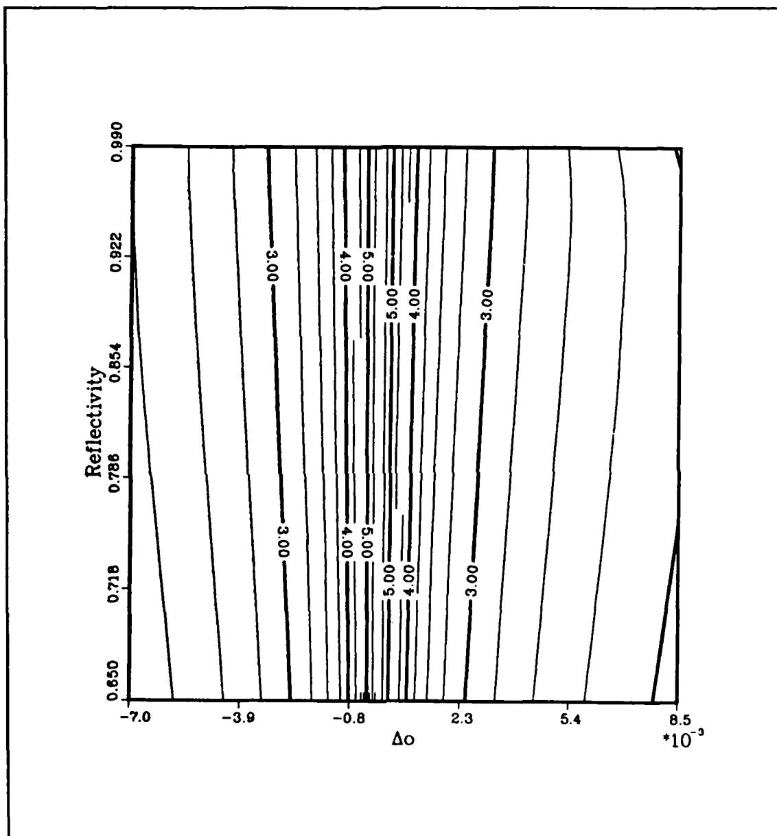
Figure C.55. \log_{10} G_2 contours at the MG1 point (data set 36).
