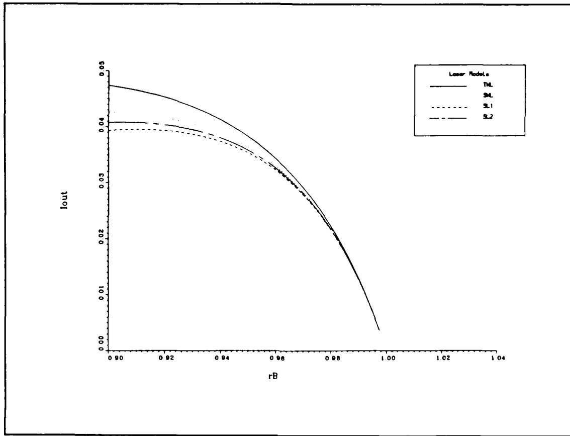
Figure 7.13. I_{out} vs r_B for the TWL, SWL, SL1, and SL2 models at high mirror reflectivities. All parameters are from data set 27.
