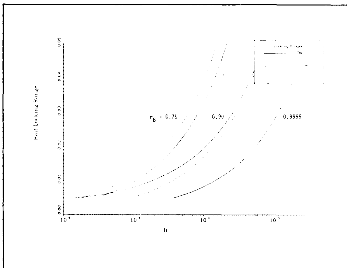
Figure 7.21. Half-locking range comparisons between the TWL and Spencer-Lamb models. The laser parameters are from data set 27.
