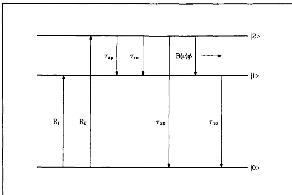
Figure 1.3. Energy level diagram of a typical lasing atom.
