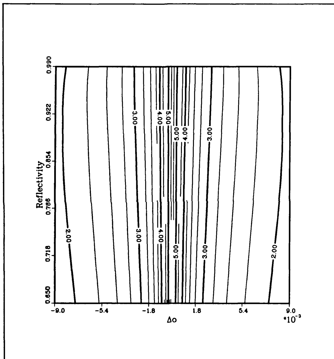
Figure C.54. \log_{10} G_2 contours at the MG1 point (data set 27).
