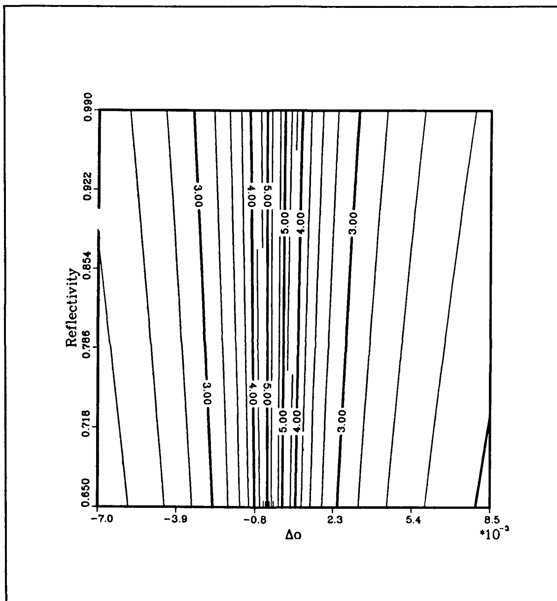
Figure C.57. \log_{10} G_2 contours at the MG2 point (data set 36). The data is from the region in the (\Delta\hat{o}, r_D) plane where the cubic curves retain the s-shape.
