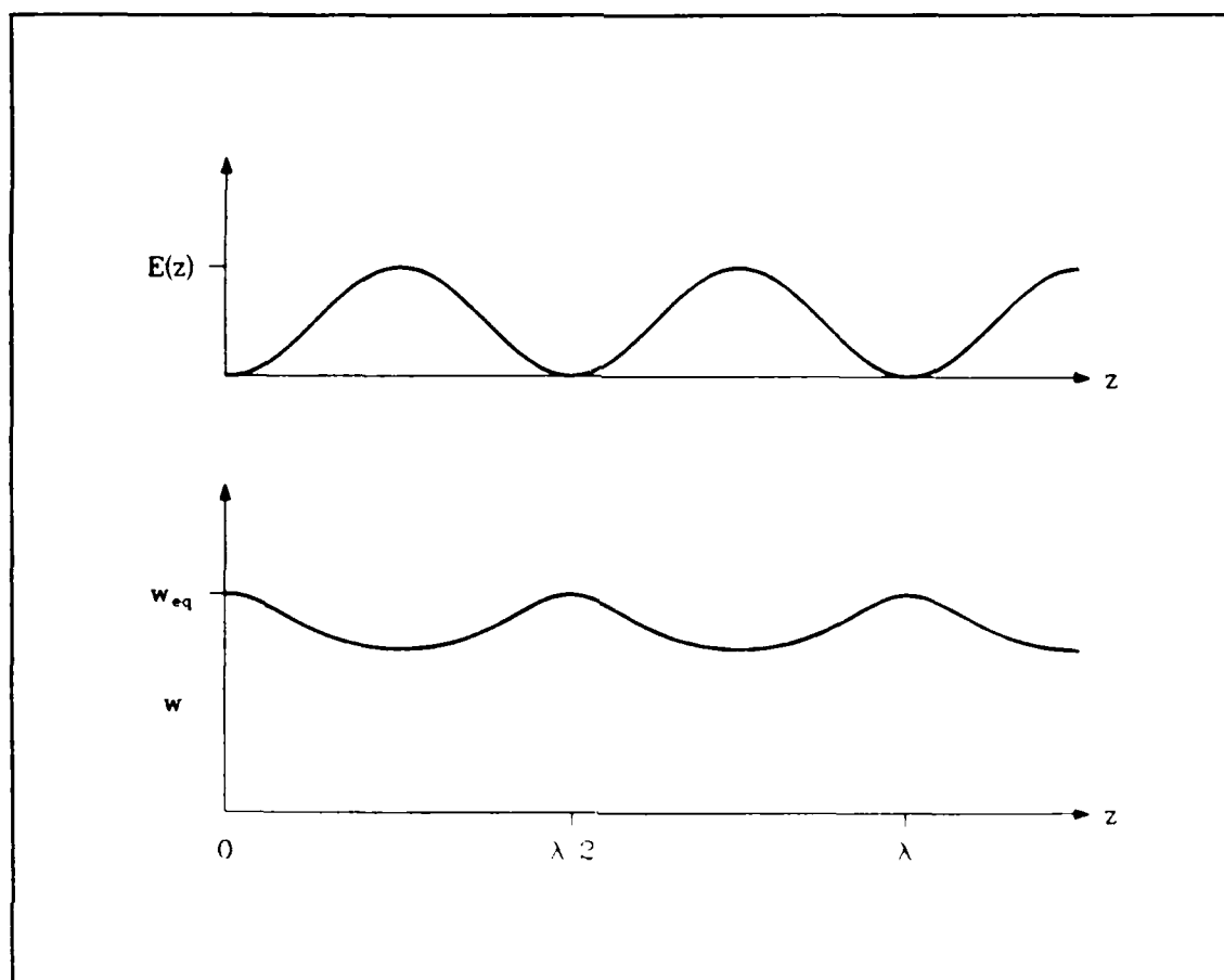
Figure 4.1. Spatial hole burning. The upper plot illustrates the standing wave electric field; the lower plot is the population inversion density.
