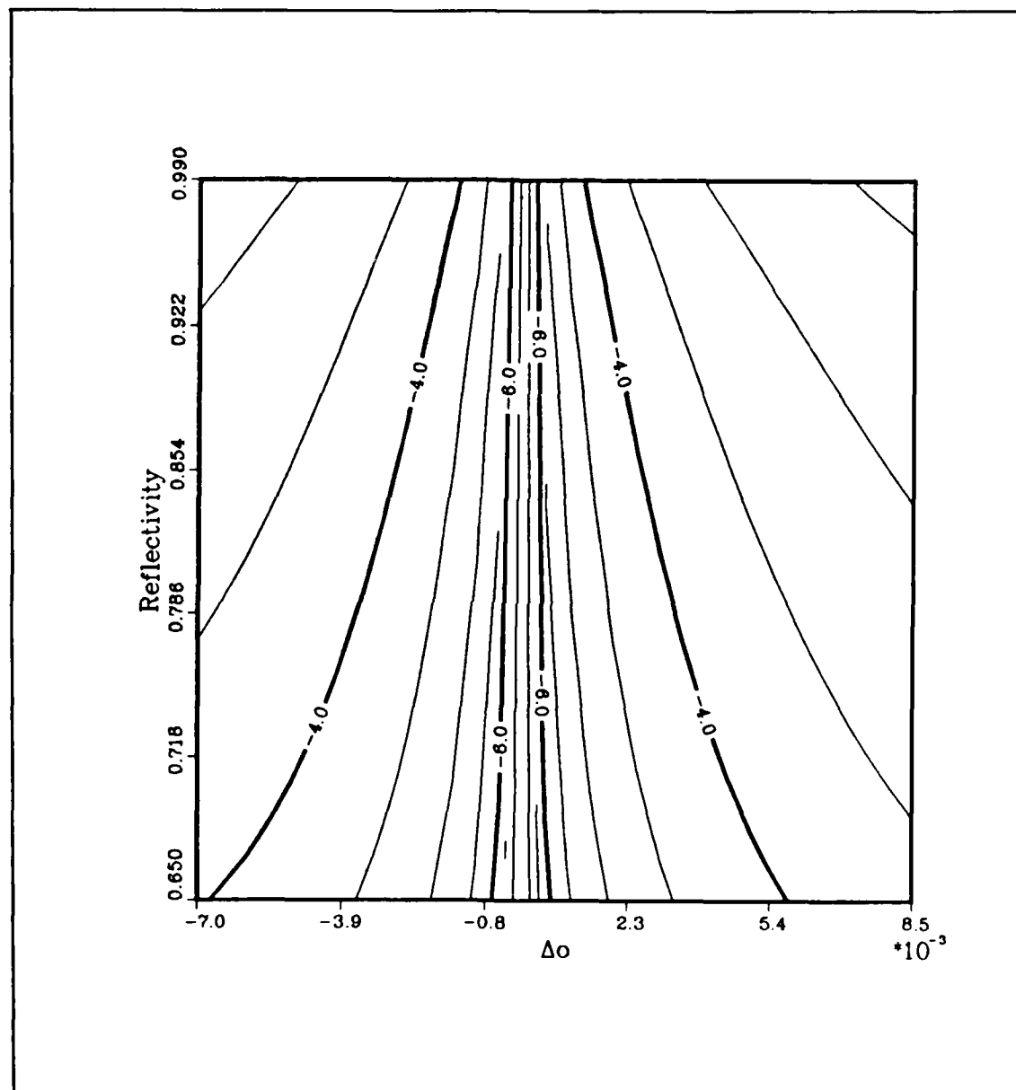
Figure C.21. \log_{10} I_l contours at the MG1 point (data set 36).
