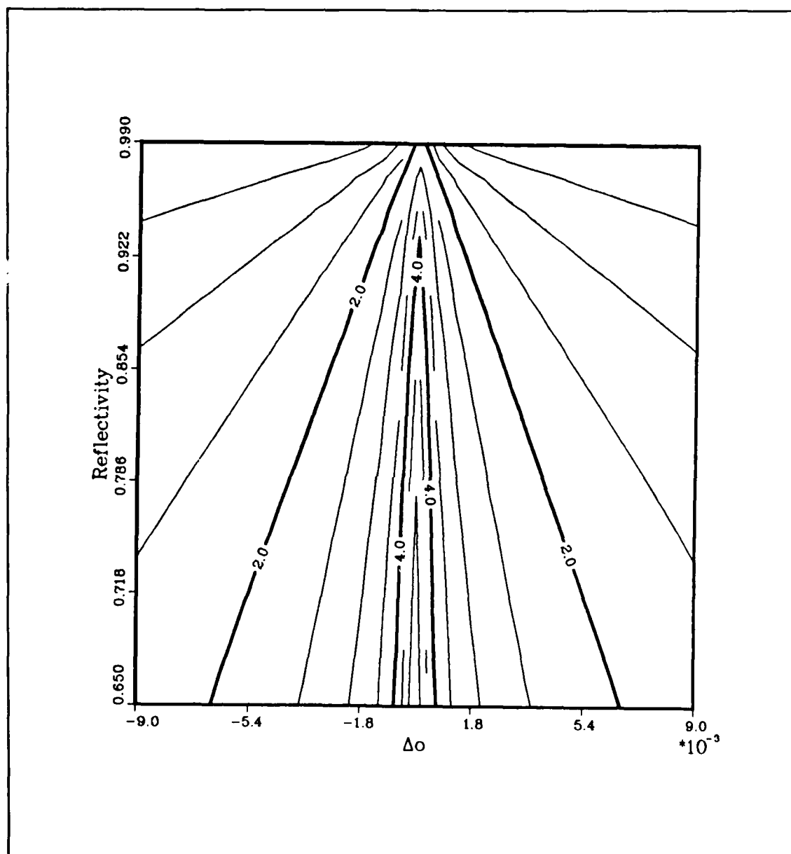
Figure C.35. \log_{10} G_1 contours at the MII point (data set 27).
