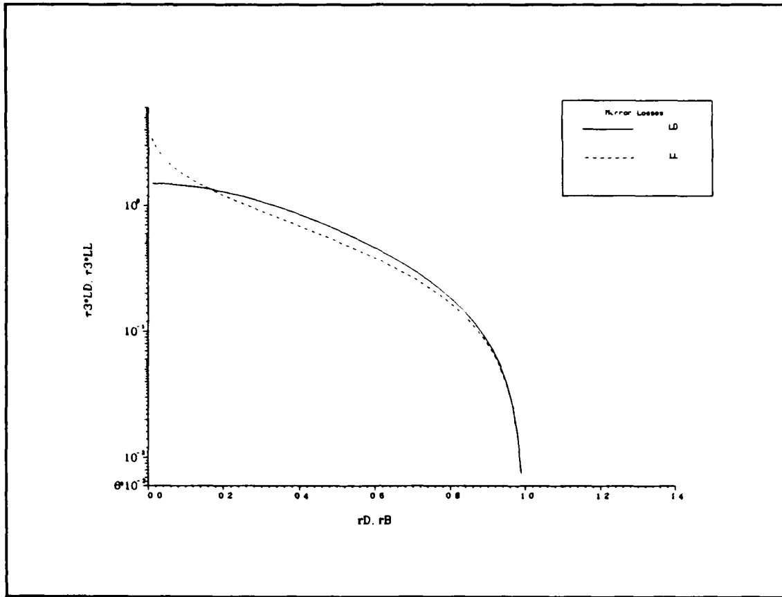
Figure A.3. Comparison of the laser losses L_{D,L} vs mirror reflectivity. Note that the losses are parameterized in terms of \hat{\tau}_3 .
