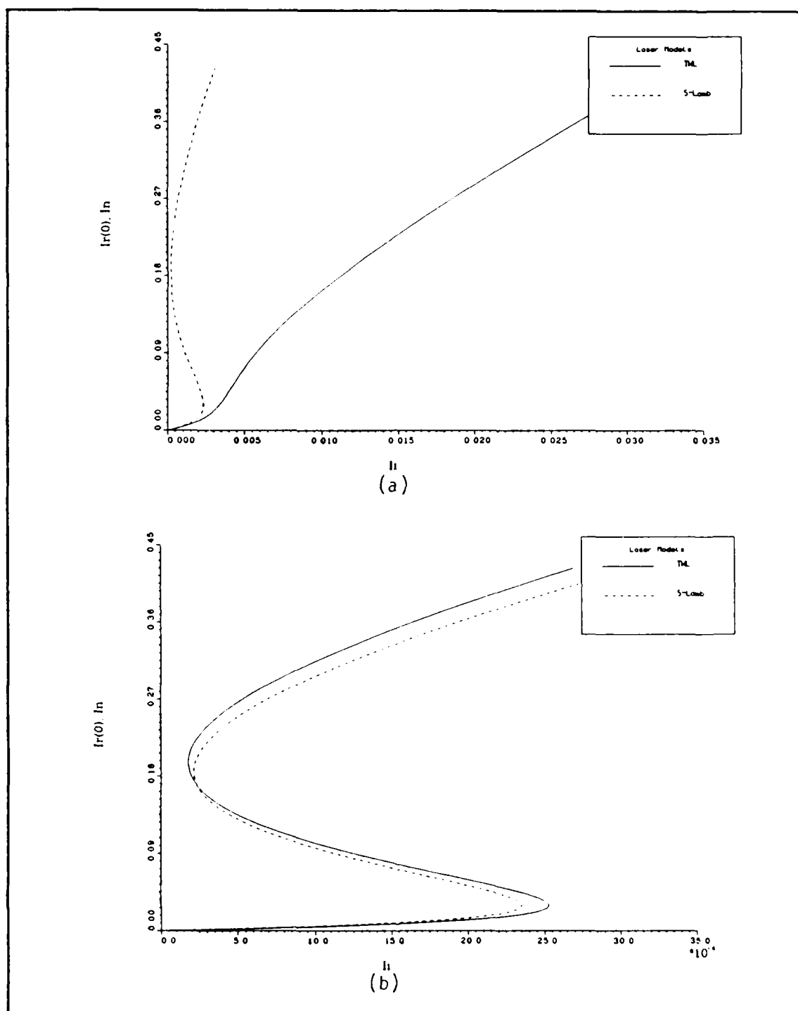
Figure 7.18. Cubic curve comparisons between the Spencer-Lamb and TWL models. r_B = 0.90 and \Delta\delta = 0.025 . All other parameters are taken from data set 27. (a) \hat{\theta} calculated from Eq (3.27b) in the TWL model. (b) \hat{\theta} = 0.0 in the TWL model. Note that the two curves are similar in shape.
