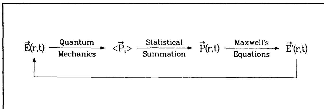
Figure 2.1. The self-consistent approach of the semiclassical theory. Adapted from (135:78).
