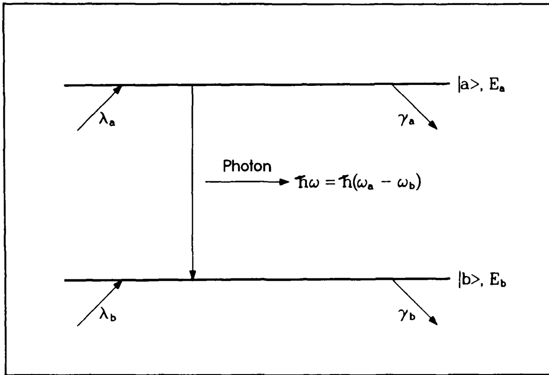
Figure 2.4. The two-level atomic system.
