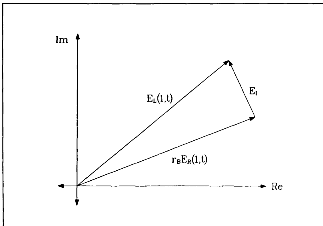
Figure 3.4. The phasor relationship at mirror B with an injected field.
