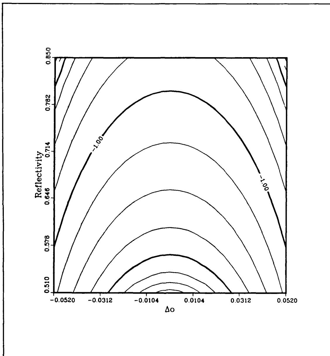
Figure C.7. \log_{10} I_R(0) contours at the MG2 point (data set 27). The data is from as large a rectangular region in the (\Delta\hat{o}, r_D) plane as possible.
