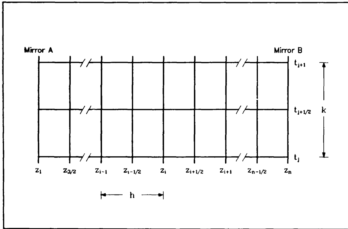
Figure B.1. The rectangular grid used with the modified Heun method.
