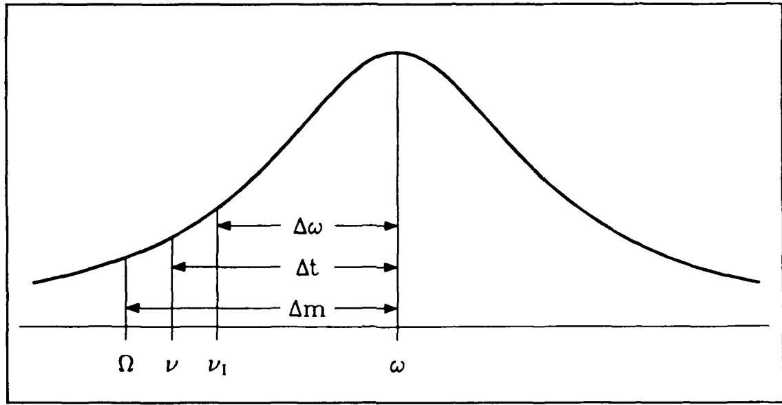
Figure 3.2. The atomic lineshape curve. Typical positions of the important frequencies are indicated.
