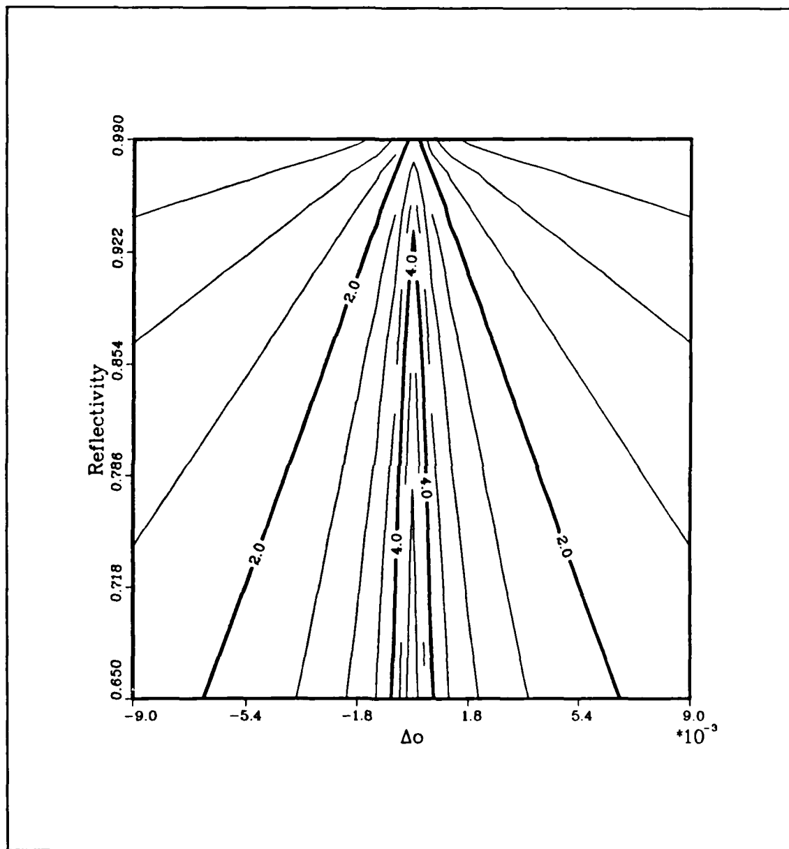
Figure C.37. \log_{10} G_1 contours at the MG1 point (data set 27).
