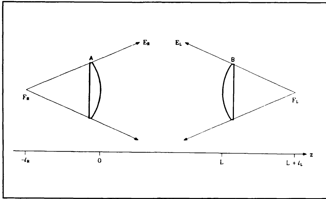
Figure 2.3. The general resonator fields. Adapted from (158:279).
