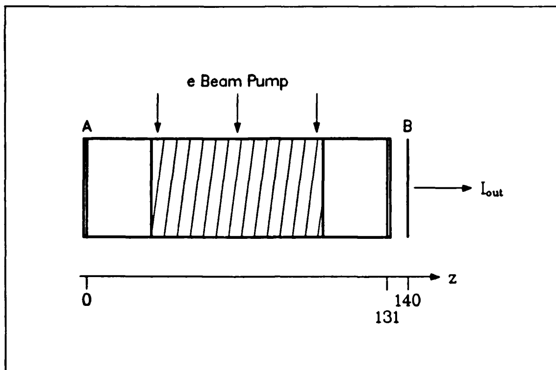
Figure 7.15. The XeF laser. Mirror A has a radius of curvature of 917 cm, whereas mirror B is a flat. Only the central portion (crosshatched) is pumped. All dimensions are in centimeters.
