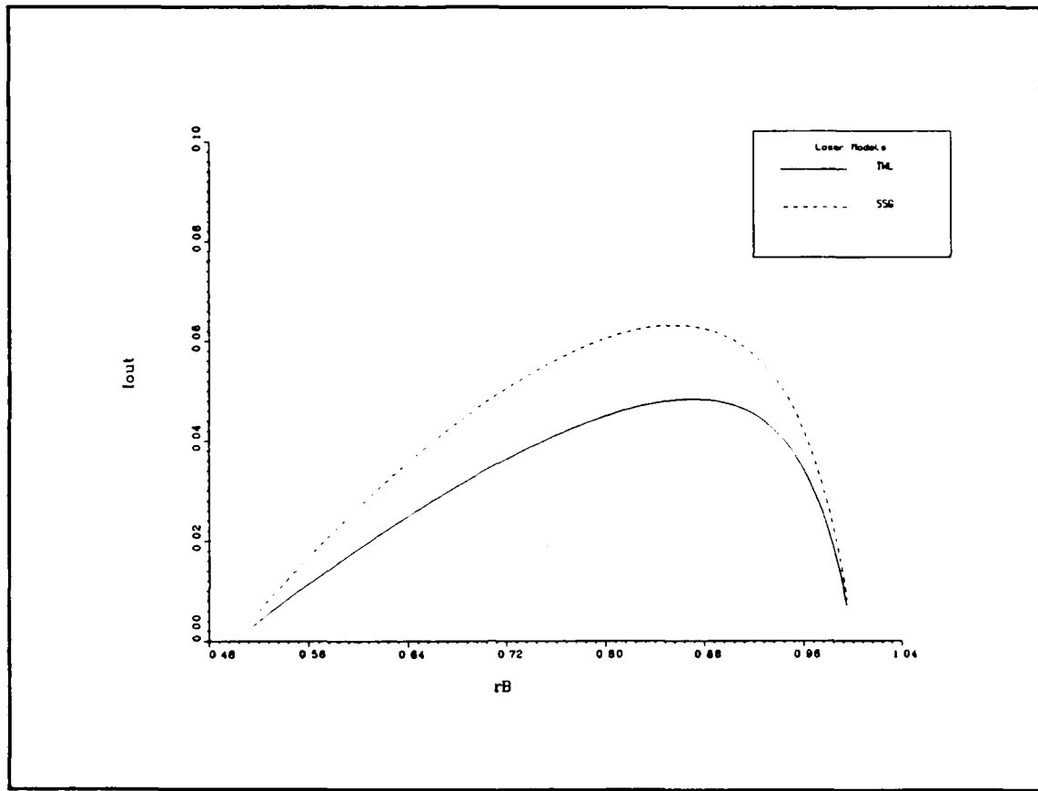
Figure 7.11. I_{out} vs r_B for the SSG and the TWL models. All parameters are the same as in Figure 7.10.
