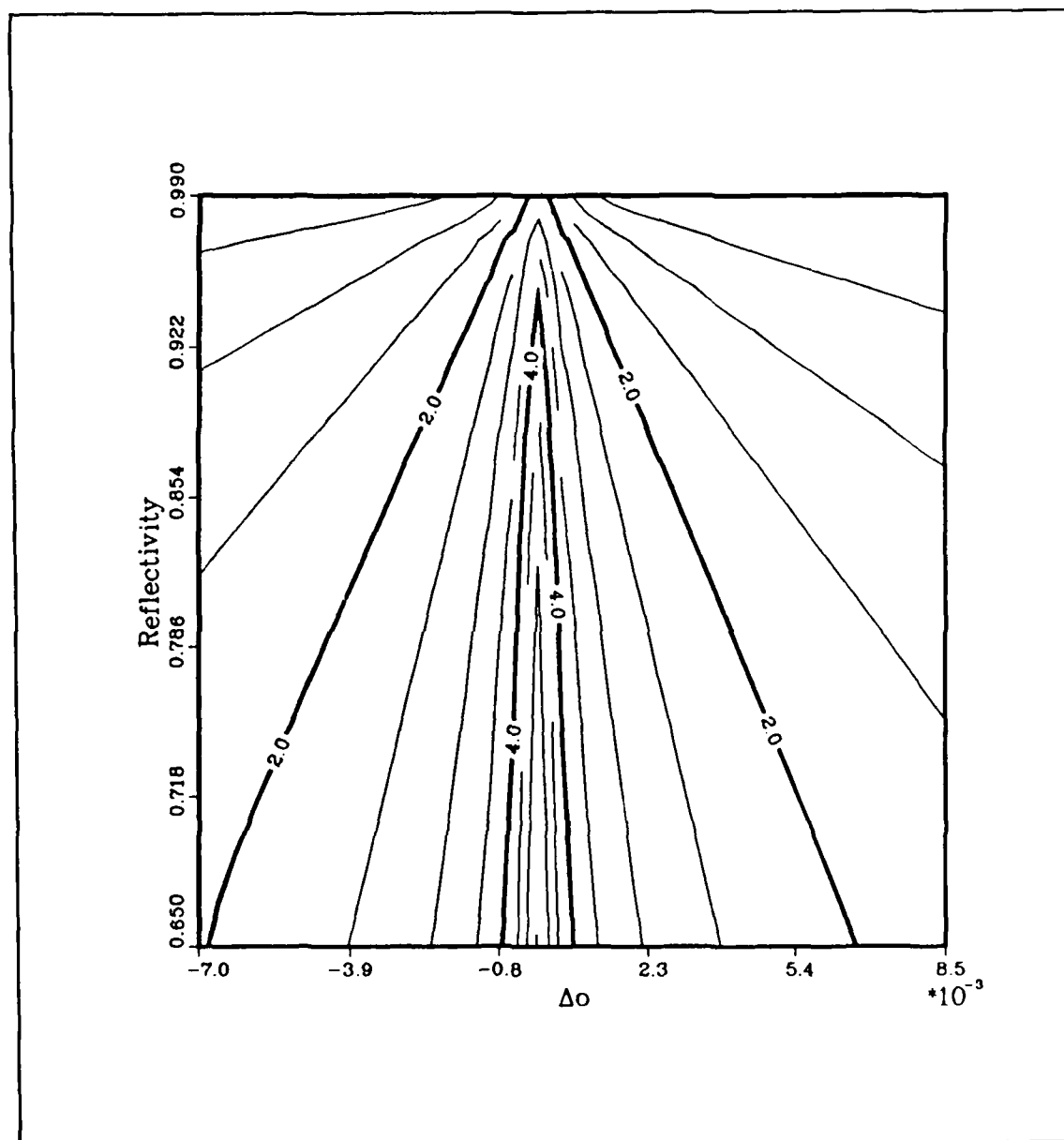
Figure C.36. \log_{10} G_1 contours at the MII point (data set 36).
