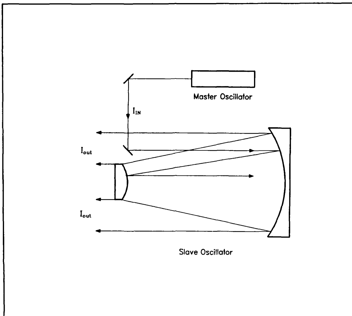
Figure 5.3. The injection technique used in the PBCUR laser. I_{IN} is the injected signal from the master oscillator; I_{out} is the beam radiated from the slave laser.
