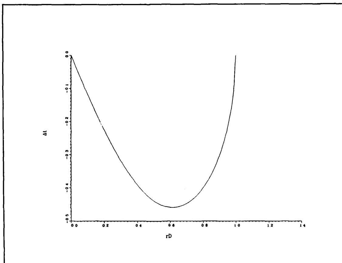
Figure A.2. The shift of \Delta \hat{t} vs r_D . The parameters used in the calculation come from data set 27: \Delta \hat{m} = 0.0 , \hat{r}_2 = 21.04145 , and \hat{r}_3 = 4/3 .
