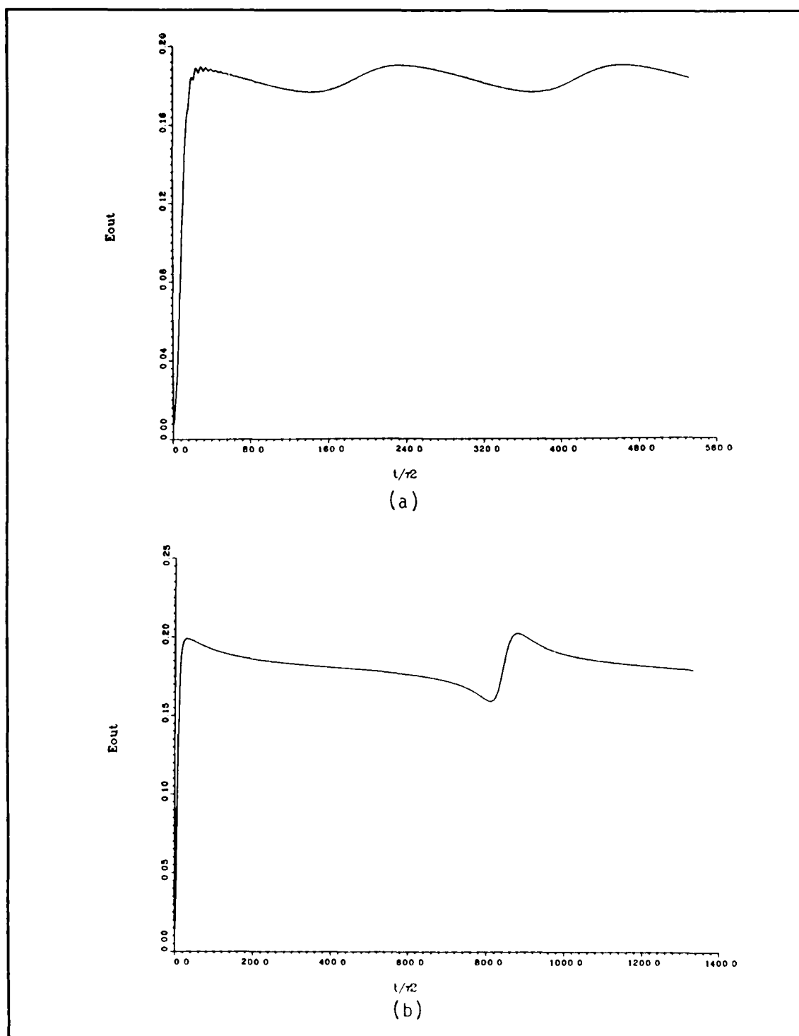
Figure 7.8. Injected laser output field amplitudes as a function of injected signal strength. (a) I_{IN} = 1.5 \times 10^{-5} . (b) I_{IN} = 1.5 \times 10^{-4} . All other parameters are taken from Figure 7.7.
