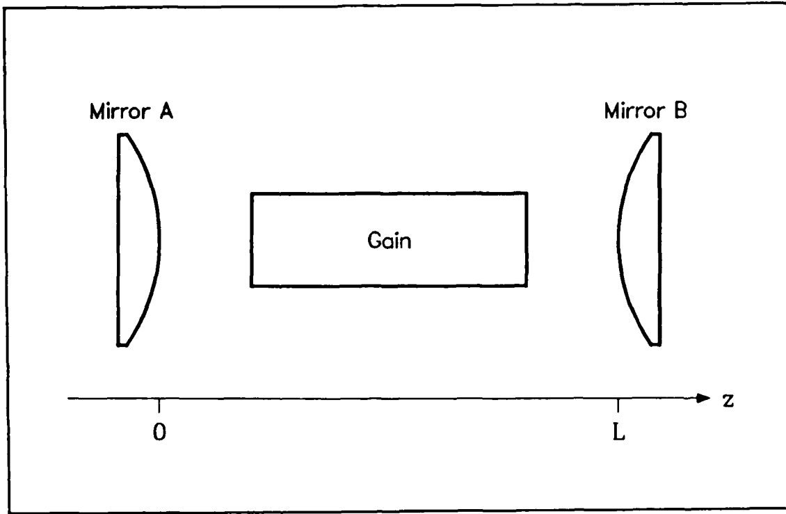
Figure 2.2. The general laser device.
