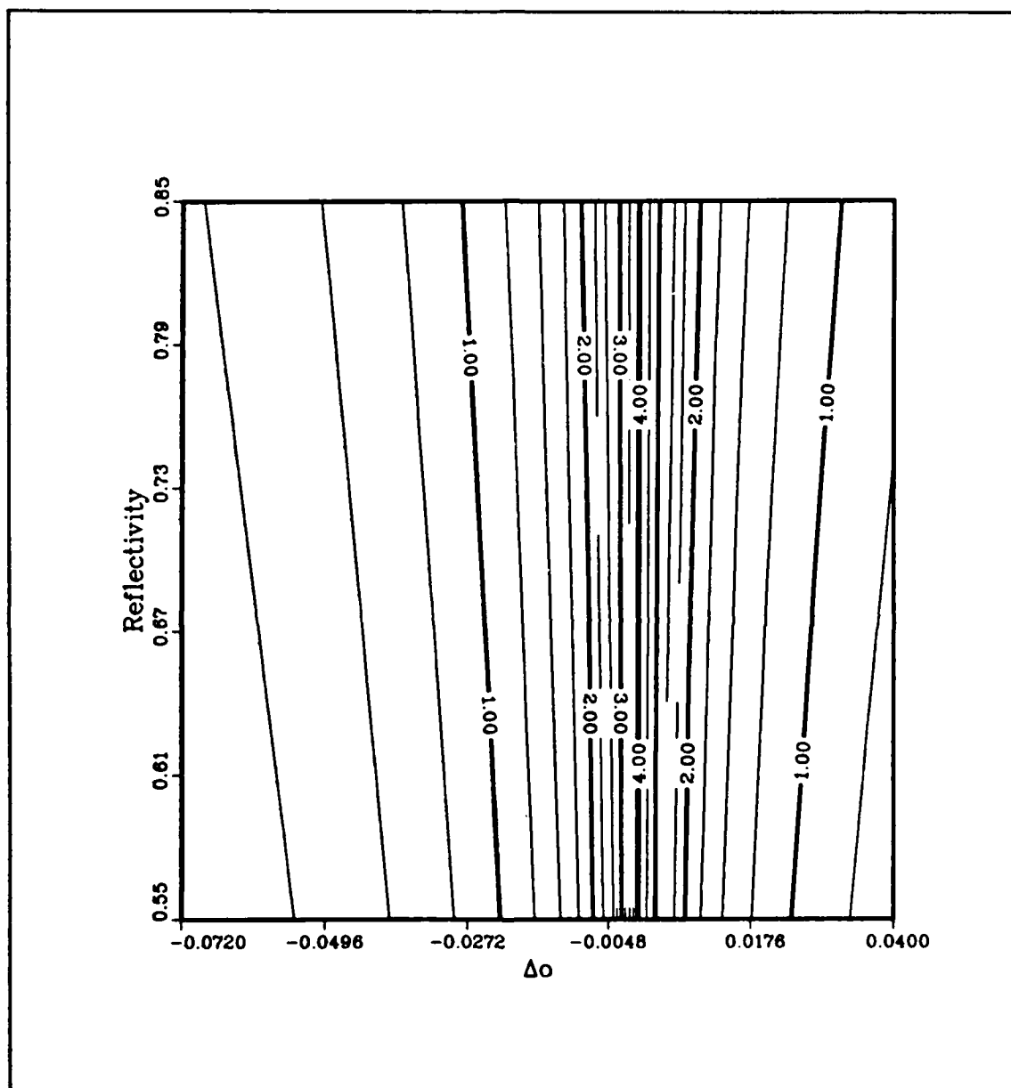
Figure C.59. \log_{10} G_2 contours at the MG2 point (data set 36). The data is from as large a rectangular region in the (\Delta\delta, r_D) plane as possible.
