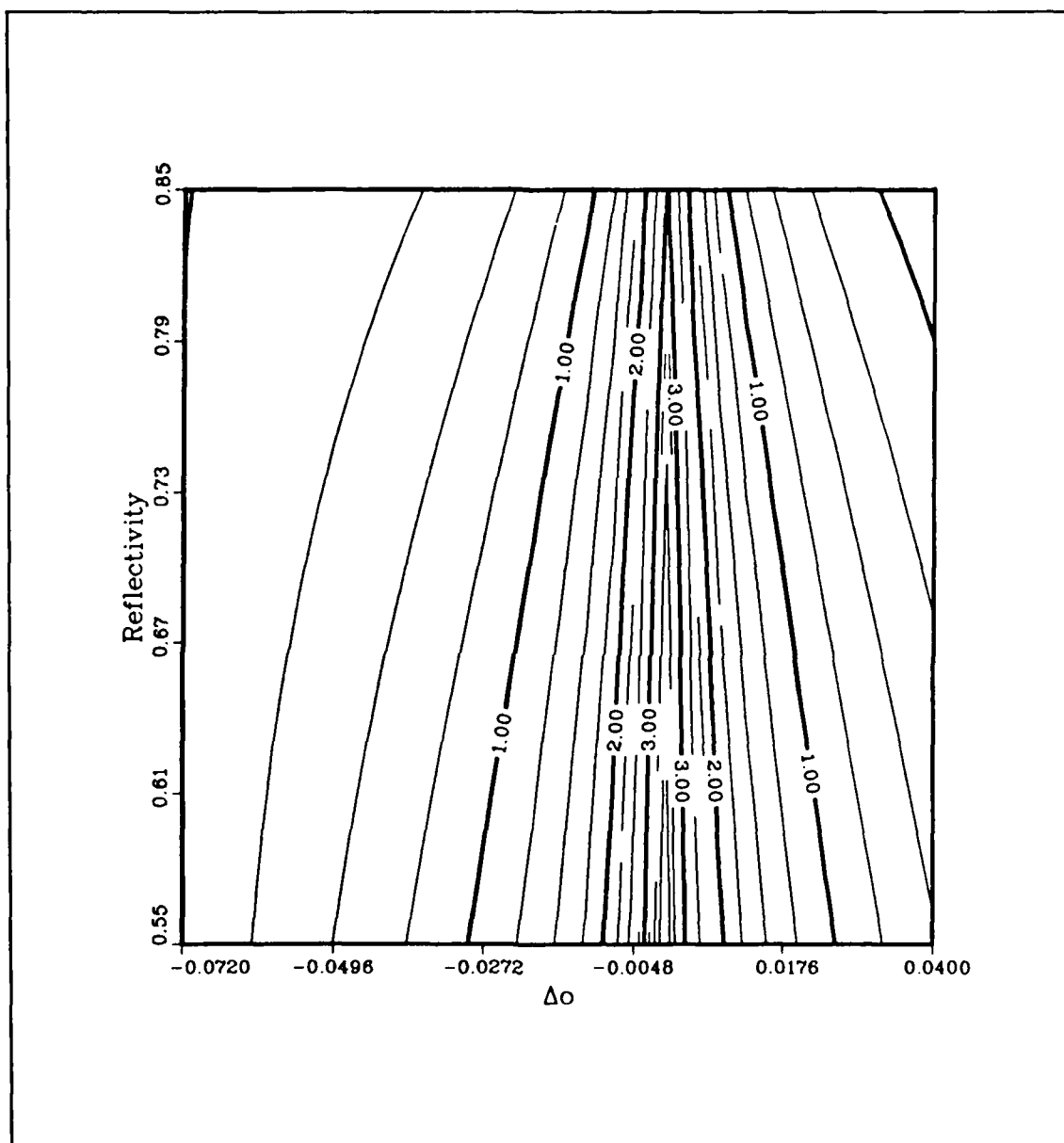
Figure C.42. \log_{10} G_1 contours at the MG2 point (data set 36). The data is from as large a rectangular region in the (\Delta\hat{o}, r_D) plane as possible.
