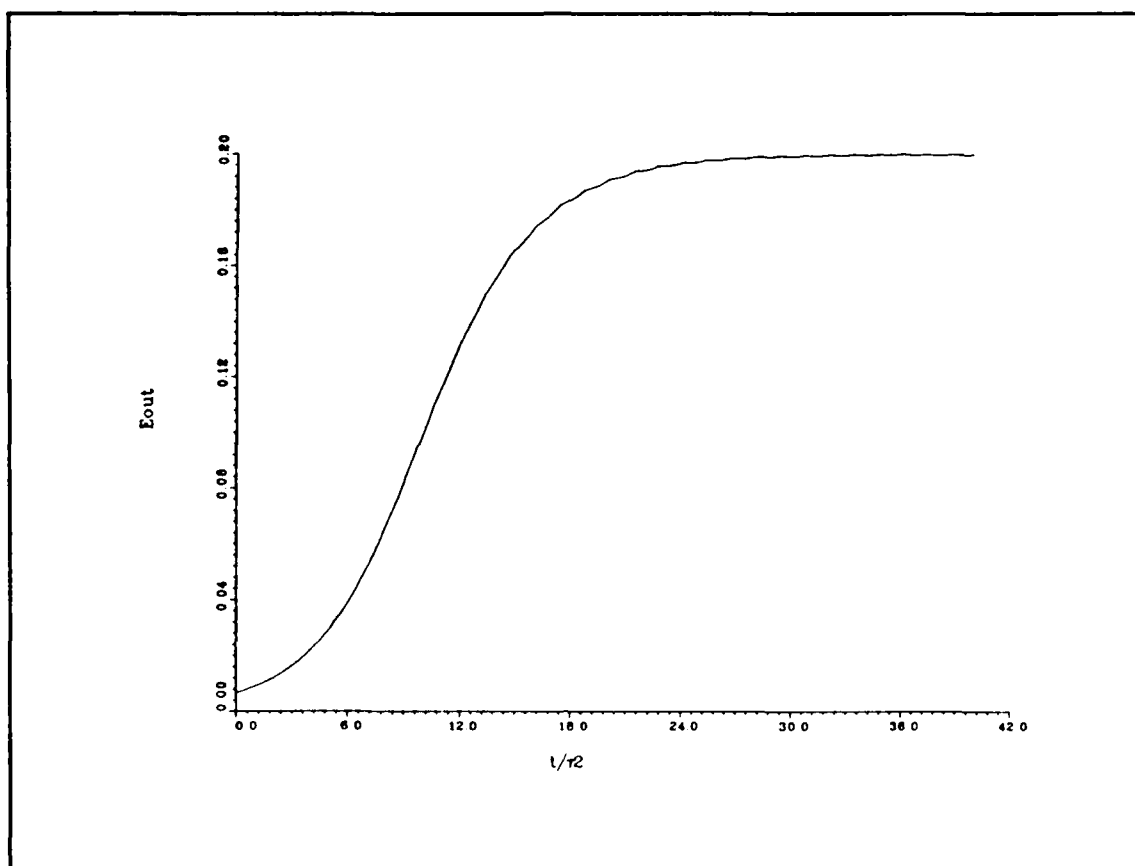
Figure 7.5. Typical time-dependent laser run. \hat{E}_{out} vs \hat{t} , for r_D = 0.75 . All other parameters are taken from data set 27.
