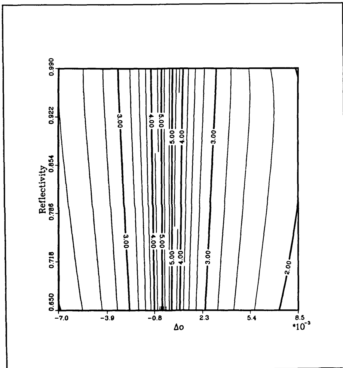
Figure C.53. \log_{10} G_2 contours at the MII point (data set 36).
