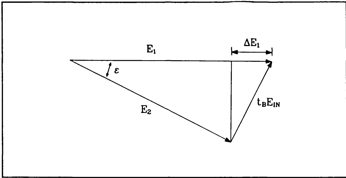
Figure 4.2. The round trip condition in the Chow model. \hat{E}_1 is the initially launched field, \hat{E}_2 is the field after a round trip, and t_B \hat{E}_{IN} is the injected field inside the laser. Adapted from (82).
