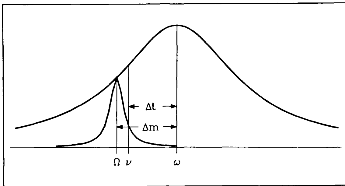
Figure 7.14. The physical mechanism underlying frequency pulling and pushing. \hat{\nu} is pulled toward linecenter, but still remains under the resonator response curve.
