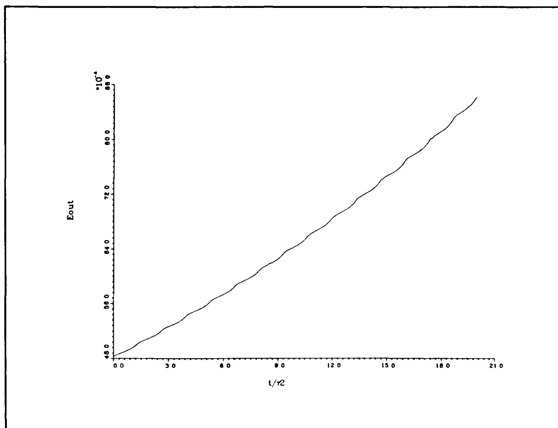
Figure 7.6. \hat{E}_{out} vs \hat{t} , for r_B = 0.26 . All other parameters are taken from data set 29. Note the ripples in the output field amplitude. Only the initial field rise is plotted.
