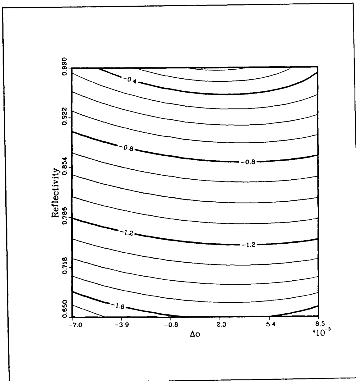
Figure C.2. \log_{10} I_R(0) contours at the MII point (data set 36).
