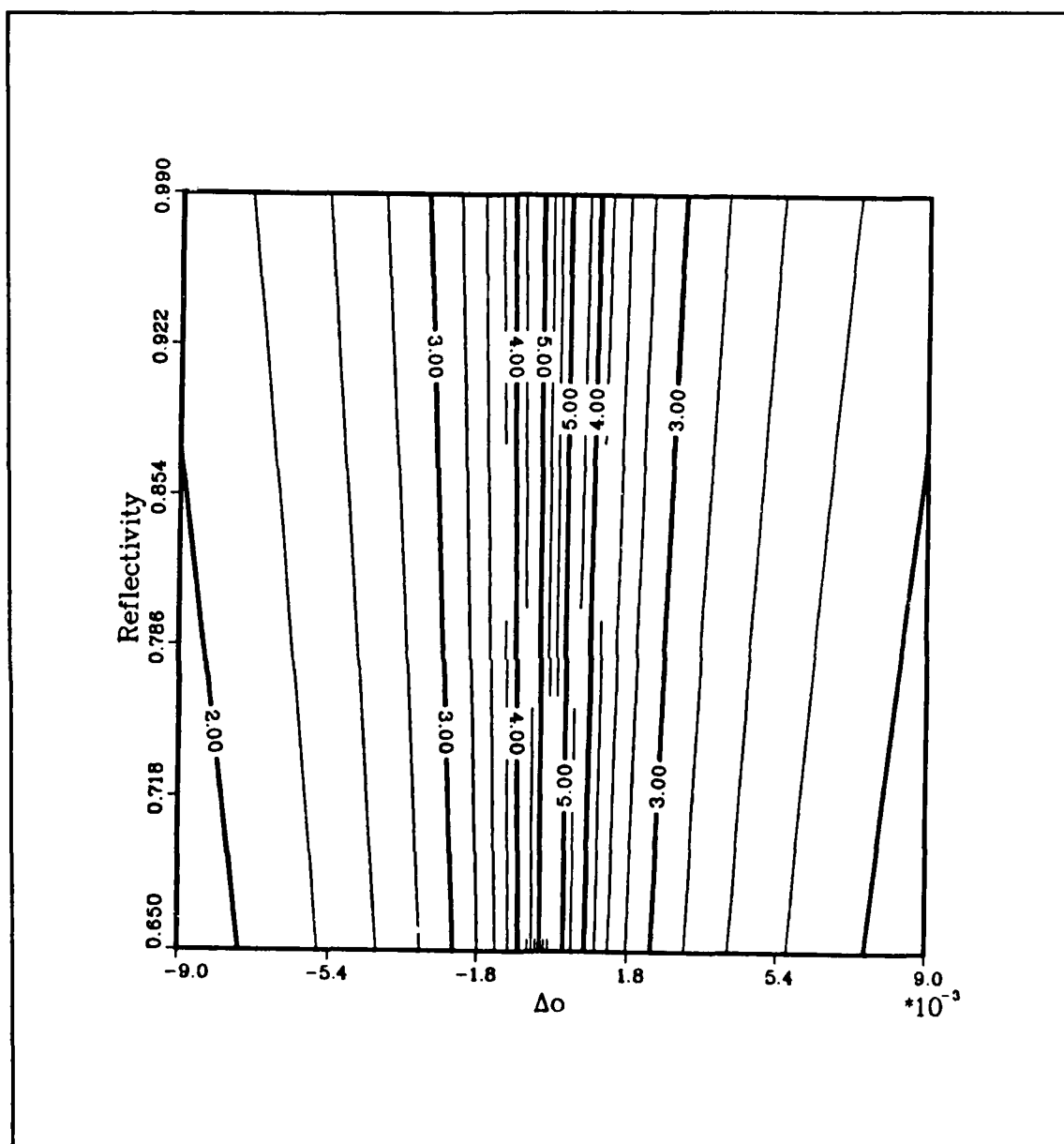
Figure C.56. \log_{10} G_2 contours at the MG2 point (data set 27). The data is from the region in the (\Delta\delta, r_D) plane where the cubic curves retain the s-shape.
