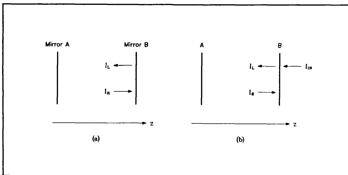
Figure 1.4. Fields at the injection mirror. (a) Without injection, (b) with injection.
