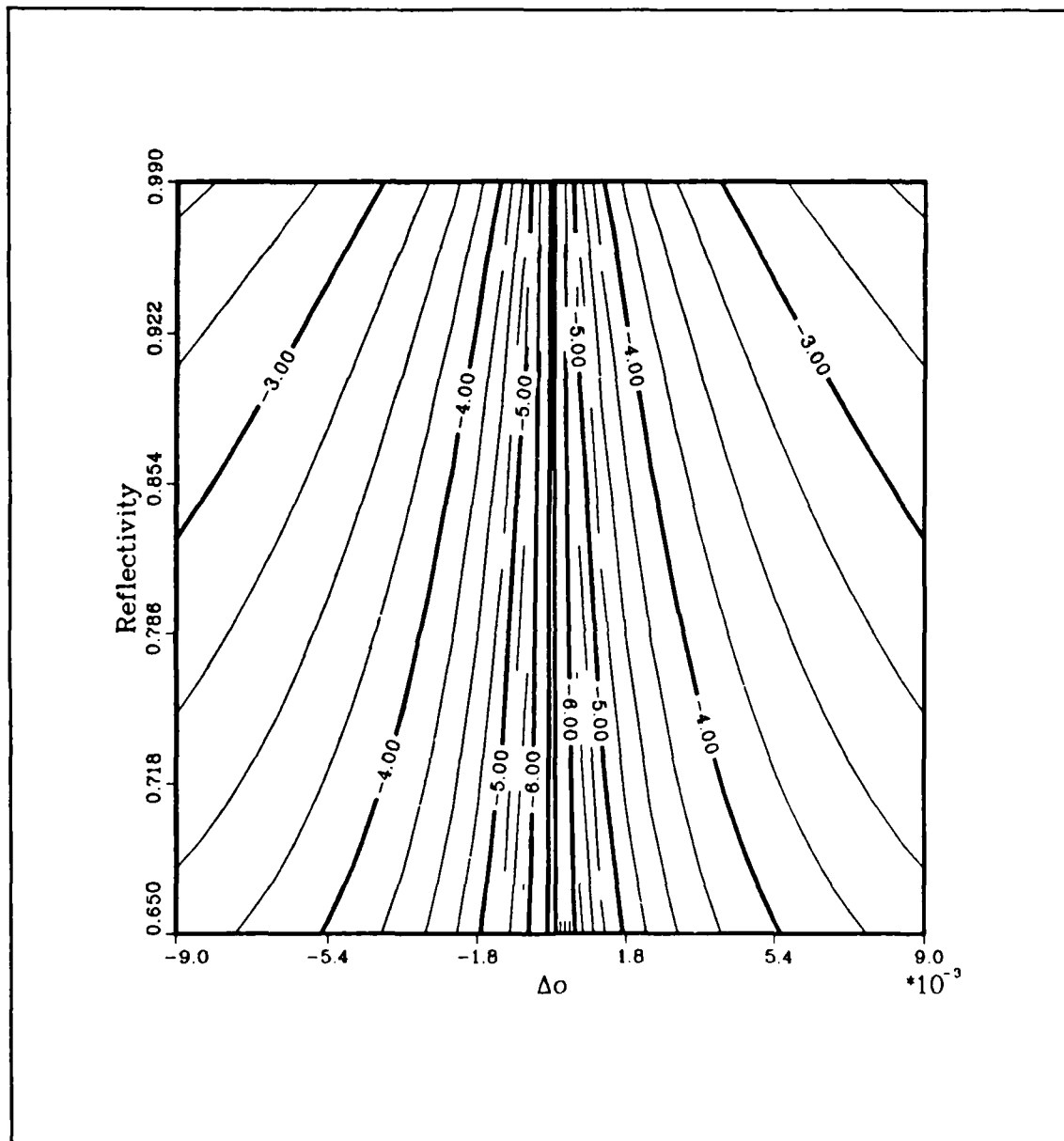
Figure C.18. \log_{10} I_I contours at the MII point (data set 27).
