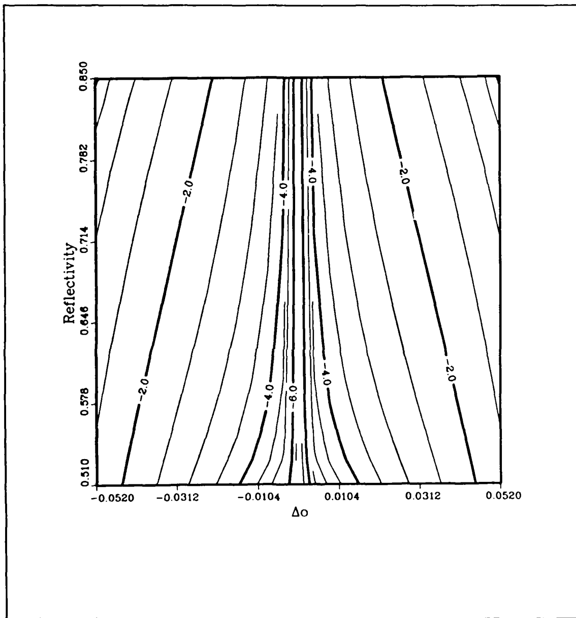
Figure C.24. \log_{10} I_I contours at the MG2 point (data set 27). The data is from as large a rectangular region in the (\Delta\delta, r_D) plane as possible.
