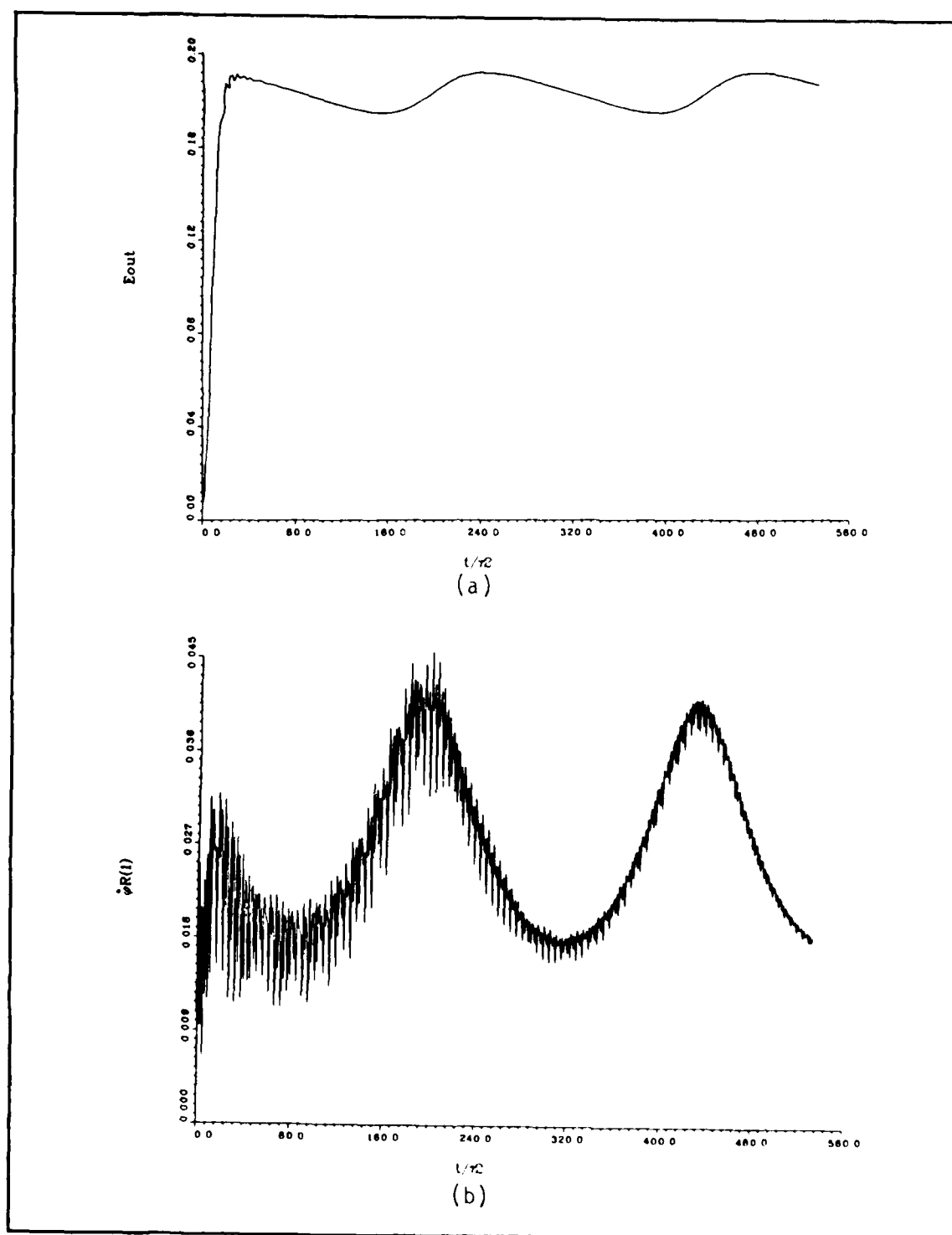
Figure 7.7. Injected laser output field with the injected signal strength below the locking threshold. r_B = 0.70 , I_{IN} = 2.50 \times 10^{-5} , \Delta\hat{m} = 0.0 , and \Delta\hat{s} = 0.005 . All other parameters are taken from data set 27. I_{IN}|_{th} = 1.661 \times 10^{-4} . (a) \hat{E}_{out} vs \hat{t} . (b) \hat{\phi}_R(1) vs \hat{t} .
