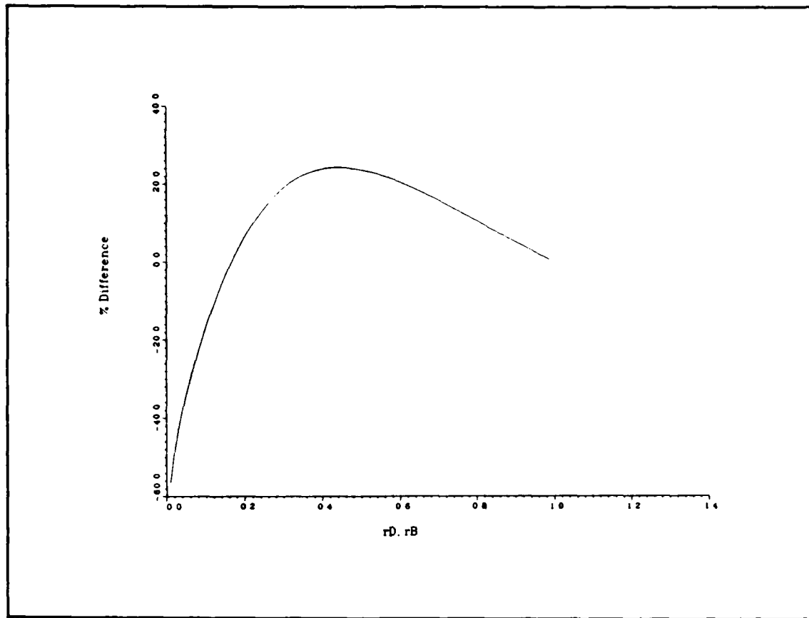
Figure A.4. Percentage difference in the losses L_D and L_L vs mirror reflectivity. The percentage difference is defined as (L_D - L_L)/L_L .
