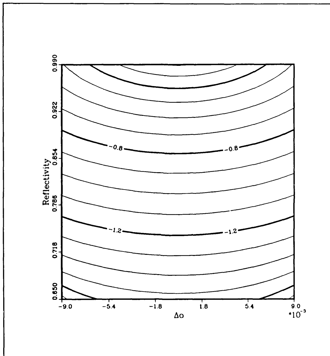
Figure C.1. \log_{10} I_R(0) contours at the MII point (data set 27).
