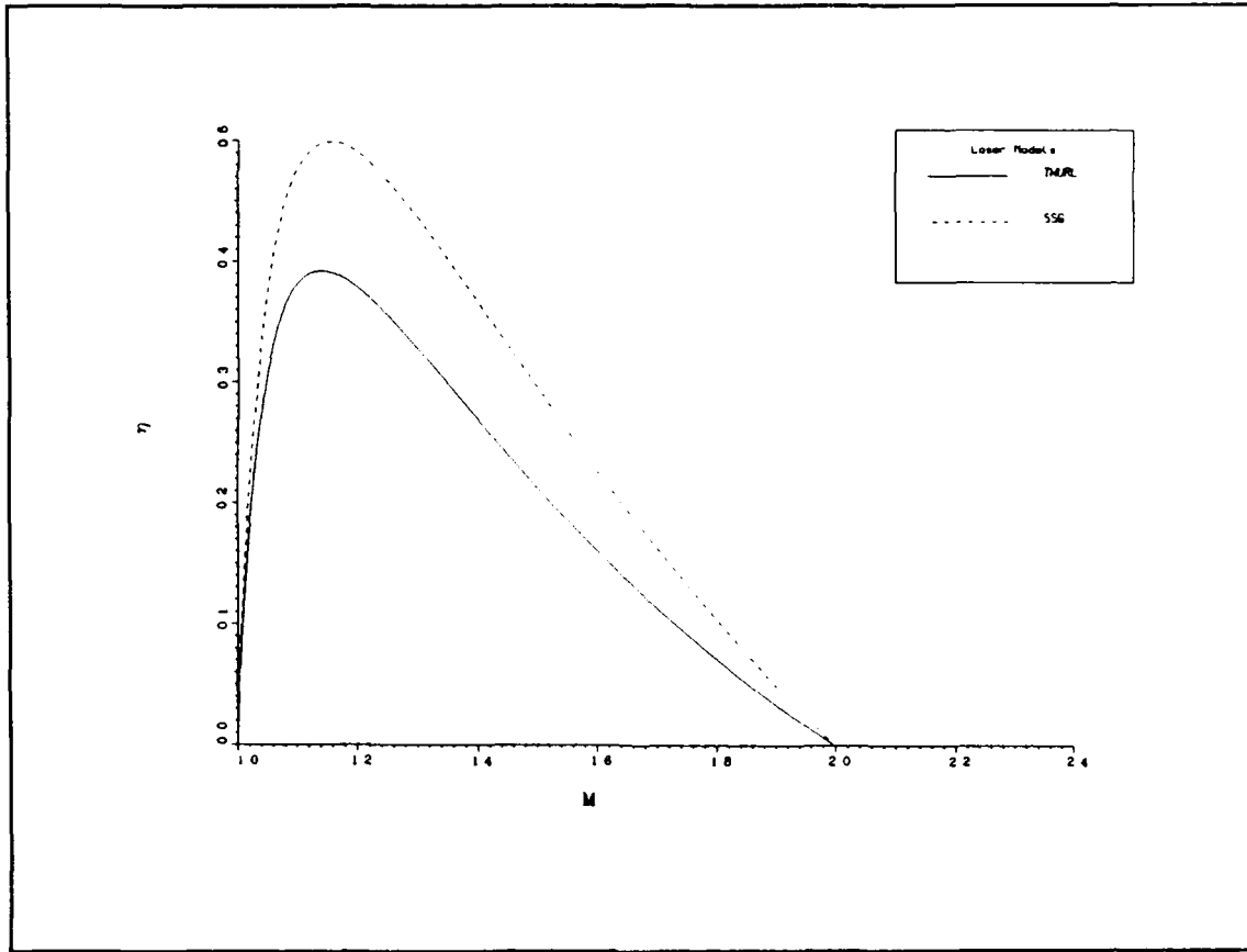
Figure 8.3. \eta_L vs M for the TWURL and simple saturable gain models. All parameters are the same as in Figure 8.2.
