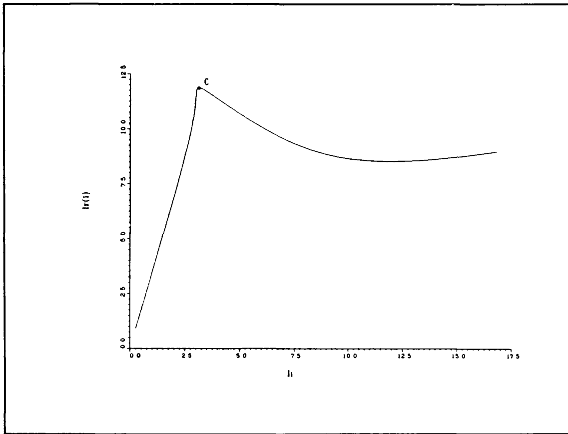
Figure 7.4. Near-vertical cusp. In this plot, \hat{r}_1 = 1.0 , \hat{r}_2 = 10^{10} , \hat{r}_3 = 1.0 , \Delta\hat{r} = 0.0 , \Delta\hat{\sigma} = 0.285 , r_A = 0.548 , r_B = 0.536 , and \hat{w}_{eq} = 17.0 . Turning point C is denoted on the plot.
