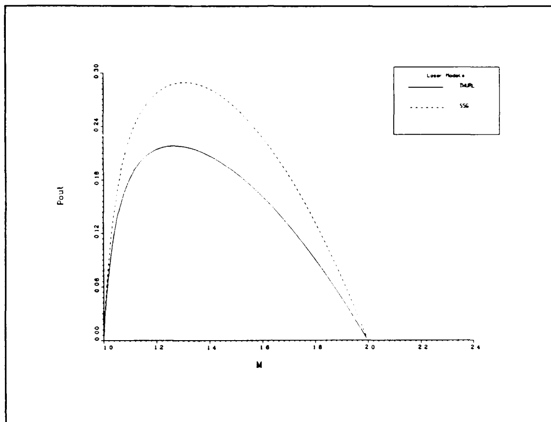
Figure 8.2. P_{out} vs M for the TWURL and simple saturable gain models. All parameters are from data set 15.
