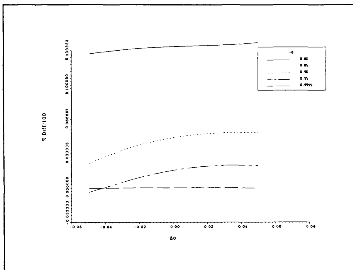
Figure 7.19. Percentage differences in I_R(0) and I_n , TWL and Spencer-Lamb models. Note that the differences increase as r_B decreases. Effects of varying |\Delta\delta| are not clear. The parameters are from data set 27.
