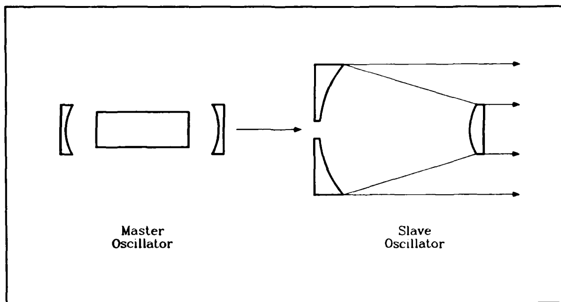
Figure 1.1. The basic concept of injection locking.
