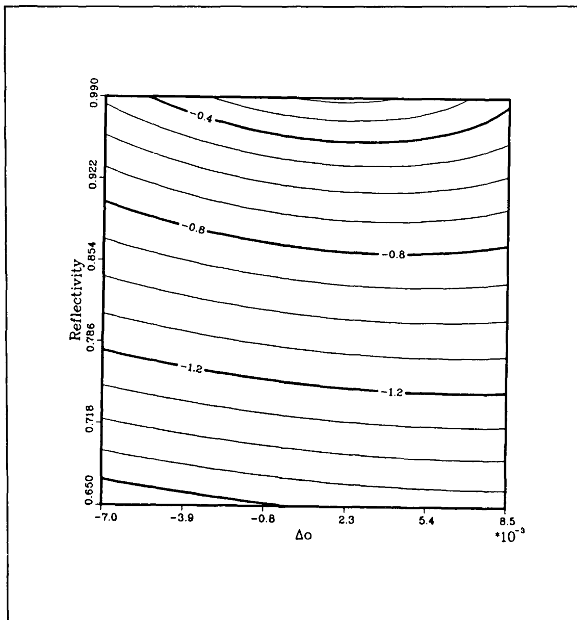
Figure C.4. \log_{10} I_R(0) contours at the MG1 point (data set 36).
