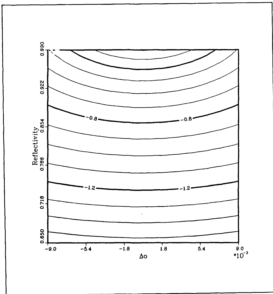
Figure C.3. \log_{10} I_R(0) contours at the MG1 point (data set 27).
