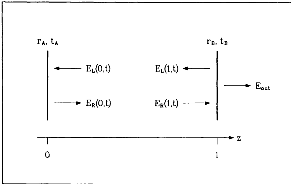
Figure 3.3. The boundary conditions for the free-running laser.
