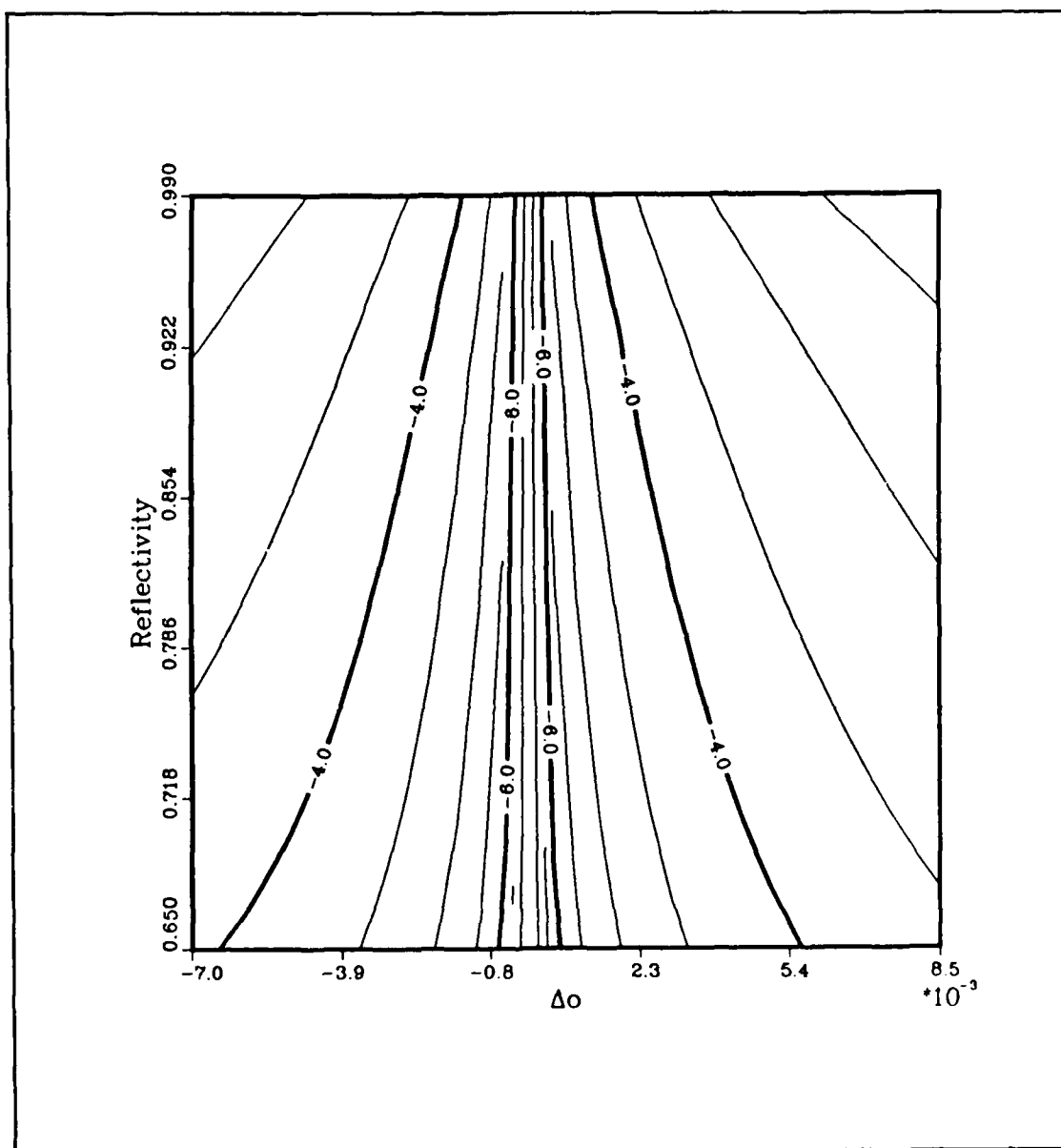
Figure C.23. \log_{10} I_I contours at the MG2 point (data set 36). The data is from the region in the (\Delta\hat{o}, r_D) plane where the cubic curves retain the s-shape.
