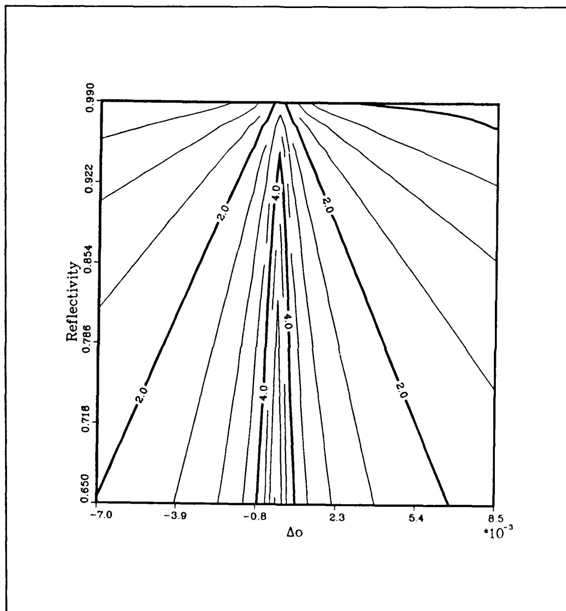
Figure C.40. \log_{10} G_1 contours at the MG2 point (data set 36). The data is from the region in the (\Delta\delta, r_D) plane where the cubic curves retain the s-shape.
