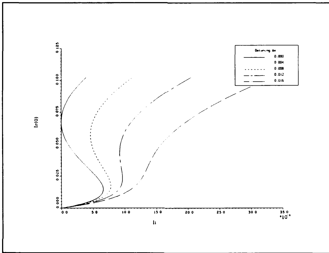
Figure 7.2. The cubic curves as functions of \Delta\delta . r_D = 0.75 and \Delta\hat{m} = 0.0 . All other parameters are taken from data set 27.
