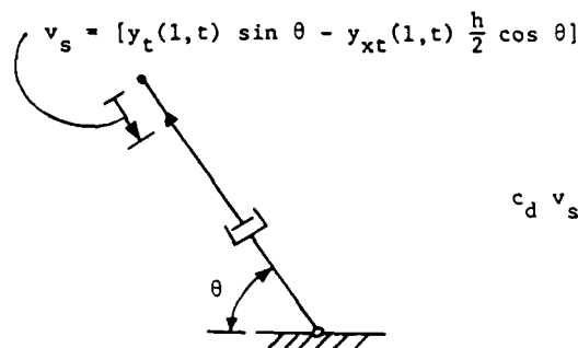
b) Shortening Velocity of Damper
