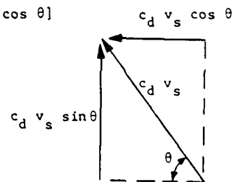
c) Damper Forces on Beam
