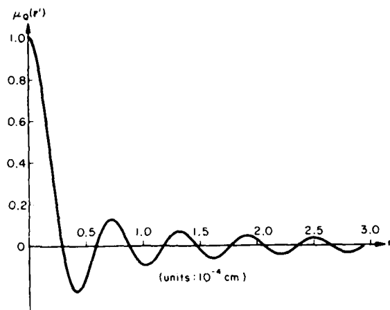
Fig. 1. The behaviour of the correlation coefficient \mu_Q(r') = [(\sin K_1 r')/K_1 r'] \exp(-r'^2/2\zeta^2) , with K_1 = 1.07 \times 10^5 \text{ cm}^{-1} , \zeta = 1.5 \text{ cm} [associated with curve (d) in fig. 2].
