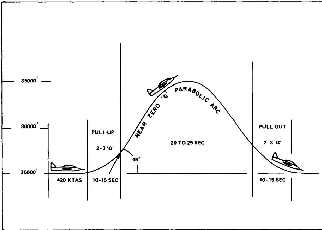
FIG. 1: ZERO "G" FLIGHT PROFILE
