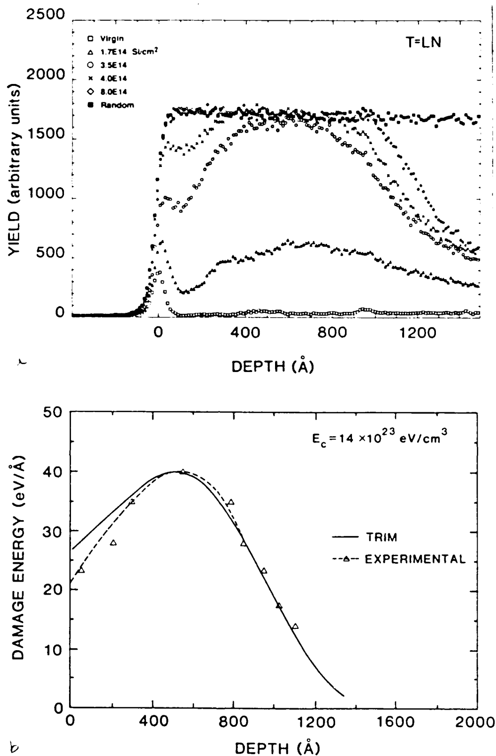
Fig. 6. (a) 2.0 MeV \text{He}^+ backscattering spectra for 87 keV LN Si-implanted \beta -SiC showing the accumulation of damage along [100] with increasing dose and (b) the corresponding comparison between TRIM and experimental damage energy profiles.
