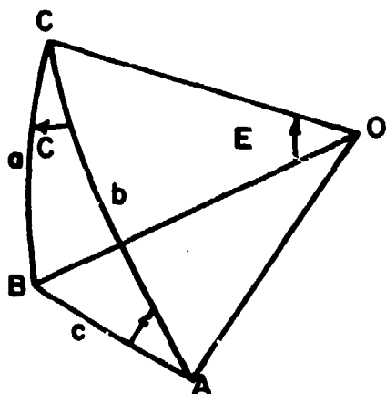
Figure B-3. Solving for Angle C .
