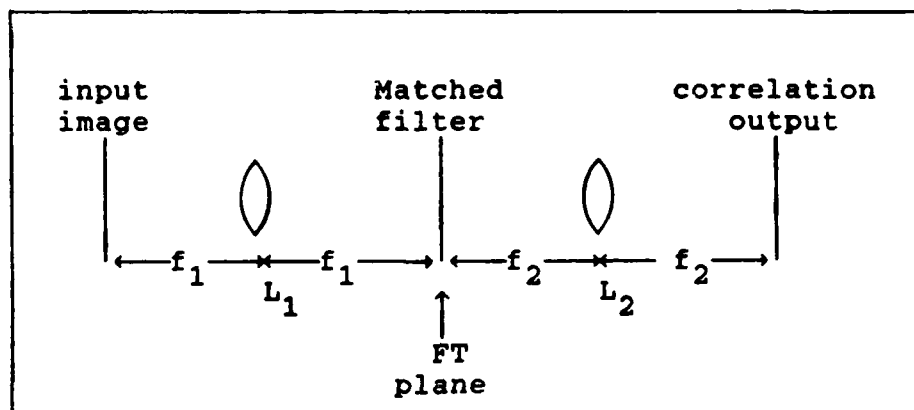
Figure 1.1. VanderLugt correlator
