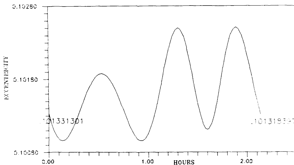
Change in Eccentricity Over One Orbital Period (6 X 0 Gravity Field)
