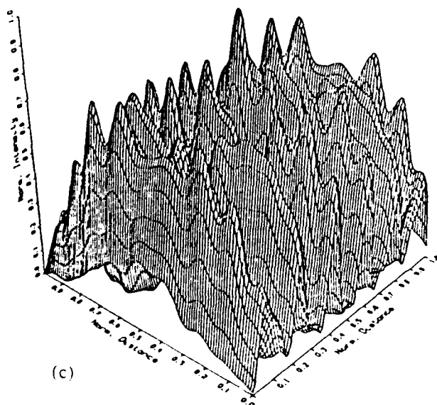
Figure 36. Lens 2 Comparison at \alpha = 10 Degrees (a) Experiment, (b) Goodman, (c) Walton, (d) FALCON
