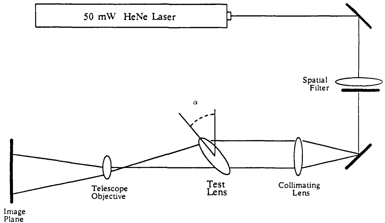
Figure 18. Experimental Set-Up
