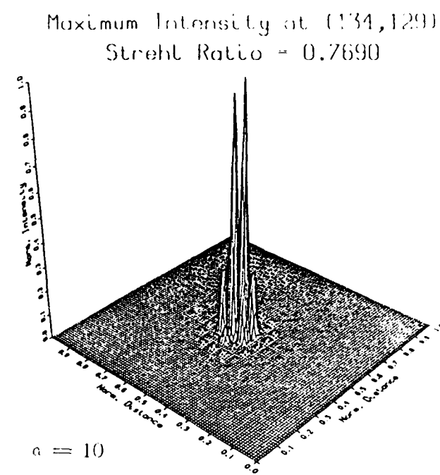
Figure 23. Goodman Lens 1 in Four Aperture Configuration
