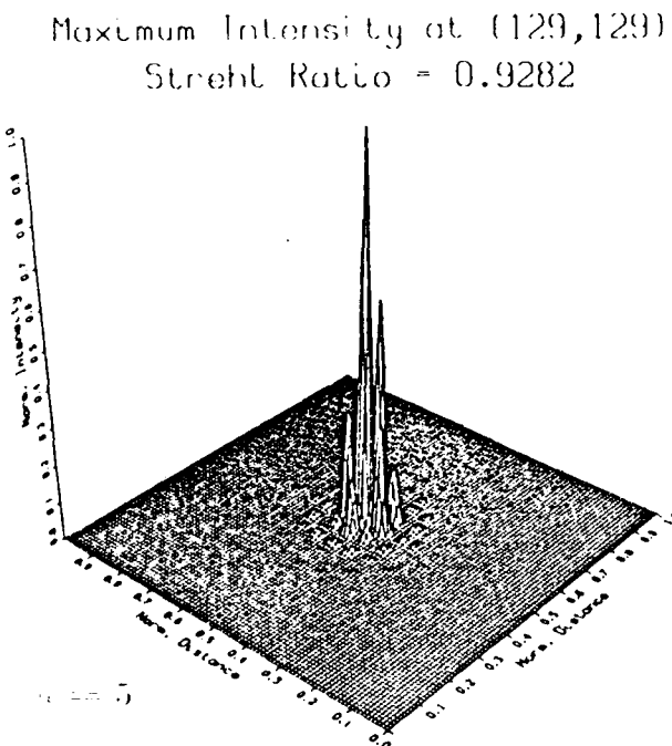
Figure 23. Goodman Lens 1 in Four Aperture Configuration
