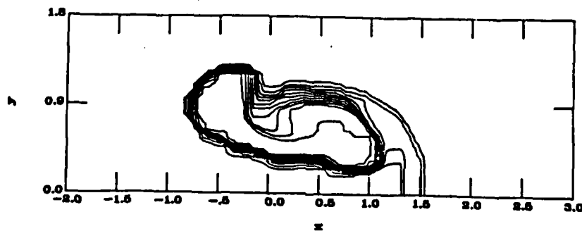
7. Density Contour Showing Separation of Hydrogen Masses.
