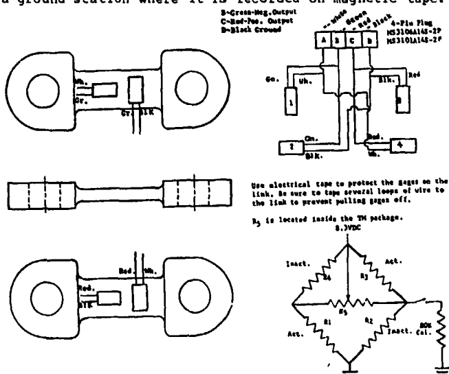
Figure 35 Typical Electrical Strain Gage Force Transducer
