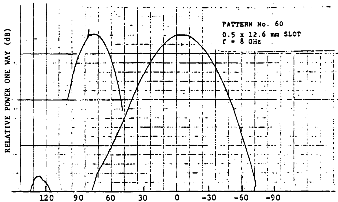
FIGURE 1.31 ANTENNA PATTERN: 0.5 X 12.6 MM SLOT AT 8.0 GHz
