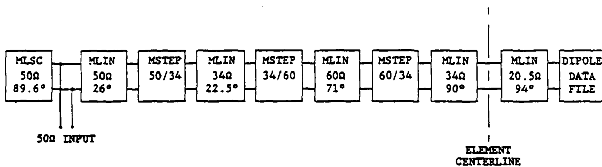
FIGURE 2.11 TOUCHSTONE EQUIVALENT CIRCUIT WITH REVISED INPUT
