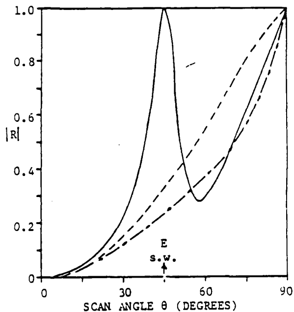
FIGURE 2.2 SCAN CHARACTERISTICS OF AN INFINITE PRINTED DIPOLE ARRAY. a = b = 0.5\lambda ; L = 0.39\lambda ; d = 0.19\lambda . w = 0.002\lambda ; \epsilon = 2.55 . E-PLANE —; H-PLANE ---; D-PLANE — —
