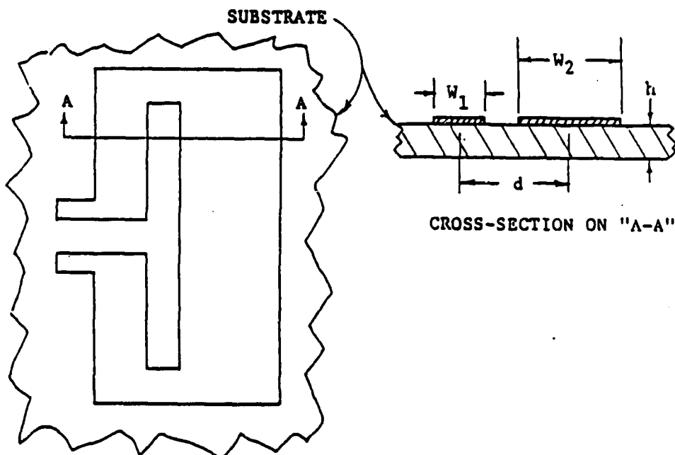
FIGURE 2.4b PARAMETERS OF MICROSTRIP FOLDED DIPOLE.
