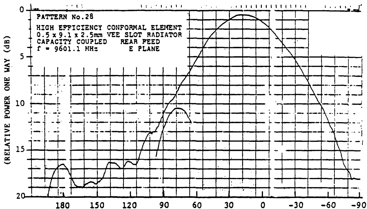
FIGURE 1.25 PATTERN OF 0.5 MM VEE SLOT ANTENNA SHOWN IN FIGURE 1.22 AT 9.607 GHz. MEASURED ANTENNA GAIN IS 5 dB.
