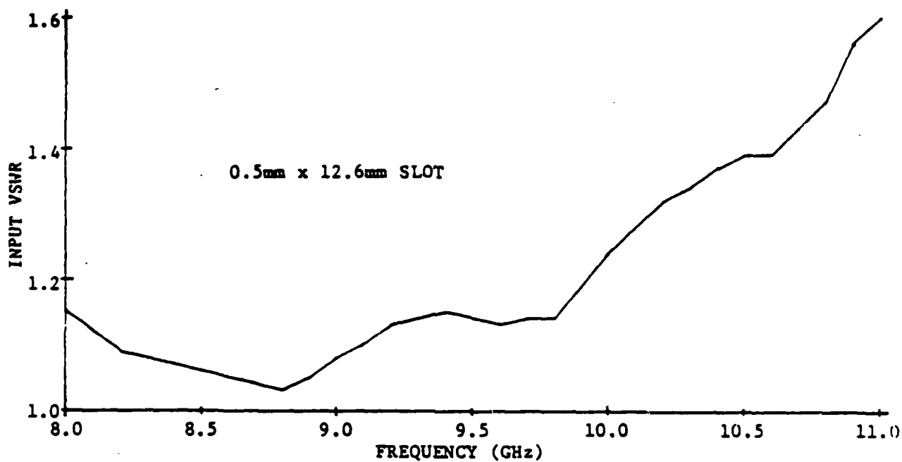
FIGURE 1.30 VSWR OF 0.5 X 12.6 MM SLOT RADIATOR USED IN PATTERN TESTS
