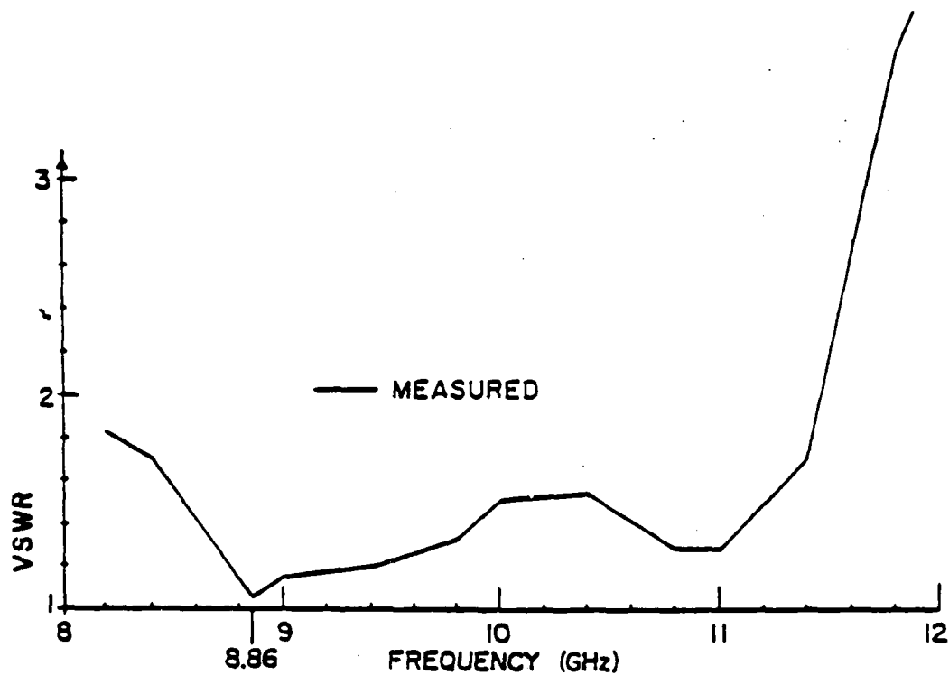
FIGURE 1.14 SINGLE X-BAND SLOT DIMENSIONS (in mm): h=0.79 , d=12.1 , W=2.99 , W_1=3.05 , S=0.1 ; \epsilon_r=2.2 .
