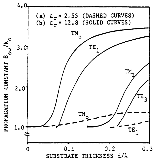
FIGURE 2.1* NORMALIZED SURFACE WAVE PROPAGATION FOR A GROUNDED DIELECTRIC SUBSTRATE: (a) \epsilon_r = 2.55 . (b) \epsilon_r = 12.8 *After Pozar and Schaubert, IEEE Trans. Antennas & Prop., Vol AP-32, June 1984.
