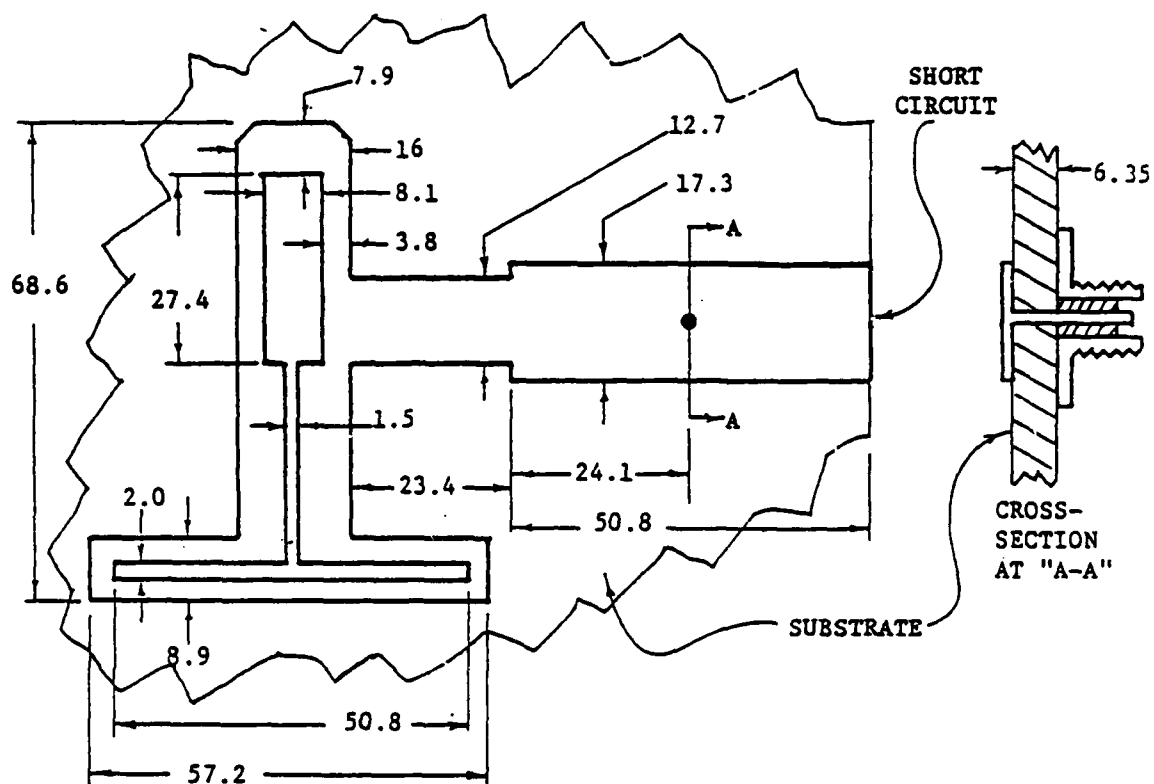
FIGURE 2.7 LAYOUT OF S-BAND FOLDED DIPOLE AT 2.25 GHz.
