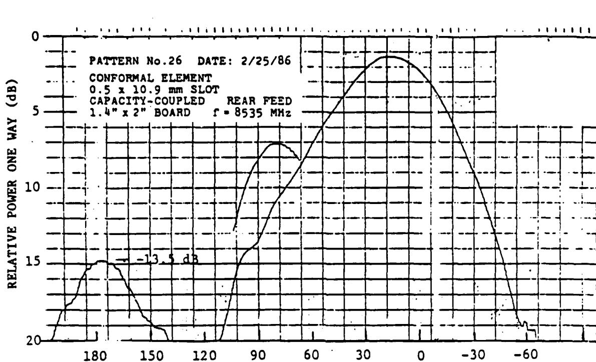
FIGURE 1.24 PATTERN OF 0.5 X 10.9 MM MICROSLLOT ANTENNA MEASURED AT 8.535 GHz. MEASURED ANTENNA GAIN IS +0.8 dBd.
