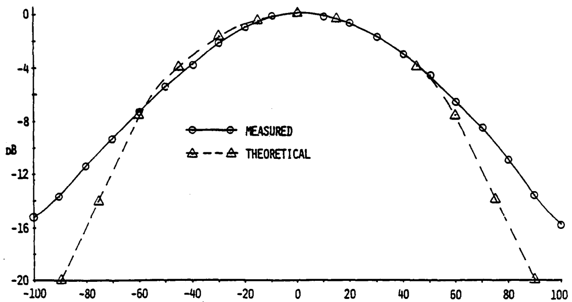
FIGURE 2.17 S-BAND E-PLANE PATTERN OF MICROSTRIP DUAL FOLDED DIPOLE
