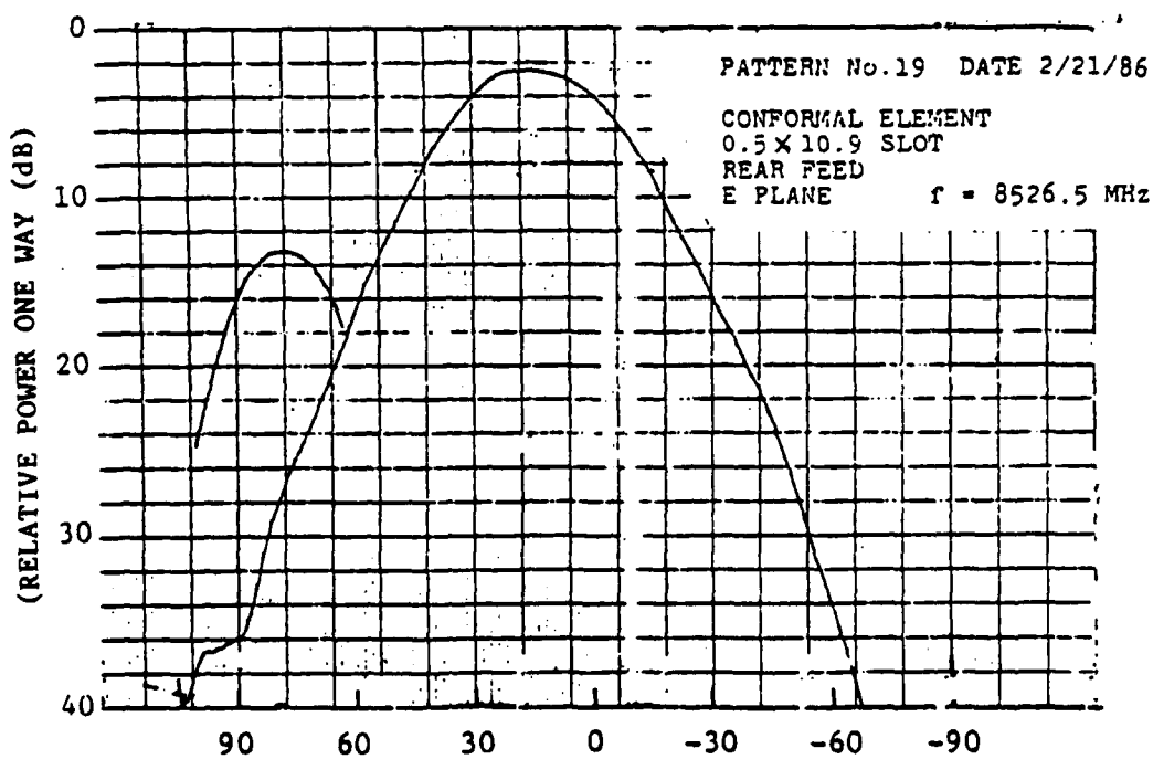
FIGURE 1.21 MICROSLLOT SHUNT RADIATOR: PATTERN WITH COAXIAL REAR-FEED THROUGH GROUND PLANE.
