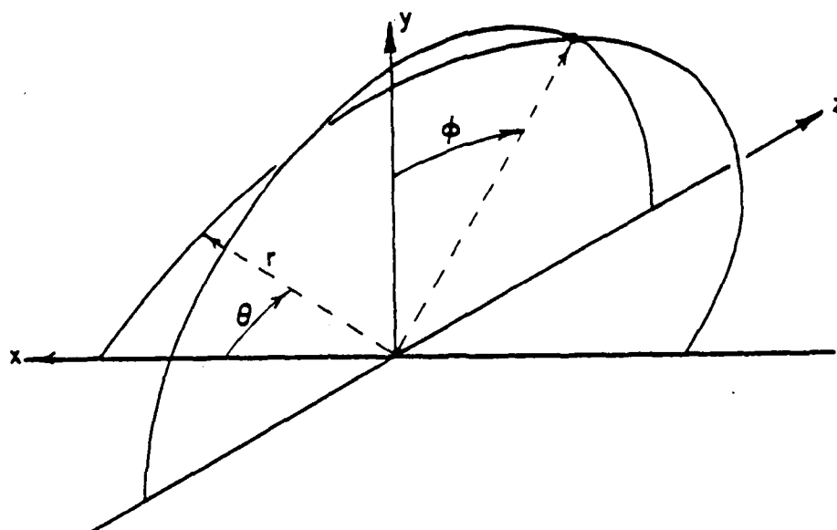
FIGURE 1.10 SPHERICAL COORDINATES IN THE FAR-FIELD ZONE
