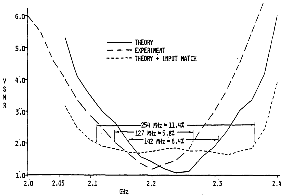
FIGURE 2.15 INPUT VSWR SUMMARY
