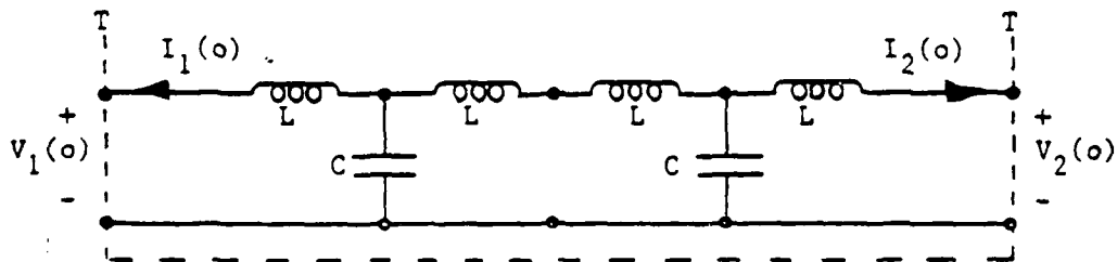
FIGURE 1.3 EQUIVALENT CIRCUIT OF TWO RIGHT-ANGLE BENDS AT THE END OF THE SLOT.
