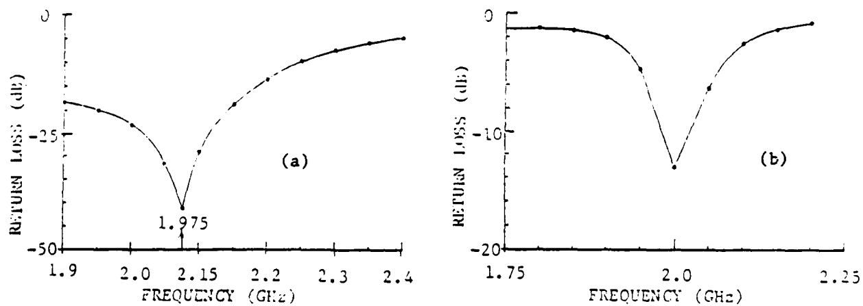
FIGURE 2.8 PREDICTED PERFORMANCE (a), AND MEASURED PERFORMANCE (b), OF S-BAND BALUN AND FOLDED DIPOLE.
