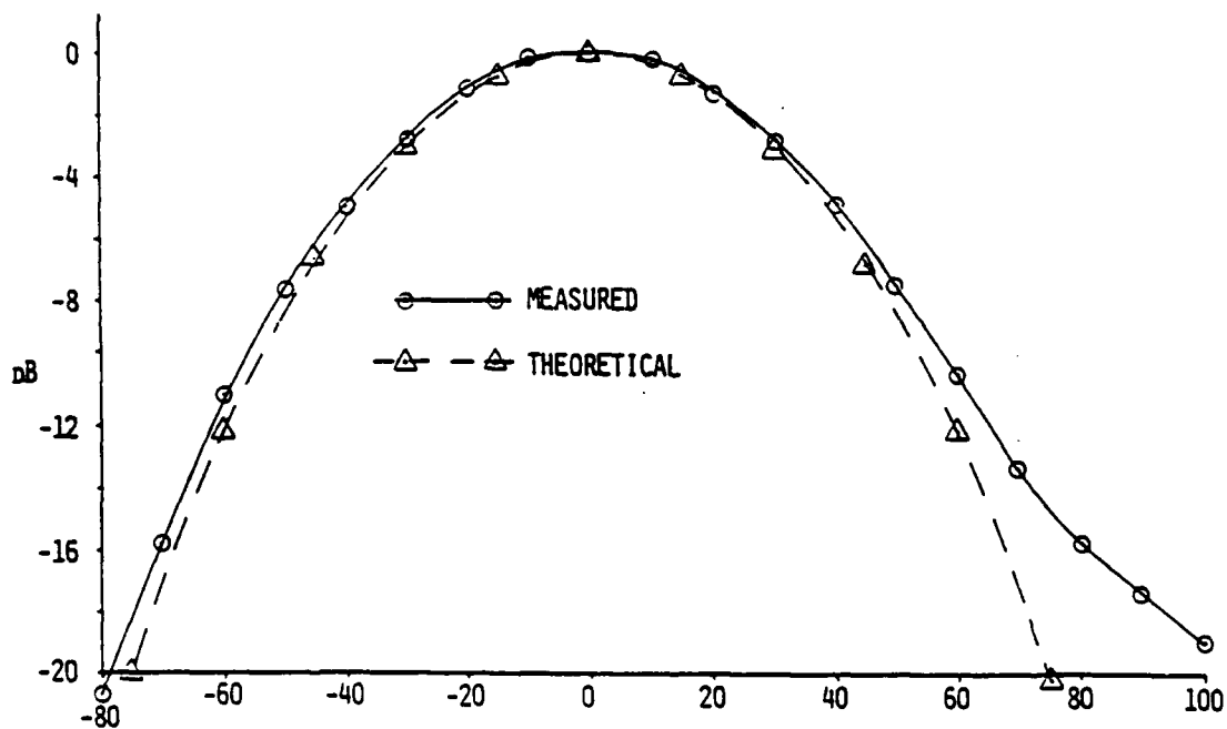
FIGURE 2.18 S-BAND H-PLANE PATTERN OF MICROSTRIP DUAL FOLDED DIPOLE
