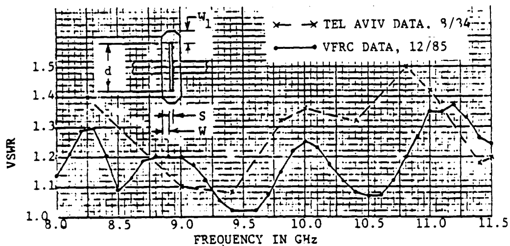
FIGURE 1.27 COMPARISON OF SINGLE X-BAND SLOT VSWR MEASUREMENTS AT TEL-AVIV UNIVERSITY AND AT VFRC. DIMENSIONS (in mm): d = 12.1 , w = .45 , w_1 = .90 , S = .1 , h = .79 , \epsilon_r = 2.2 .
