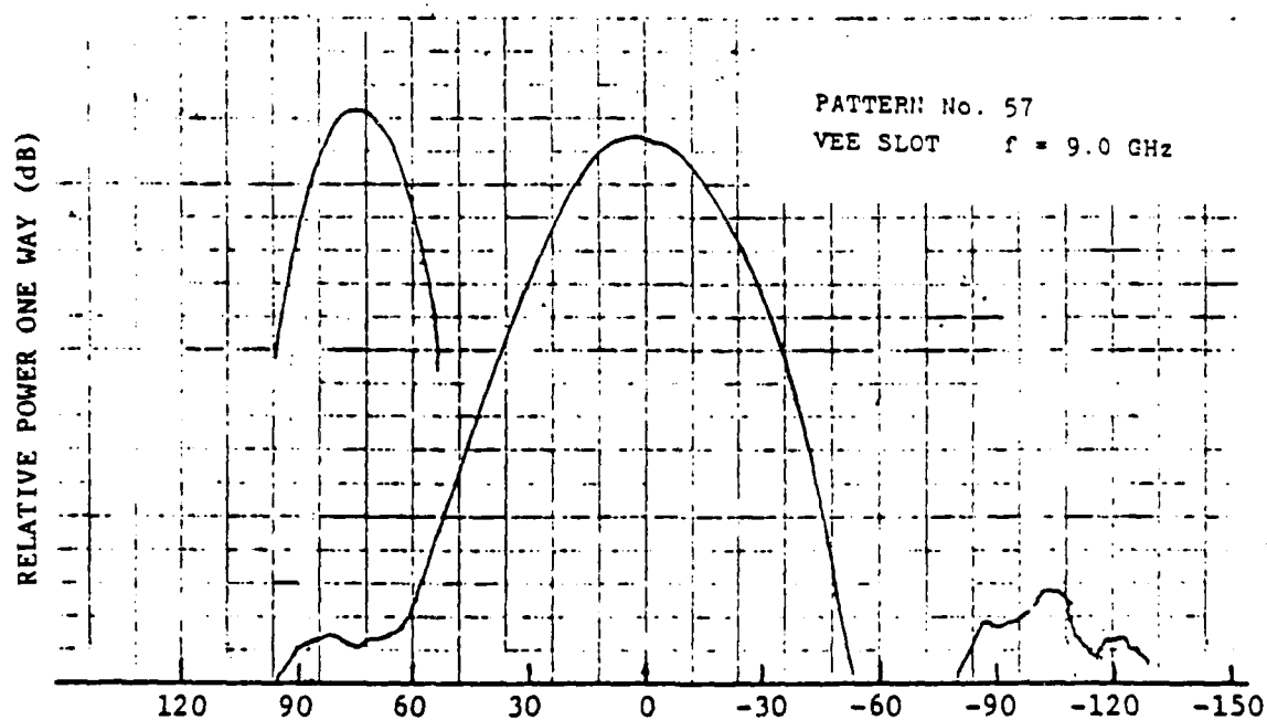
FIGURE 1.34 ANTENNA PATTERN: 0.5 MM VEE SLOT ANTENNA AT 9.0 GHz.
