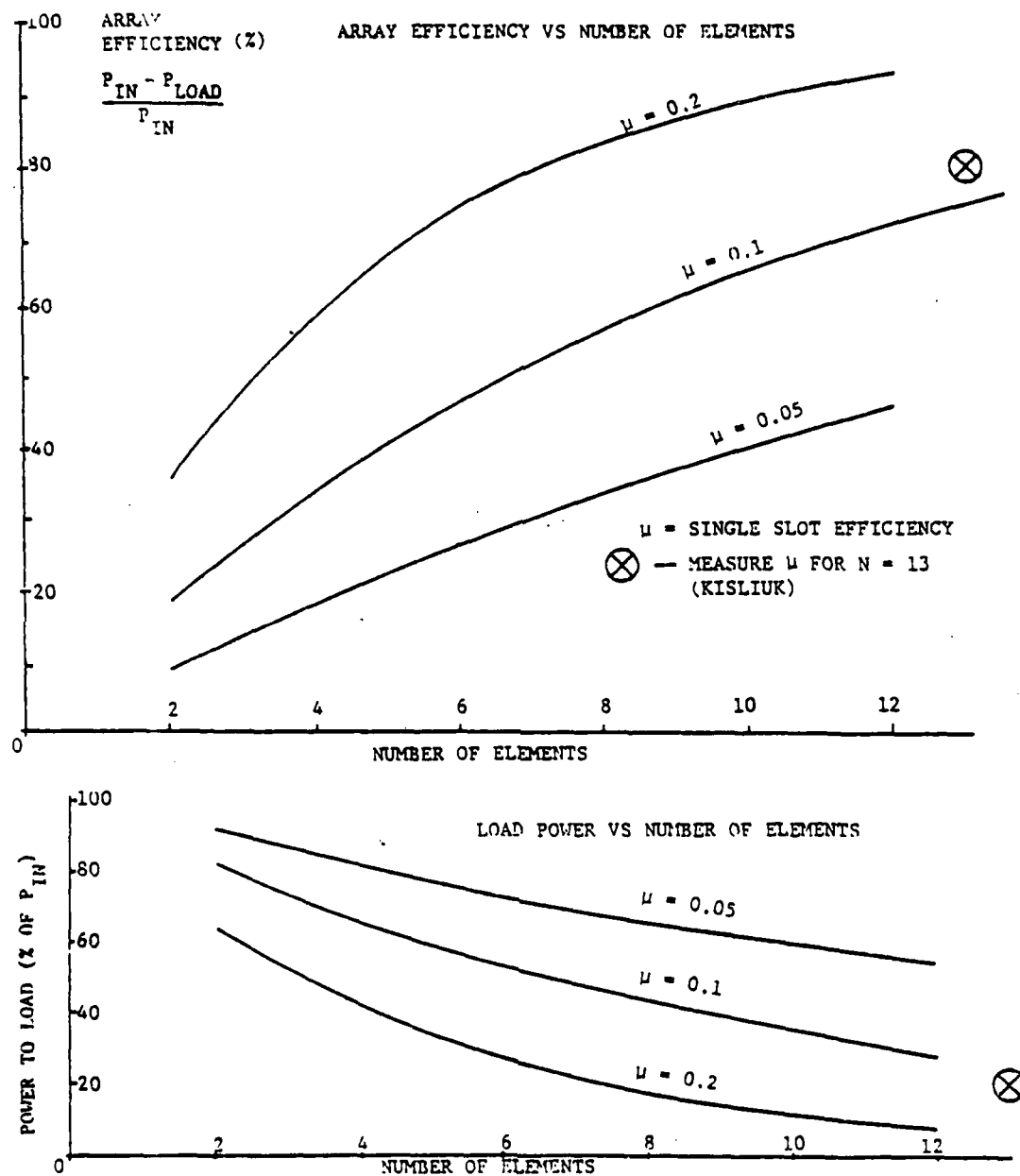
FIGURE 1.7 ARRAY POWER RELATIONS
