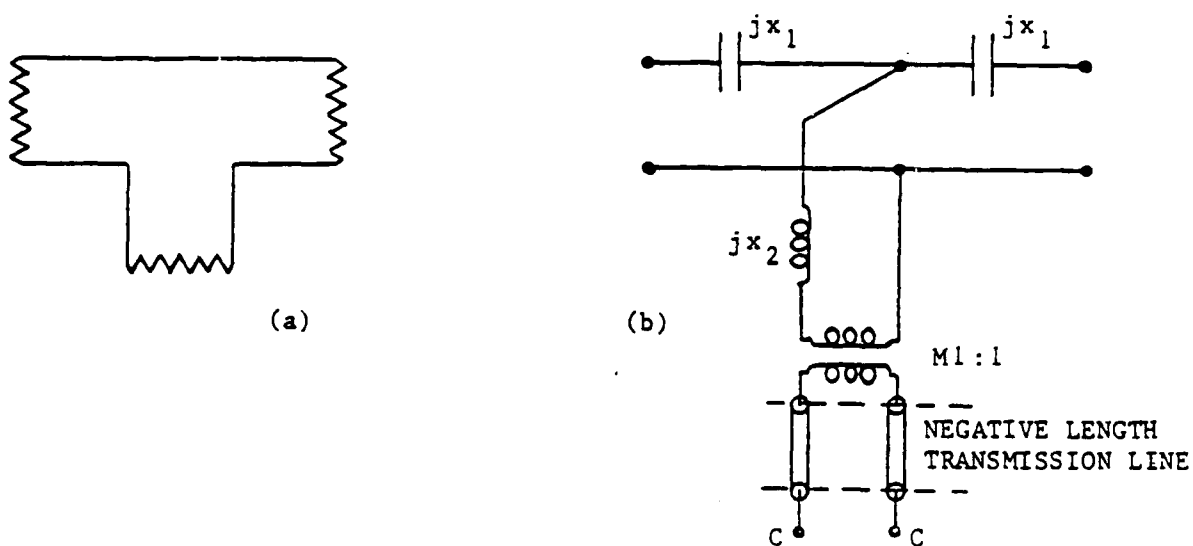
FIGURE 1.4 (a) TEE JUNCTION
