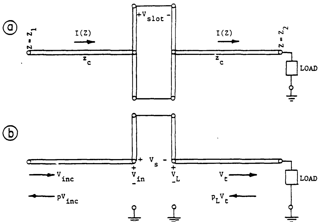
FIGURE 1.6 SIMPLIFIED EQUIVALENT CIRCUIT OF A MICROSTRIP MEANDER-LINE SLOT ANTENNA
