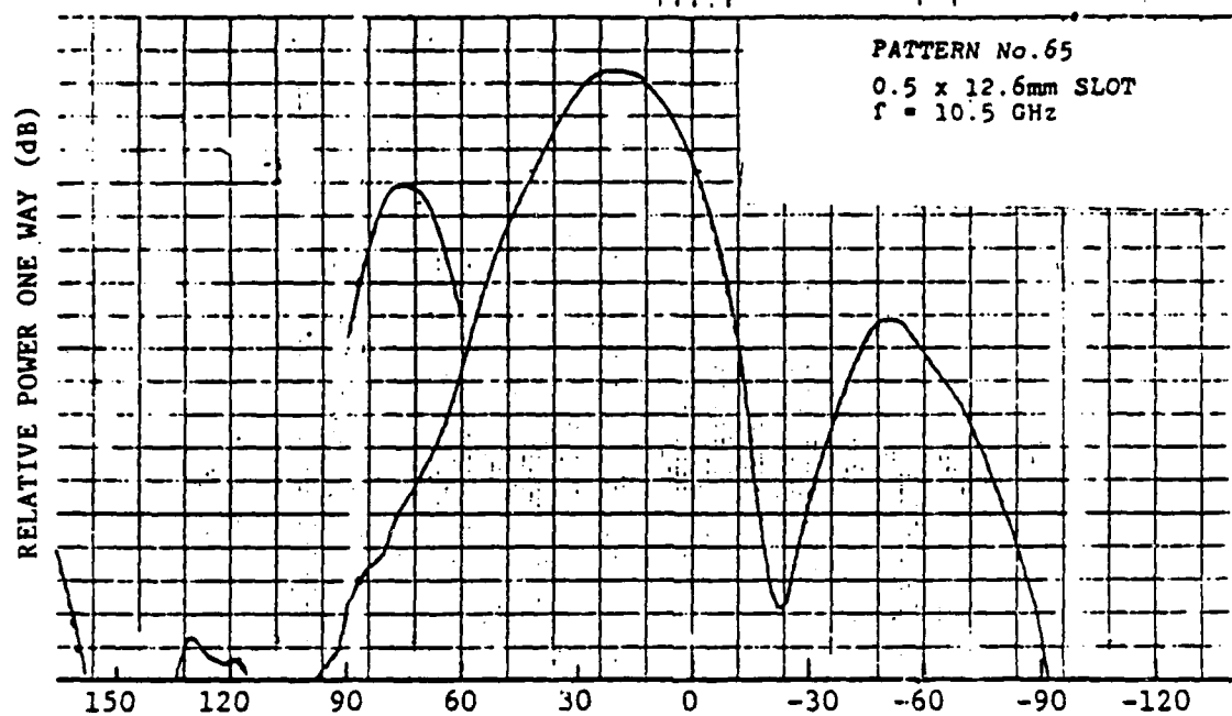
FIGURE 1.33 ANTENNA PATTERN: 0.5 X 12.6 MM SLOT AT 10.5 GHz.
