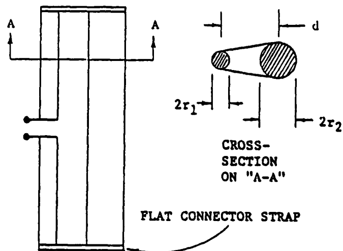
FIGURE 2.4a PARAMETERS OF ROUND-CONDUCTOR FOLDED DIPOLE.
