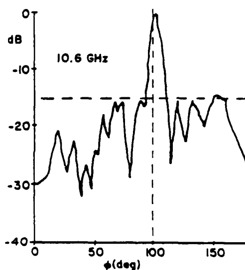
FIGURE 1.16 E-PLANE RADIATION PATTERNS OF THE SLOT ARRAY SHOWN IN FIGURE 1.15.
