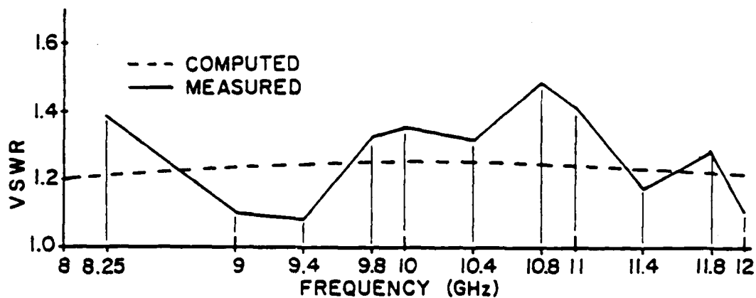
FIGURE 1.13 SINGLE X-BAND SLOT, COMPUTED AND MEASURED. DIMENSIONS (in mm): h=0.79 , d=12.1 , W=0.45 , W_1=0.98 , S=0.1 , \epsilon_r=2.2 .
