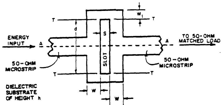
FIGURE 1.1 MICROSTRIP-FED RADIATING SLOT (UPPER VIEW).
