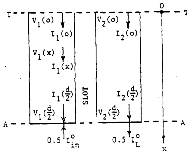
FIGURE 1.2 COUPLED MICROSTRIP LINES MODELING HALF OF THE SLOT.
