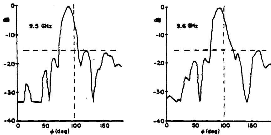
FIGURE 1.18 E-PLANE RADIATION PATTERNS OF THE 10-SLOT ARRAY OF FIGURE 1.17.
