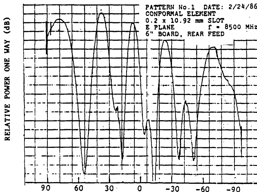
FIGURE 1.28 ANTENNA PATTERN OF 0.5 X 12.6 MM MICROSLLOT ON 15.3 CM DIELECTRIC SUBSTRATE. \epsilon_r = 2.2 , CONNECTORS BEHIND GROUND PLANE.
