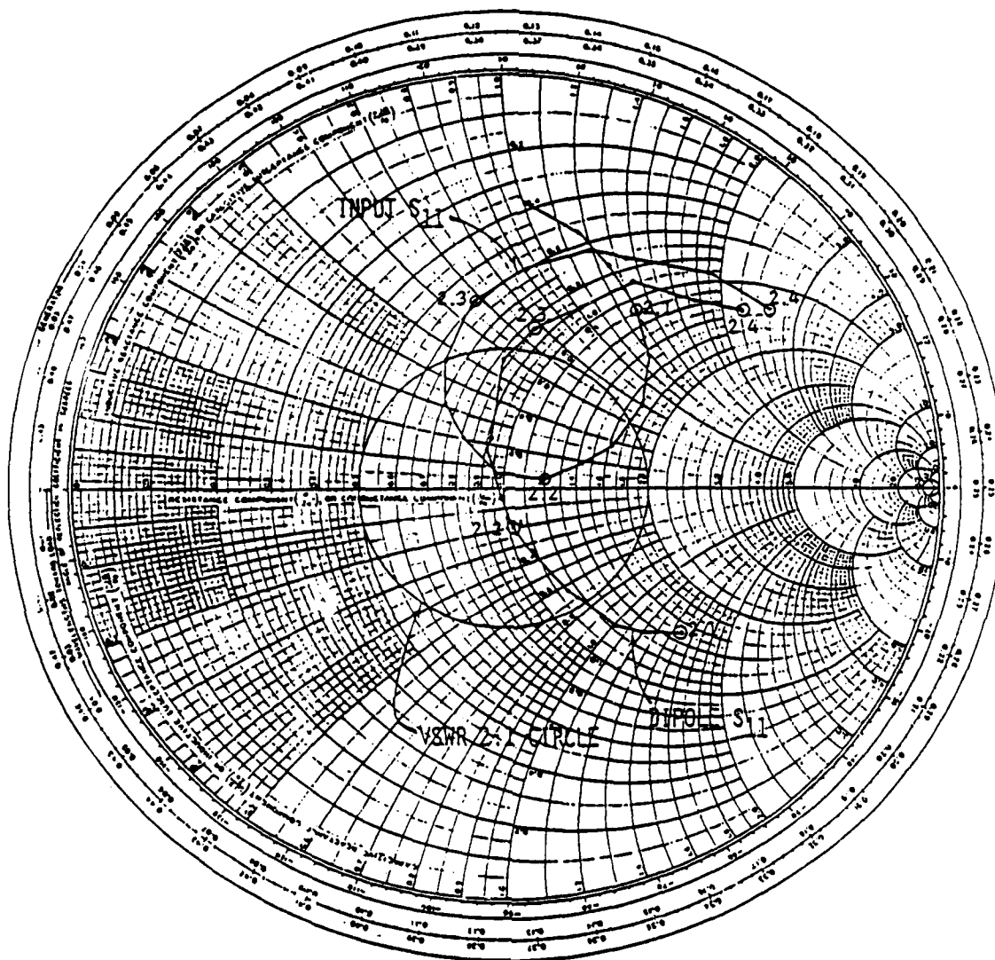
FIGURE 2.12 ANTENNA AND DIPOLE INPUT IMPEDANCES
