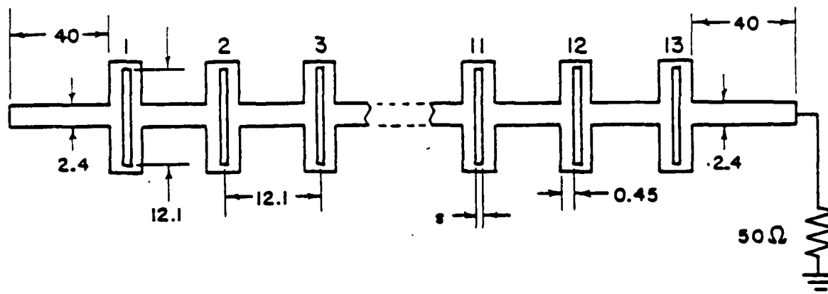
FIGURE 1.15 13-SLOT ARRAY. THE WIDTH OF THE SLOTS IS TAPERED.
