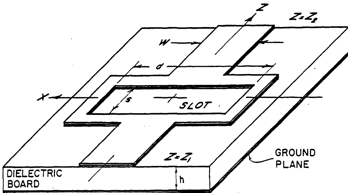
FIGURE 1.9 THE MICROSTRIP SLOT ANTENNA.
