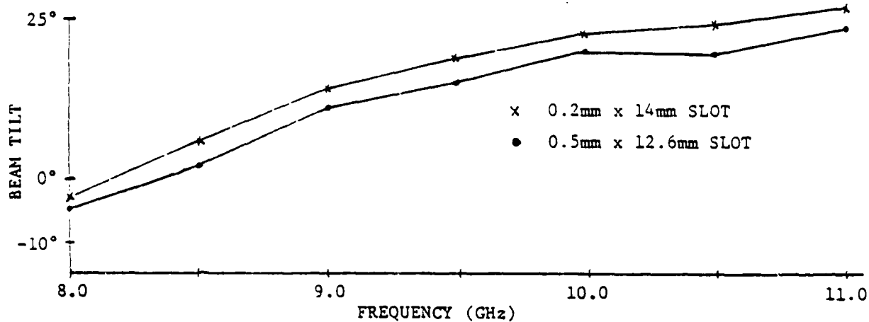
FIGURE 1.35 GAIN AND BEAM TILT VS FREQUENCY GRAPHS FOR 0.5 X 12.6 MM AND 0.2 X 14 MM MICROSTRIP SLOTS AND 0.5 MM VEE SLOT RADIATORS.
