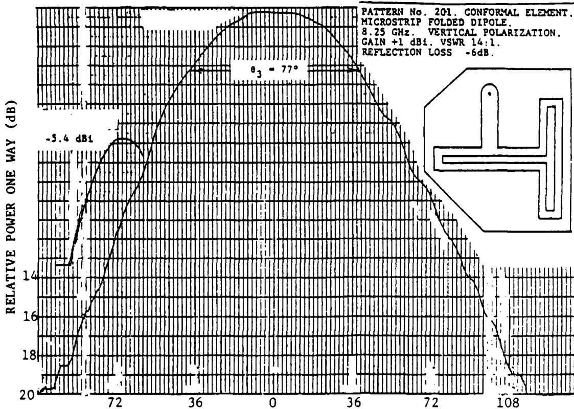
FIGURE 2.6 H-PLANE PATTERN, FOLDED DIPOLE + BALUN AT 8.25 GHz.
