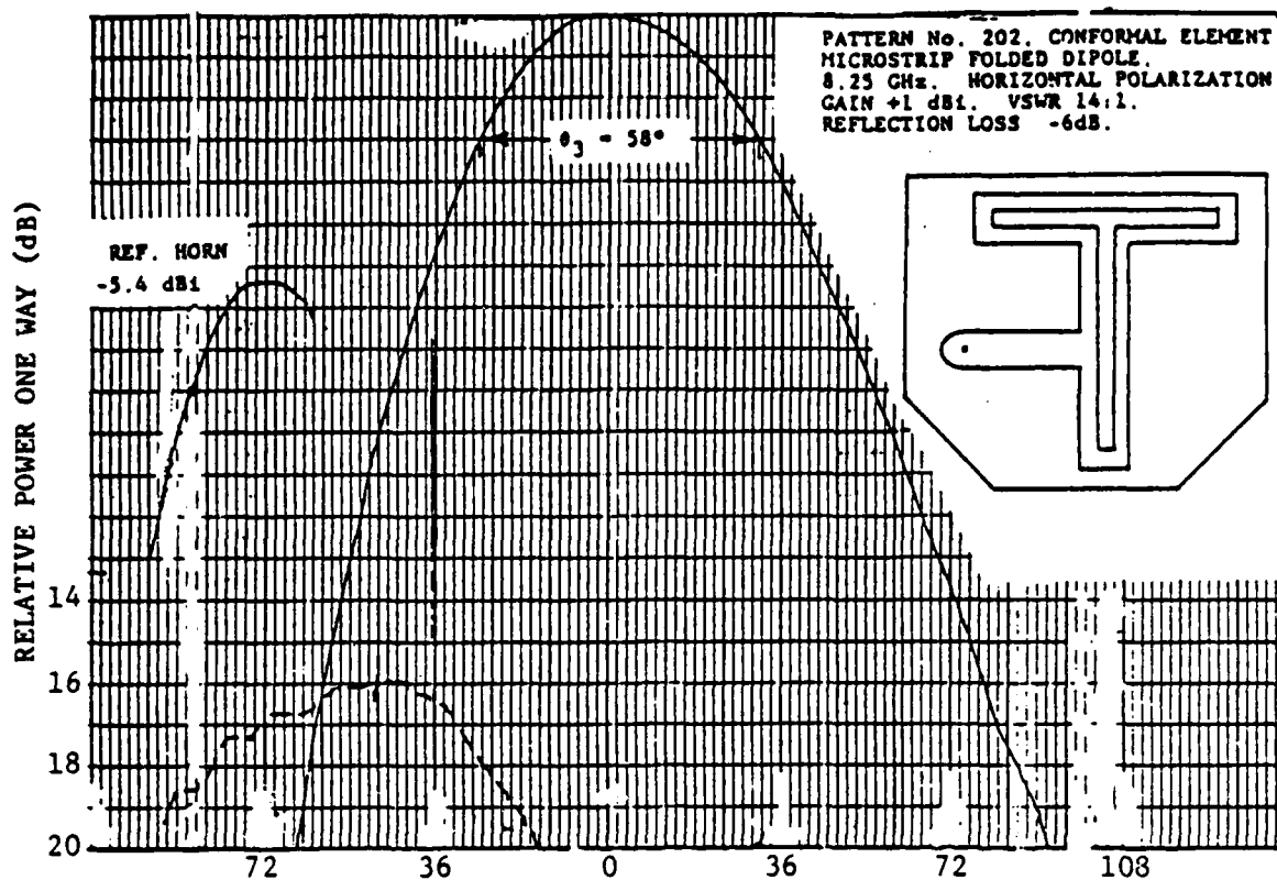
FIGURE 2.5 E-PLANE PATTERN, FOLDED DIPOLE + BALUN AT 8.25 GHz.
