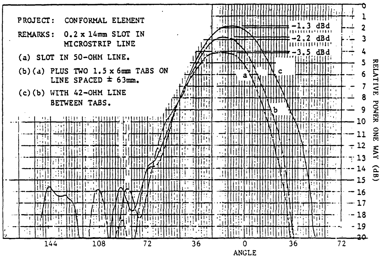
FIGURE 1.36 COMPARISON OF ANTENNA PATTERNS OF THREE MICROSTRIP SLOT RADIATORS.
