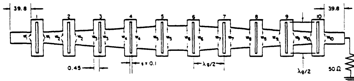
FIGURE 1.17 10-SLOT ARRAY. THE WIDTH OF MICROSTRIP LINES FEEDING THE SLOTS IS TAPERED.
