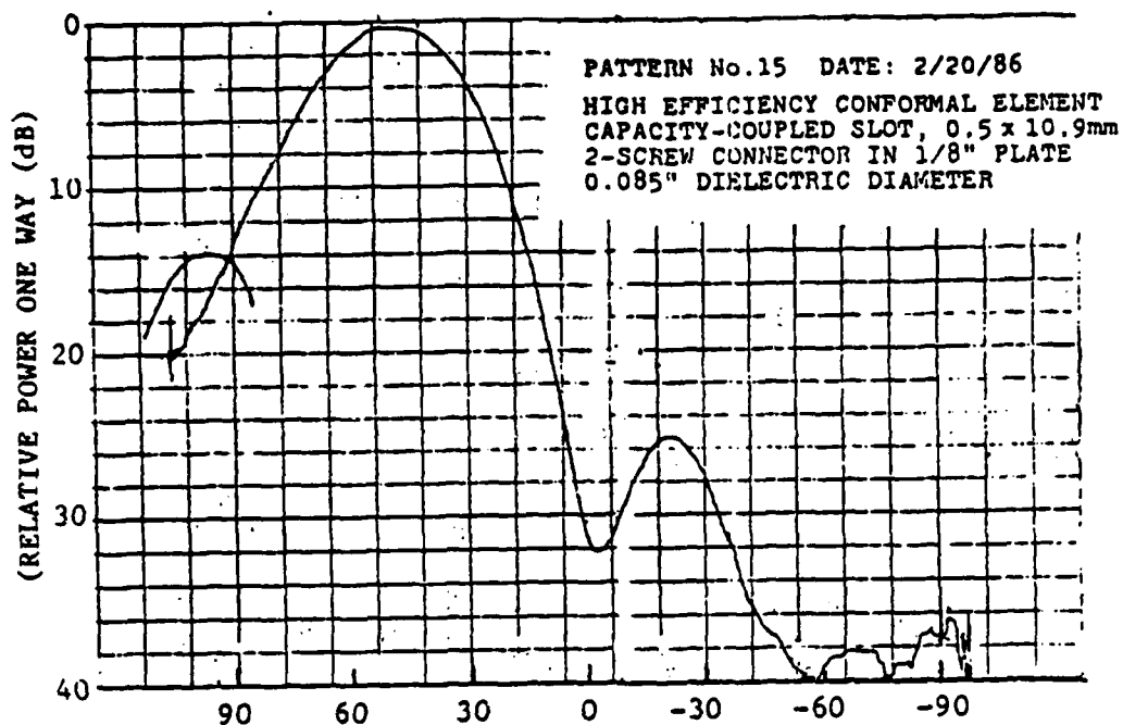
FIGURE 1.20 MICROSLLOT SHUNT RADIATOR: PATTERN WITH COAXIAL EDGE-BOARD FEED.
