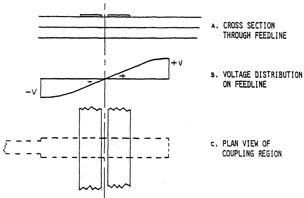
FIGURE 2.10 TRANSFORMER COUPLING
