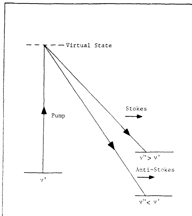
Figure 16. Raman Scattering Diagram
