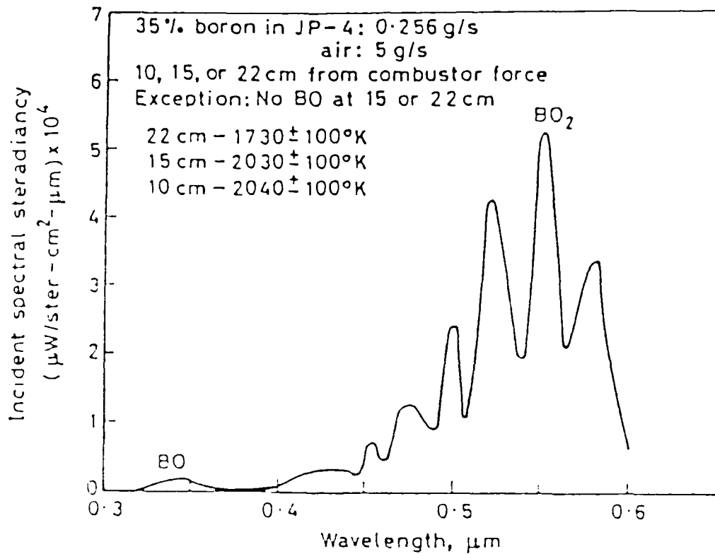
Figure 5. Boron Oxide Fluctuation Bands (10:96)
