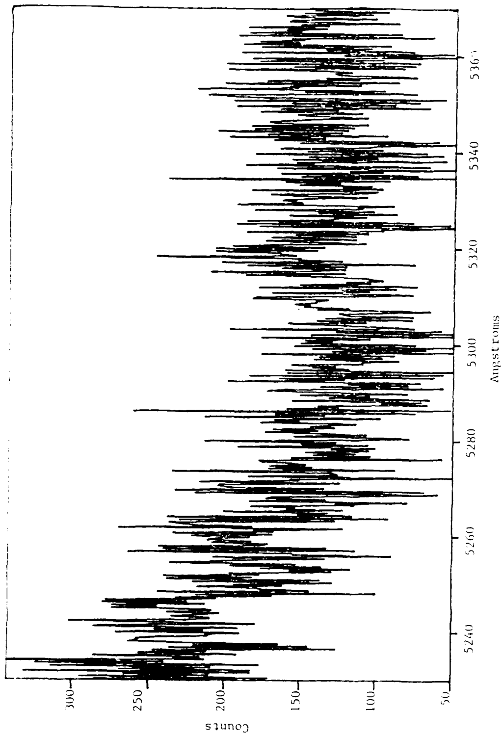
Figure 38. Induced Fluorescence, 5230-5370 Å
