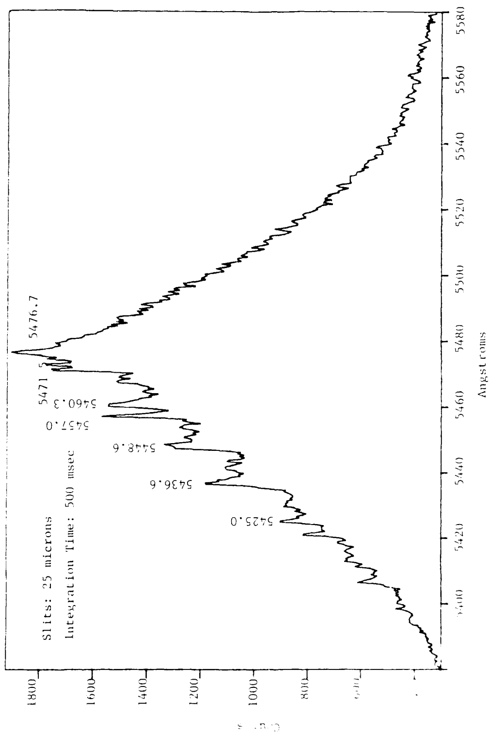
Figure 21. Flame Emission, 5380-5580 Å
