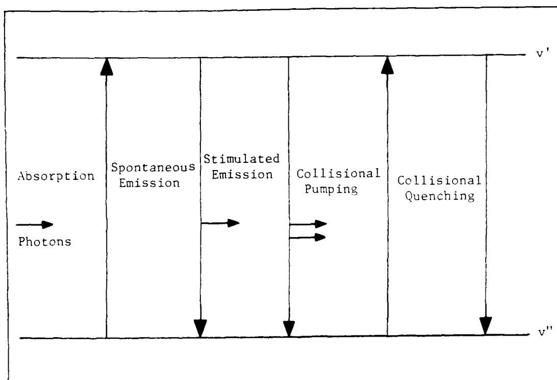
Figure 2. Energy Change Processes
