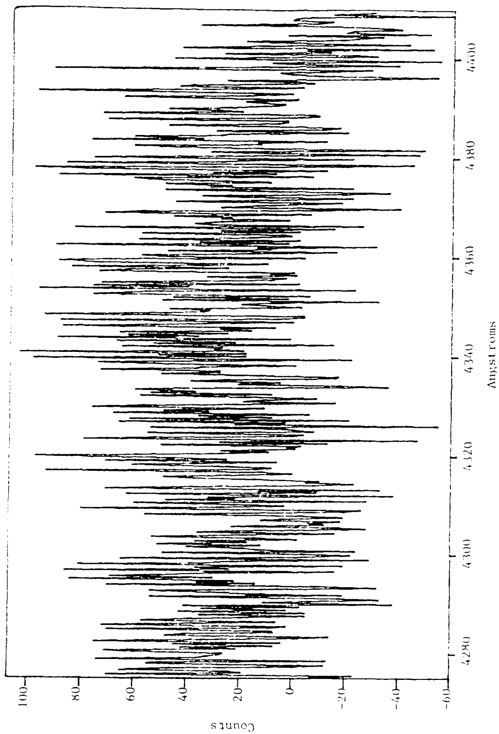
Figure 46. Induced Fluorescence, 4275-4405 Å
