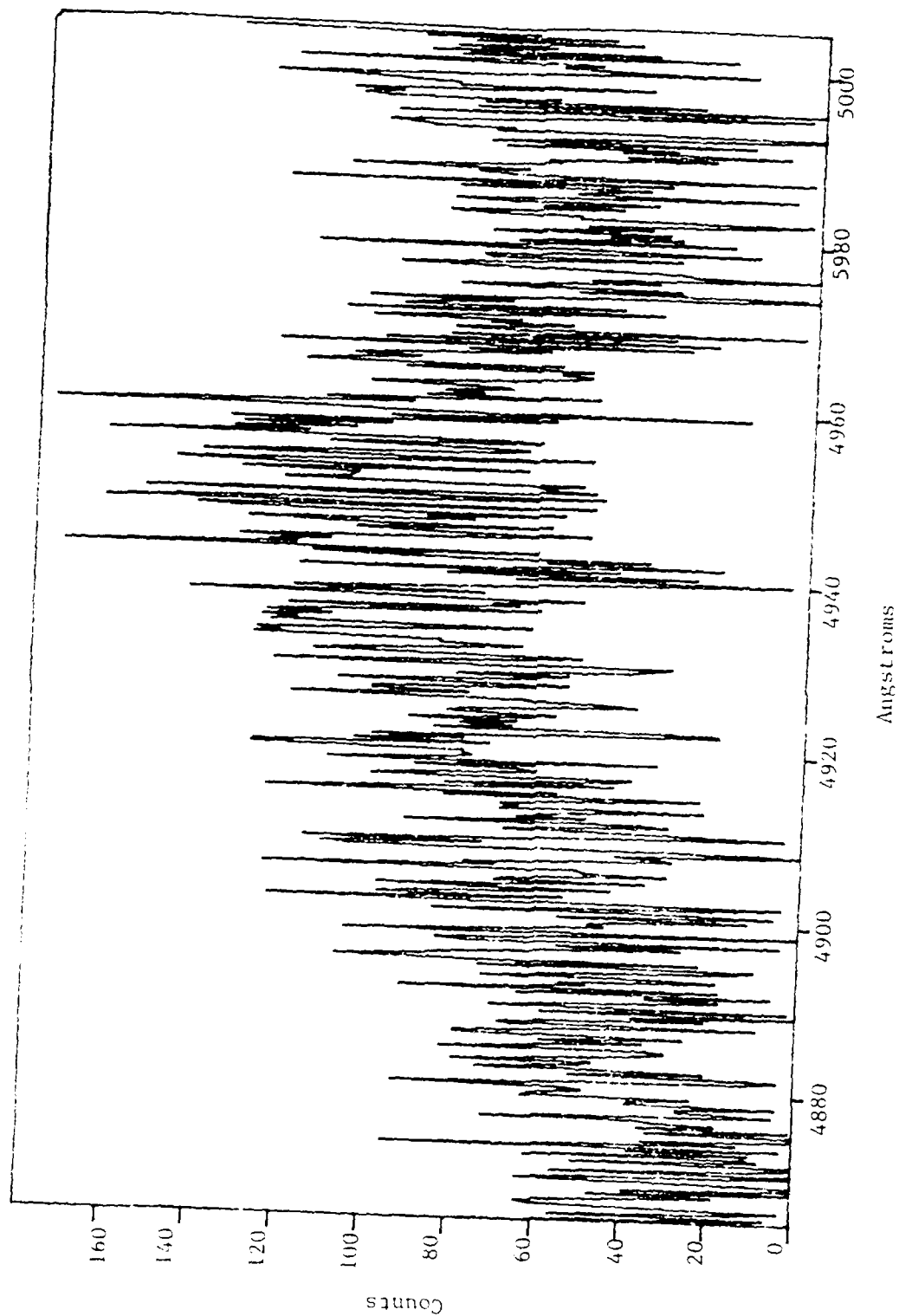
Figure 41. Induced Fluorescence, 4860-5000 Å
