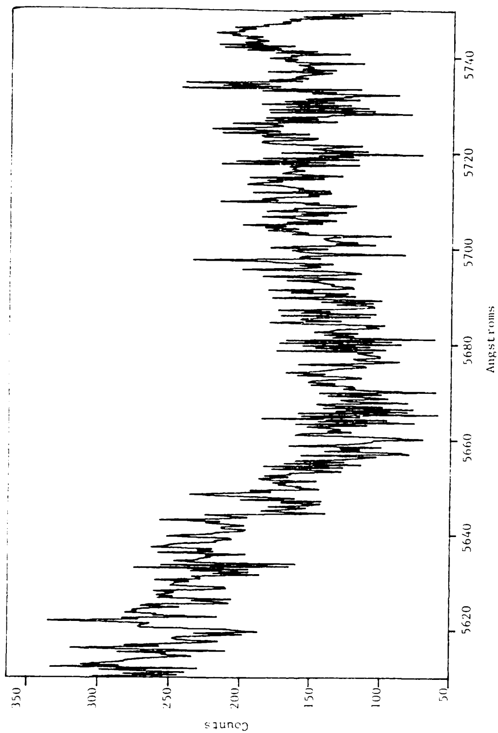
Figure 35. Induced Fluorescence, 5610-5750 Å
