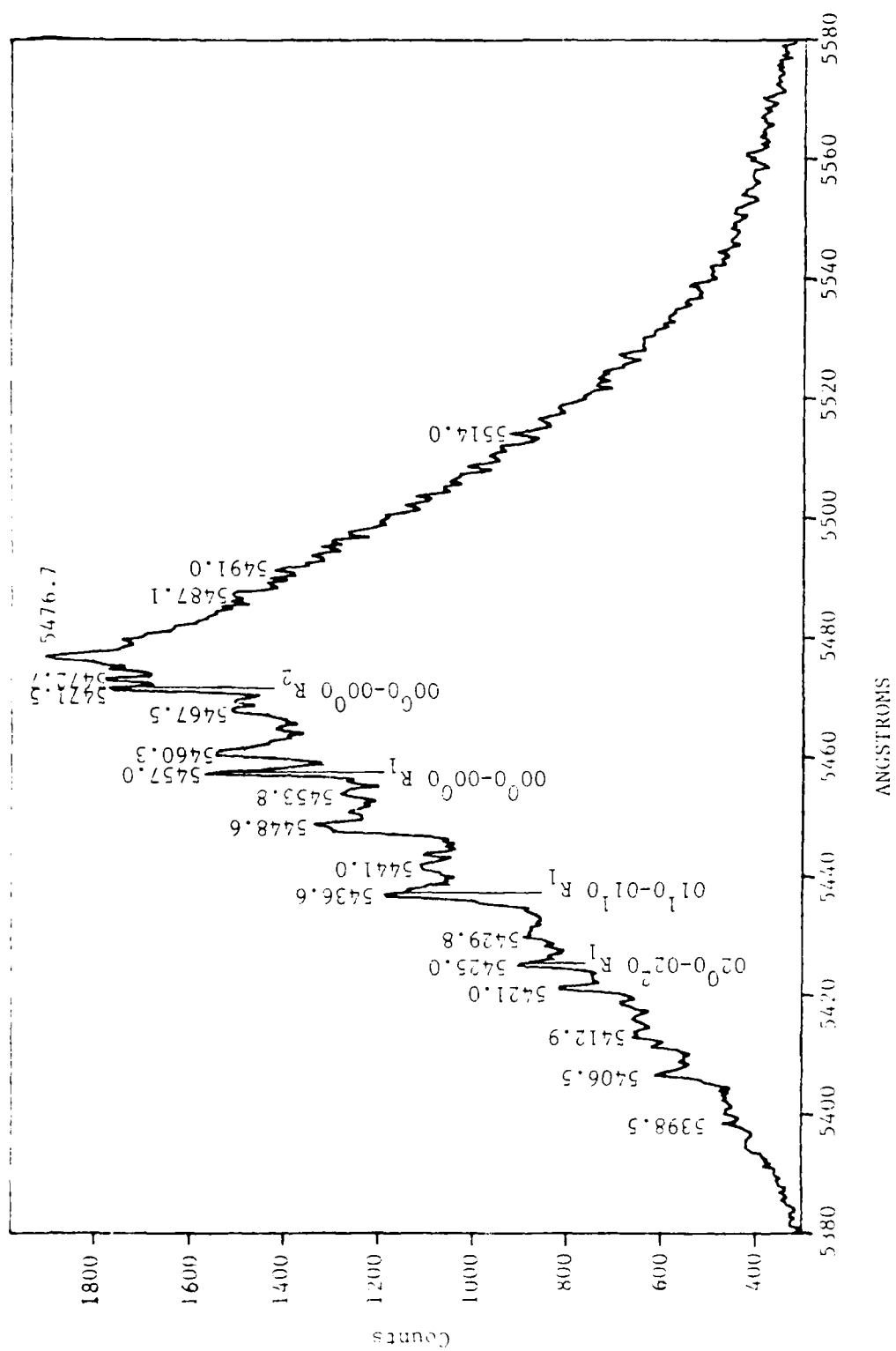
Figure 6. Emission From 0^0_0-0^0_0 Bandhead Region of A-X System of \text{BO}_2
