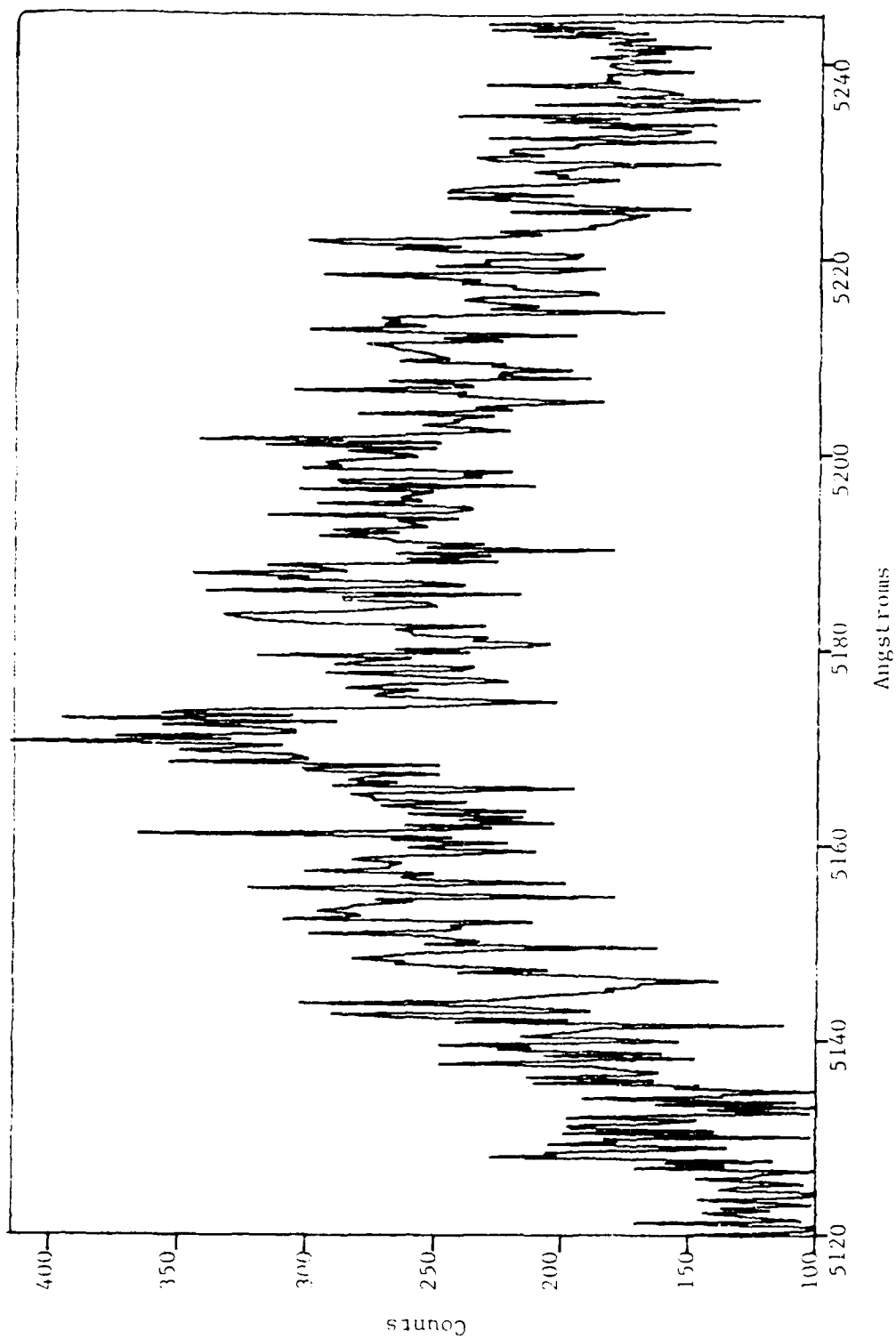
Figure 39. Induced Fluorescence, 5120-5240 Å
