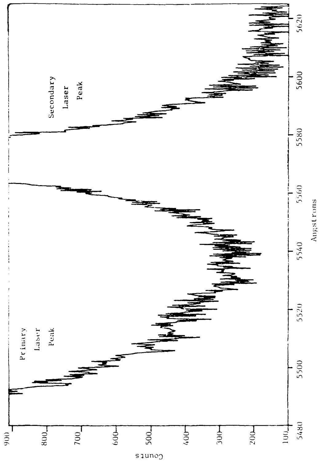
Figure 36. Induced Fluorescence, 5480-5620 Å
