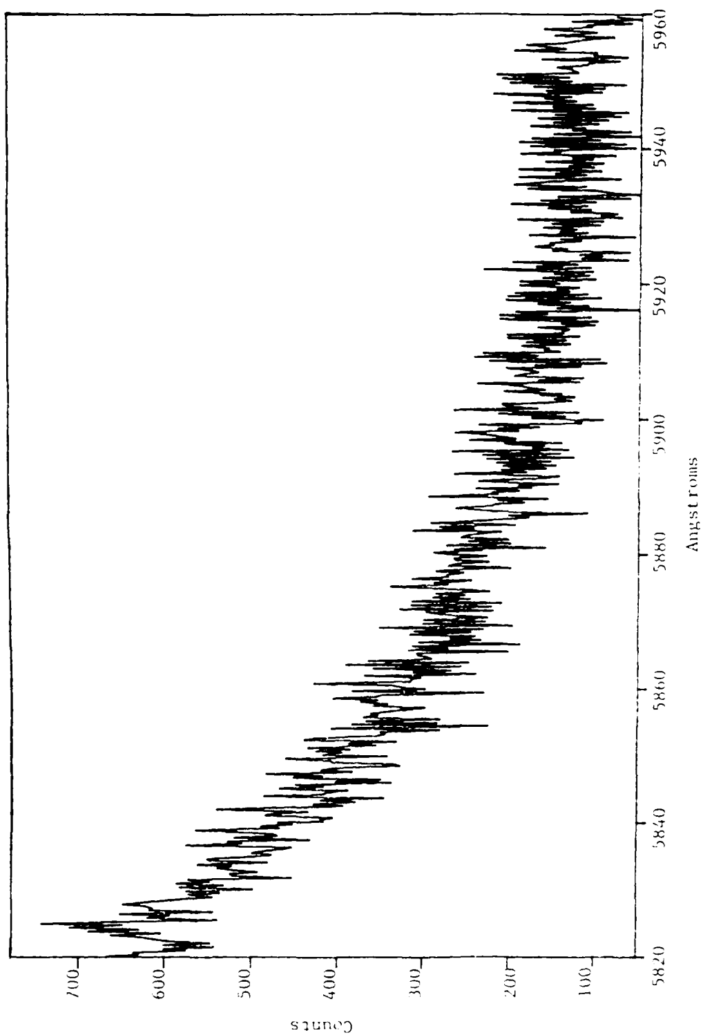
Figure 33. Induced Fluorescence, 5820-5960 Å
