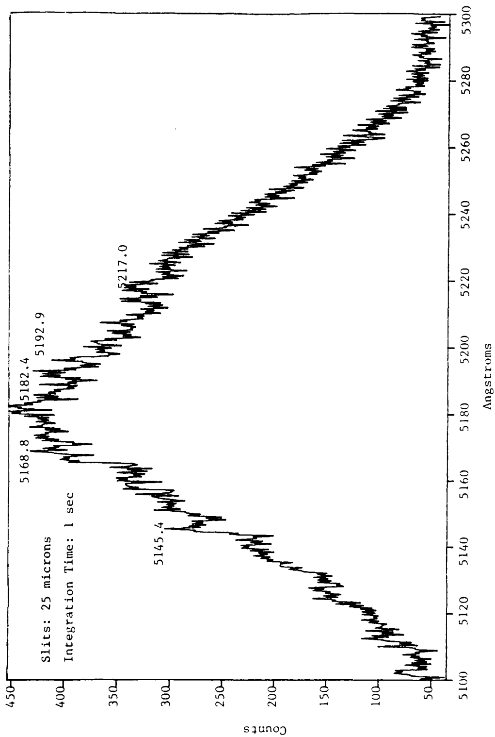
Figure 23. Flame Emission, 5100-5300 Å
