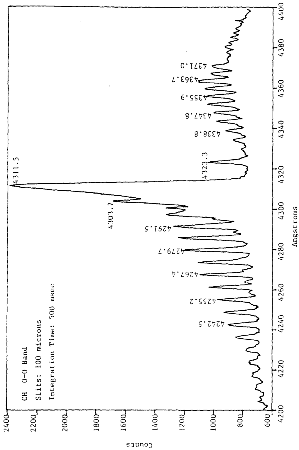
Figure 27. Flame Emission, 4200-4400 Å
