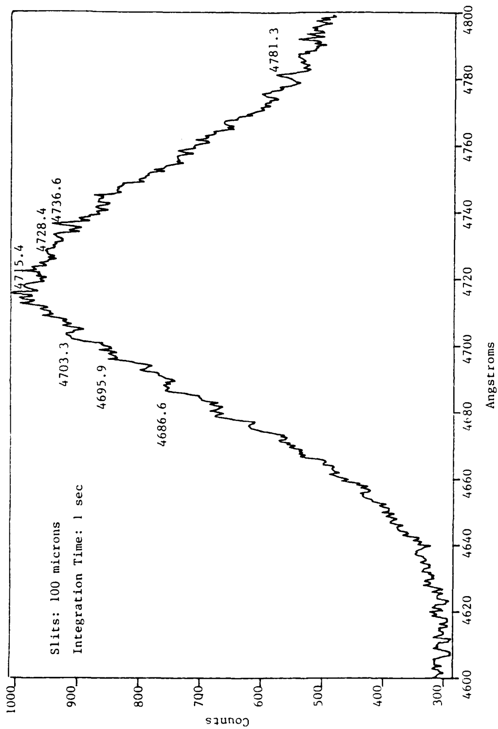
Figure 25. Flame Emission, 4600-4800 Å
