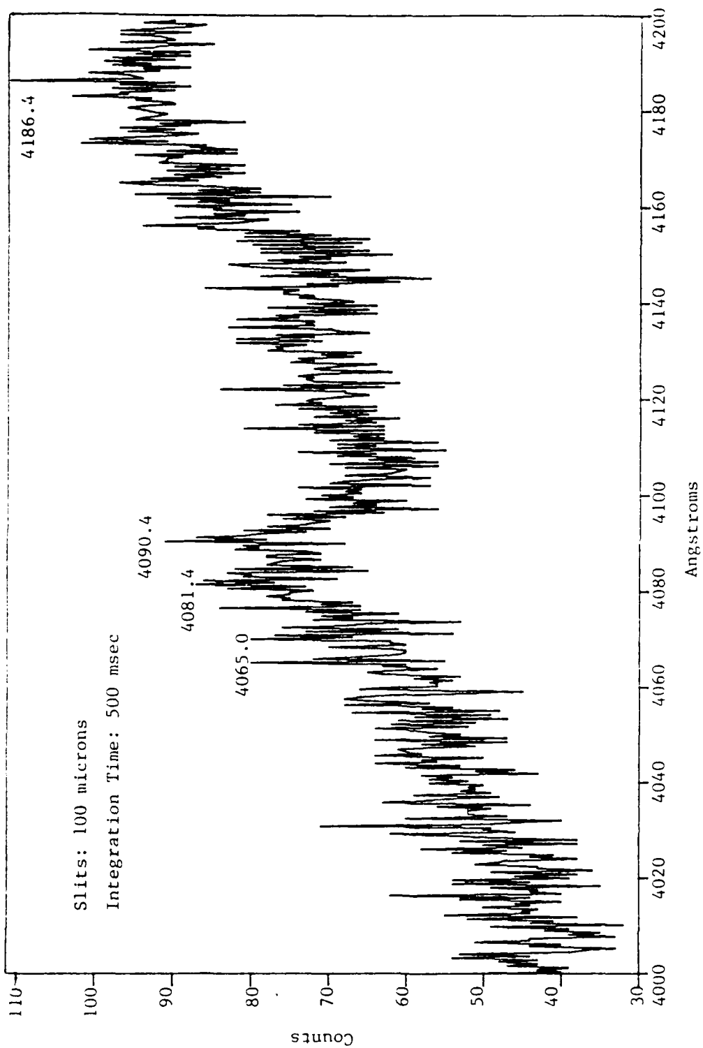
Figure 28. Flame Emission, 4000-4200 Å
