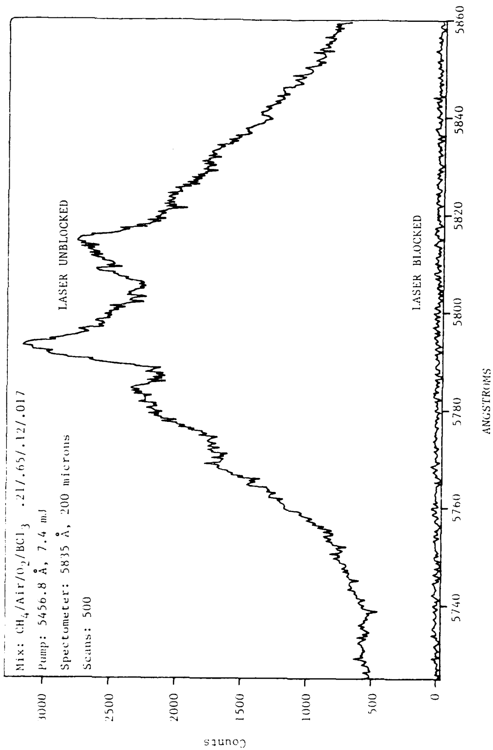
Figure 7. Non-Resonant Laser-Induced Fluorescence Signal from B0 2
