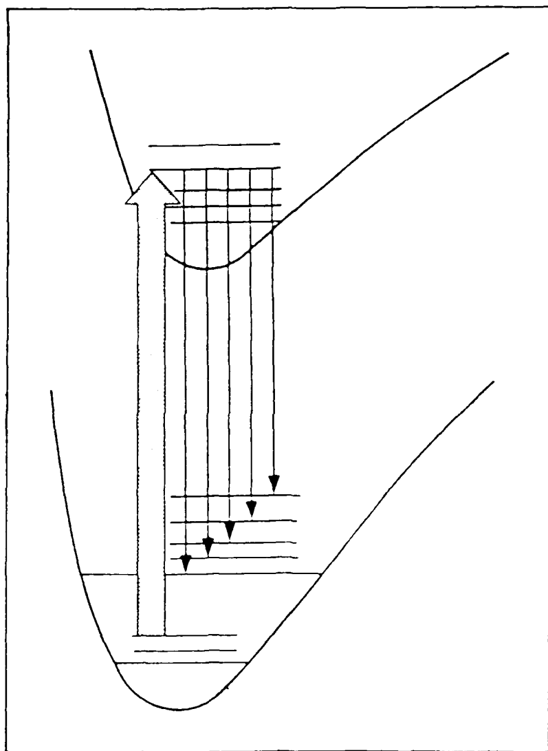
Figure 1. Ceneric Laser-Induced Fluorescence Scheme (29:550)
