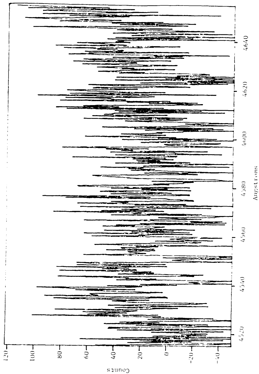
Figure 44. Induced Fluorescence, 4515-4655 Å
