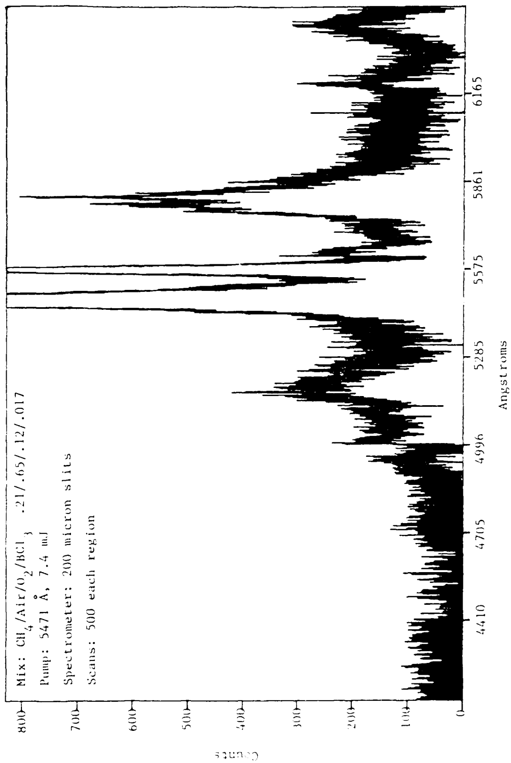
Figure 12. Composite Fluorescence Scan
