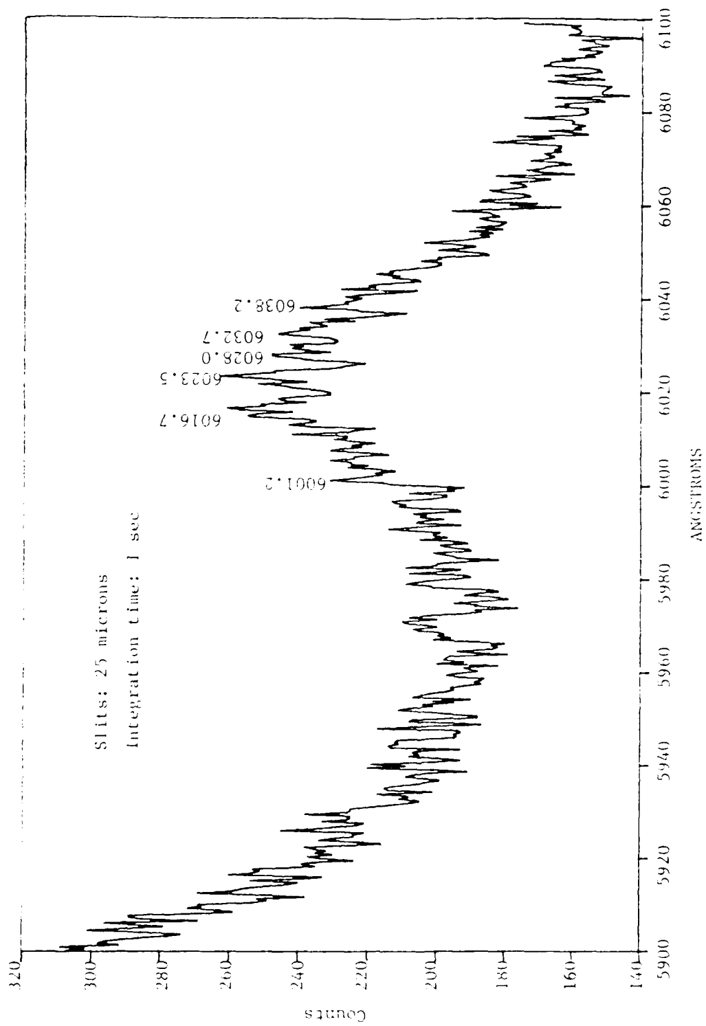
Figure 18. Flame Emission, 5900-6100 Å
