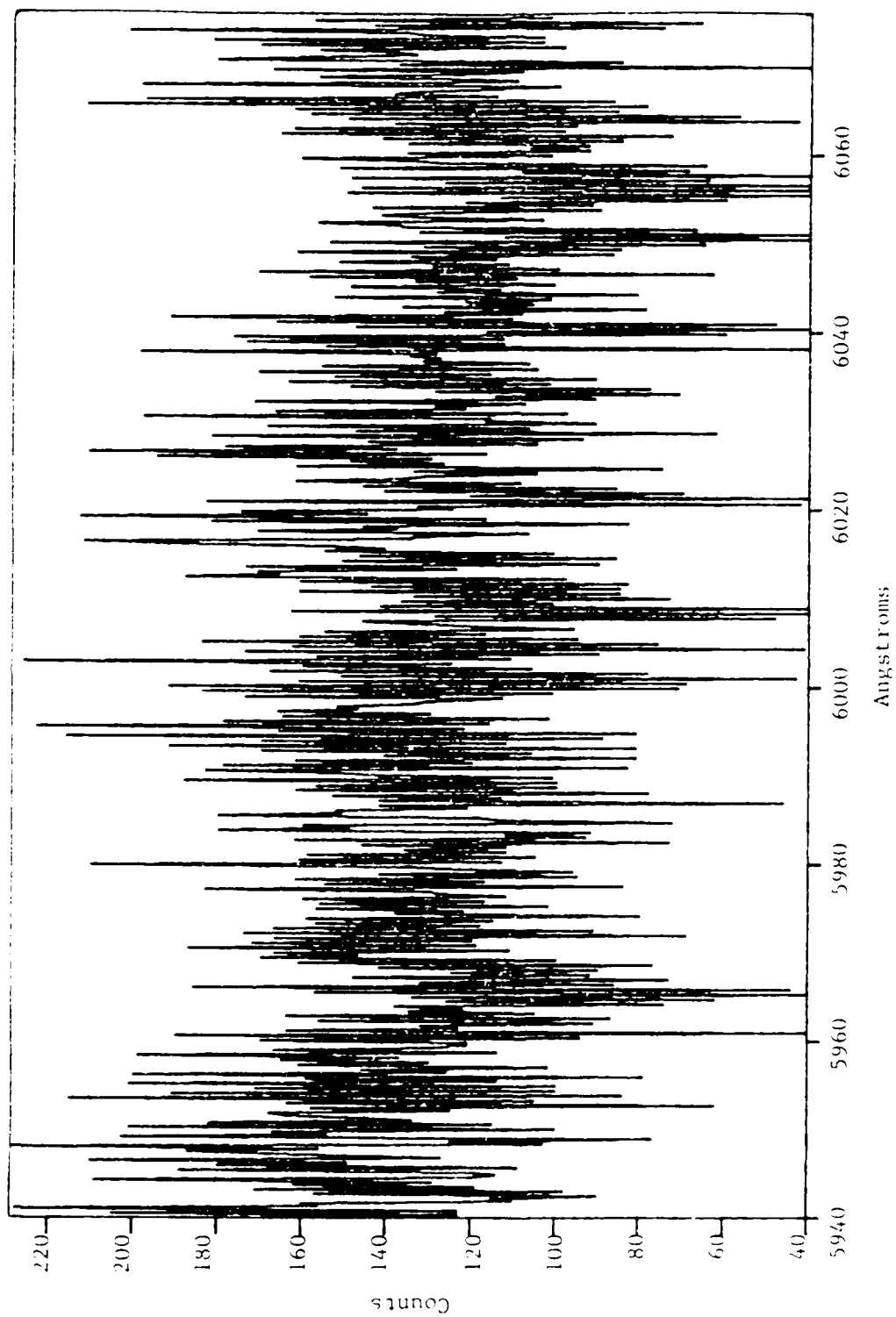
Figure 32. Induced Fluorescence, 5940-6080 Å
