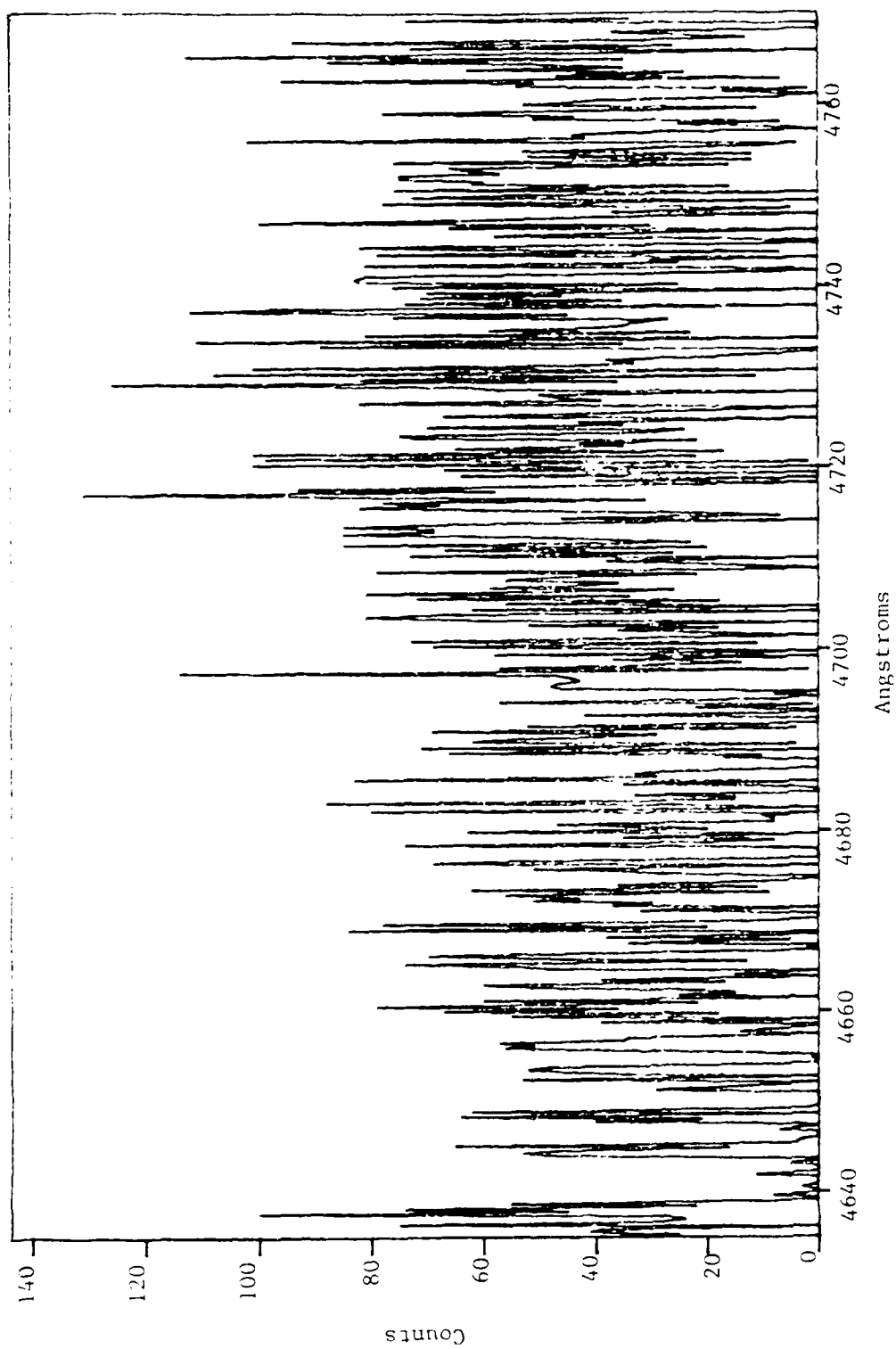
Figure 43. Induced Fluorescence, 4635-4765 Å
