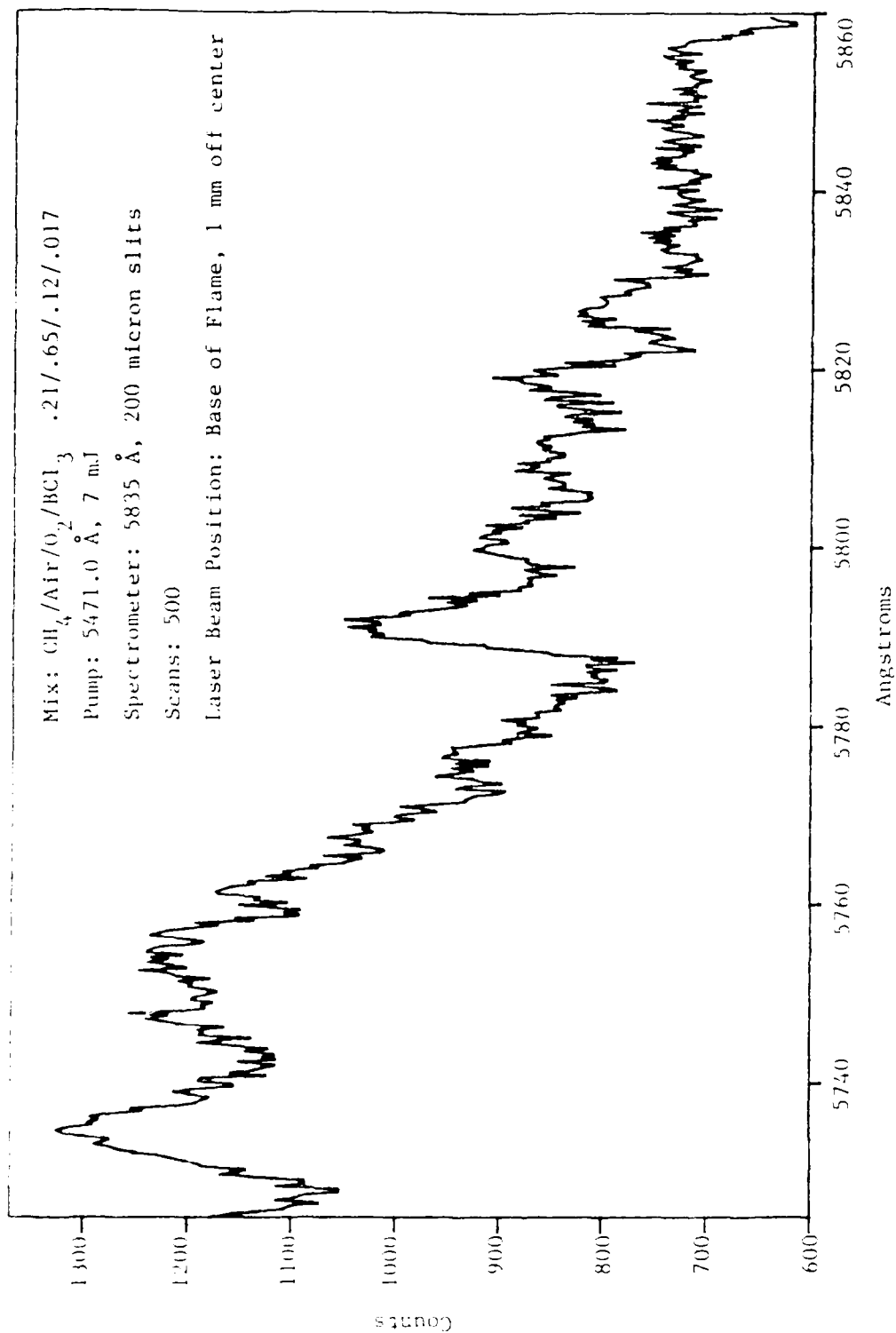
Figure 1b. Fluorescence Scan at Flame Base
