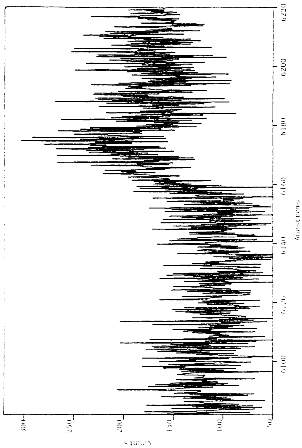
Figure 31. Induced Fluorescence, 6080-6220 Å
