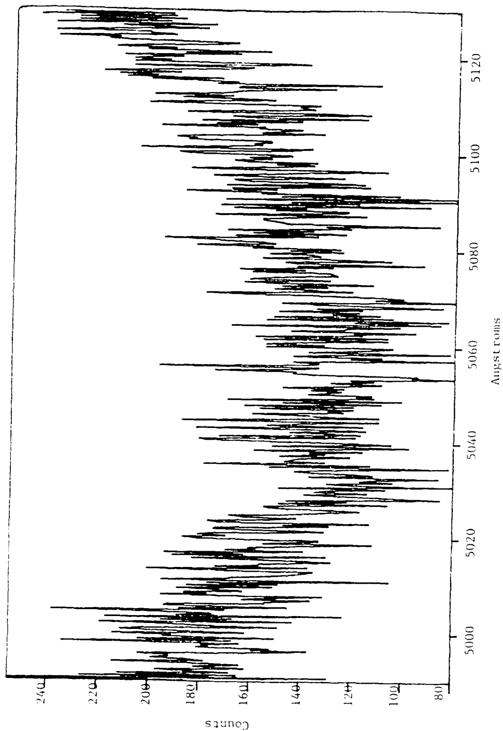
Figure 40. Induced Fluorescence, 4990-5130 Å
