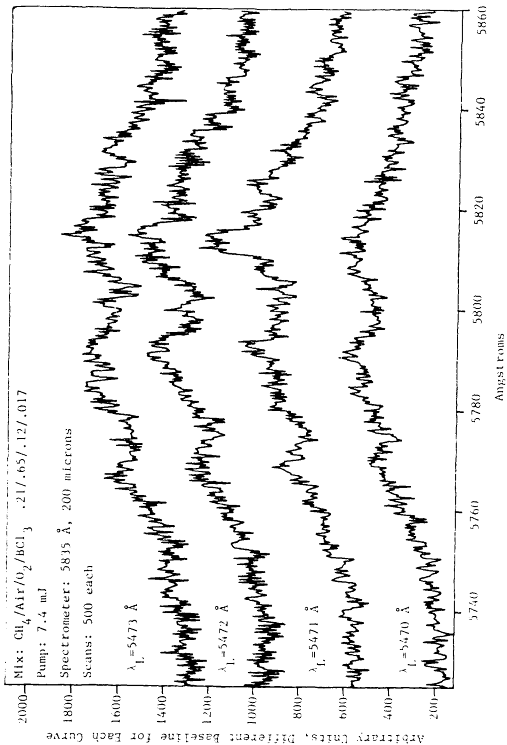
Figure 10. Excitation Scans of 00^0-00^0 0 R_2 Transition of \text{BCl}_3
