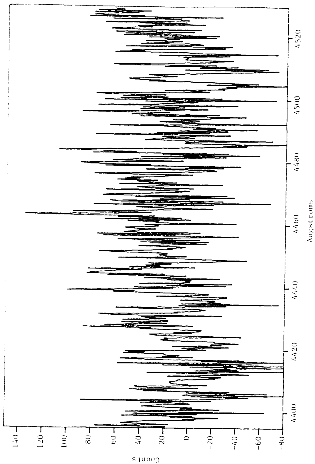
Figure 45. Induced Fluorescence, 4395-4525 Å
