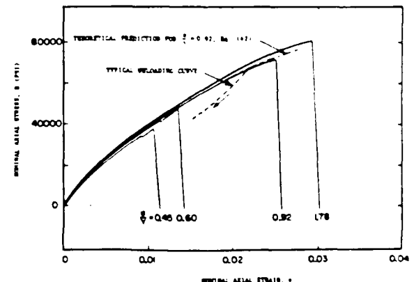
Fig. 4. Representative axial stress-strain curves with proportional axial and torsional straining from the same tests used for Fig. 3.
