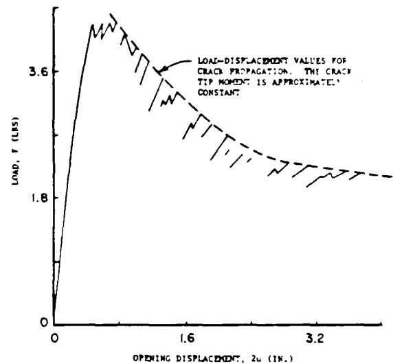
Fig. 11. A typical load-displacement record for opening mode loading of a double cantilevered beam with off-axis plies at the center interface. Hercules AS4/3502 graphite/epoxy. After Jordan (26).
