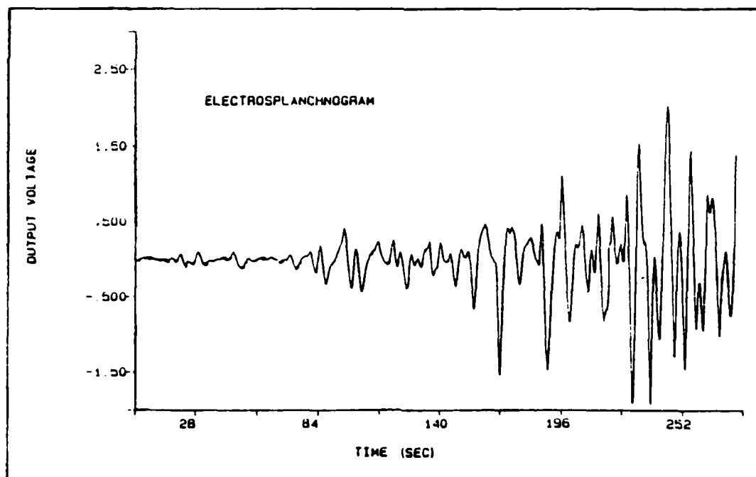
Figure 1. Electrosplachnogram Signal
