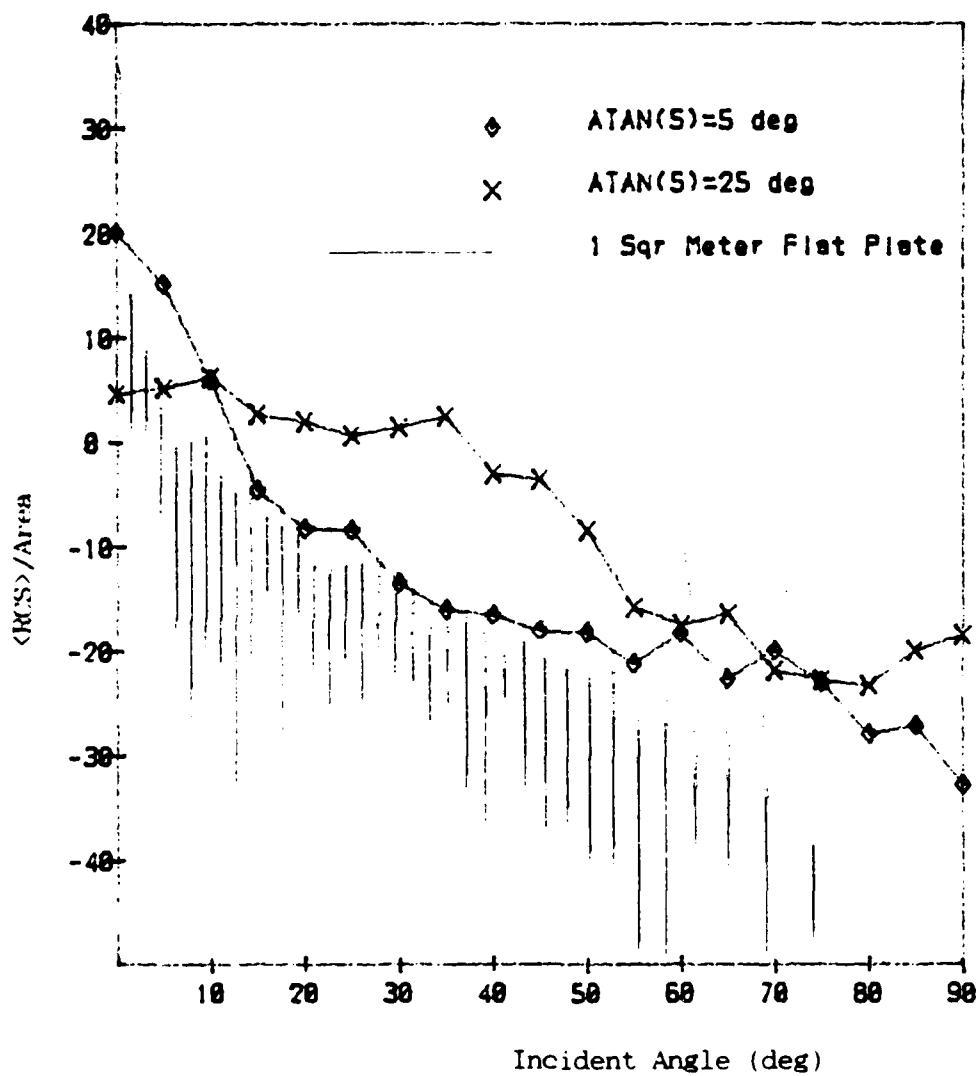
Fig. 23. \langle \text{RCS} \rangle / \text{Area} for Computer Generated Exponential Surfaces at 5.46 Ghz
