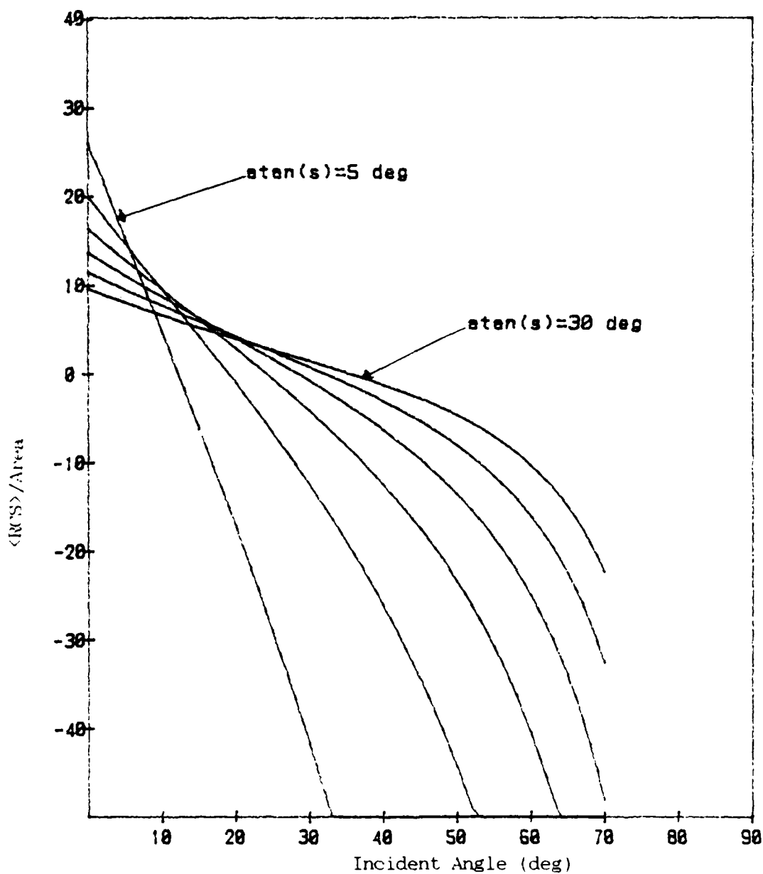
Fig. 15. \langle \text{RCS} \rangle / \text{Area} for an Exponential-type Surface as a Function of Incident Angle with 5 deg Mean Surface Slope Steps
