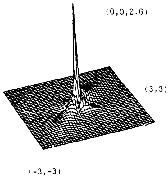
Fig. 8c. Joint Exponential pdf, \rho=.95
