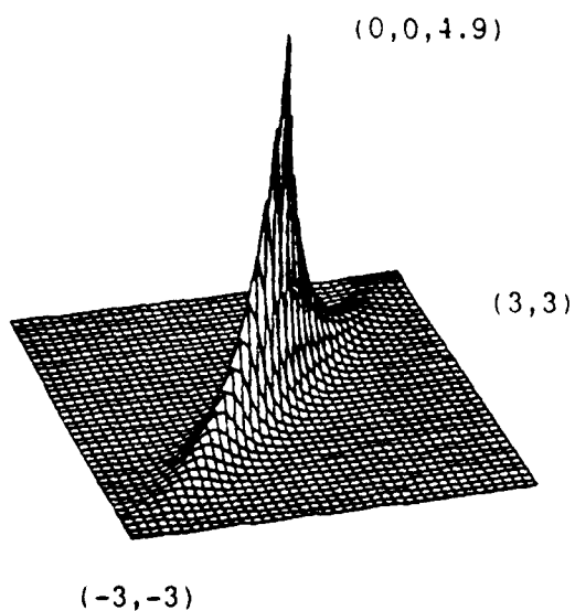
Fig. 6c. Joint Expo-type pdf, \rho=.95
