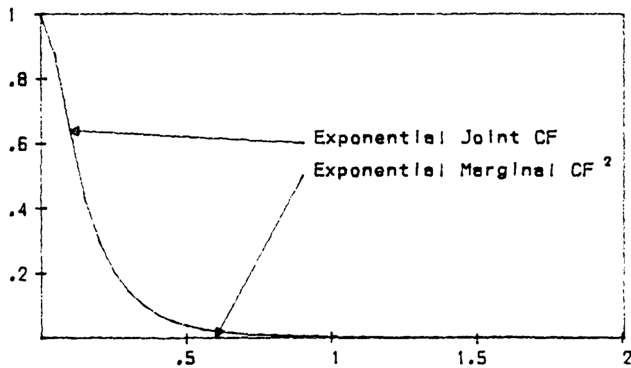
Fig. 12b. Exponential Joint CF and \chi_1^2 as a Function of Correlation Lengths with h \cdot v_z = 5
