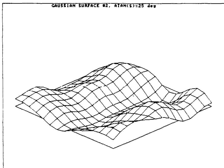
Fig. E1a. Gaussian Surface with Mean Slope of 25^\circ
