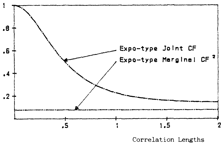
Fig. 11a. Expo-type Joint CF and \chi_1^2 as a Function of Correlation Lengths with h \cdot v_z = 2
