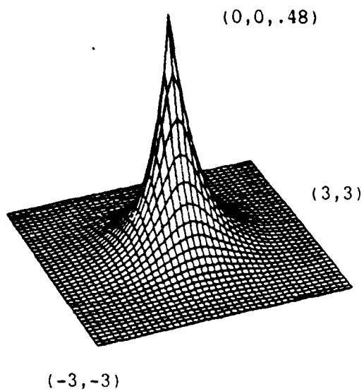
Fig. 6a. Joint Expo-type pdf, \rho=0
