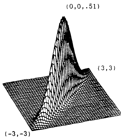
Fig. 4b. Joint Gaussian pdf with \rho=.5
