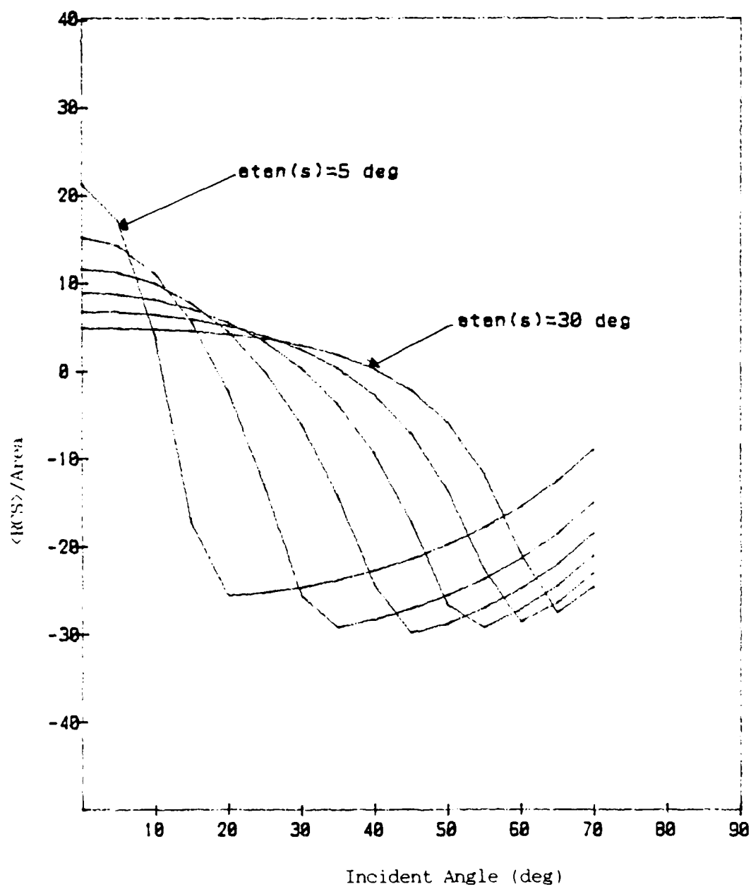
Fig. 18. Numerically Computed \langle \text{RCS} \rangle / \text{Area} for a Gaussian Surface as a Function of Incident Angle with 5 deg Mean Surface Slope Steps
