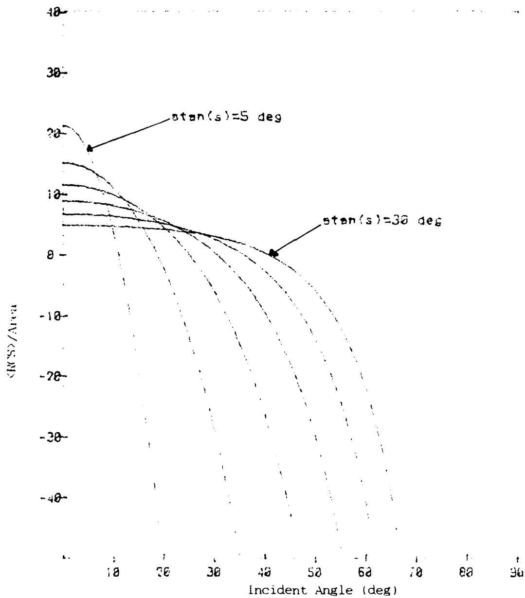
Fig. 14. \langle \text{RCS} \rangle / \text{Area} for a Gaussian Surface as a Function of Incident Angle with 5 deg Mean Surface Slope Steps
