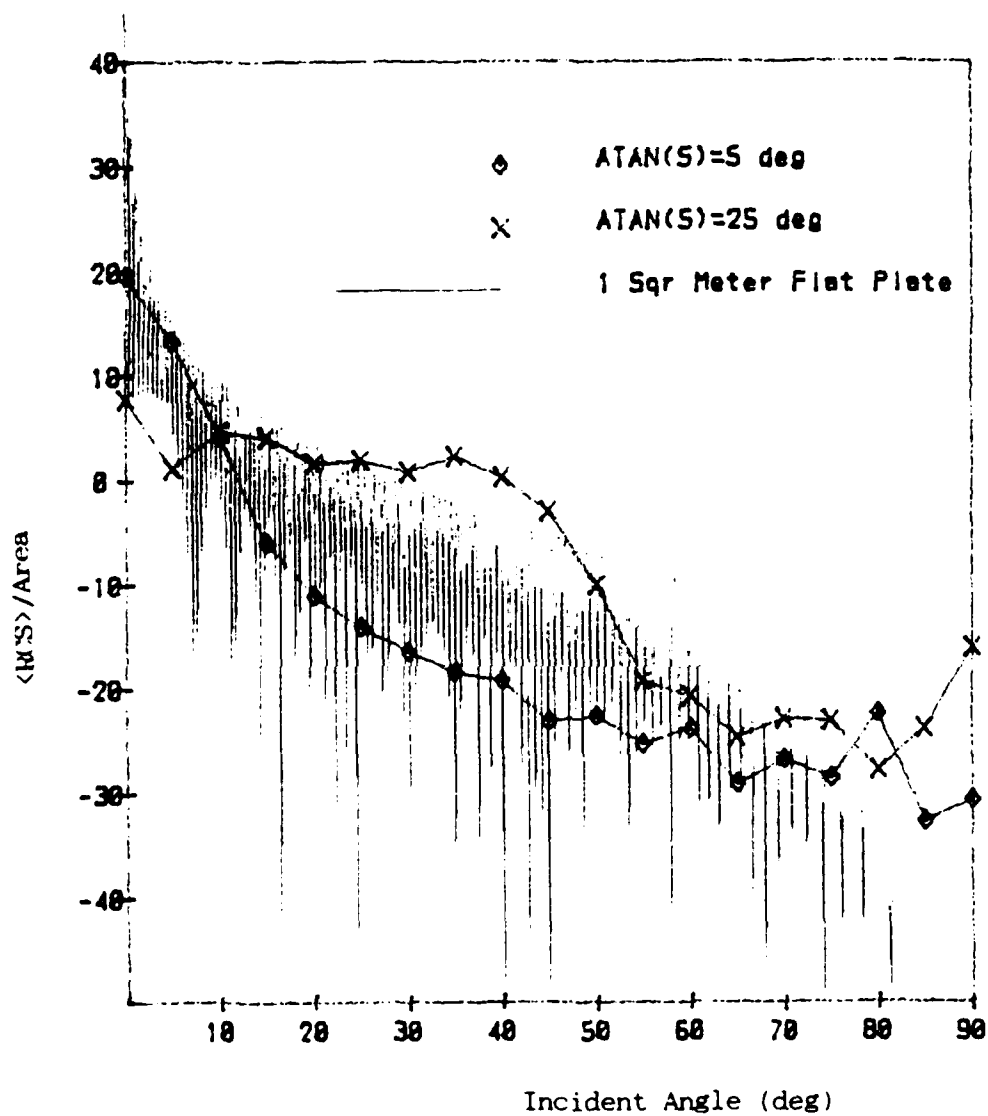
Fig. 24. \langle \text{RCS} \rangle / \text{Area} for Computer Generated Exponential Surfaces at 17.0 Ghz
