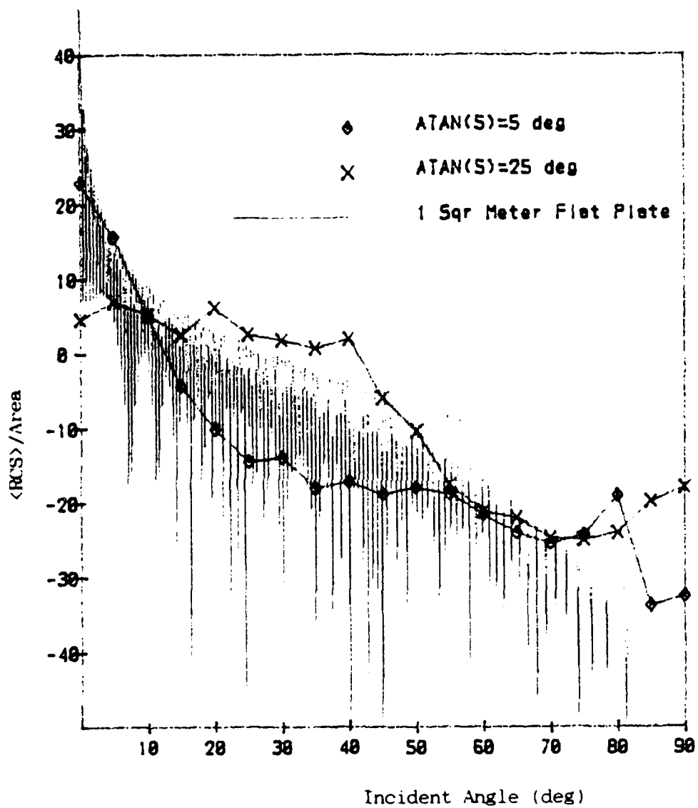
Fig. 22. \langle \text{RCS} \rangle / \text{Area} for Computer Generated Gaussian Surfaces at 17.0 Ghz
