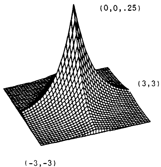
Fig. 8a. Joint Exponential pdf, \rho=0
