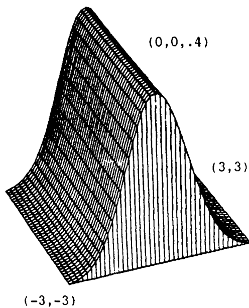
Fig. 5a. Conditional Gaussian pdf, \rho=0
