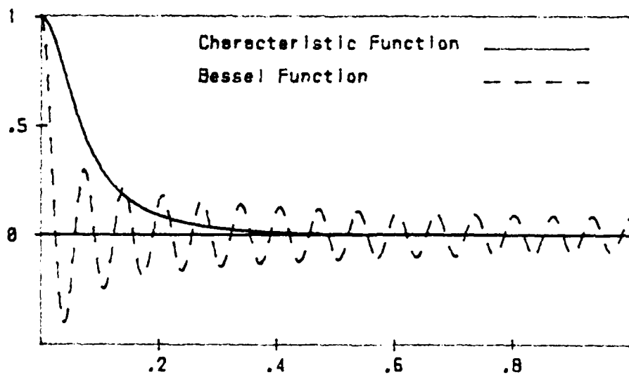
Fig. 16a. Exponential CF, h \cdot v_z = 10 , \text{atan}(s) = 20^\circ Angle of Incidence = 10^\circ
