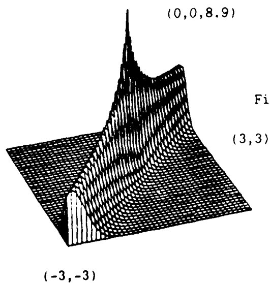
Fig. 7c. Conditional Expo-type pdf, \rho=.95
