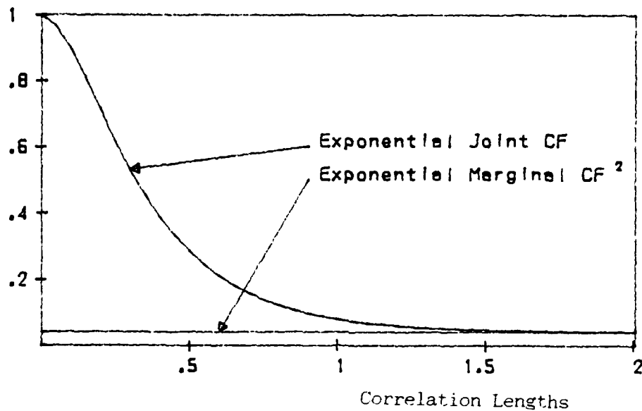
Fig. 12a. Exponential Joint CF and \chi_1^2 as a Function of Correlation Lengths with h \cdot v_z = 2
