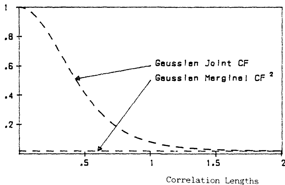
Fig. 10a. Gaussian Joint CF and \chi_1^2 as a Function of Correlation Lengths with h \cdot v_z = 2
