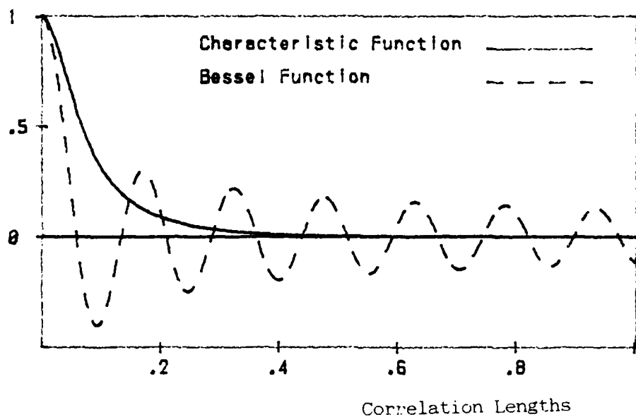
Fig. 17a. Exponential CF, h \cdot v_z = 10 , \text{atan}(s) = 10^\circ Angle of Incidence = 20^\circ
