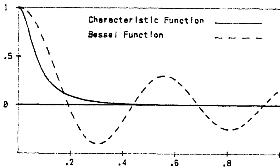
Fig. 17b. Exponential CF, h \cdot v_z = 10 , \text{atan}(s) = 30^\circ Angle of Incidence = 20^\circ
