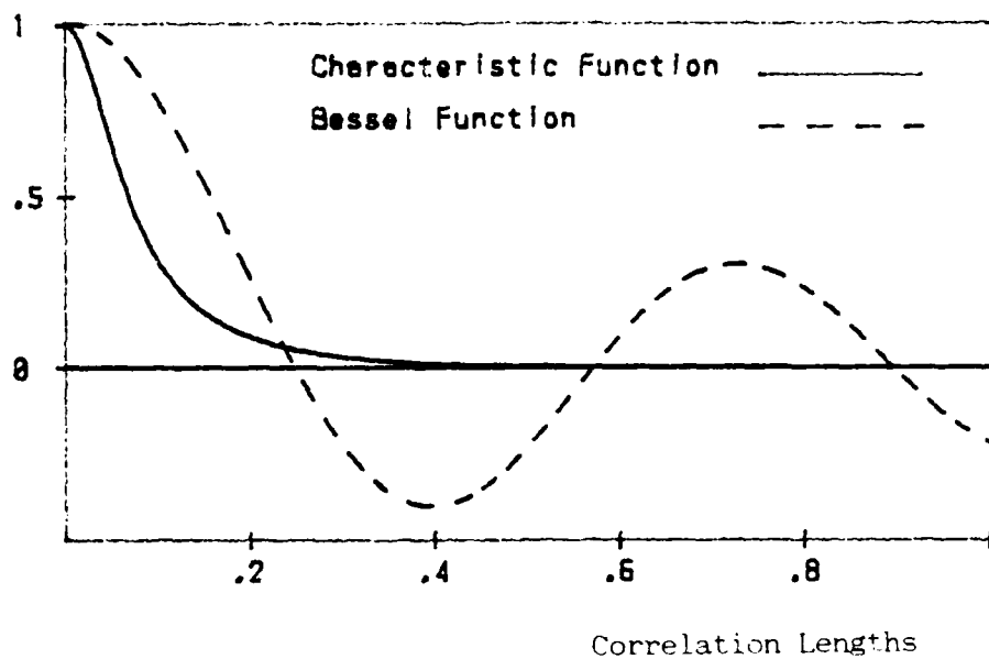
Fig. 16a. Exponential CF, h \cdot v_z = 10 , \text{atan}(s) = 20^\circ Angle of Incidence = 10^\circ
