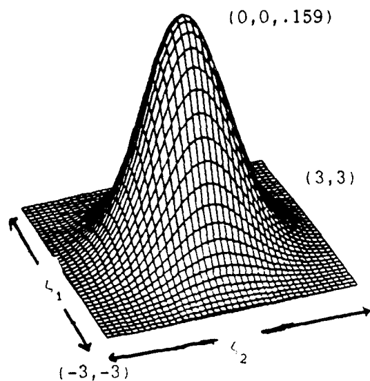
Fig. 4a. Joint Gaussian pdf with \rho=0
