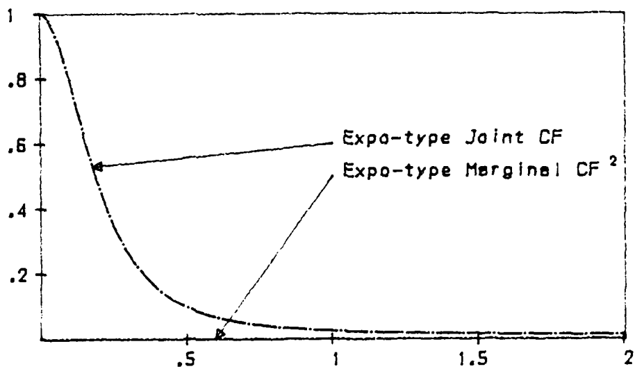
Fig. 11a. Expo-type Joint CF and \chi_1^2 as a Function of Correlation Lengths with h \cdot v_z = 2
