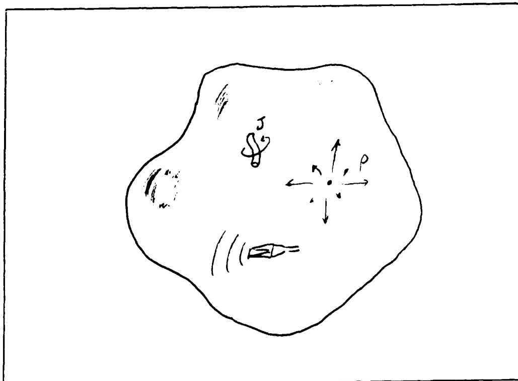
Fig. 1. Geometry Associated with the Stratton-Chu Equations
