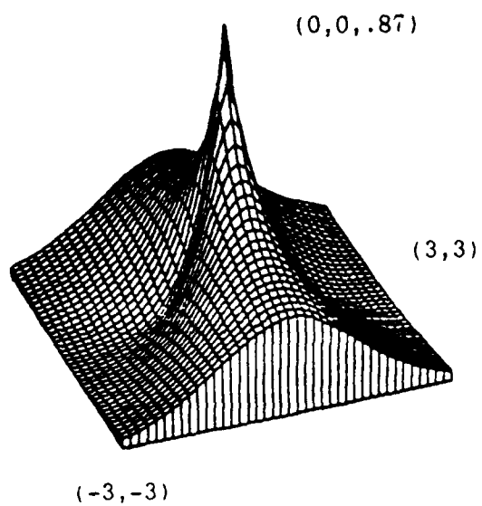
Fig. 7a. Conditional Expo-type pdf, \rho=0
