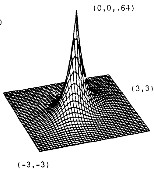
Fig. 6b. Joint Expo-type pdf, \rho=.5
