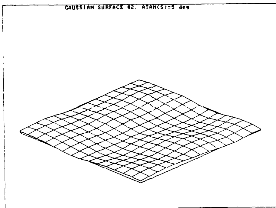
Fig. E1b. Gaussian Surface with Mean Slope of 5^\circ
