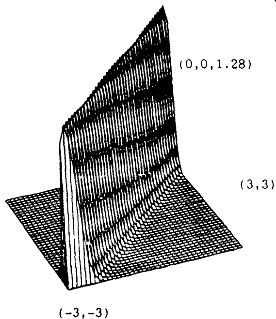
Fig. 5c. Conditional Gaussian pdf, \rho=.95
