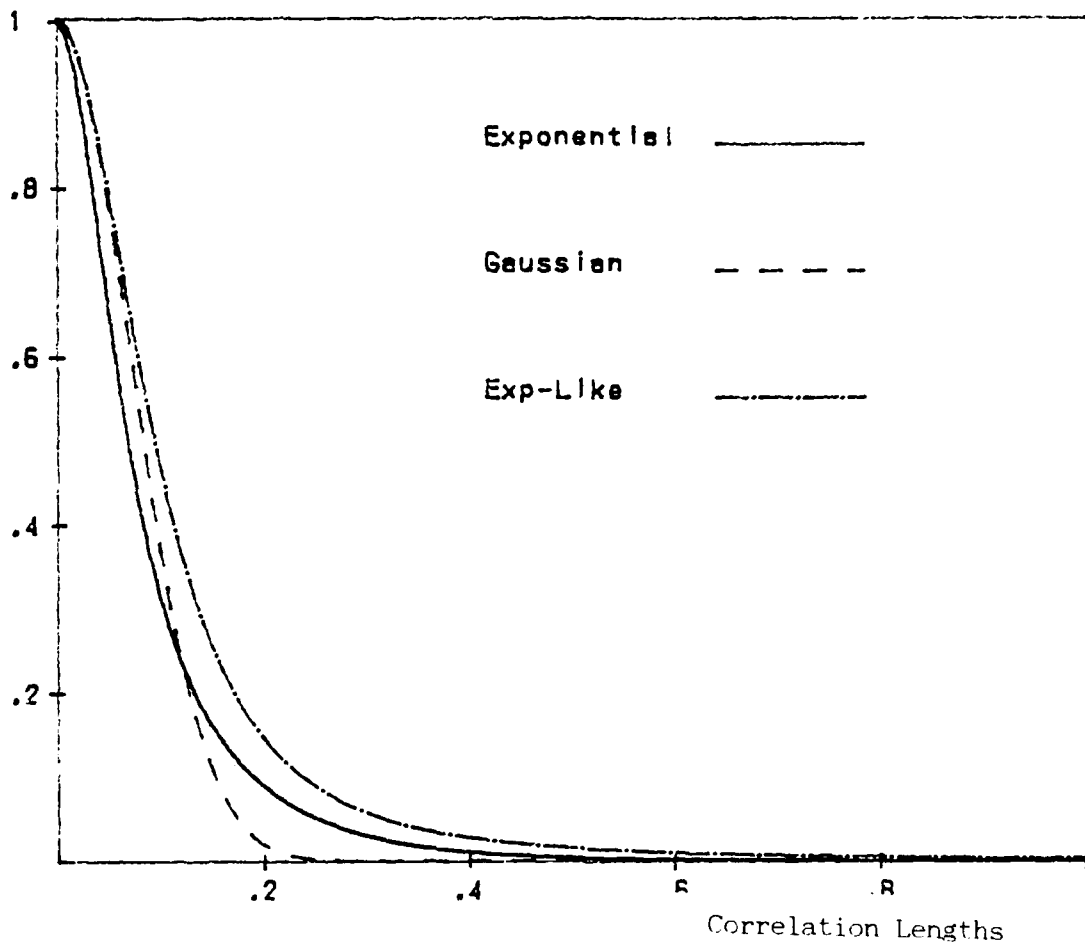
Fig. 13. Characteristic Functions \chi_2(10, -10)
