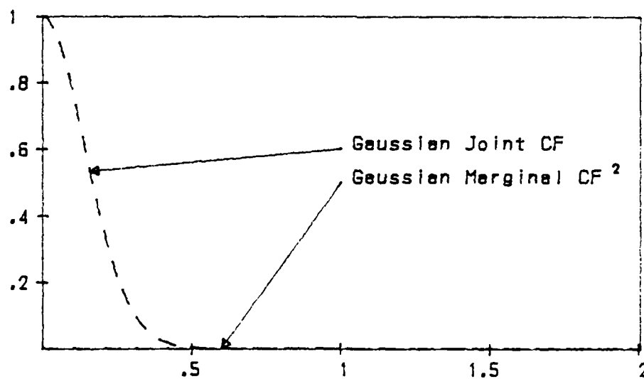
Fig. 10a. Gaussian Joint CF and \chi_1^2 as a Function of Correlation Lengths with h \cdot v_z = 2
