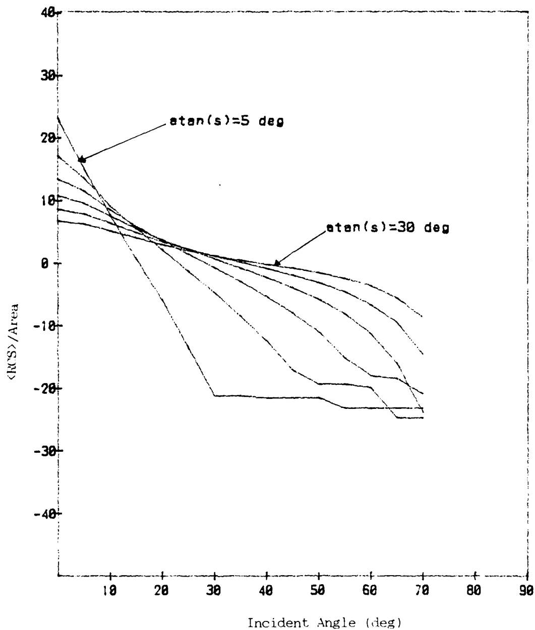
Fig. 19. Numerically Computed \langle \text{RCS} \rangle / \text{Area} for an Exponential Surface as a Function of Incident Angle with 5 deg Mean Surface Slope Steps
