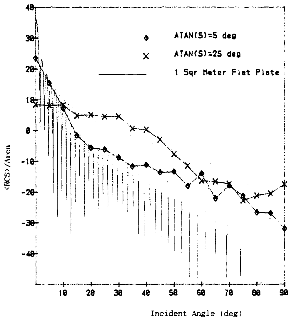
Fig. 21. \langle RCS \rangle / Area for Computer Generated Gaussian Surfaces at 5.46 Ghz
