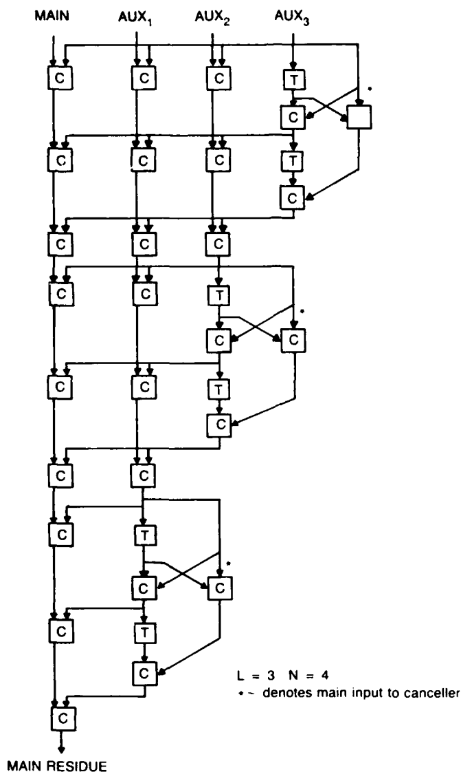
Fig. 9 — Efficient implementation of GS/ALF
