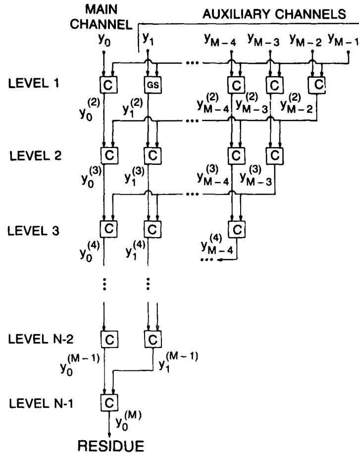
Fig. 4 — GS canceller
