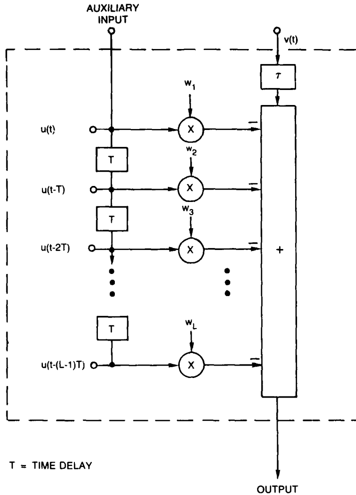
Fig. 6 — Transversal filter
