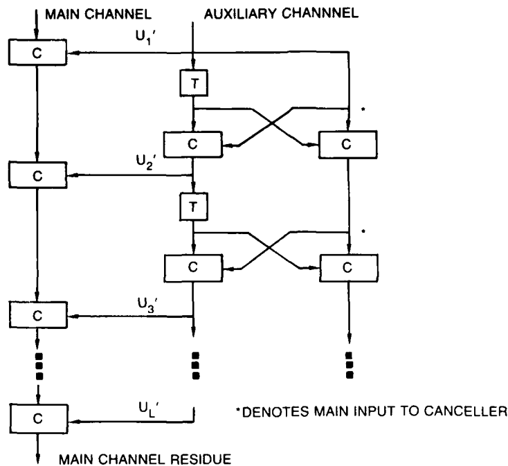
Fig. 7 — Adaptive lattice filter
