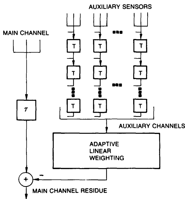
Fig. 1 — Generic space-time adaptive canceller
