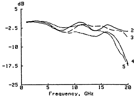
Figure 4: Small-signal gate voltages vs. frequency in a 5-FET 2-18 GHz distributed amplifier.
