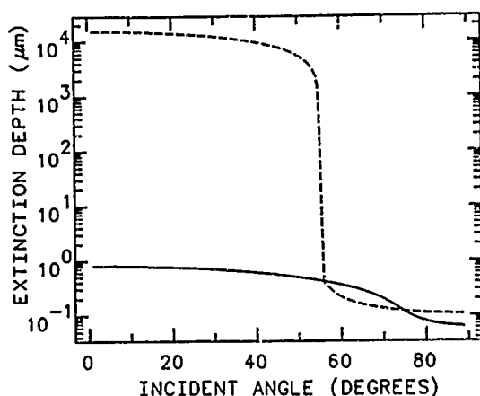
Fig. 2 -- Extinction depth for 0.83 \mu\text{m} . pulses incident through trigonal selenium upon GaAs (solid curve) and for 3.0 \mu\text{m} . pulses incident through Ge upon n-GaAs (dashed curve). Note sharp decreases above critical angles ( 75^\circ for Se/GaAs, 55^\circ for Ge/n-GaAs).
