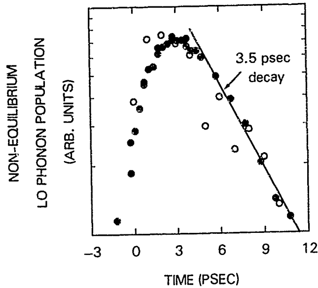
Figure 1. Room temperature nonequilibrium phonon kinetics for LO phonons in GaAs (filled circles), and the GaAs-like LO phonon in \text{Al}_{0.24}\text{Ga}_{0.76}\text{As} (open circles). Laser wavelength is 580nm for GaAs, 567nm for \text{Al}_{0.25}\text{Ga}_{0.76}\text{As} . Pulse width in both cases is 0.7 psec (autocorrelation FWHM). Risetime differences result from differences in bandgap.
