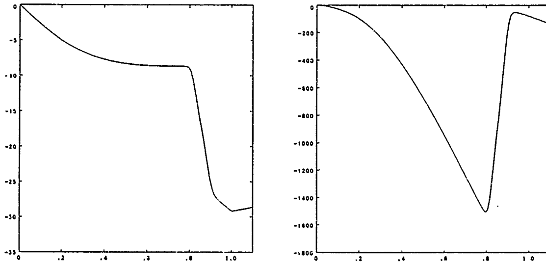
Figure 4. Calculation of current through diode (left) and voltage across diode (right) corresponding to Fig. 3. Scales: Amps or Volts vert, nsec horiz.
