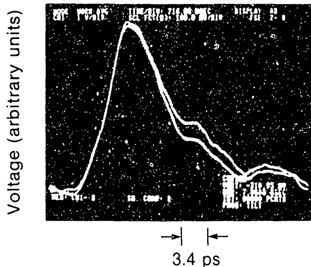
Figure 1. Junction voltage waveforms. Upper curve corresponds to the "no junction" condition in the transmission line, and the lower curve in the unbiased junction response.
