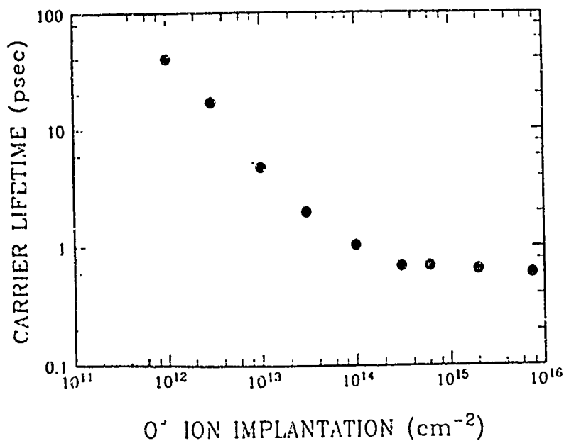
FIGURE 2. Carrier lifetime vs. ion-implantation dose. Lifetimes are derived from individual reflectivity data at each dose.
