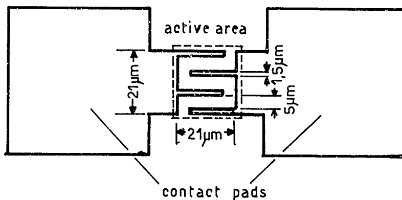
Fig.2: The detector and its dimensions
