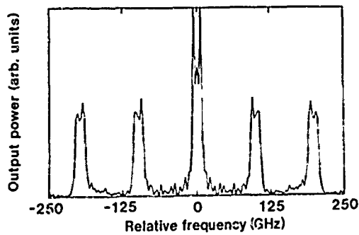
Fig. 2 (a) Measured modulus of the ACF for a pulsed ridge waveguide SQW laser (b) Power spectrum calculated from Fig. 2a
