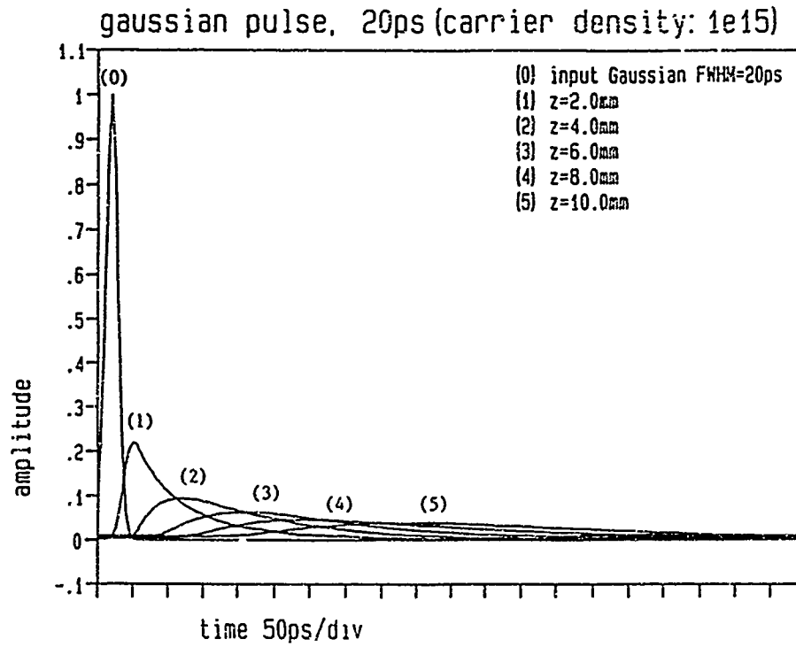
Figure 2: Pulse evolution with electron concentration in layer 2 of Fig. 1 at 10^{15}\text{ cm}^{-3} .
