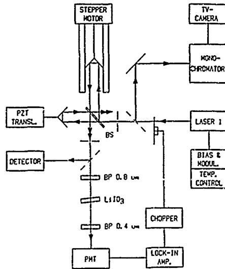
Fig. 1 Experimental setup for temporal coherence measurements
