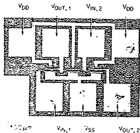
Figure 3 Top view of a monolithically integrated inverter circuit, consisting of 3 MISFET's and 3 resistors.
