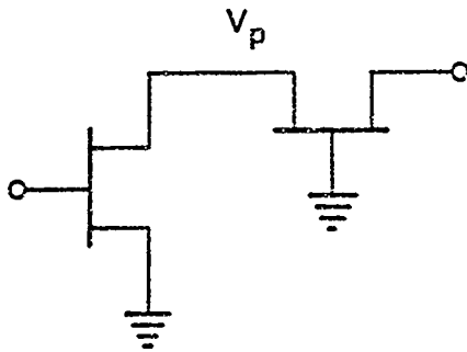
Fig. 4 Cascode connection of two FETs.
