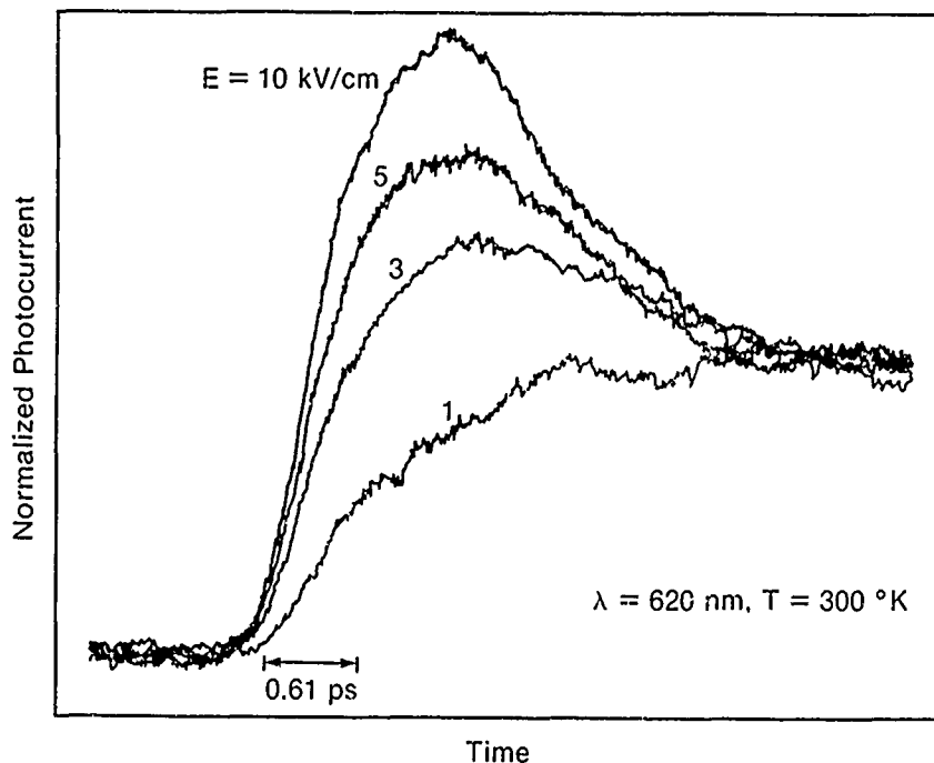
Fig. 1 The photocurrent induced in intrinsic GaAs by a 100 fs pulse is shown as a function of time for different electric field strengths. The photocurrent exhibits a strong enhancement indicating the presence of velocity overshoot.
