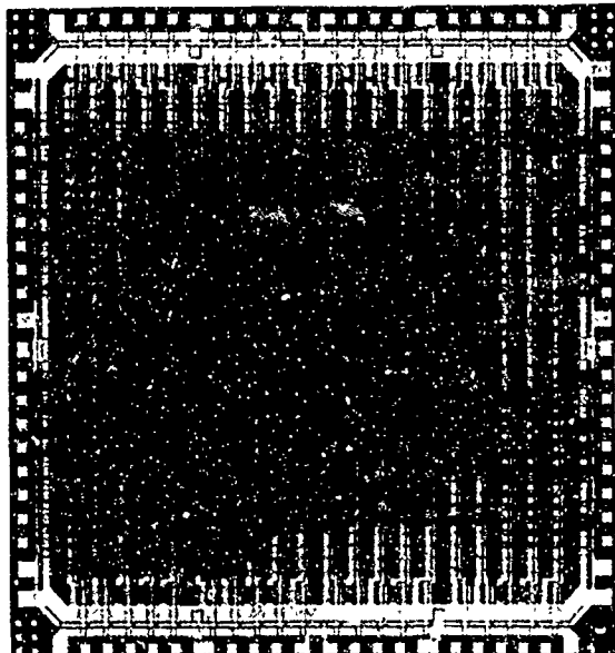
Fig. 3 Microphotograph of HEMT 1.5 kgate gate array.
