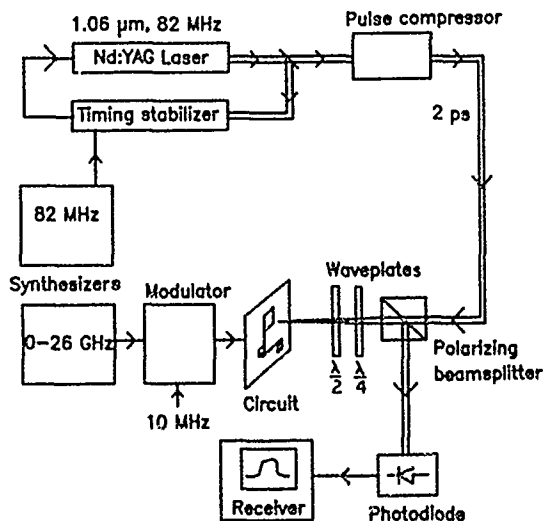
Figure 1: Electrooptic sampling system.
