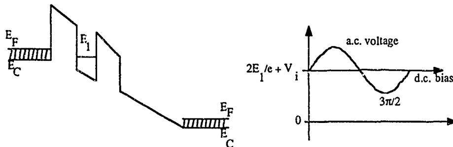
Fig. 2. Energy band diagram when the device is biased for conduction to occur at 3\pi/2 .
