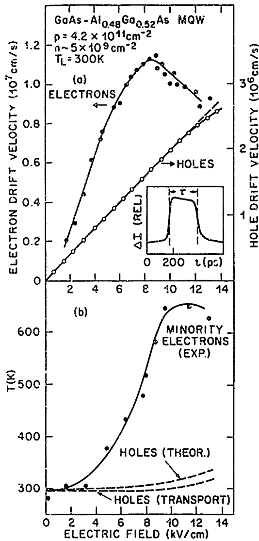
Fig. 1 (a) Electron drift velocity in p-GaAs quantum wells measured by picosecond time-of-flight technique and hole drift velocity from I-V measurements. The inset shows the photocurrent pulse from which drift velocity is determined. (b) Electron temperature as a function of applied electric field deduced from luminescence measurements and hole temperatures as discussed in text.
