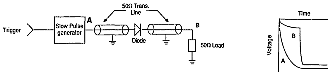
Figure 1. Schematic diagram of pulse sharpening diode circuit and typical voltage waveforms at points A and B in the circuit.
