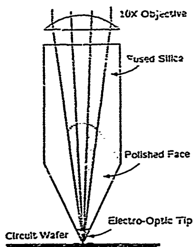
Fig. 1. The electro-optic probe
