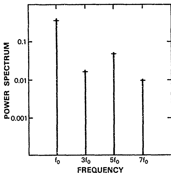
Figure 5. Power spectrum calculated from the current waveform in Fig. 4. The even harmonics are absent because of the symmetry of the I-V curve, while the large 5th harmonic content derives from the occurrence of one negative resistance region.
