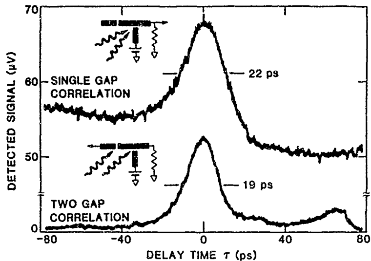
Figure 1. Comparison of two-gap and single gap correlation techniques on an InP correlation circuit.
