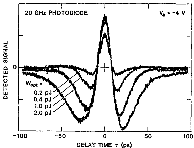
Figure 3. The nonlinear response of a 20 GHz Schottky-barrier GaAs photodiode at several incident optical energies W_{\text{opt}} .
