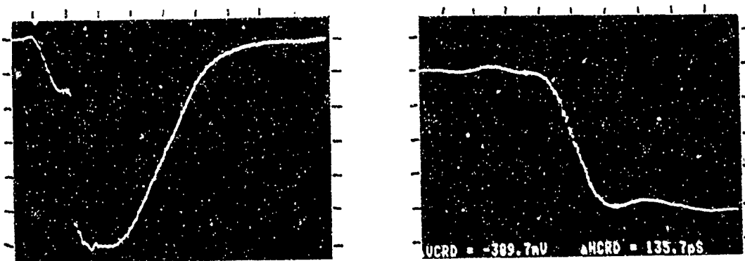
Figure 2. Fastest rise (fall) time waveform generated (63 ps - fast transition). Left picture - 500 V/div vert, 1 ns/div horiz; Right picture - 500 V/div vert, 50 ps/div horiz.
