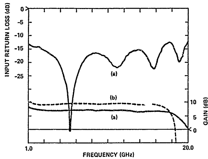
Fig. 3 (a) Distributed amplifier gain and return loss with nominal channel doping of 3-5 \times 10^{17} \text{ cm}^{-3} ; (b) amplifier gain with nominal doping of 5 \times 10^{17} \text{ cm}^{-3} .
