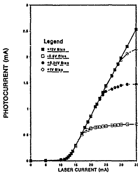
PHOTOCURRENT vs LASER CURRENT
