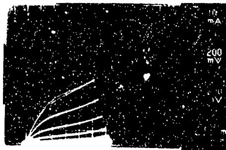
Figure 2 Drain-source I-V characteristic of a MISFET at room temperature having a gate length and gate width of 1 \mu\text{m} and 250 \mu\text{m} , respectively. Vertical scale is 10 mA/div, horizontal scale is 200 mV/div, gate voltage is increased in steps of 200 mV.
