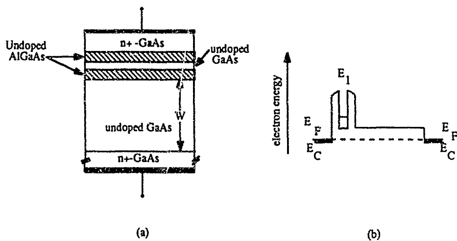
Fig. 1(a). Physical structure of the QWITT. (b) Energy band diagram of the device when no d.c. bias is applied.
