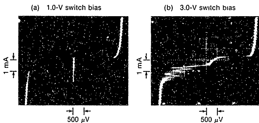
Figure 2. Junction DC I-V curves for two different values of the amplitude of the input pulse. Due to the corrected, two-wire measurements, the gap voltages displayed appear to be slightly reduced.
