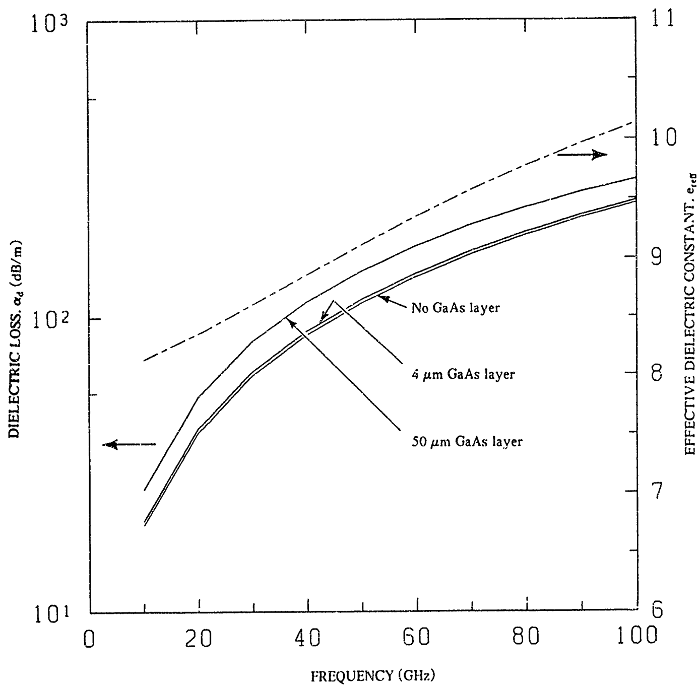
Fig. 1. Dielectric loss and effective dielectric constant versus frequency for \rho_{Si} = 2000 \Omega\text{-cm} , \rho_{GaAs} = 1000 \Omega\text{-cm} .
