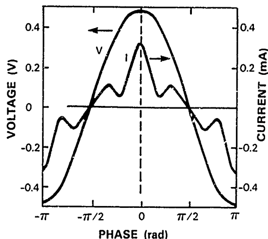
Figure 4. Calculated voltage and current waveforms for the DC I-V curve of Fig. 3 when driven by a pump with a 50 \Omega source impedance.
