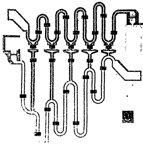
Fig. 2 2-20 GHz coplanar distributed amplifier.
