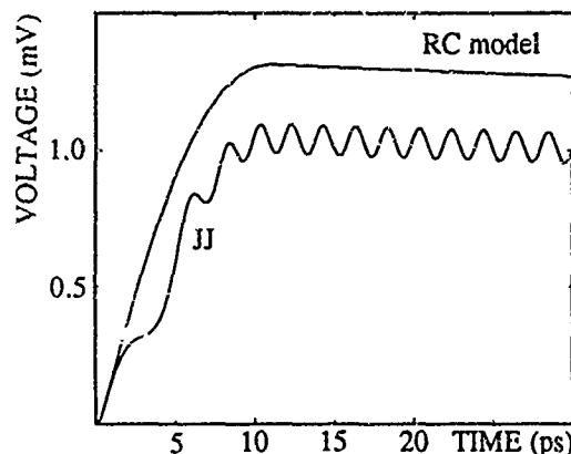
Figure 3. The simulated Josephson junction response (JJ curve) to a stepped input pulse of amplitude 1.2I_C and duration t_p \approx 10 ps. The full solution of the RCSJ model is compared to the prediction of the charging capacitance model. 3 Junction parameters are the following: I_C = 2.75 mA, R_J = 0.6 \Omega , R_1 = 35 \Omega , C_J = 16 pF.
