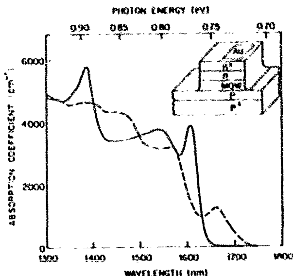
Figure 1: Room temperature absorption spectra at 0V (solid line) and 30V (dashed line). The sample structure is shown in the insert.
