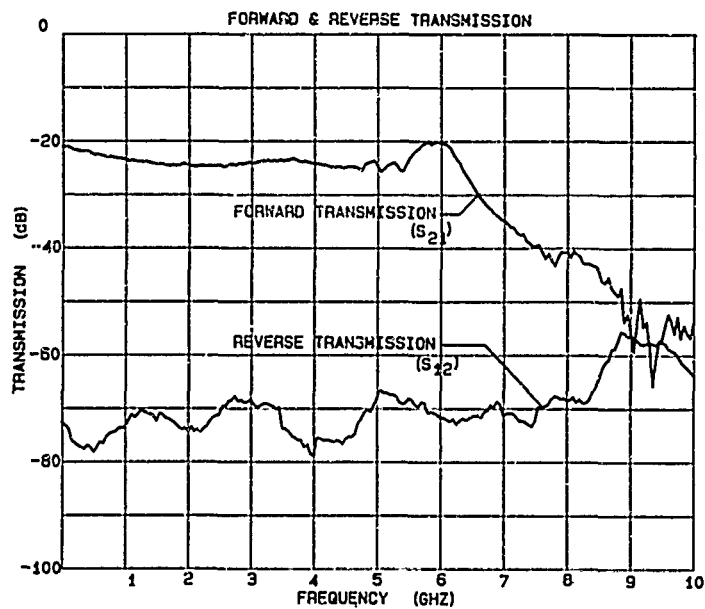
Fig. 3 Microwave forward and backward transfer characteristics
