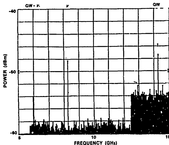
Figure 2. Measured power spectrum of a resonant tunneling oscillator (marked QW) mixing with an injected signal (marked v) to produce a difference-frequency output (marked QW-v). This oscillator was cooled to 20 K.
