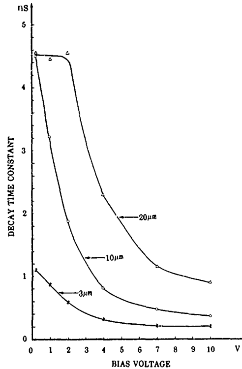
Fig. 1: Decay time constant as a function of applied voltage for three Fe:InGaAs switches of different gap size.
