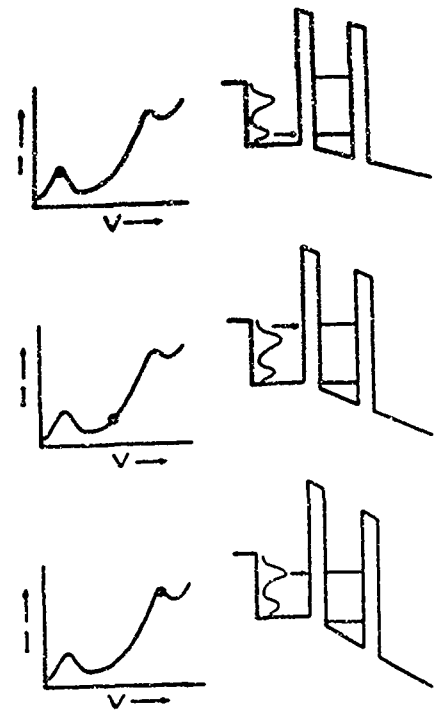
Fig. 2 Schematics of RTS. By measuring the current as a function of reverse bias (left) one directly probes the energy distribution perpendicular to the layers n(E_1) (right).
