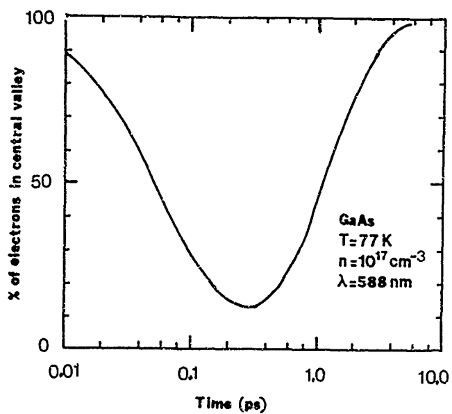
Fig. 1 Fraction of photoexcited electrons in the central valley as function of time after excitation by a 588nm laser pulse.
