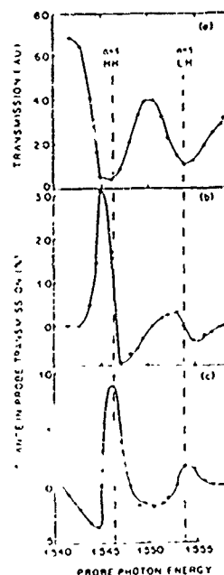
Fig. 3 a) Unperturbed transmission showing n=1 heavy (hh) and light (lh) hole excitons. b) and c) Percent change in probe transmission induced by 10^6 Watts/cm 2 pump 31 meV below the n=1 hh transition. (b) zero pump-probe delay; (c) delay = 100 psec.
