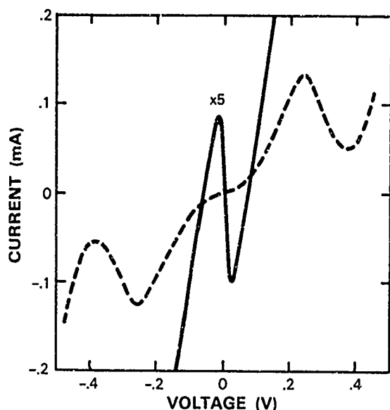
Figure 3. Current-voltage curves for one of our early resonant-tunneling structures operating at 20 K: dashed line is measured DC characteristics; the full line results when a 1 GHz pump with an amplitude of about 0.4 V has been applied. The negative resistance in the region near V = 0 can be varied by changing the amplitude of the pump.
