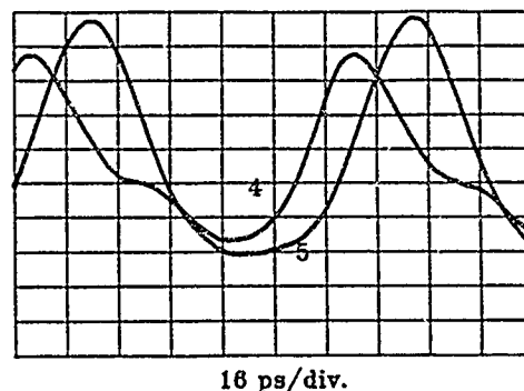
Figure 5: Saturation waveforms at drains 4 and 5 of the distributed amplifier at 10 GHz and 1 dB gain compression
