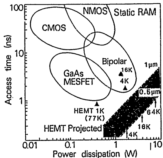
Fig. 5 Address access time and power dissipation of the static RAMs. The plots show the performances of the HEMT static RAMs,
