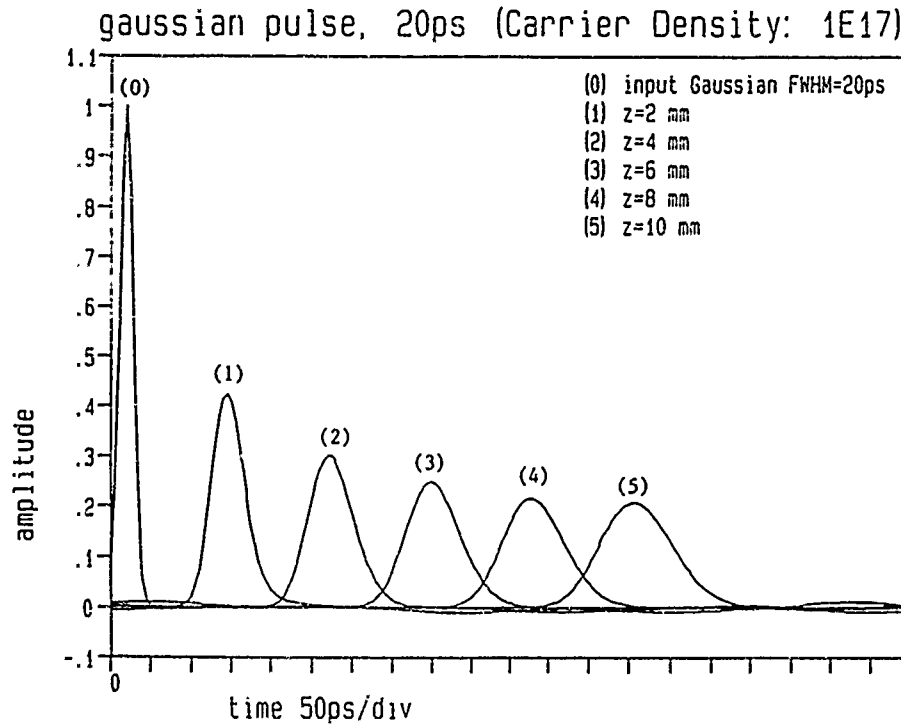
Figure 3: Layer 2 with 10^{17}\text{ cm}^{-3} concentration.
