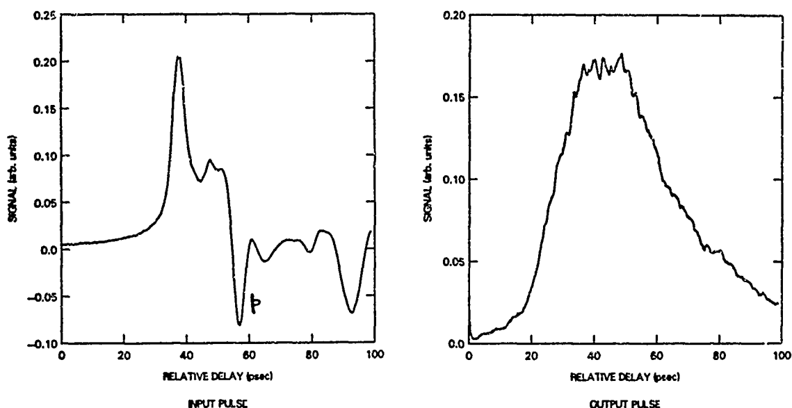
Figure 2. Input and output pulses measured at points b and c in figure 1. The negative feature p is due to the pulse generated at point a in figure 1 reflecting back from the interface between the wirebonds and the low impedance transmission line.
