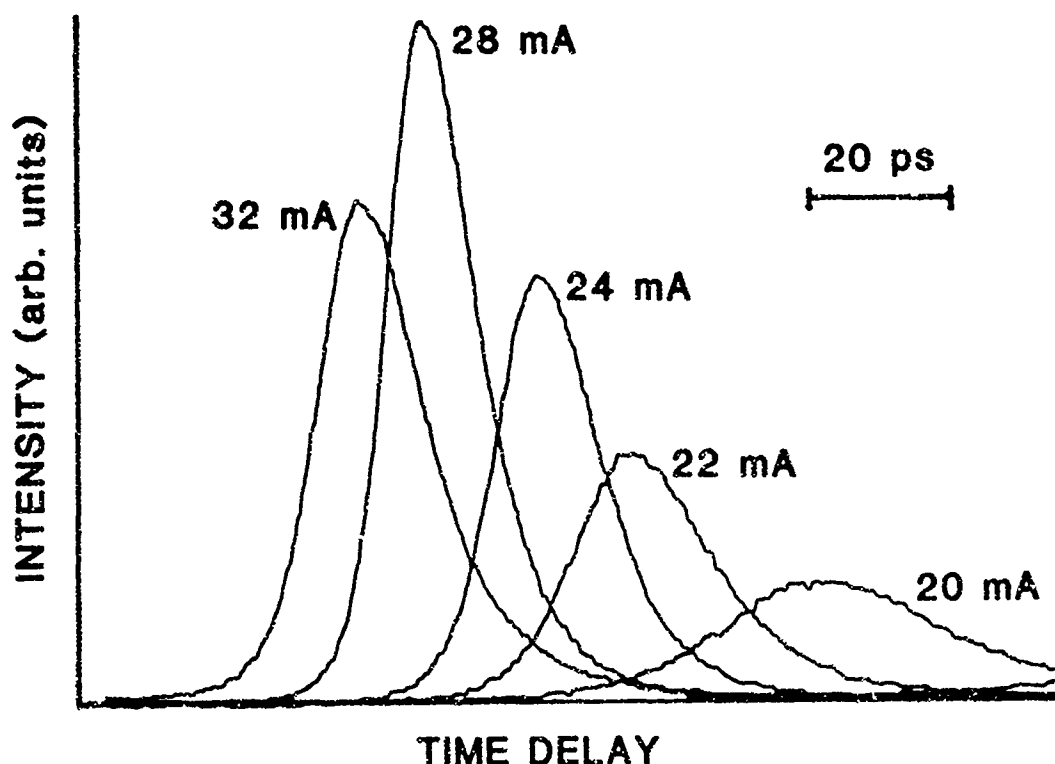
Figure 3. Temporal profiles of the optical pulses from the laser diode operated at 16 °C and driven by 360 mA, 17 ps electrical pulses. The curves are labeled with the dc bias level.
