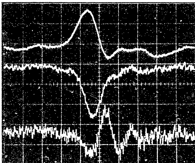
Figure 3: Measured waveforms for the comb generator. Traces are input to the first FET (top), output of the first FET (middle), and output of the second FET (bottom). Horizontal scale is 50 ps/div. Vertical scale is 0.8V/div (top), 0.08 V/div (middle) and 0.04 V/div (bottom).
