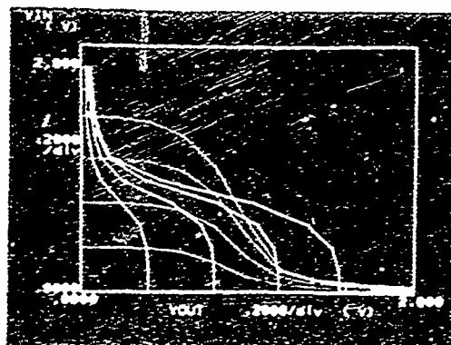
Figure 4 A plot of voltage transfer characteristics for an inverter whose output is linked to the gate of a second MISFET. Two separate traces are obtained by plotting V_{OUT} vs. V_{IN} and repeating the plot after interchanging the axis. Both horizontal and vertical axis extend linearly from 0 volt to 2.0 volts, while V_{DD} is a parameter varying from 0 to 1.6 volts in steps of 0.4 volt. V_{SS} is connected to ground.
