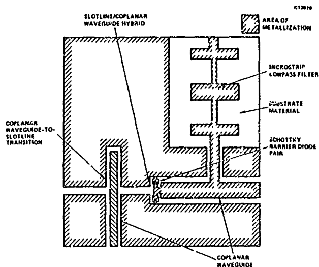
Fig. 2 Planar Balanced Monolithic Mixer Circuit
