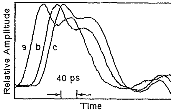
Fig. 3. Transmission line waveforms at a) 0 mm, b) 3.5 mm, and c) 5.0 mm. Propagation delays are 34.8 ps from a to b, and 15.6 ps from b to c.
