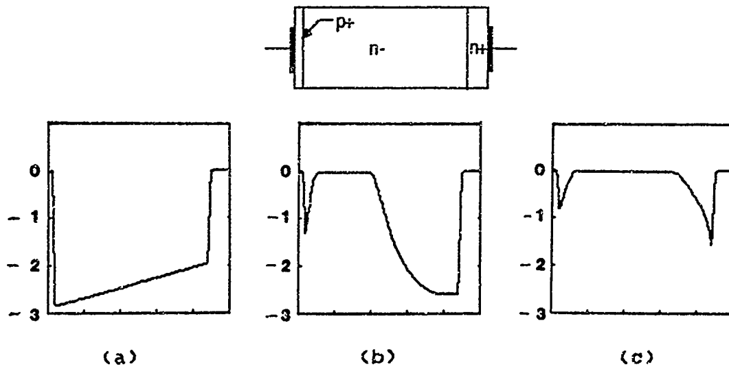
Figure 3. Calculated electric field at three different times during the breakdown process. a) 0.7 ns, b) 0.85 ns, and c) 1.0 ns after trigger (see Fig. 4 for corresponding current and voltage pulses). Scales: V/cm \times 10^5 vert, relative distance across diode horiz.
