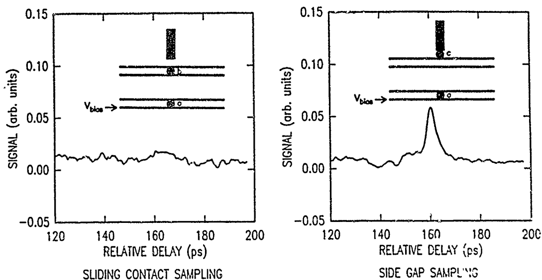
Figure 1: Waveform sampled in a cross talk measurement with the traditional side gap sampling and the sliding contact technique. In both cases a pulse is generated on the bottom transmission line at point "a". Points "b" and "c" are the sampling sites.
