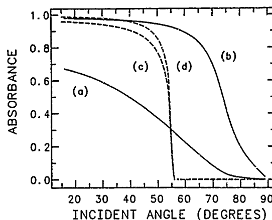
Fig. 3 -- Absorbance of GaAs layer for Se internal reflection element, \lambda = 0.83 \mu\text{m} ., with air gap a) 500 \text{\AA} and b) 100 \text{\AA} ; and for Ge internal reflection element, \lambda = 3.0 \mu\text{m} ., with air gap c) 500 \text{\AA} and d) 100 \text{\AA} (absorbance is \sim 10^{-4} above critical angle for curves c) and d)).
