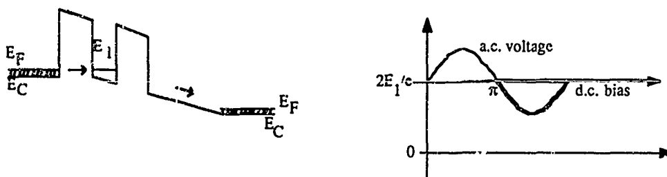
Fig. 1(c). Energy band diagram when the device is biased for the quantum well to be at resonance so that current injection occurs at an instant \pi (the current conduction cycle through the device is highlighted).
