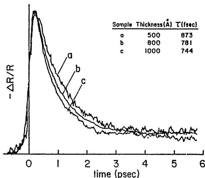
Figure 3. Front surface reflectivity change versus time for various thickness gold films. As the thickness of the film increases, the decay time constant decreases. This can be interpreted as due to the effect of rapid electronic heat transport.
