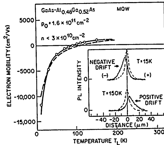
Fig. 3 Minority electron mobility as a function of lattice temperature; the points are experimental and the curve is a comparison with theory. The inset shows the luminescence images, showing negative drift at 15 K and positive drift at 150 K.
