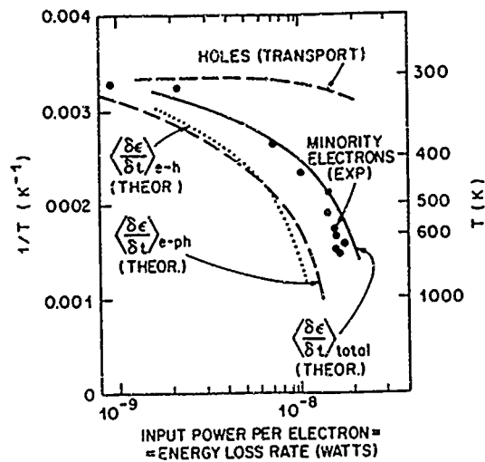
Fig. 2 Inverse of electron temperature vs. electron energy loss rate; circles are experimental and curves are calculated for different scattering mechanisms.
