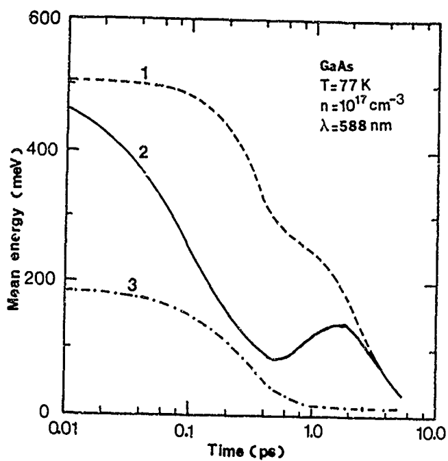
Fig. 2 Mean kinetic energy of the photoexcited electrons in: 1) central valley, 2) central+L-valley, 3) L-valley.
