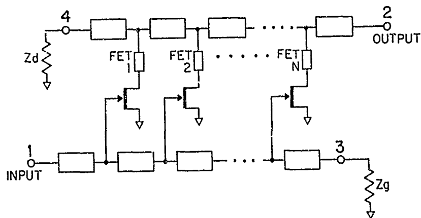
Fig. 1 Distributed amplifier schematic.
