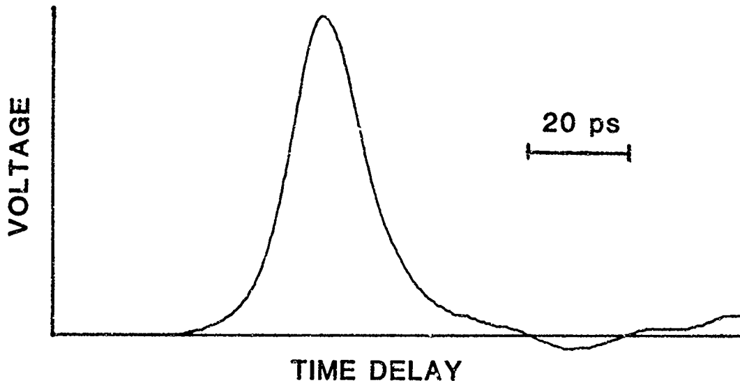
Figure 2. The temporal profile of the electrical pulse used to drive the laser.
