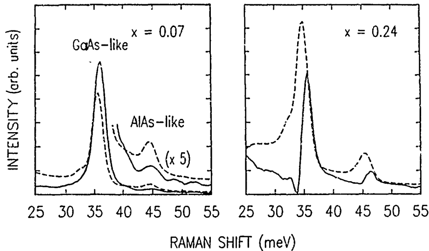
Figure 2. Picosecond Raman scattering from room temperature \text{Al}_x\text{Ga}_{1-x}\text{As} excited by 5 psec (autocorrelation FWHM) pulses at 567nm. Dashed curves are spectra from thermal phonons, excited when the probe precedes the pump by 10 psec. Solid curves are the additional scattering (multiplied by 5) due to nonequilibrium phonons when the probe follows the pump by 2 psec. The slight frequency shift between thermal and nonequilibrium phonons is due to a slight LO phonon-plasmon coupling at our injected carrier concentration of about 10^{17} \text{ cm}^{-3} .
