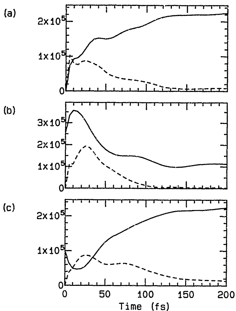
Figure 2. Transient response of the device structure of Figure 1. The solid line shows the current density (in \text{A/cm}^2 ) averaged over the structure and the dashed line shows the standard deviation from this average (to provide a measure of the convergence to steady-state). In (a), the voltage was switched from 0 to the peak value at t=0 . In (b) it was switched from the peak to the valley. In (c) it was switched from the valley to the peak.
