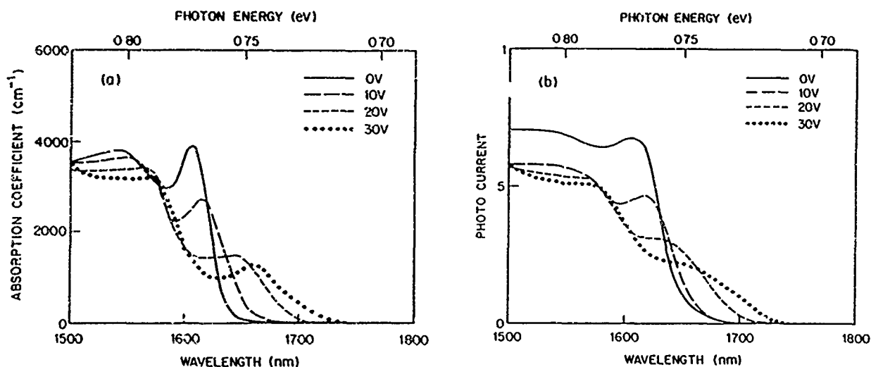
Figure 2: Absorption (a) and photocurrent (b) spectra in the vicinity of the n_z=1 .
