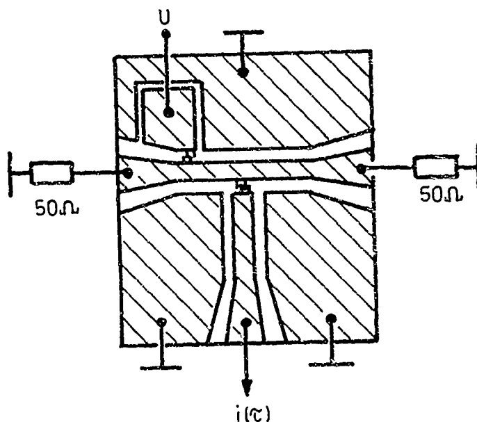
Fig.5: Schematic arrangement for measuring i(\tau)
