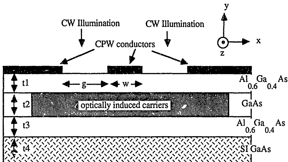
Figure 1: Cross section used to model pulse propagation (in the z direction) on a coplanar waveguide phase shifter; t_1 = 0.1 \mu\text{m} ; t_2 = 3.2 \mu\text{m} ; t_3 = 3.4 \mu\text{m} ; t_4 = 250 \mu\text{m} ; d = 12 \mu\text{m} ; g = 7 \mu\text{m} ; w = 10 \mu\text{m} .
