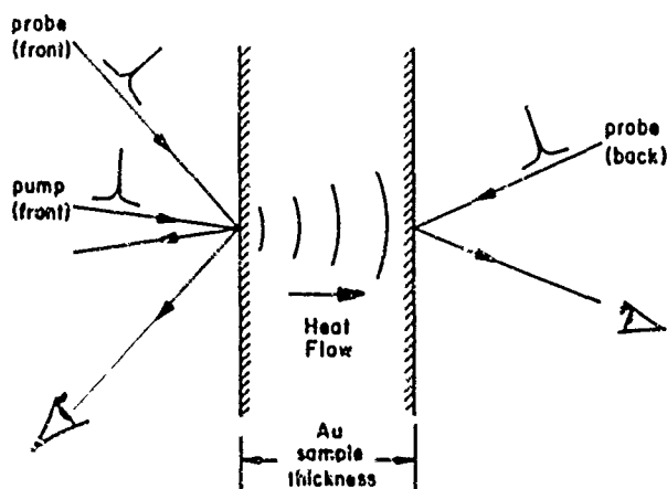
Figure 1. Simplified schematic of the thermomodulation experiment. In the usual case, the sample is pumped and probed on the front surface. By probing the back, we are able to measure the transport of heat across the sample.
