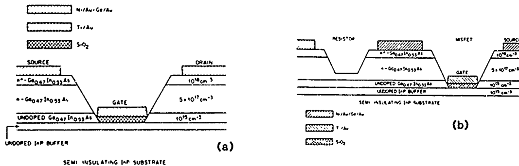
Figure 1 (a) Cross sectional view of the MISFET structure; (b) Cross sectional view of MISFET and integrated load resistors. Both figures not to scale.
