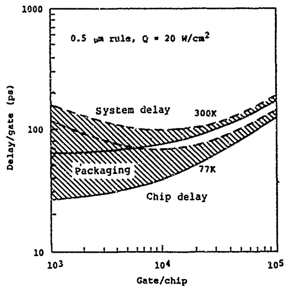
Fig. 4 Chip and system delays calculated as a function of complexity.
