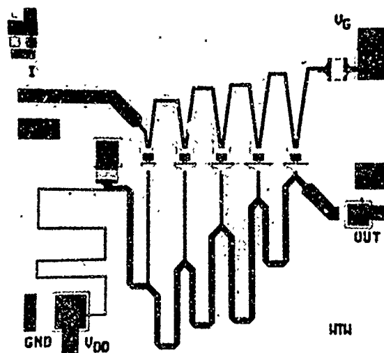
Fig. 6 HEMT distributed amplifier.
