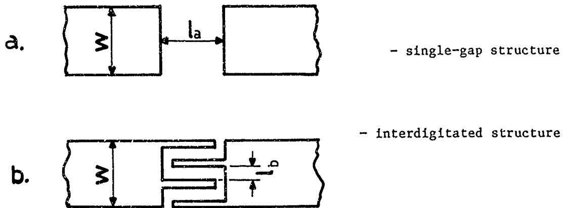
Fig. 1 Detector structures
