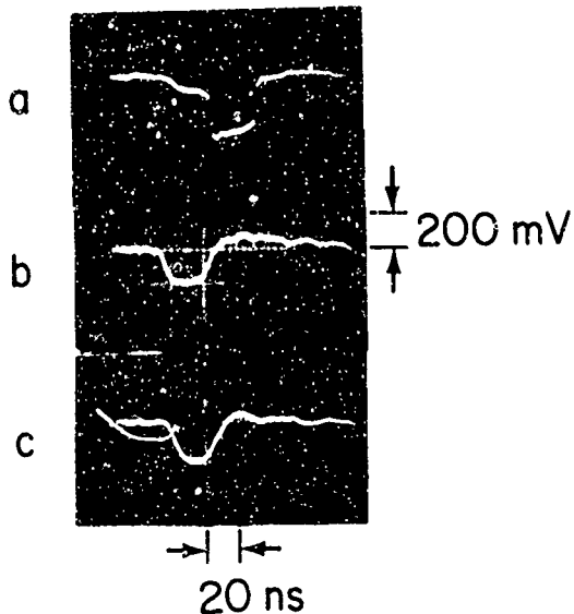
Fig. 2: Three examples of waveforms generated as the graphite switch opens. Each trace is obtained with a different laser pulse but the sample of graphite is the same. The laser pulse energy is: a: 0.15 mJ, b: 0.14 mJ, c: 0.16 mJ.
