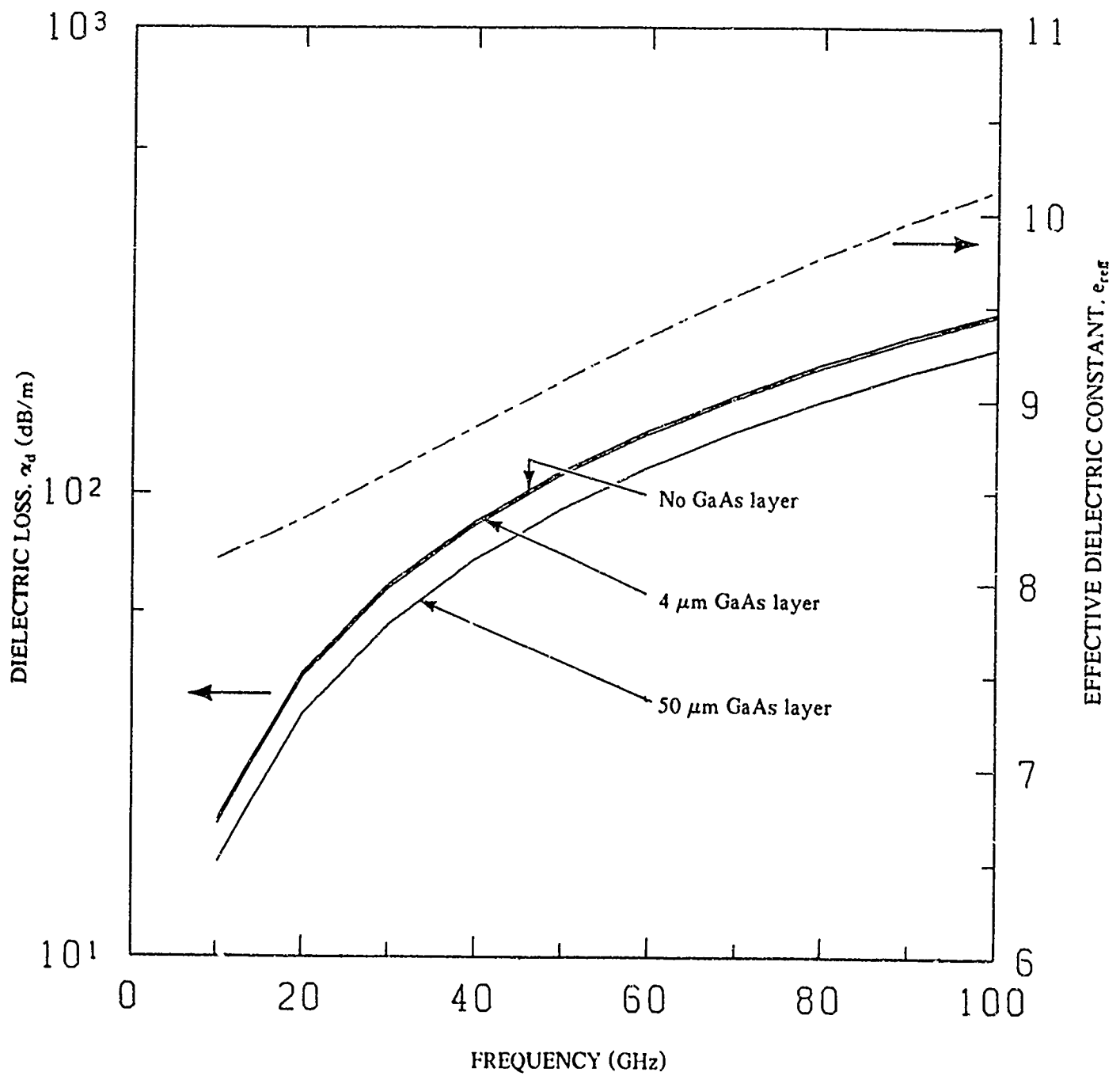
Fig. 2. Dielectric loss and effective dielectric constant versus frequency for \rho_{Si} = 2000 \Omega\text{-cm} , \rho_{GaAs} = 4000 \Omega\text{-cm} .
