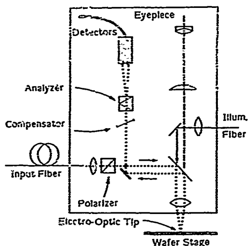
Fig. 2. Schematic of the probe sampling system (not to scale)
