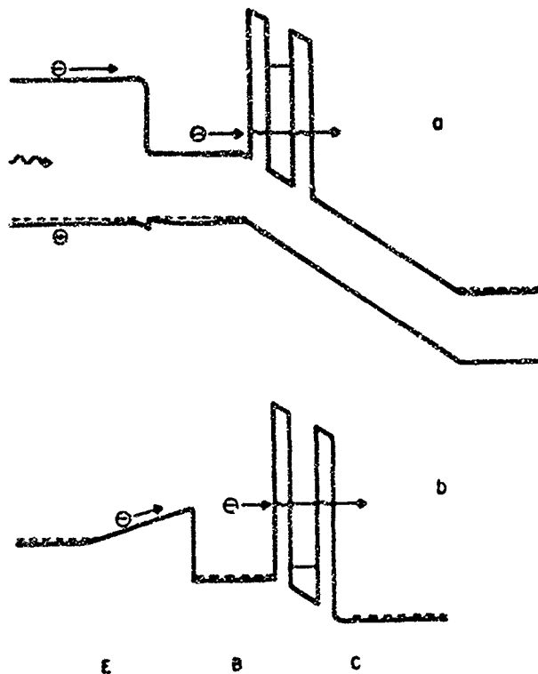
Fig. 1 a. Band diagrams of structure used for resonant tunneling spectroscopy (RTS) of hot minority carrier electrons.
