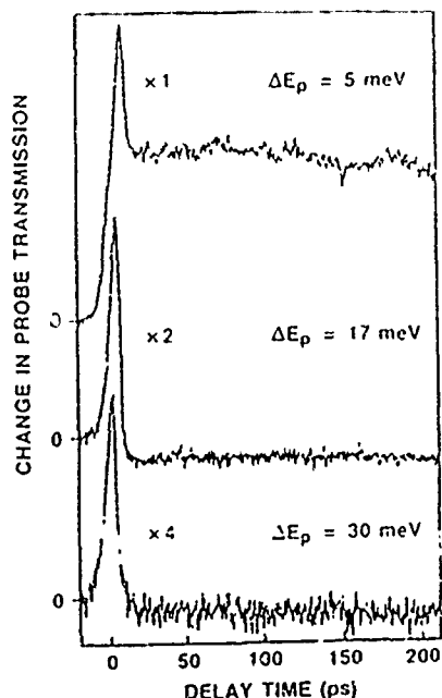
Fig. 2 Change in probe transmission as a function of the time delay between pump and probe. As the detuning \Delta E_p increases the fast component due to the AC Stark shift dominates the slow component associated with free carrier bleaching of the exciton.
