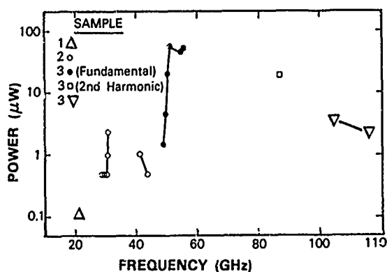
Figure 1. Output power as a function of frequency for recent resonant-tunneling oscillators. The connected dots indicate continuous tunability in a particular waveguide structure. All measurements were made at room temperature.
