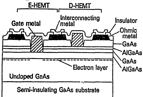
Fig. 2 Cross sectional view of a self-aligned gate E/D-HEMTs.
