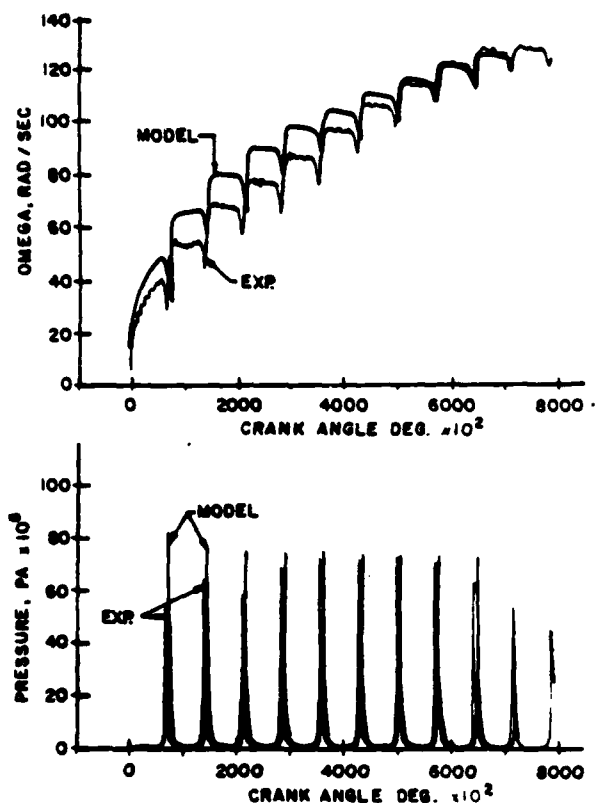
Figure 9 - Instantaneous Angular Velocity and Cylinder Pressure During Cranking and Starting from the Model and Experiment
