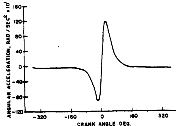
Figure 8 - Instantaneous Angular Velocity and Acceleration, 1100 rpm, No Load
