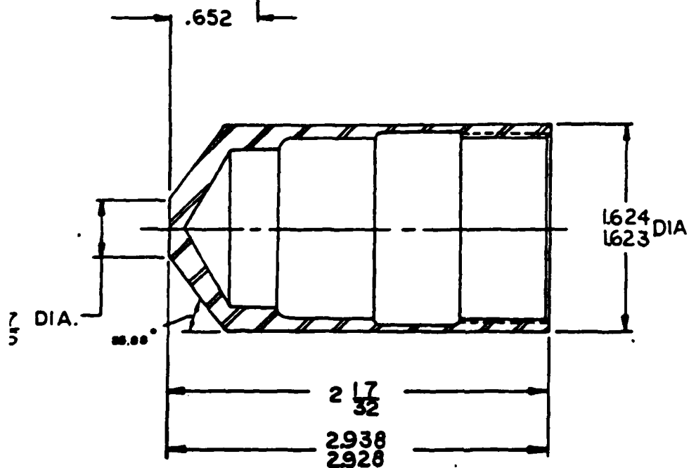
TRUNCATED CONICAL EXPERIMENTAL HIGH COMPRESSION PLUG
