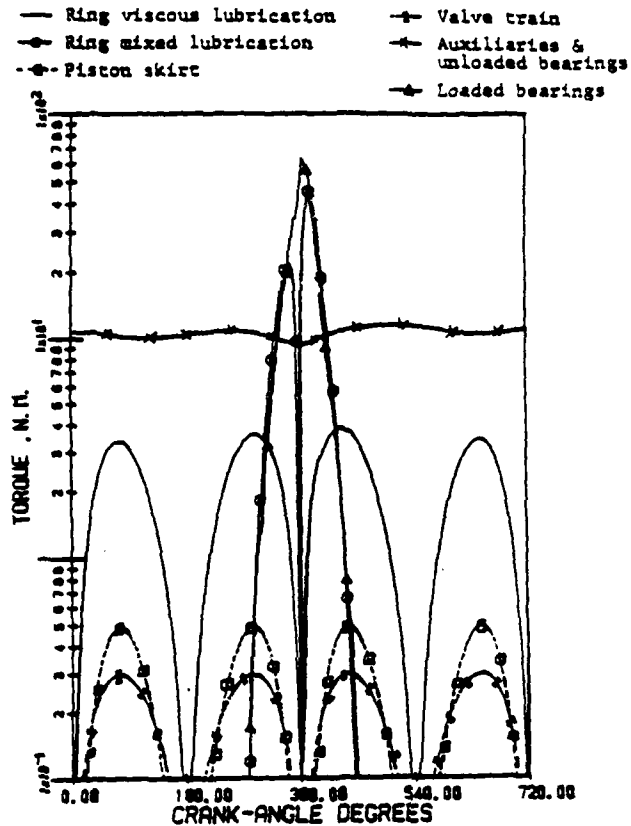
Figure 3 - Instantaneous Friction Components From Model Correlations (Ref.18) 900 rpm, No Load
