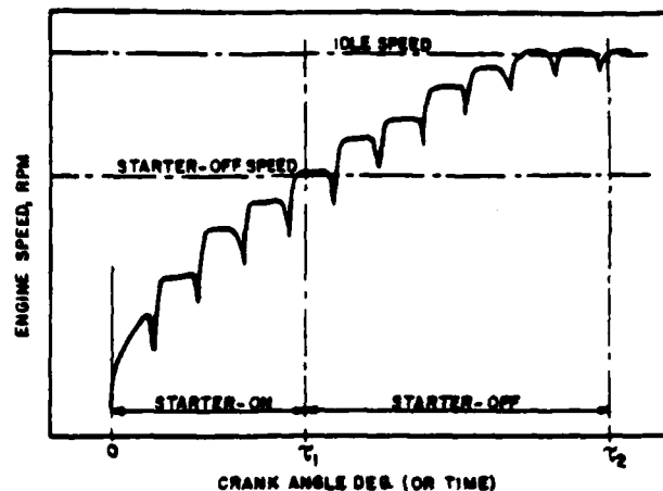
Figure 1 - Model for Starting Process
