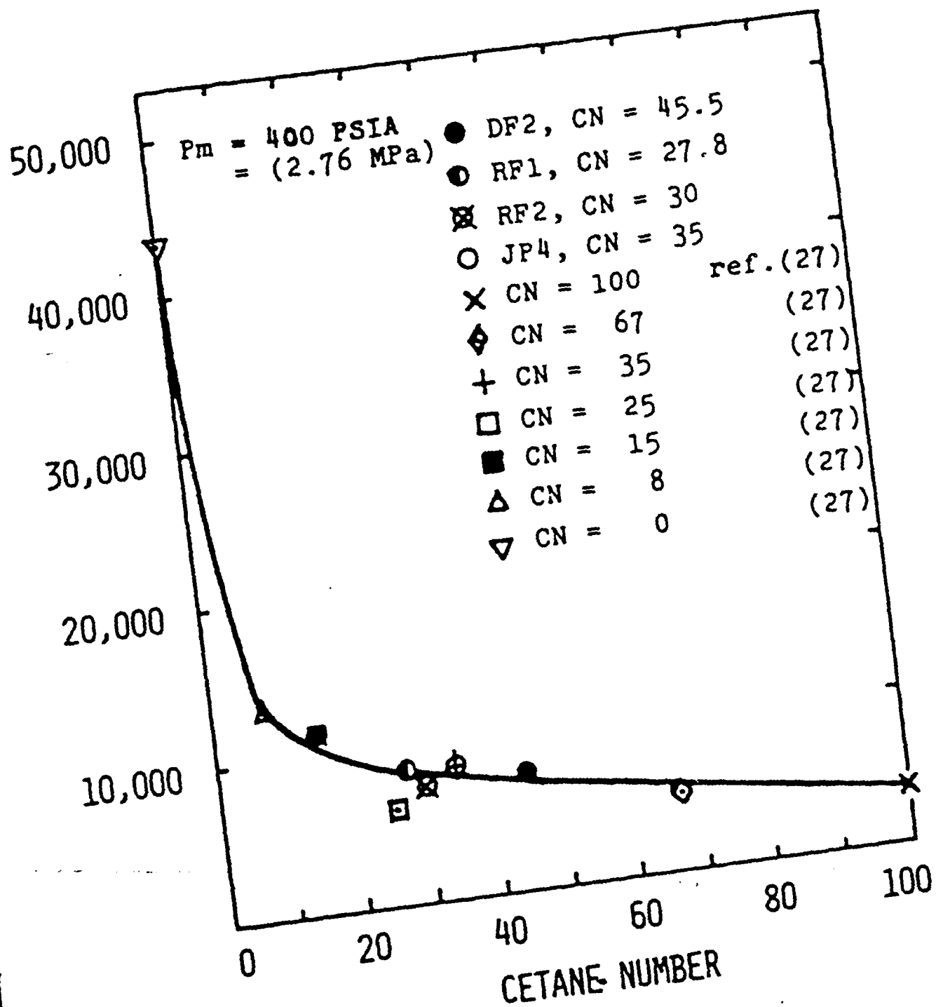
Fig. (17): Relationship between E and C.N. at P_m = 400 \text{ PSIA} .
