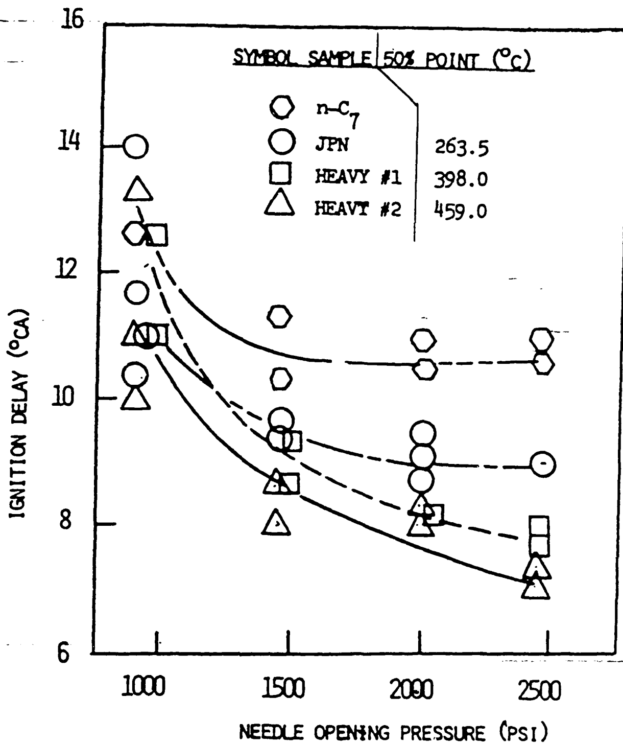
Fig. (11): Effect of needle opening pressure on I.D. in the CFR-Cetane engine.
