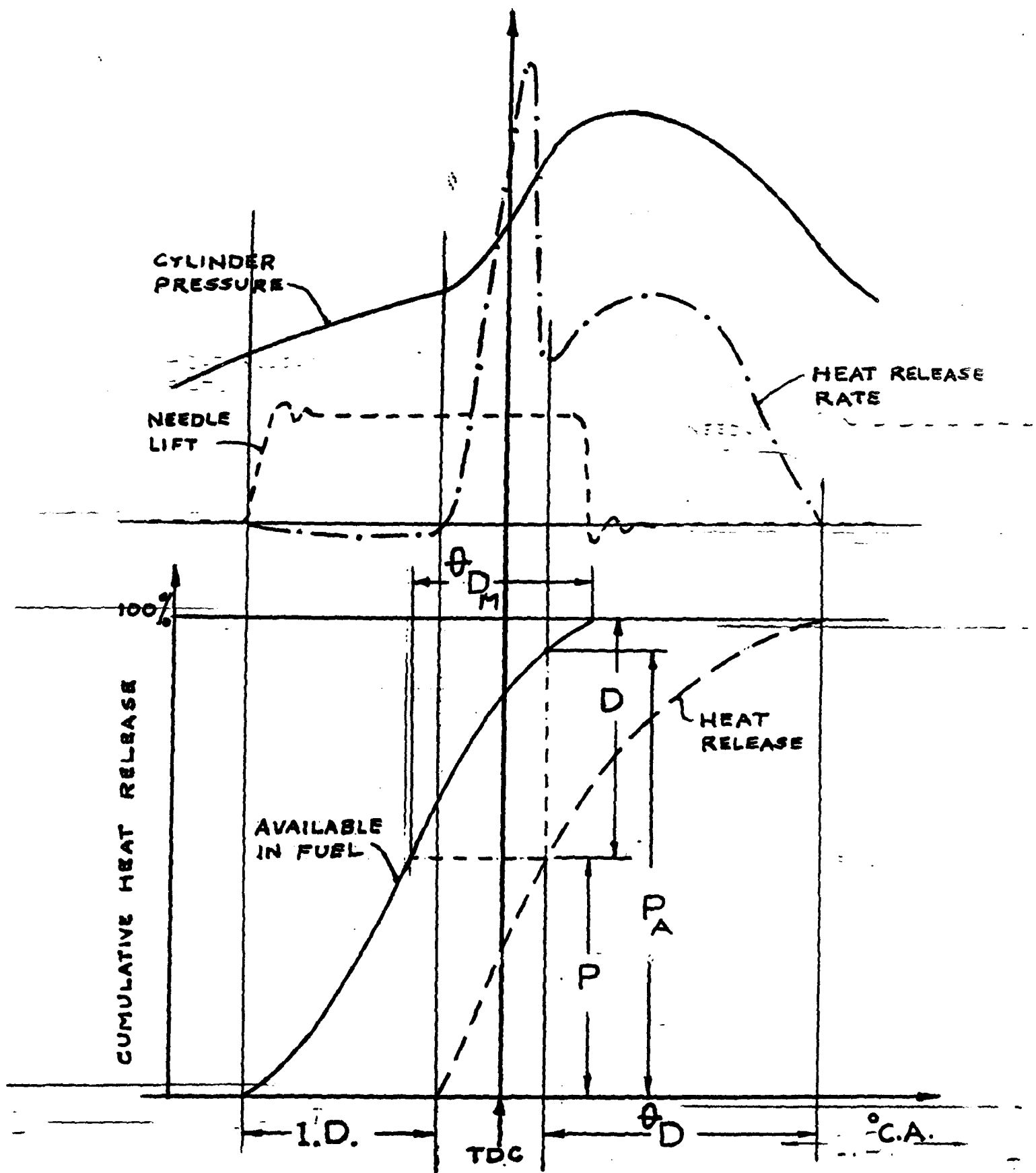
Fig (18): Global Combustion Parameters for Diesel engines.
