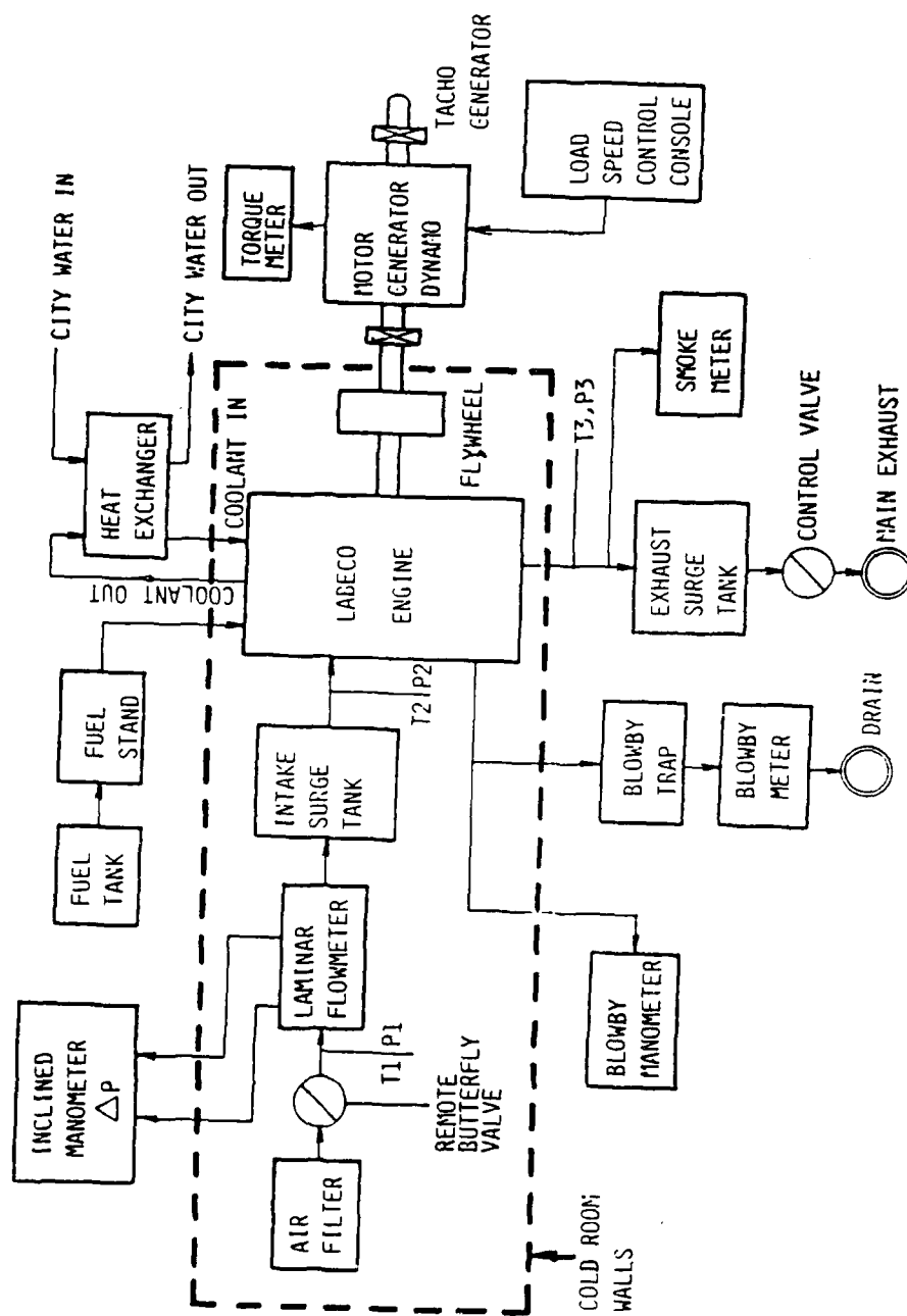
Figure 42 Layout of Experimental Setup
