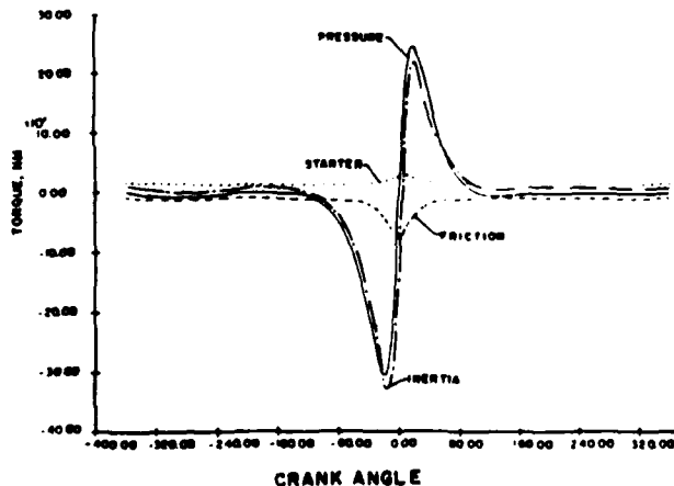
Figure 7 - Instantaneous Torque Components 1100 rpm, No Load
