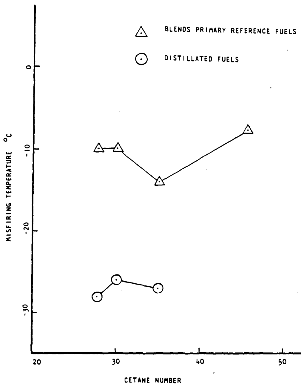
Figure 44 Variation of Misfiring Temperature with Cetane Number for Distillated and Blend Fuels
