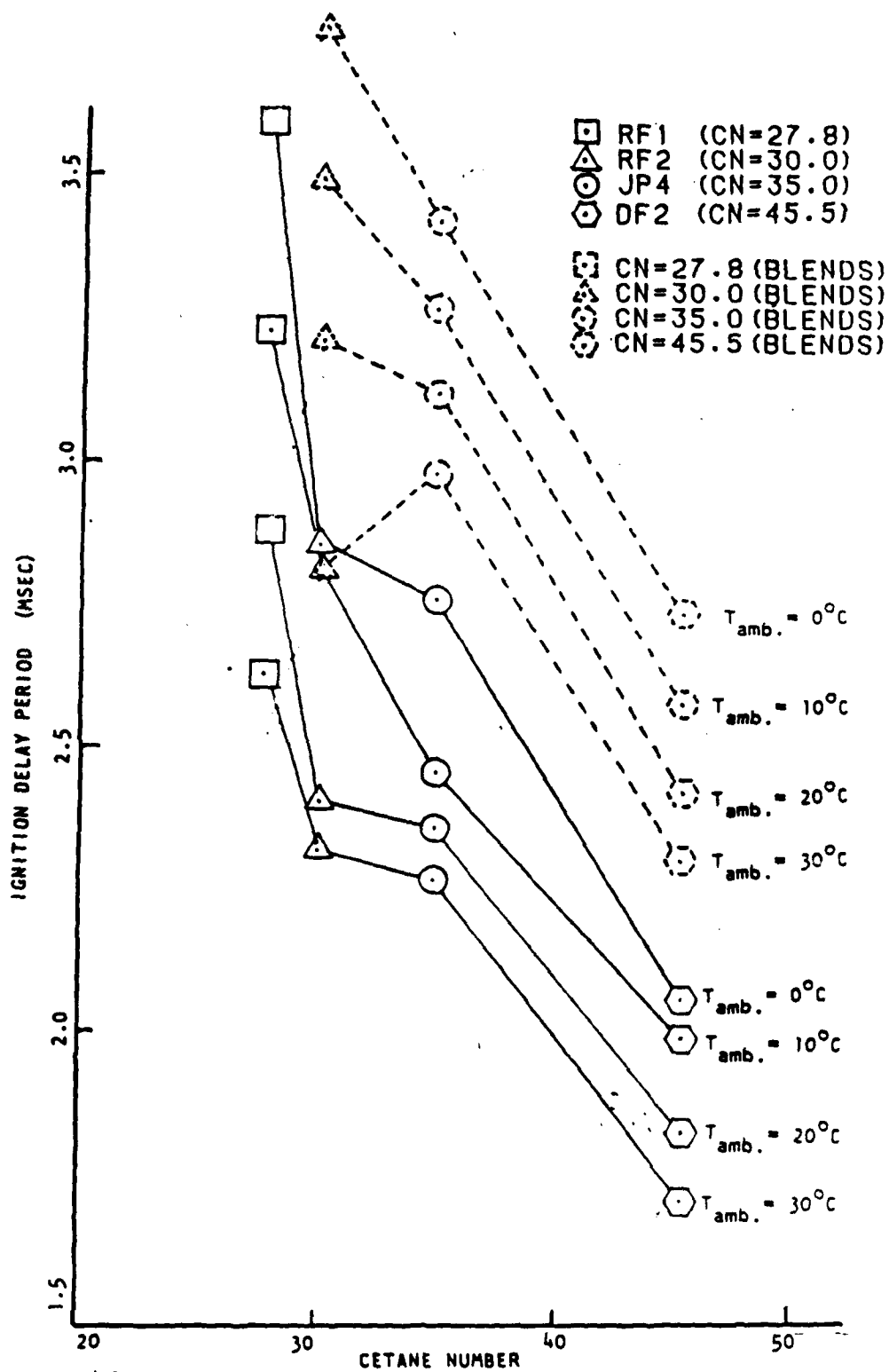
Figure 46 Variation of Ignition Delay Period with Cetane Number at Different Ambient Temperature (distillated and blend fuels)
