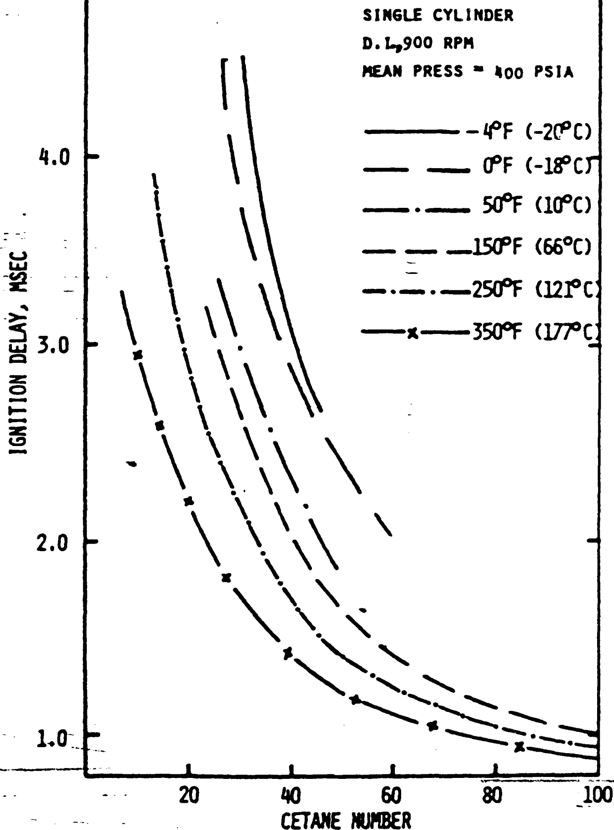
Fig. (13): Effect on C.N. on I.D. at different inlet air temperatures.
