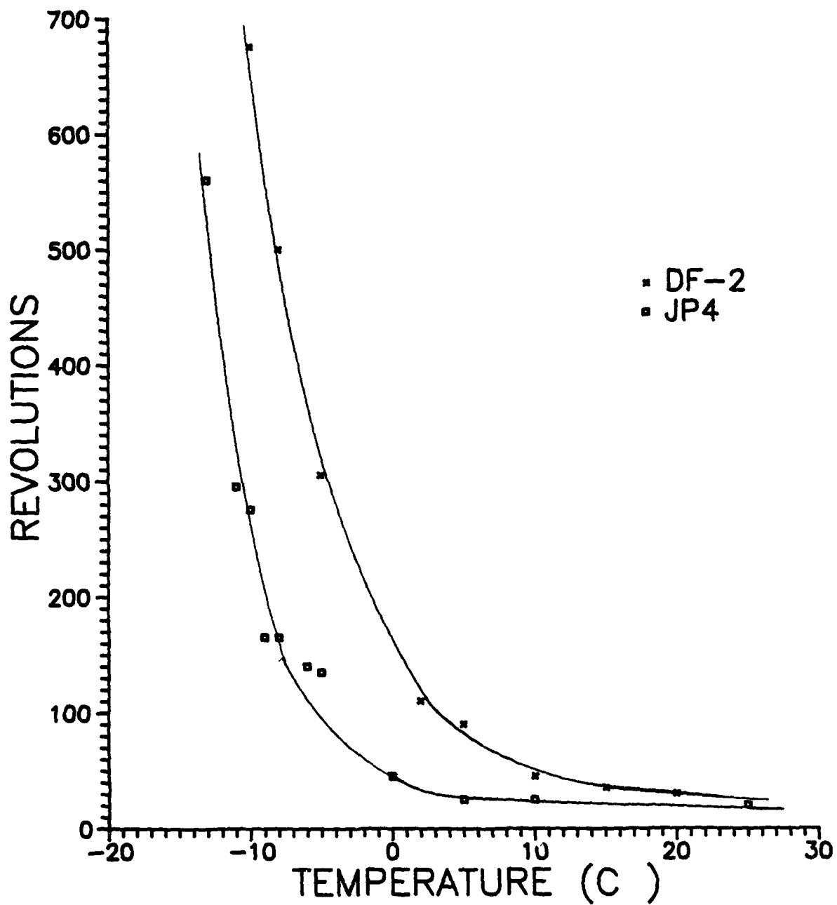
Fig. 41 Comparison between the engine revolution to maximum starting speed on DF 2 and JP4 fuels.
