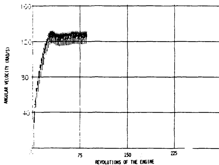
Fig. 22 Plot of angular velocity vs. engine revolutions, Fuel: DF 2, Oil: arctic oil, ambient temperature: 20 C, cold soak time: 5 hrs., startability conditions Started easily.
