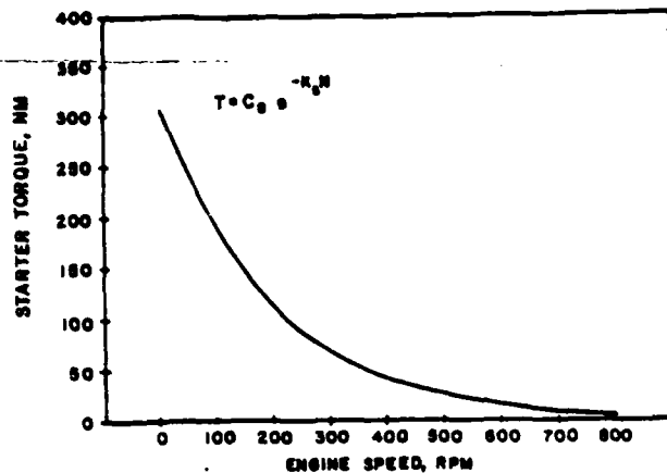
Figure 6 - Starter Motor Torque as a Function of Engine Speed
