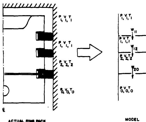
Figure 5 - Model for Blowby Gas Flow Past the Piston Rings
