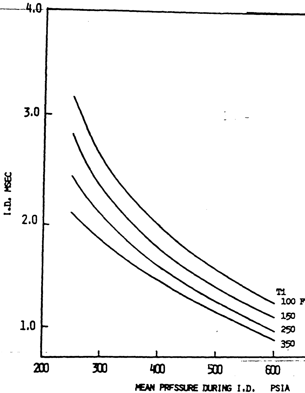
Fig. (15): Effect of mean pressure on I.D.
