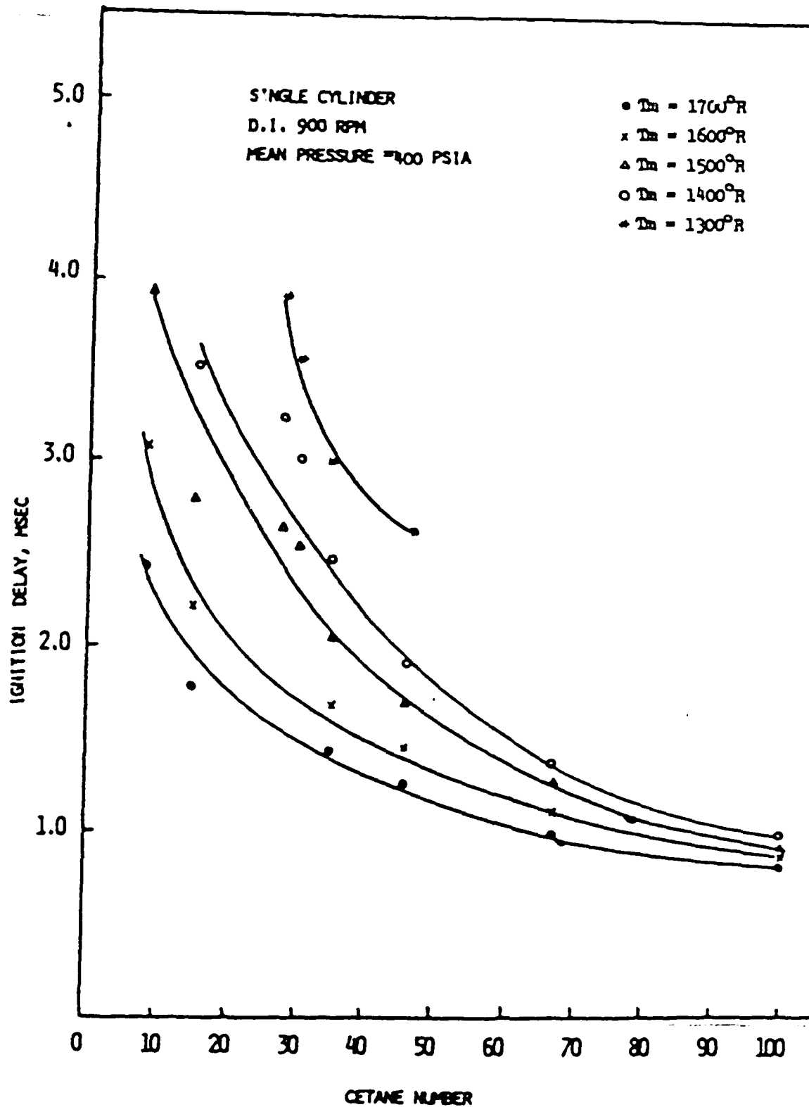
Fig. (14): Effect of C.N. on I.D. at different mean temperature during I.D.
