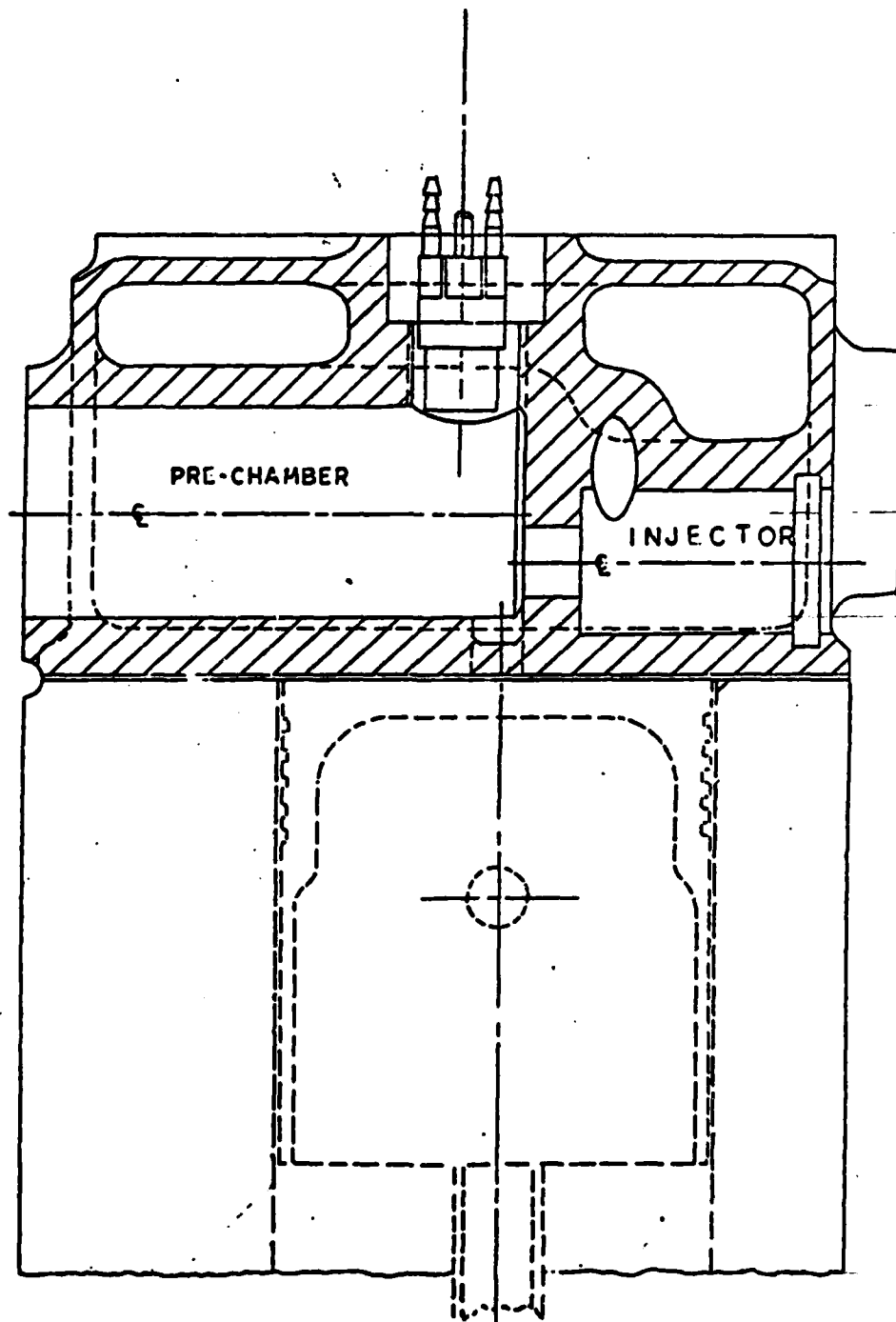
Fig. (9): Cross-section A-A of figure 6 showing the injector and pre-chamber in the CFR-Cetane engine.
