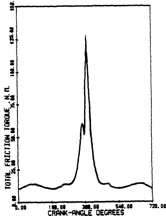
Figure 4 - Total Friction Torque (Ref.18) 900 rpm, No Load
