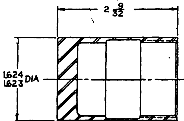
STANDARD FLAT COMPRESSION PLUG
