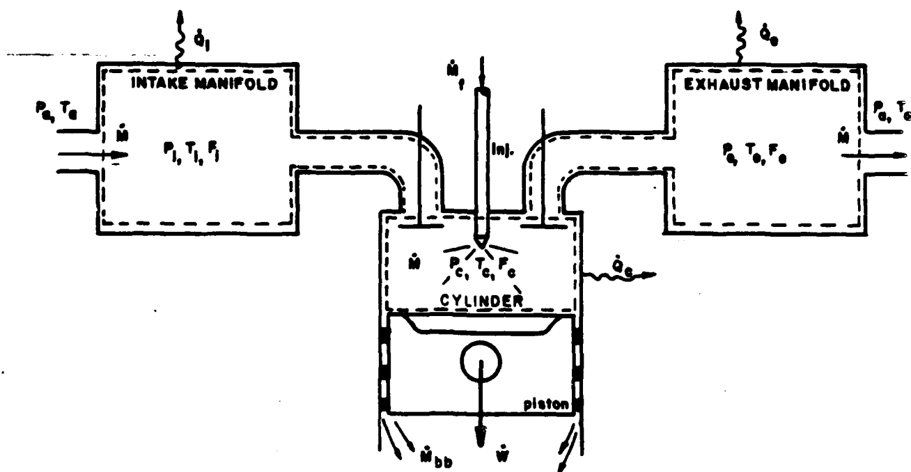
Figure 2 - Engine Thermodynamic System
