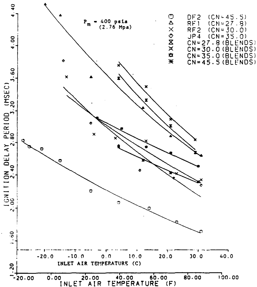
Figure 45 Variation of Ignition Delay Period with Inlet Air Temperature at P_E=400 \text{ psia} (2.76 MPa), for Distillated and Blend Fuels
