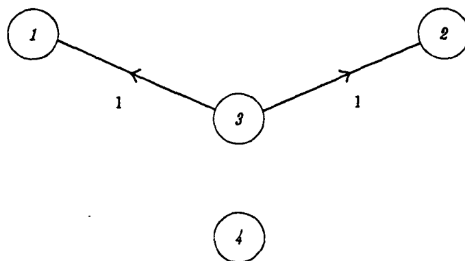
(a) O(1) time scale model — A^{(0)}
