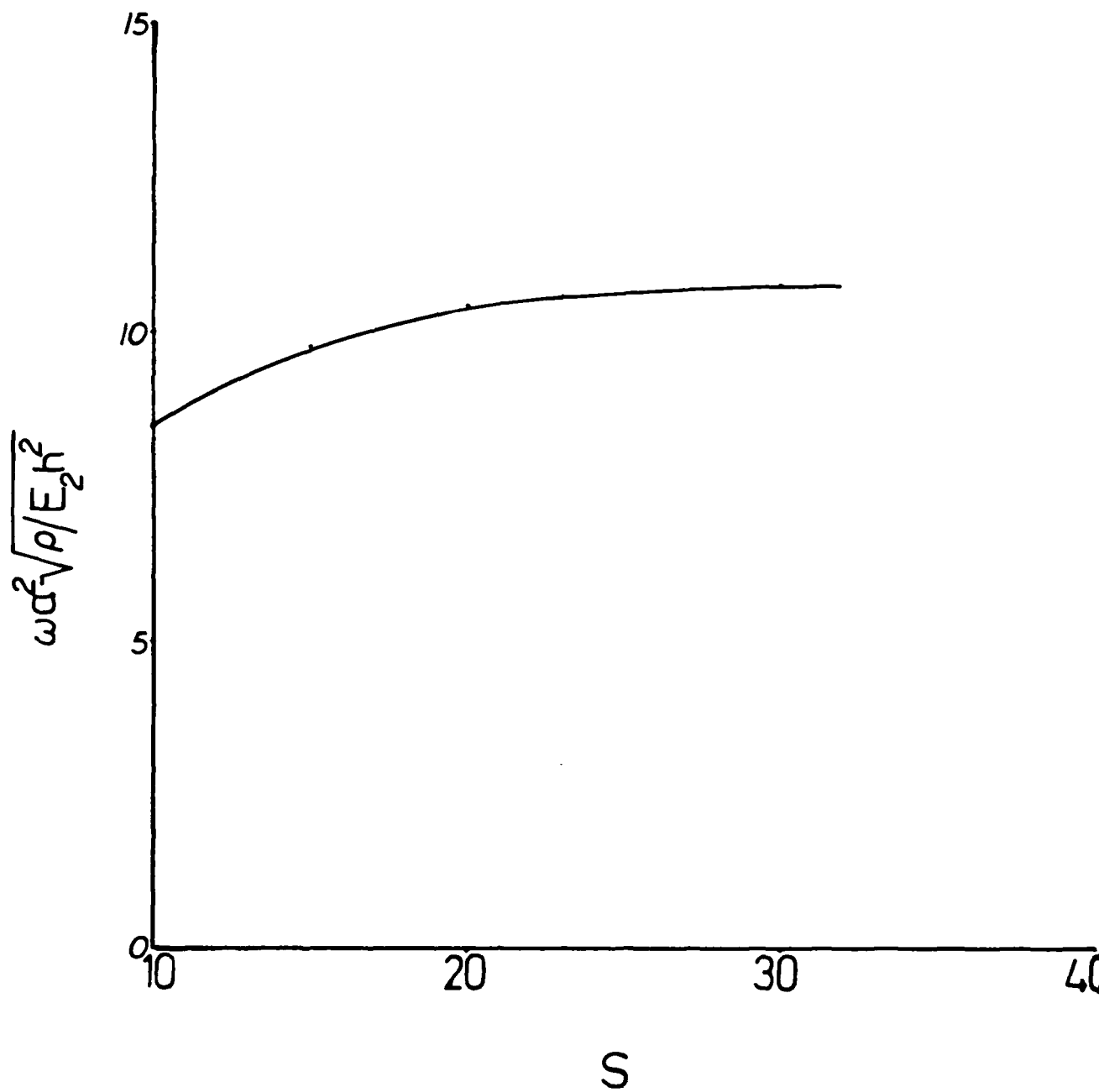
Figure 3.7 Plot of Frequency vs Thickness Ratio For Simple-Simple Boundaries.
