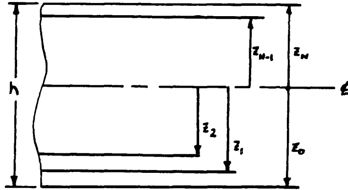
Figure 2.3. Geometry of laminate consisting of N lamina
