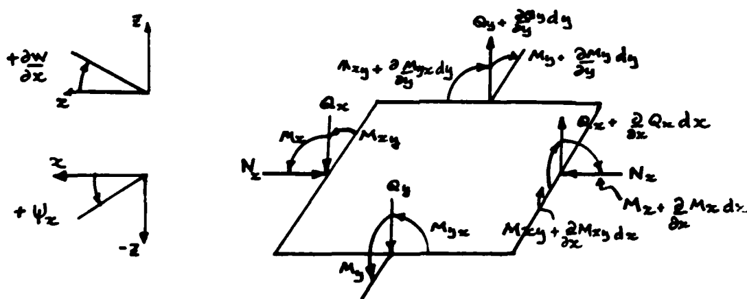
Figure 2.4. Moment and Shear Resultants on Plate
