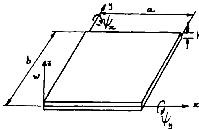
Figure 2.2. Coordinate System of Plate
