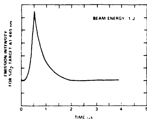
FIG. 2. Temporal behavior of the luminescence signal of the evaporant plume of \text{SiO}_2 at 440-nm wavelength.
