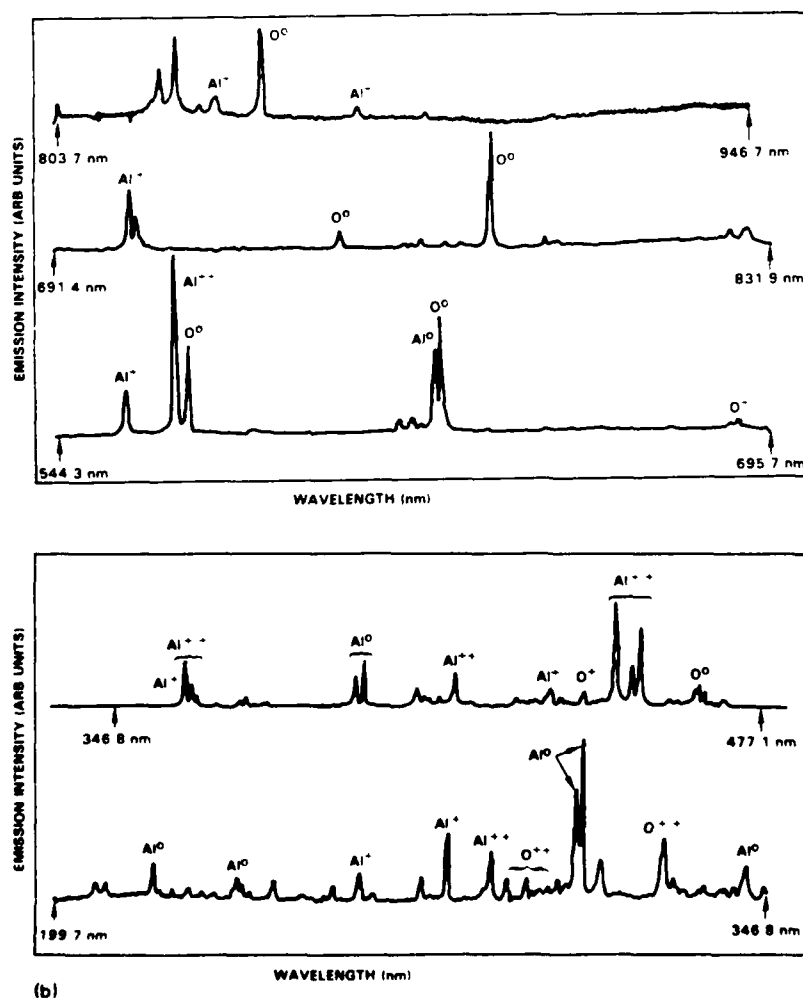
FIG. 3. Spectrum of the luminescence of the evaporant plume of \text{Al}_2\text{O}_3 under TEA- \text{CO}_2 laser radiation. (Power density > 10^4 \text{ W/cm}^2 .)
