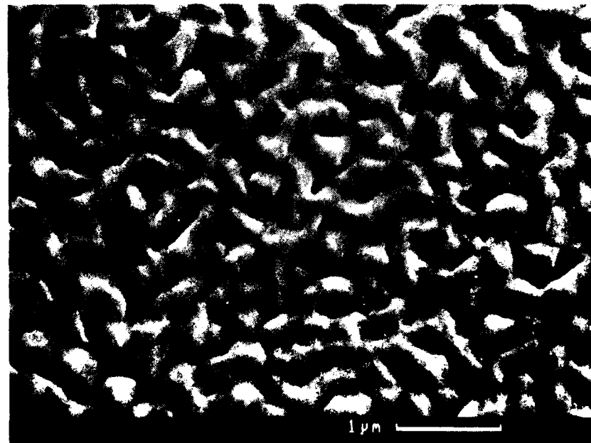
Fig. 11 Surface morphology of Ge films deposited on Si substrates at 300°C. (a) Thermal evaporation, and (b) pulsed laser evaporation.
