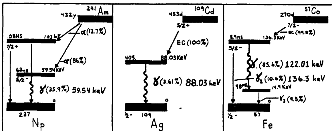
Figure 3.3. ^{109}\text{Cd} Decay Scheme (38:250)
