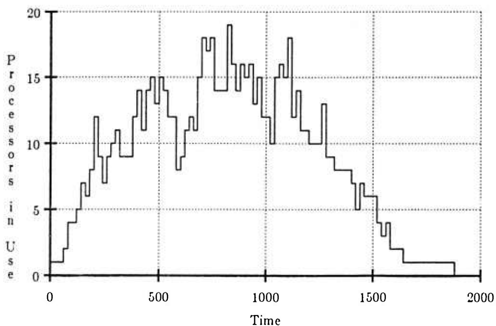
Figure 10. QSORT: Number of processors in use
