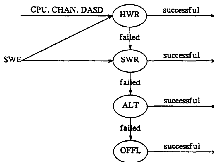
Figure 2. Flow chart of recovery processes
