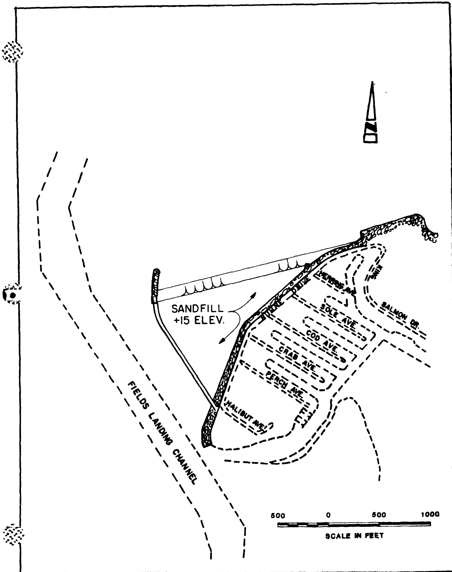
Figure 12. Phase II General Plan
