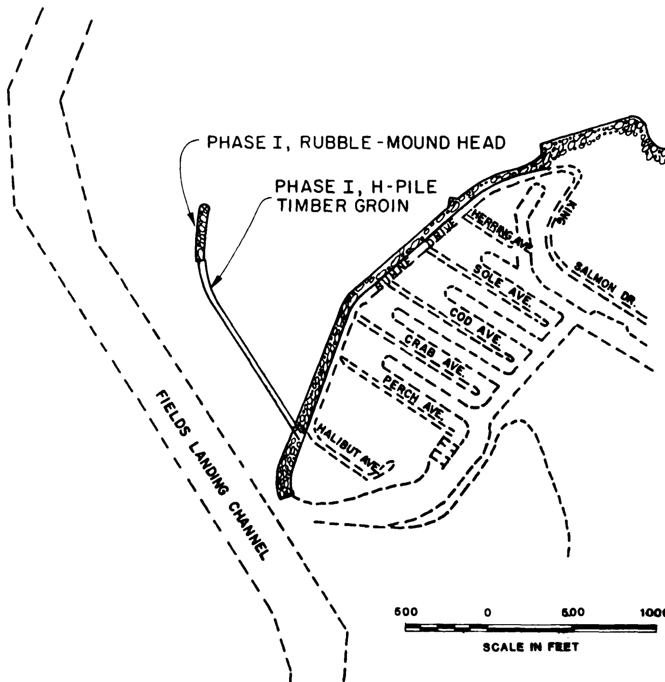
Figure 9. Phase I General Plan
