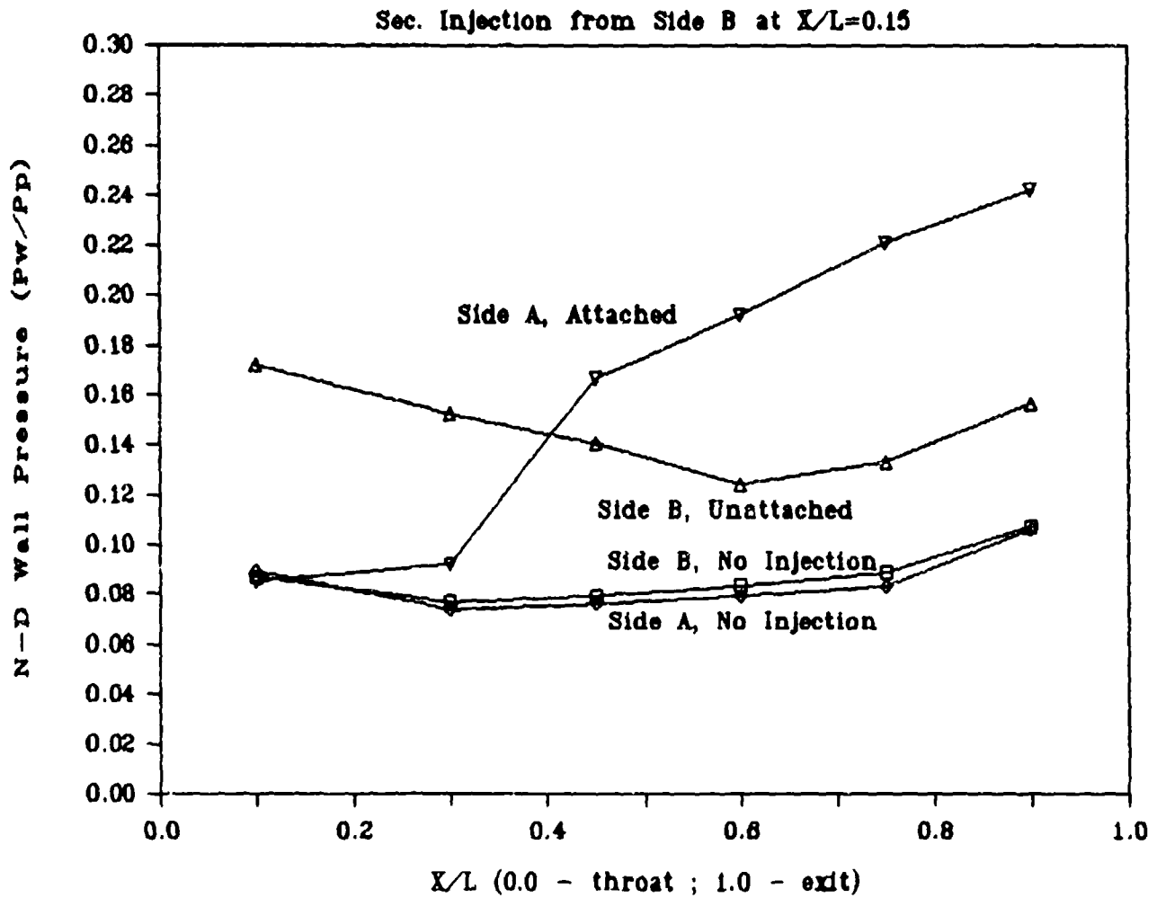
Fig 36. Wall Pressure Distribution of Vecteded Condition LM, A_s/A_t = 0.20 , P_p = 194.4 psia, P_s/P_p = 0.33
