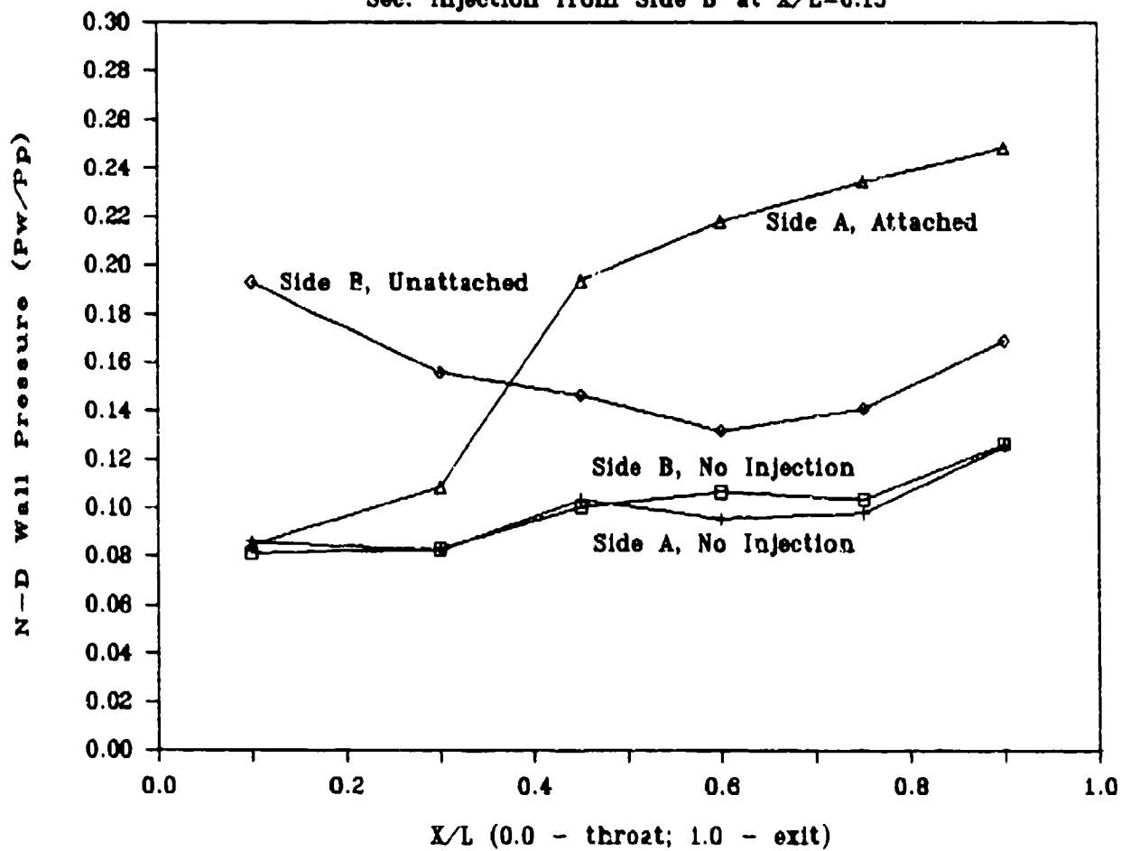
Fig 48. Wall Pressure Distribution of Vectored Condition LM, A_s/A_t = 0.20 , P_p = 154.4 psia, P_s/P_p = 0.42
