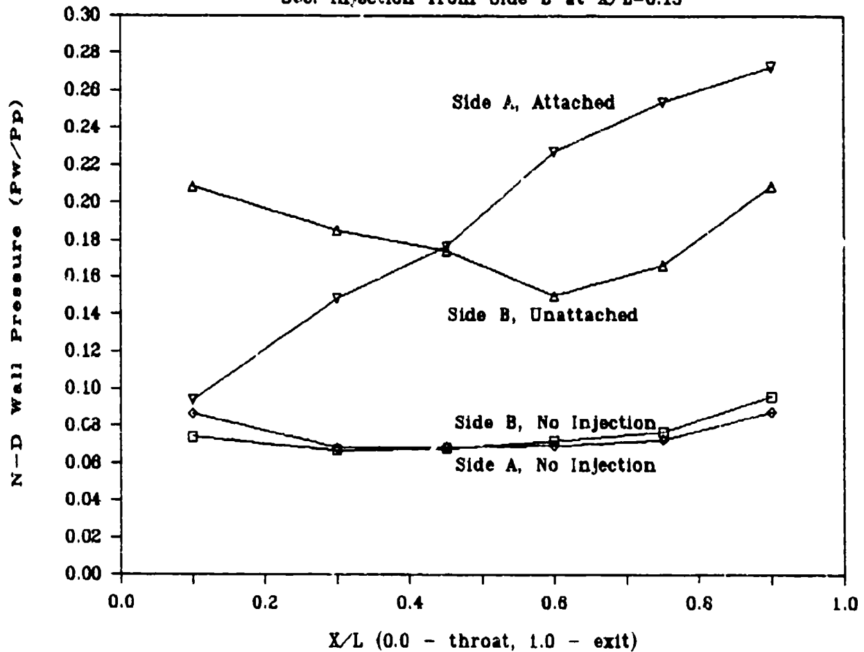
Fig 47. Wall Pressure Distribution of Vektored Condition LM, A_s/A_t = 0.20 , P_p = 174.4 psia. P_s/P_p = 0.54
