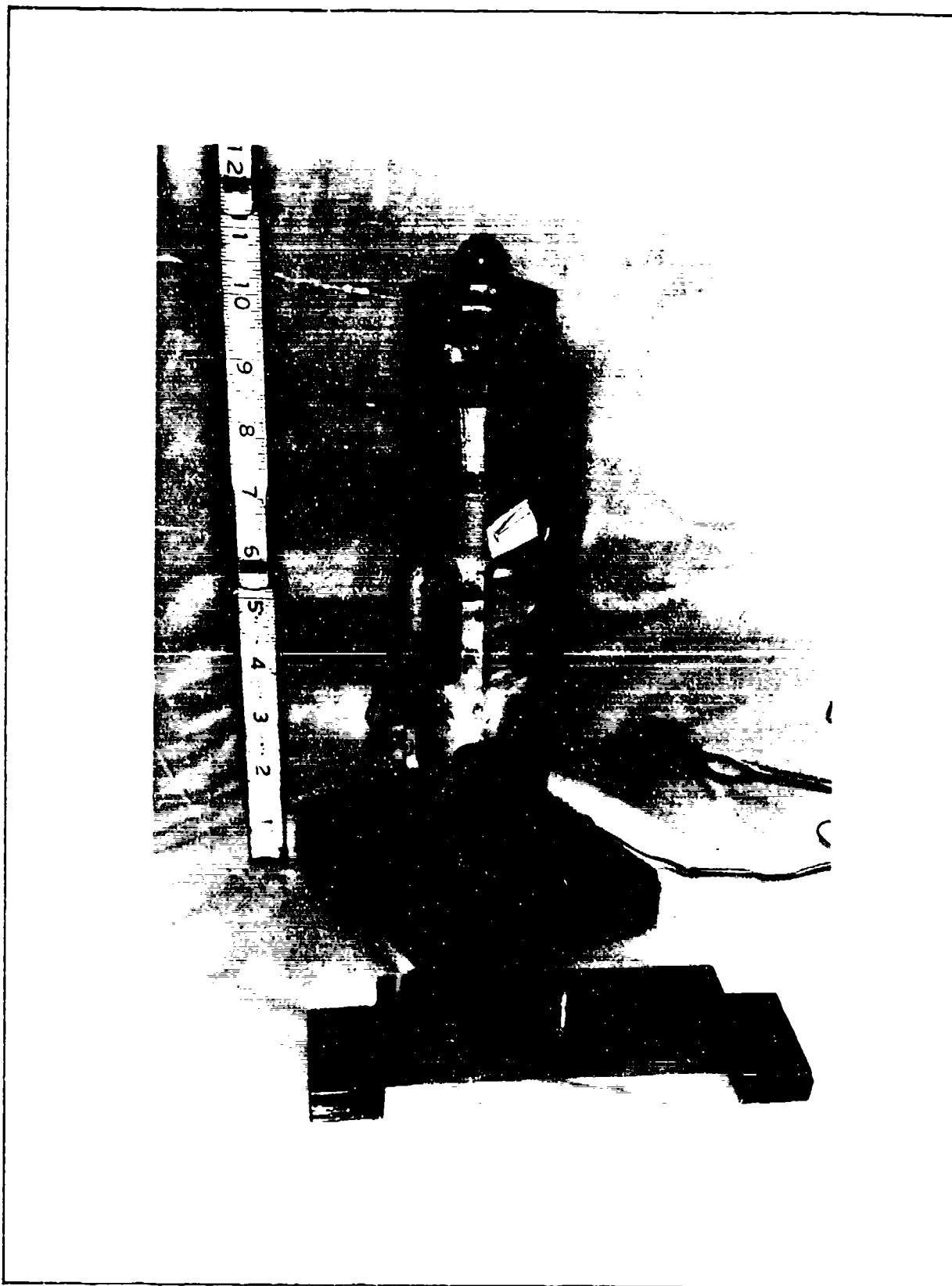
Fig 11. Load Cell with Adapter for Nozzle Bracket
