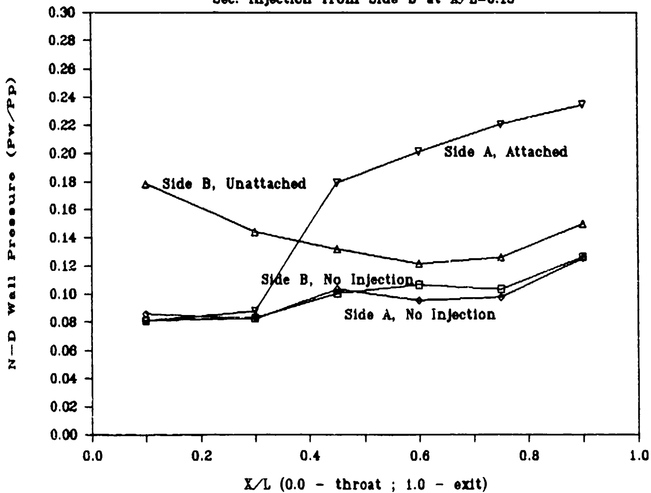
Fig 35. Wall Pressure Distribution of Vected Condition LM, A_s/A_t = 0.20 , P_p = 154.4 psia, P_s/P_p = 0.35
