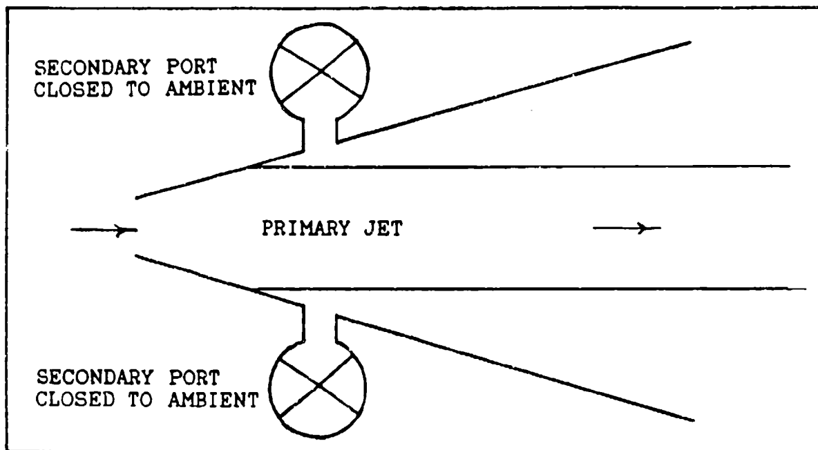
Axial
