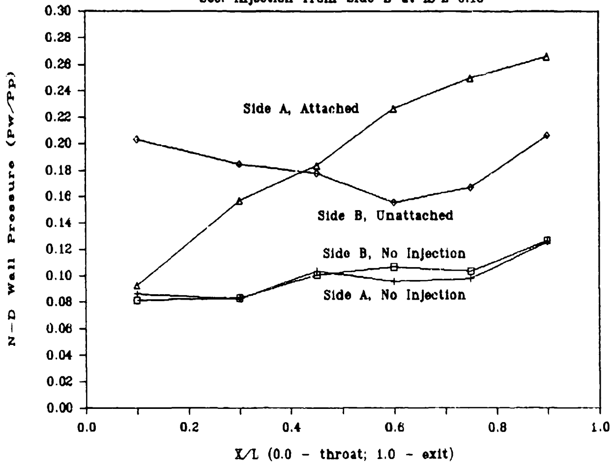
Fig 51. Wall Pressure Distribution of Vectored Condition LM, A_s/A_t = 0.20 , P_p = 154.4 psia, P_s/P_p = 0.61
