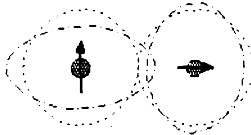
Two Electrons Moving at Right Angles
