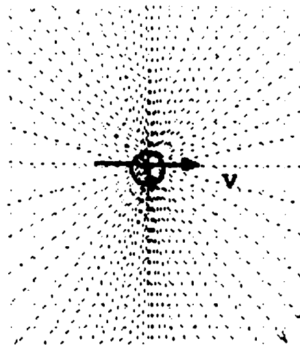
Charged Particle with Velocity V
