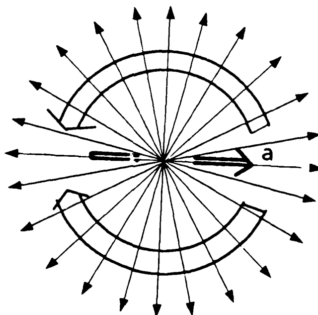
Change of Symmetry Due to Acceleration a
