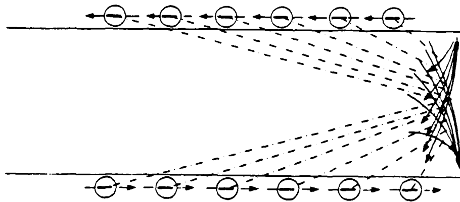
Propagation of a Wave Front Applying Huygen's Principle
