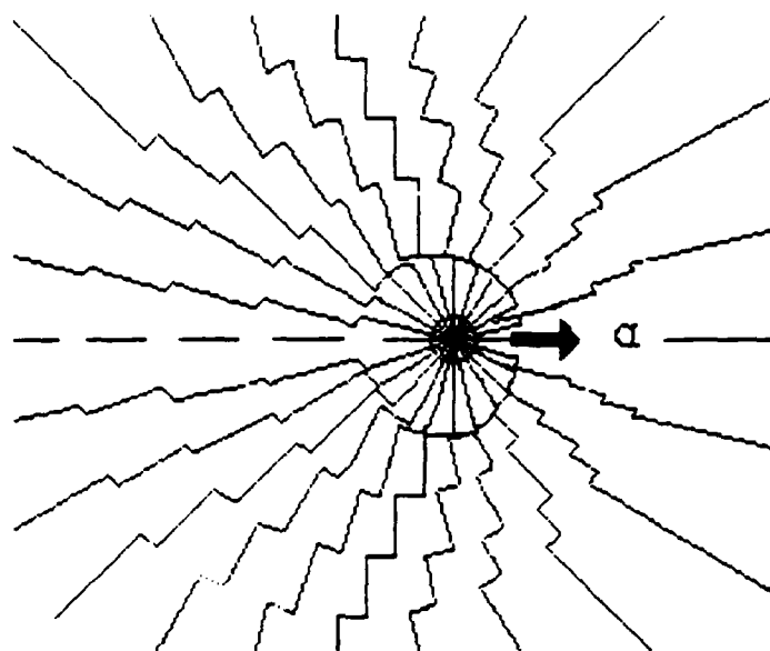
Model for a Jumping Charge Carrier
