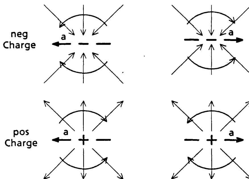
Representation of Circular Waves for Different Charges and Different Direction of Acceleration
