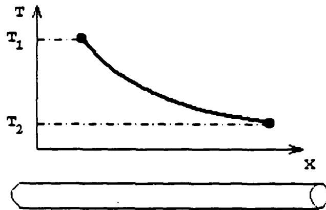
Heat Flow along a Rod
