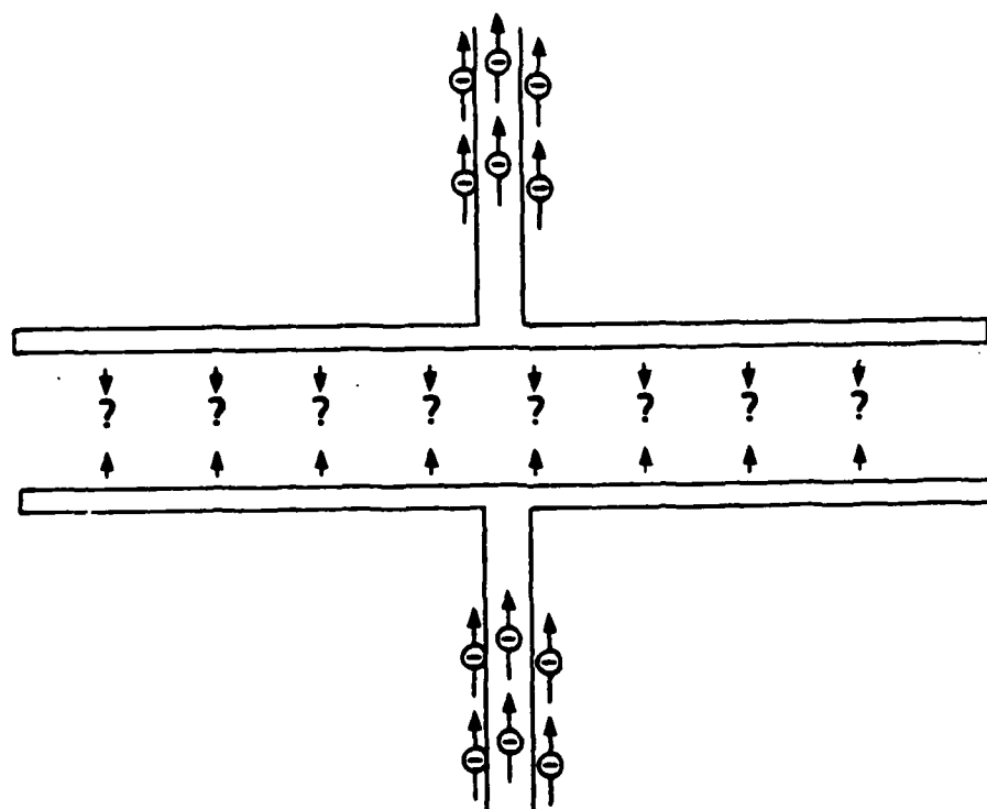
Displacement Current In a Capacitor ??
