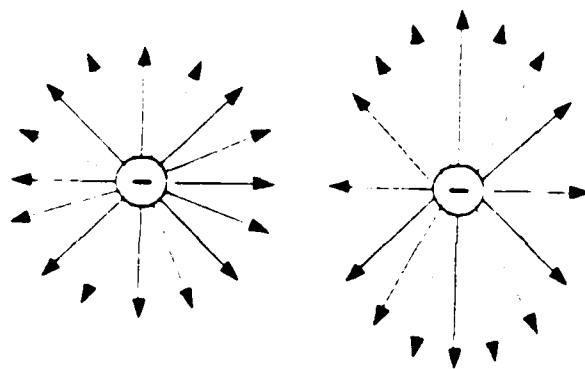
Field of a Charge at Rest and Moving with Constant Velocity
