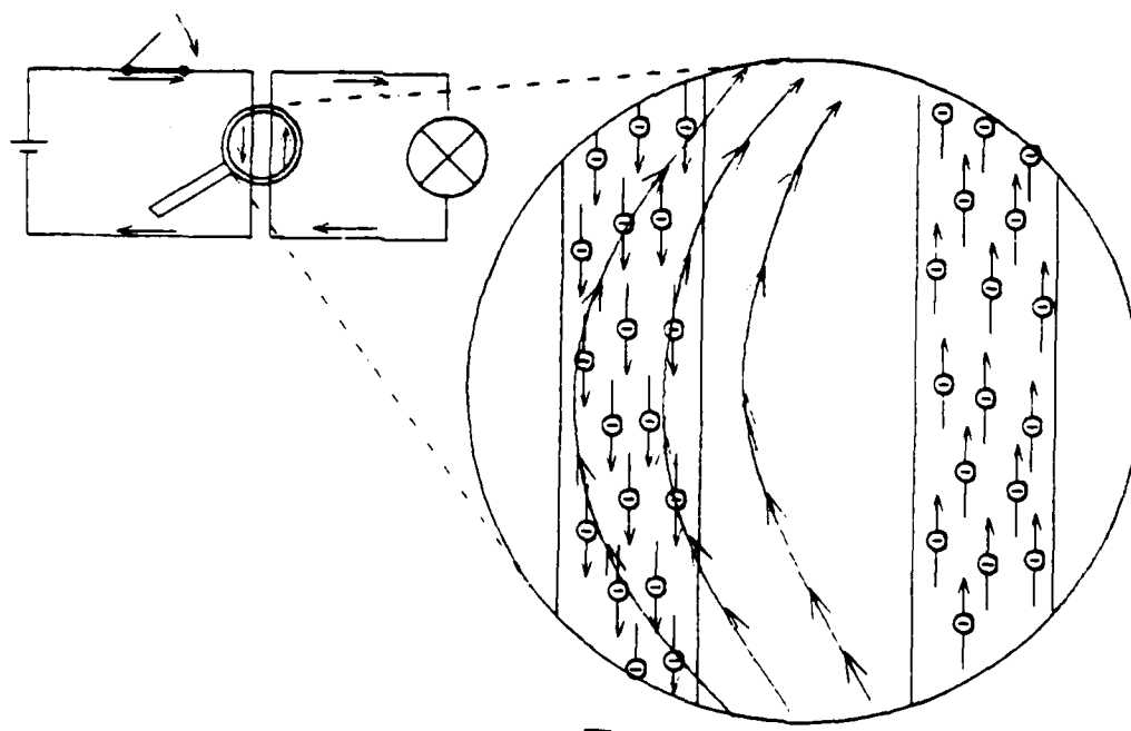
Feedback from the Secondary to the Primary Coil
