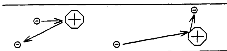
Conduction Mechanism in Metal
