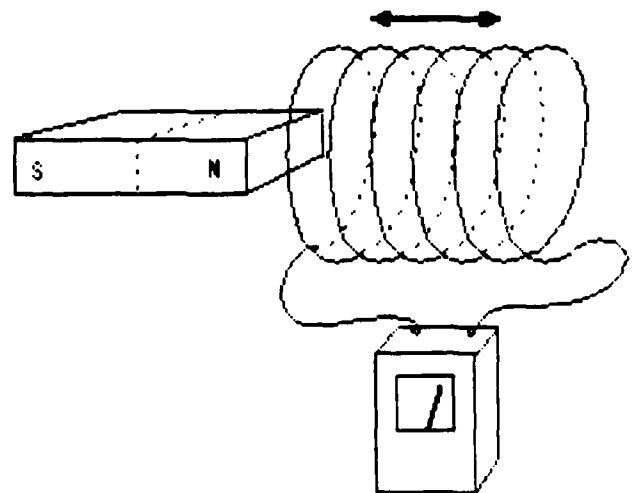
Induction by Moving the Coil
