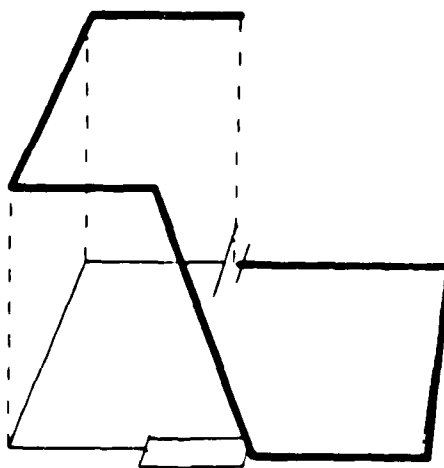
Representation of Voltage (Change of Reference Point)
