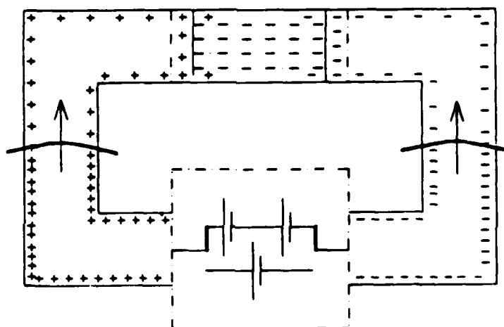
Change of Voltage
