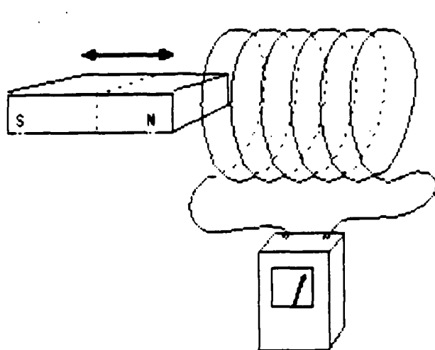
Induction by Moving the Magnet
