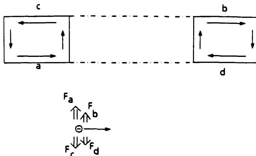
Particle Moving Outside of a Solenoid (View of a Cross-section)
