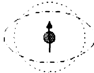
Charged Particle with Different Velocity
