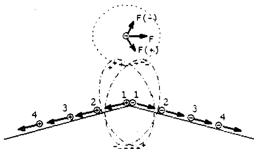
Electron Moving Away from a Current (At Right Angle)
