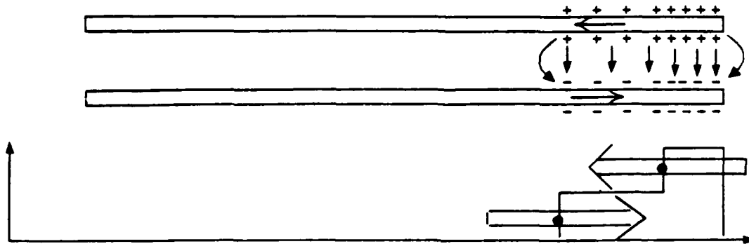
The Voltage is Doubled and the Length Shortened
