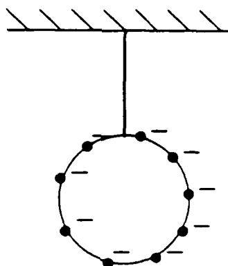
Distribution of Charges on an Isolated Conductor
