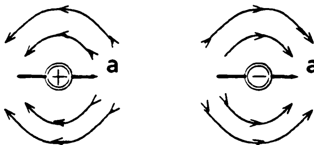
Representation of Circular Waves around an accelerated Charge Carrier
