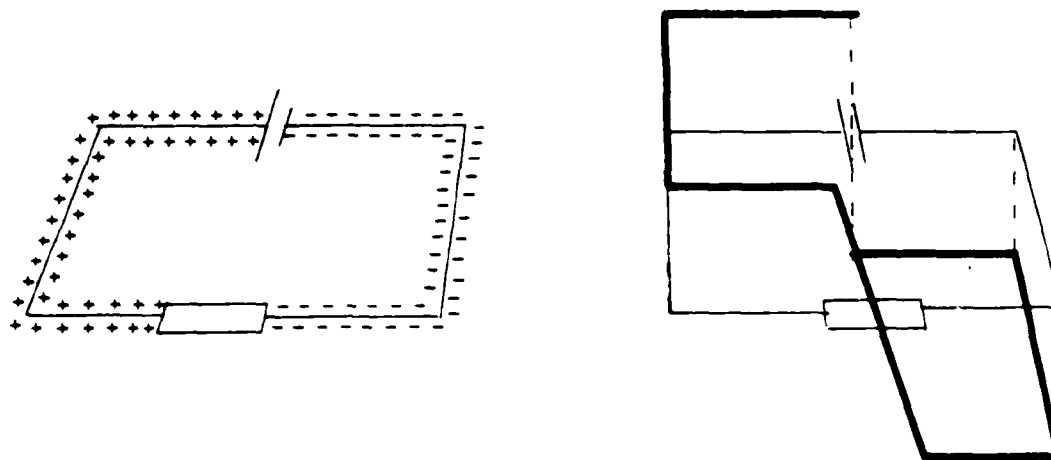
Representation of Voltage
