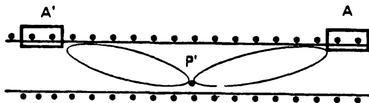
Influence of a Constant Surface Charge (for Points P' of Axis)
