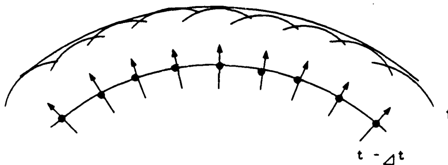
Huygens' Principle
