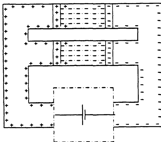
Surface Charge Distribution in Series and Parallel Circuits
