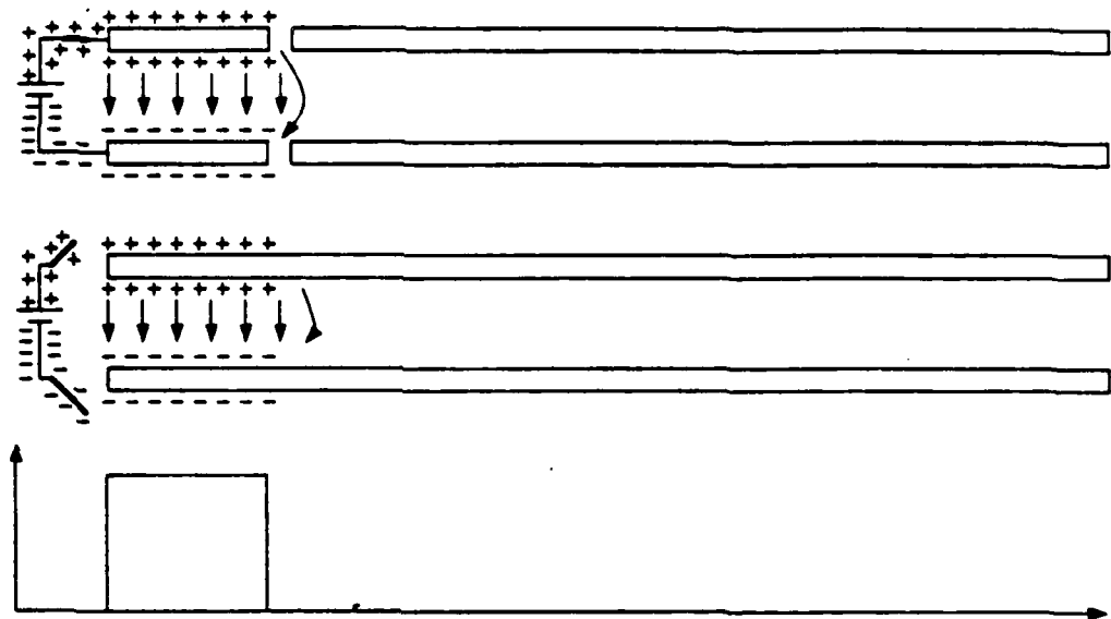
A Charged Transmission Line is Connected to Another One
