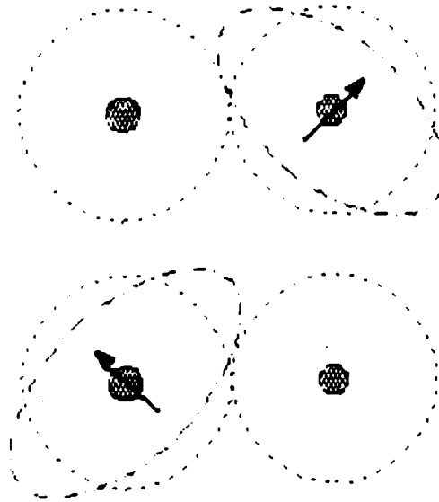
Two Electrons Moving at Right Angles (Represented in Different Frames of Reference)
