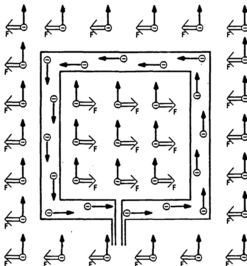
Movement Parallel to a Loop
