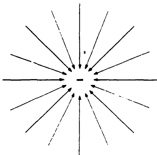
Isolated Charge Carrier at Rest
