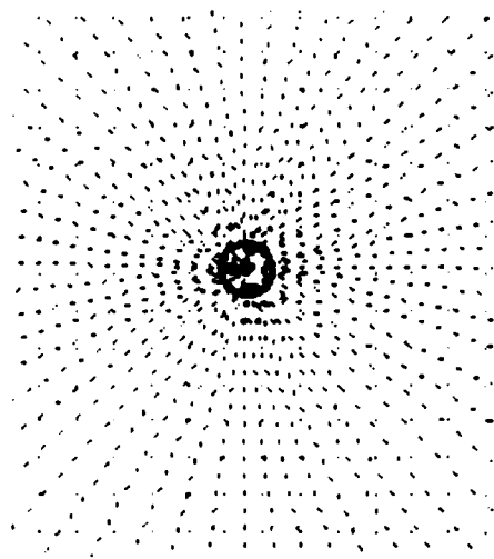
Charged Particle at Rest
