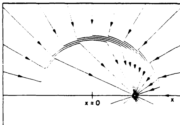
Figure A: A charge initially at rest is accelerated, and moves with constant velocity thereafter.
