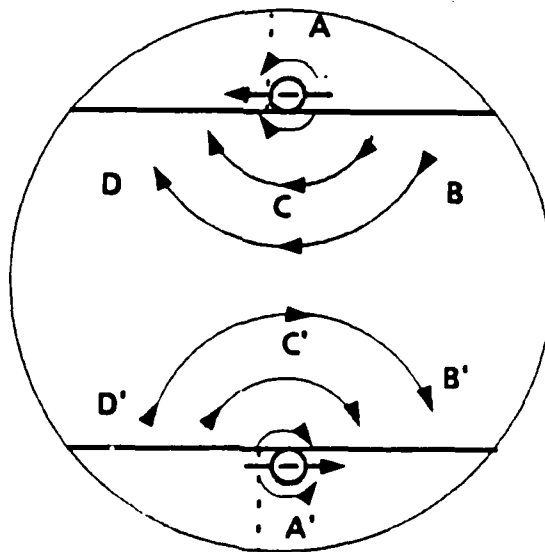
Circular Waves and Wave Propagation
