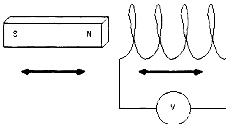
Relative Motion Between Magnet and Coil
