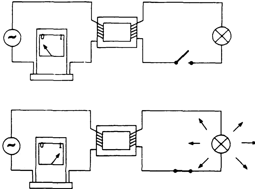
The Current in the Primary Coils is Controlled by the Current in the Secondary Coil
