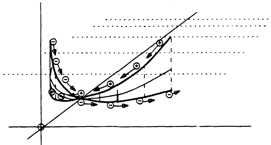
Single Electron Moving Perpendicular to the Plane Formed by the Current and the Electron (Reference Frame of the Single Electron)
