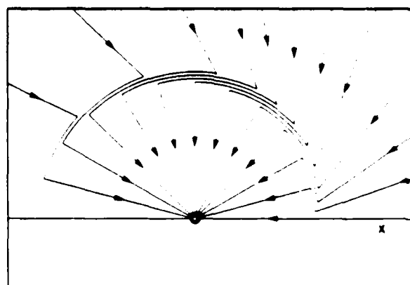
Figure B: A charge that has been moving with constant velocity is abruptly stopped.
