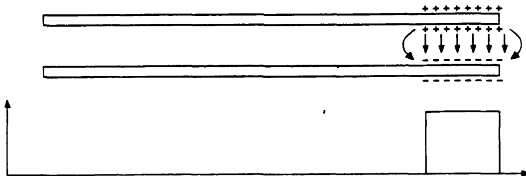
Re-Formation of the Original Situation
