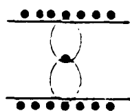
Influence of Opposite Surface Charges
