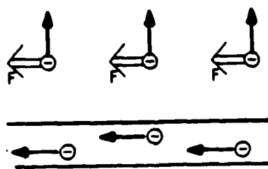
Moving Away from a Current (At Right Angle)
