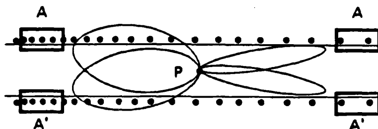
Gradient in Surface Charge Distribution
