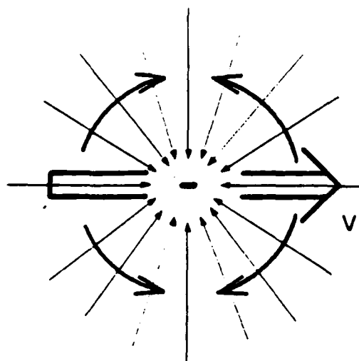
Isolated Charge Carrier Const. Velocity
