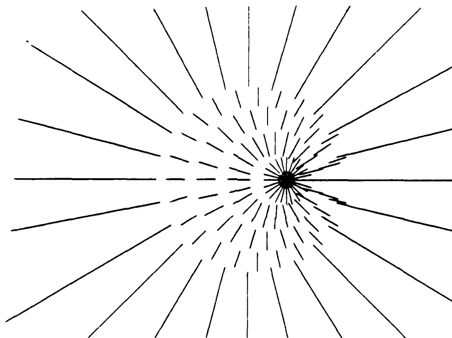
Model for a Moving (Jumping) Charge Carrier
