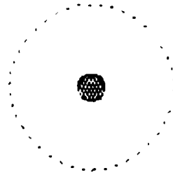
Charged Particle at Rest
