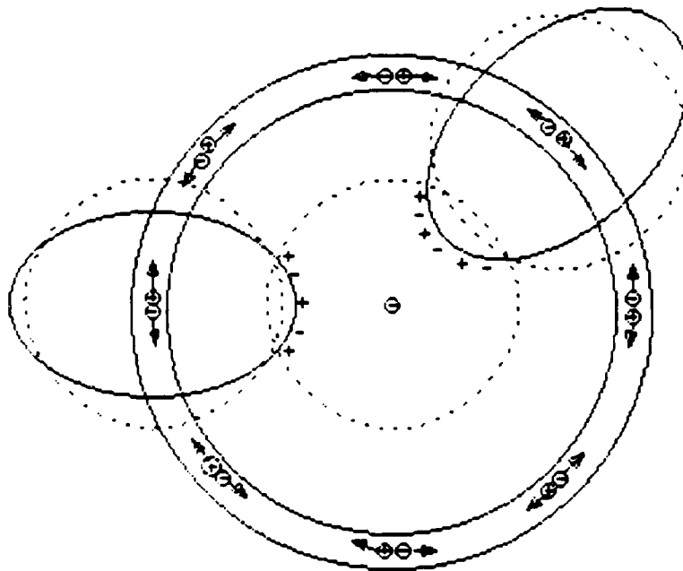
Movement Perpendicular to a Loop
