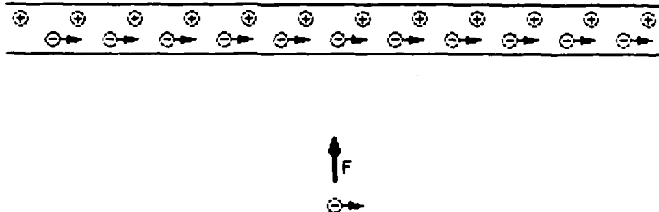
Representation of a Current and a Electron Moving in Parallel
