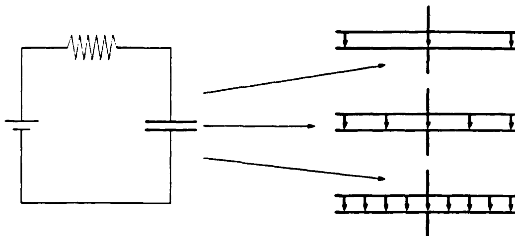
Charging of a Capacitor
