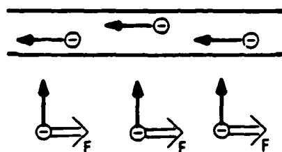
Approaching a Current (At Right Angle)
