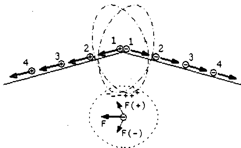
Electron Moving Towards a Current (At Right Angle)
