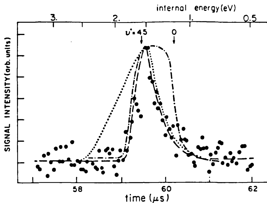
Fig. 5. Forward photofragment spectrum (large solid circles) together with three different simulations. \cdots , impact parameter b=5 and only v''=0 populated. - \cdot - \cdot - , b=0 and all vibrational levels equally populated. - - - , b=2 and vibrational population linear with v'' level. Latter choice is best fit to measured spectrum. Note that - \cdot - \cdot - is displaced slightly to the right for clarity. The left edge is almost congruent with - - - .
