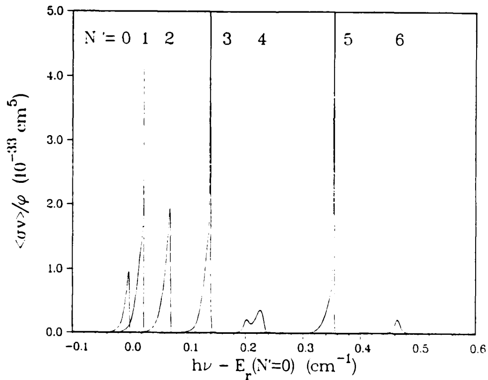
Fig. 8. Detail of 1\Sigma_g + 1\Sigma_g absorption spectrum showing P, R branch progression and resonances.
