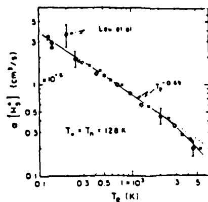
Fig.9. Rate coefficient vs Temperature for e - H_5^+ recombination. (Reprinted from MacDonald et al, 1984).
