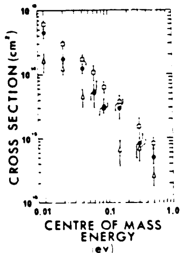
Fig.8. Cross sections for the dissociative recombination of H_2^+ with electrons leading to the individual channels, H+H+H (Circles) and H_2+H (Triangles). Squares show the total recombination cross section. (Reprinted from Mitchell et al, 1983a).
