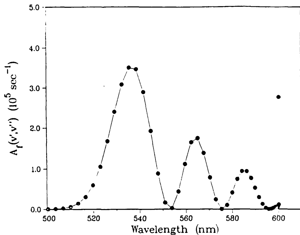
Fig. 7. Round-Round 1\Sigma_g + 1\Sigma_g emission spectrum from v'=107 .
