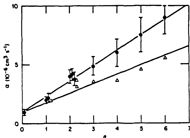
Fig.10. Rate coefficients for the dissociative recombination of water cluster ions (H_2O^+)_n as a function of n as measured by Leu et al, (1973). The full circles are measured data. The open triangles are the same data normalised to a temperature of 540K assuming a variation according to T^{-1} . (Reprinted from Bottcher, 1978).
