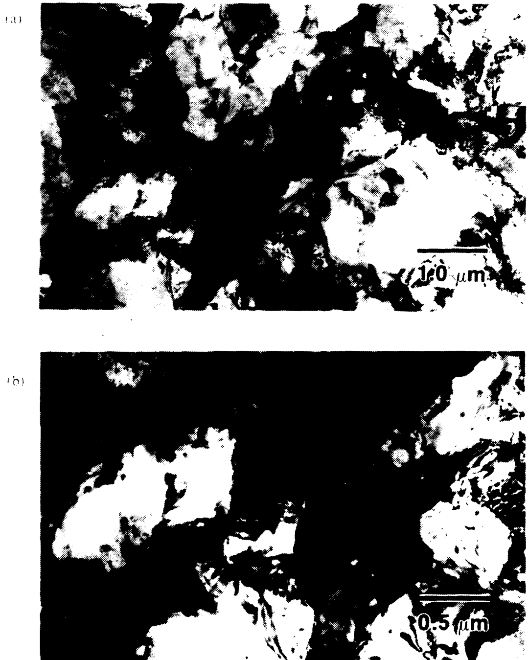
Figure 4.15 6% Mg-1% Li Aged at 120°C for 168 Hours, Dislocations
