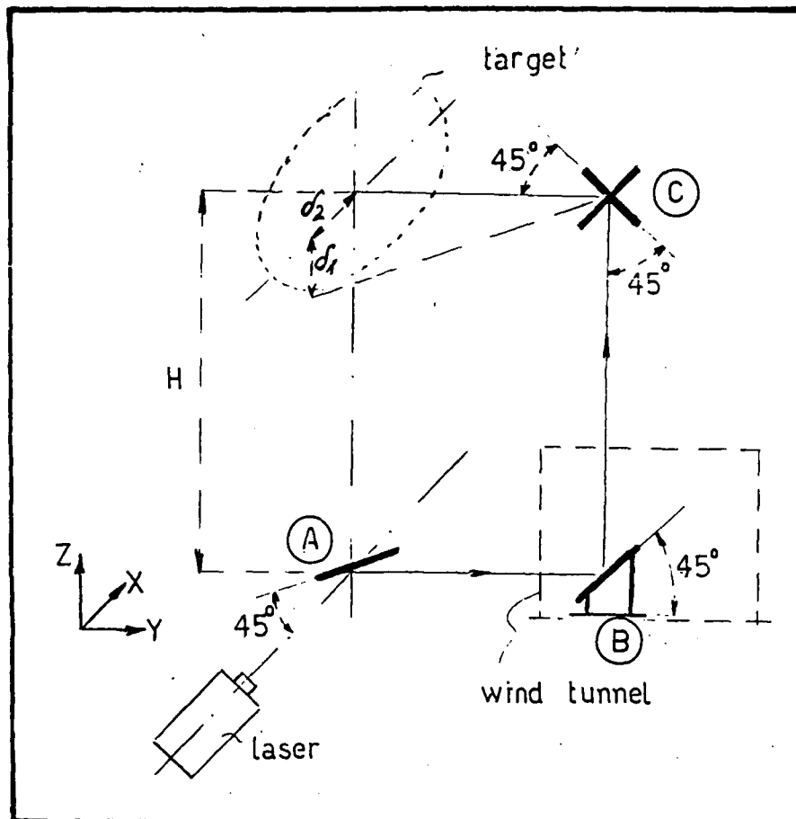
fig.A4-3 : alignement procedure for the perpendicularity of the collecting optics axis to the wind tunnel axis.
