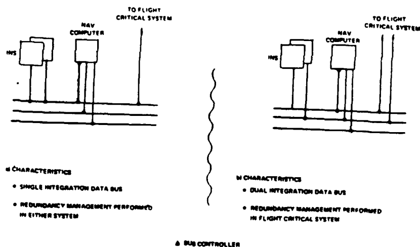
Integration Concepts Using Parallel Avionics Architecture
